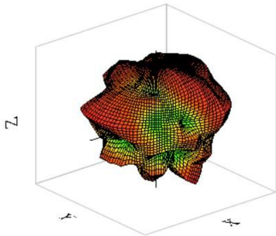
WIFI 2400MHz
