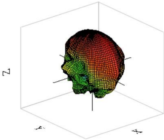
WIFI 5350MHz
