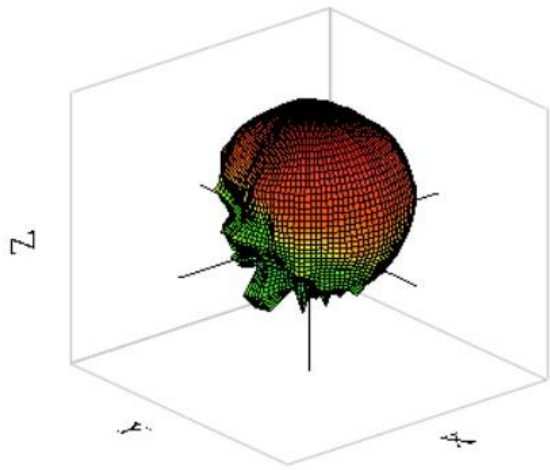
WIFI 5600MHz
