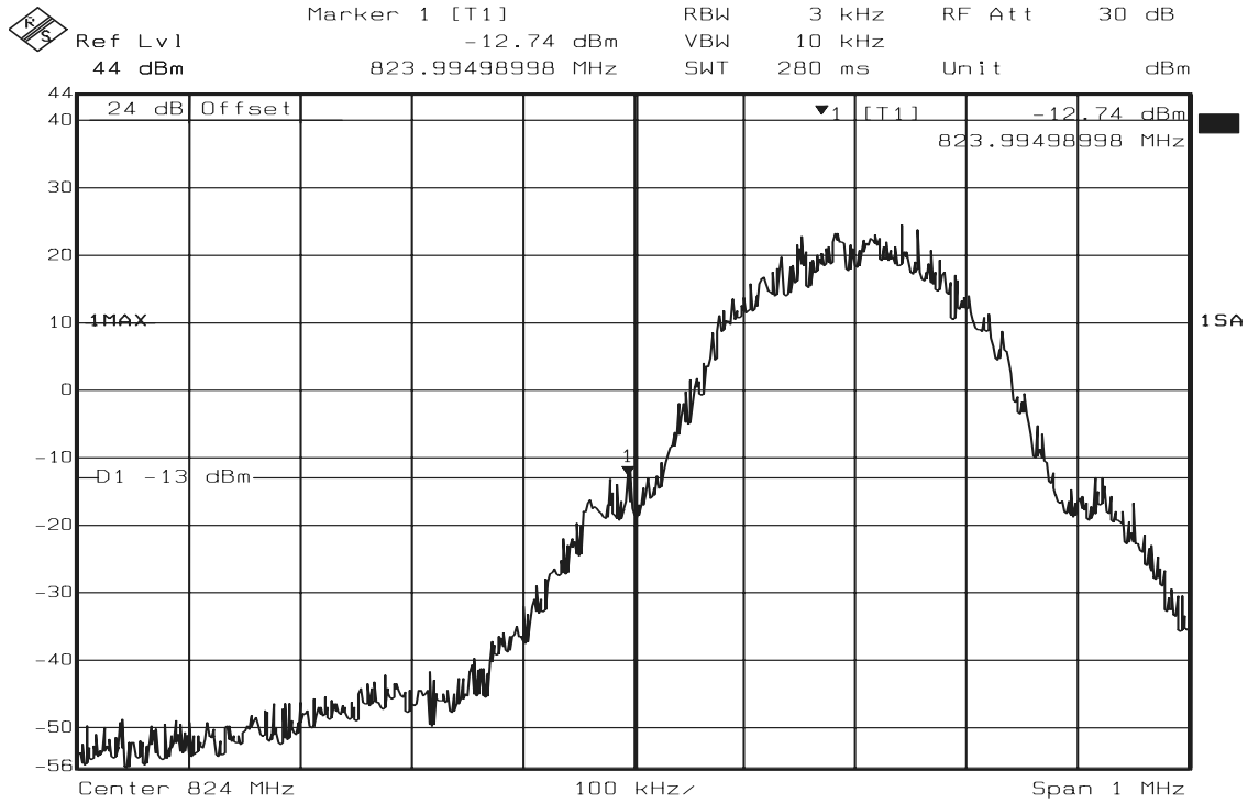
Figure 9-1: Band Edge emissions – GSM CH Low
