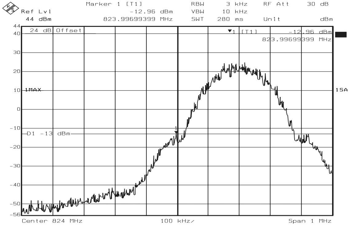
Figure 9-3: Band Edge emissions – GPRS CH Low
