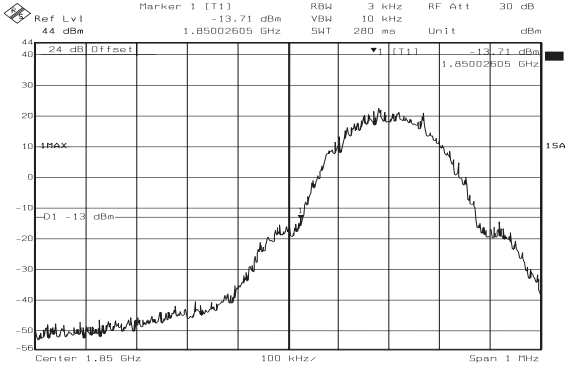
Figure 10-1: Band Edge emissions – GSM CH Low
