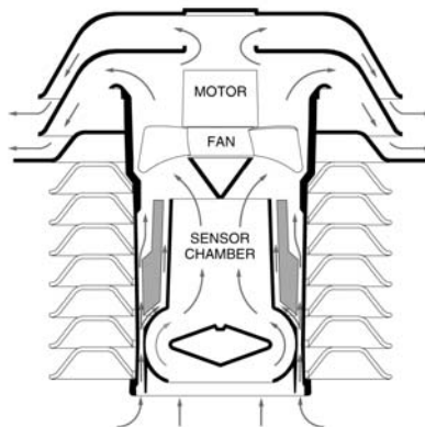
Fan-Aspirated Radiation Shield in Operation
