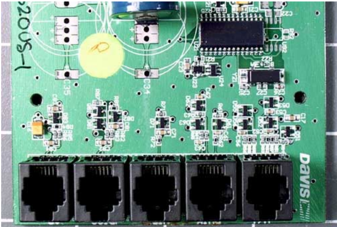
RF PCB – Front Section 1
