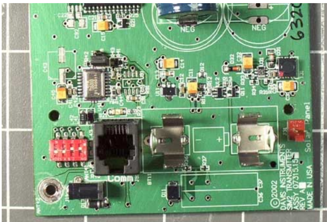
RF PCB Front Section 2
