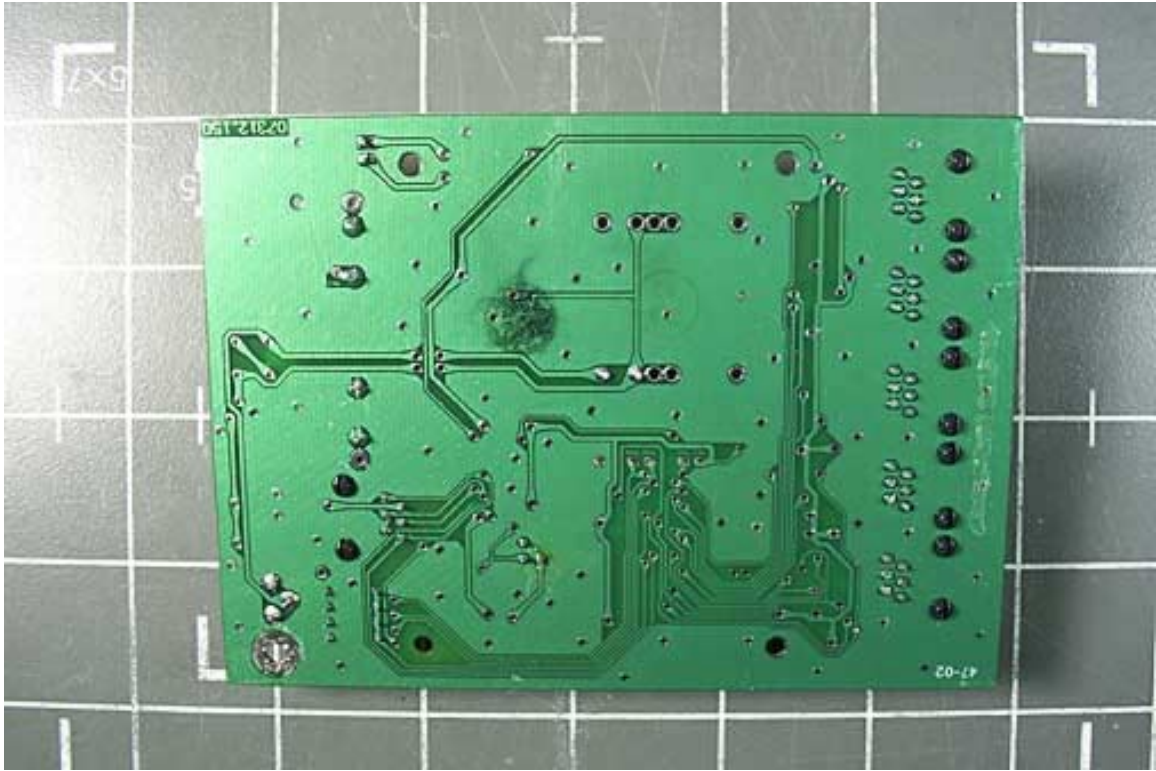
Close-Up RF PCB – Overall Back
