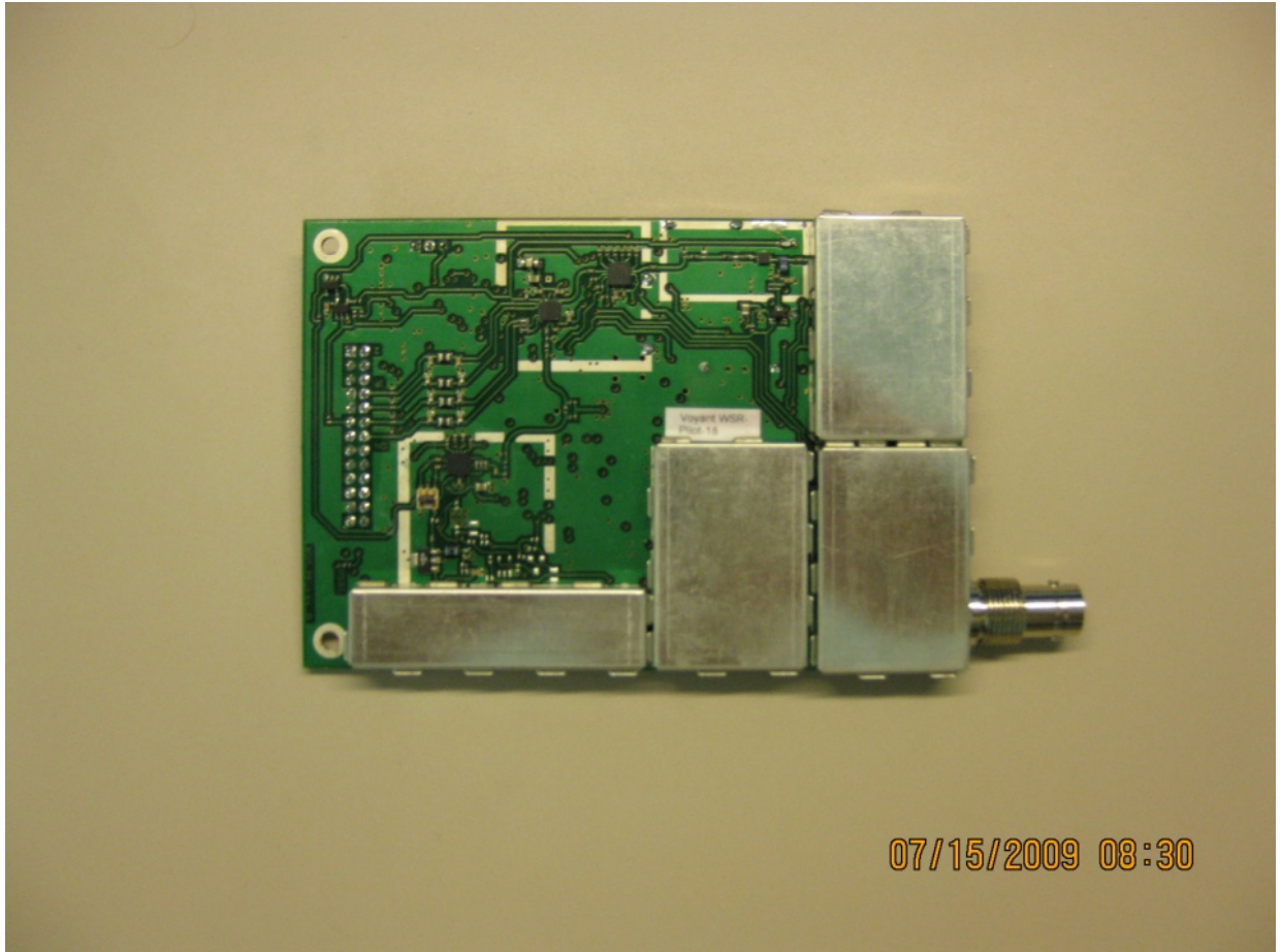
Figure 3: RF PCB with Shields - Front
