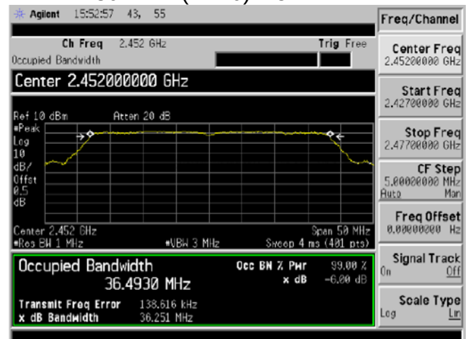
802.11n (HT40)2452MHz
