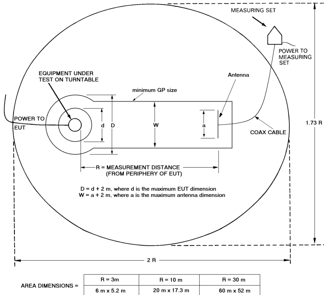
Diagram 1 Test setup for radiated emissions tested on Open Area Test Site (OATS)
