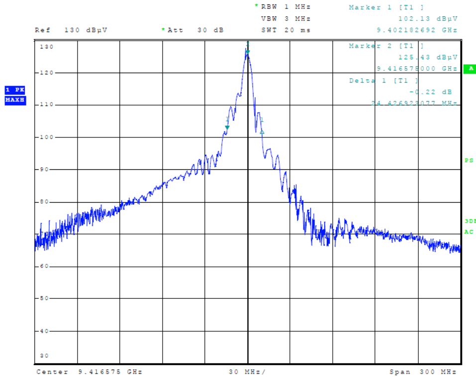
Figure 4 Plot of analyzer screen showing 23-dB OBW (Pulse Expansion 0.25 nm)
