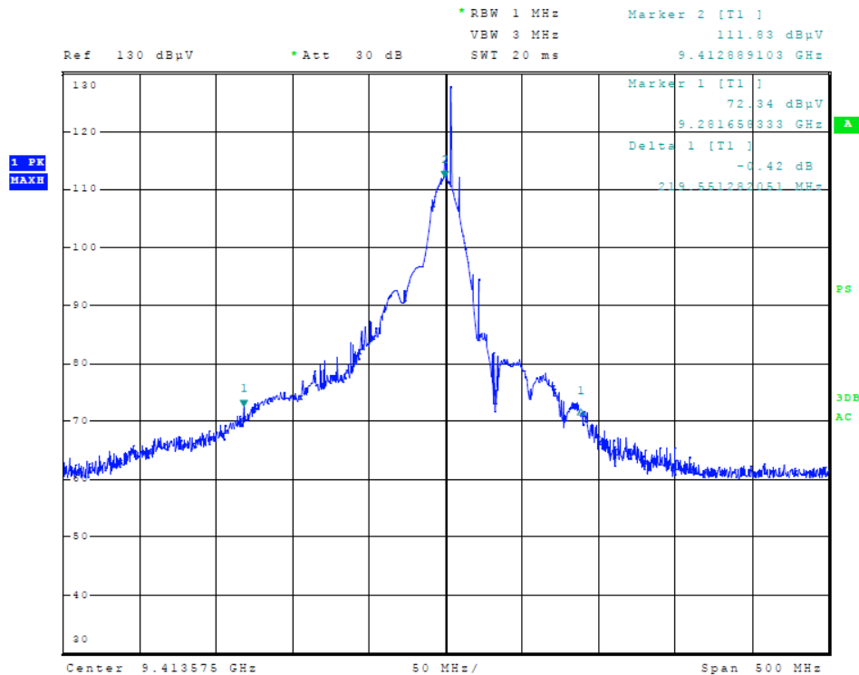
Figure 3 Plot of analyzer screen showing 40-dB occupied bandwidth (0.25 nm)
