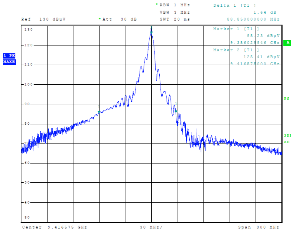
Figure 5 Plot of analyzer screen showing 40-dB OBW (Pulse Expansion 1/2 nm)
