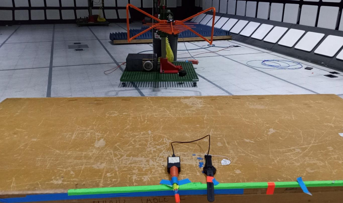
30 MHz – 1 GHz Test Setup
