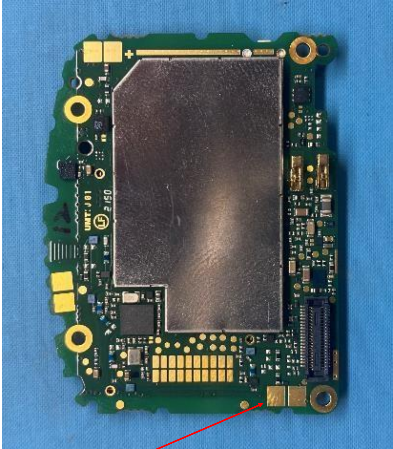
Antenna connection Points
