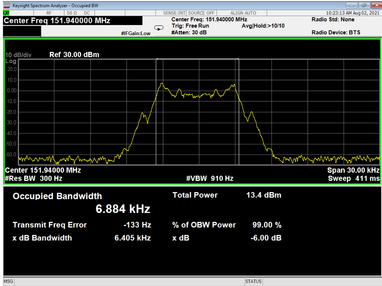
Figure 11 - Bandwidth, 151.940 MHz
