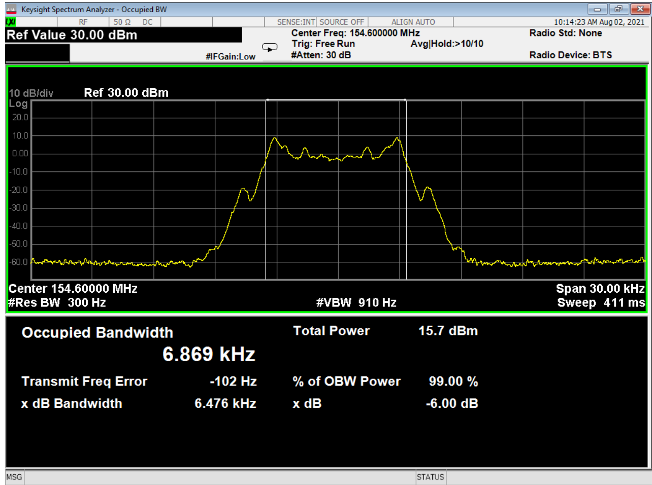
Figure 13 - Bandwidth, 154.600 MHz
