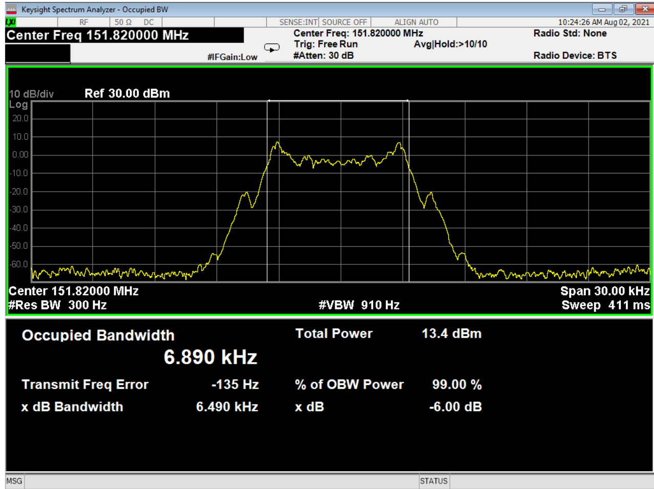
Figure 9 - Bandwidth, 151.820 MHz
