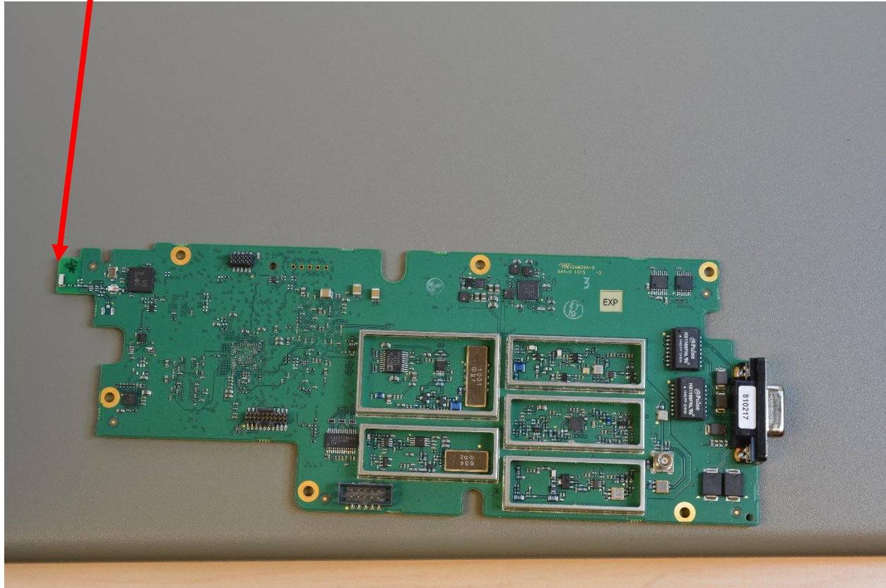
Internal Photographs of transmitter Antenna
