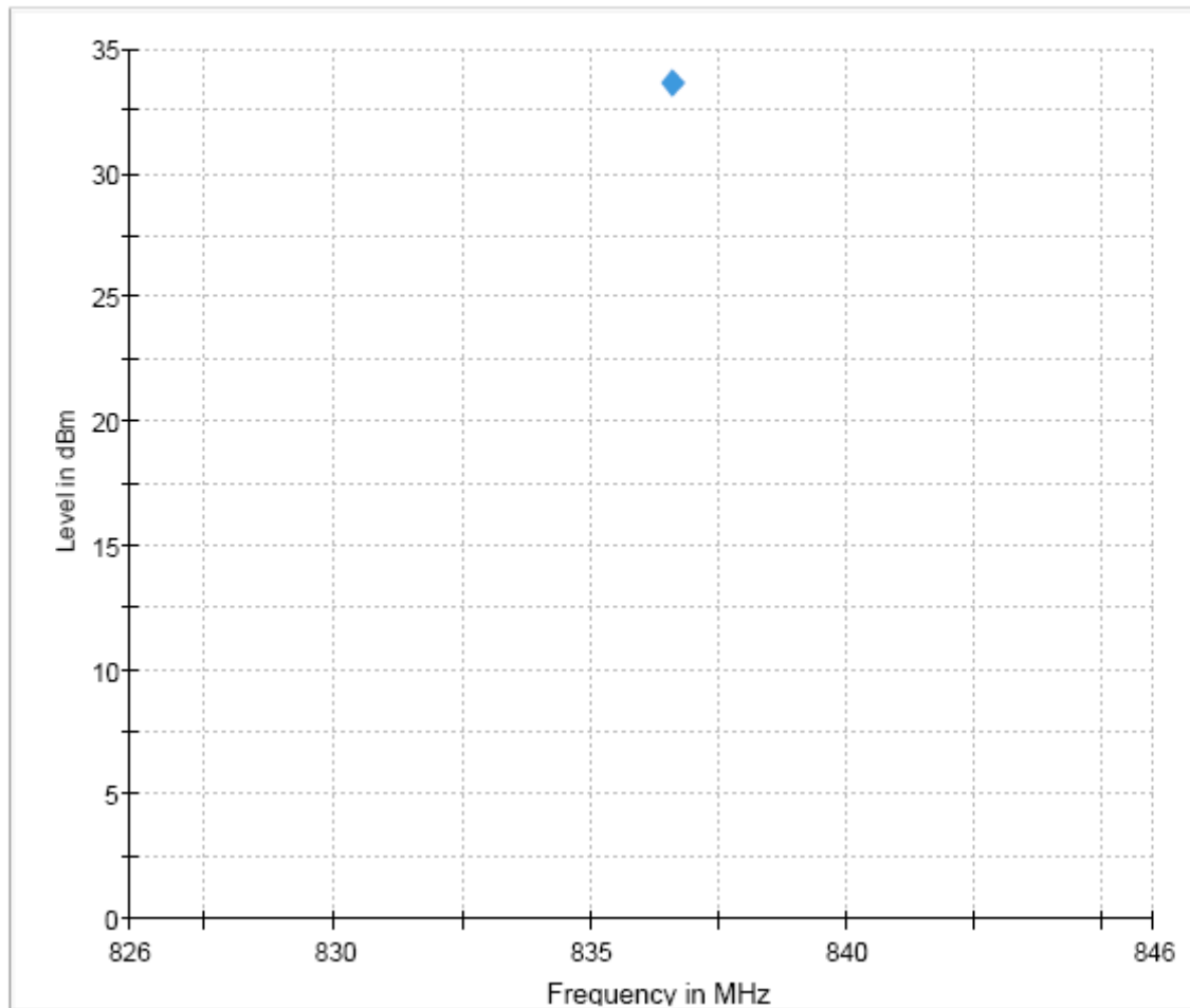
EIRP 836
