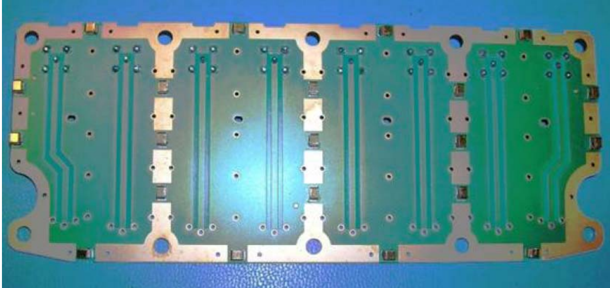
GTS8XX Internal photograph of Qtr Wave Stub Board (bottom side)
