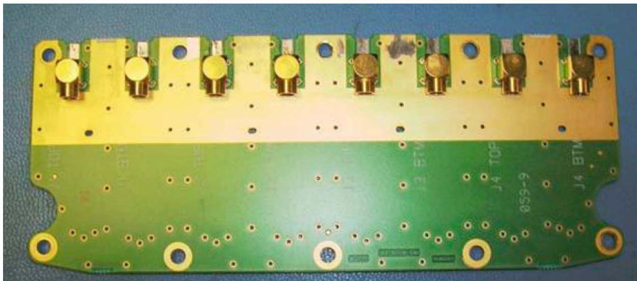
GTS8XX Internal photograph of Qtr Wave Stub Board (top side)
