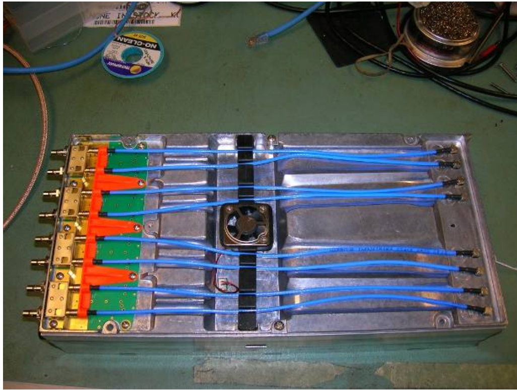
GTS8XX External photograph of RF cables within the chassis
