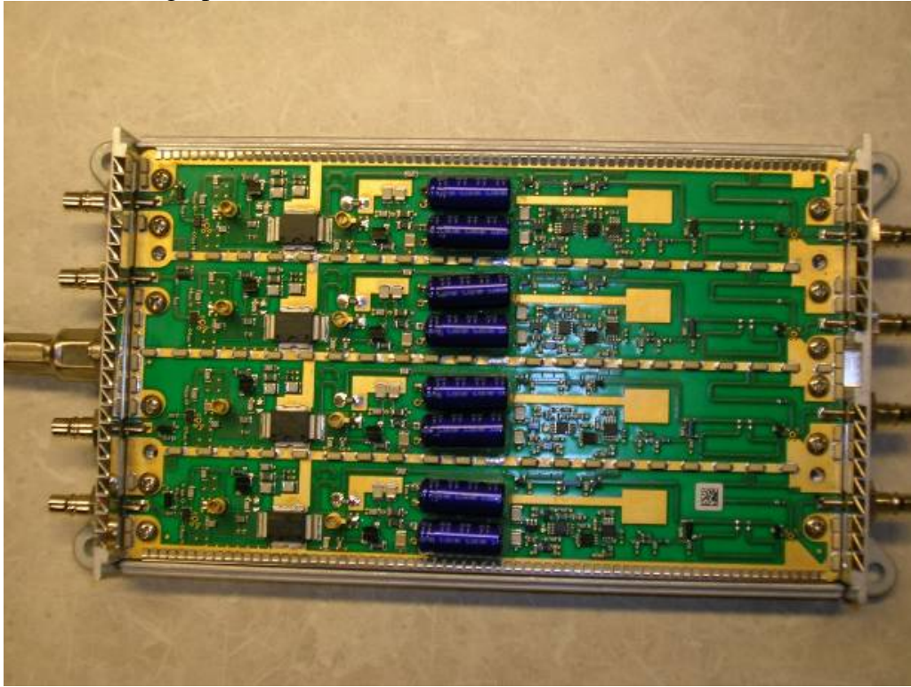
GPA65 Internal photograph of the Transmitter board
