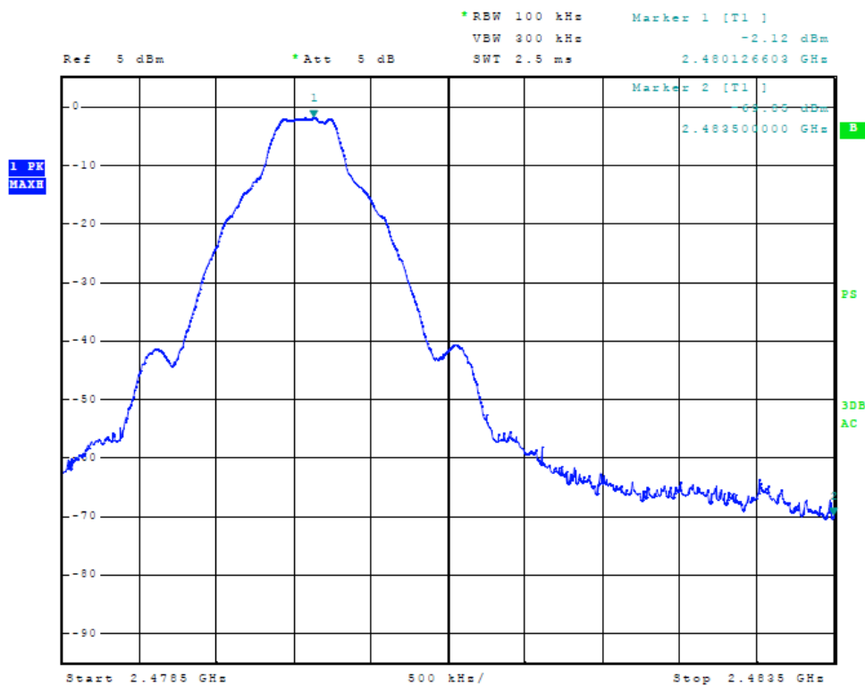
Figure Twenty-eight High Frequency Band Edge
