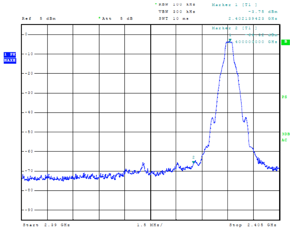
Figure Twenty-seven Low Frequency Band Edge
