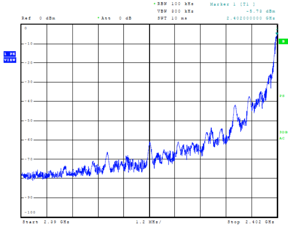
Figure 3 Plot of Transmitter Emissions (Low Band Edge Protocol 1)
