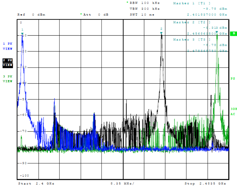
Figure 5 Plot of Transmitter Emissions (Output in Operational Band Protocol 2)
