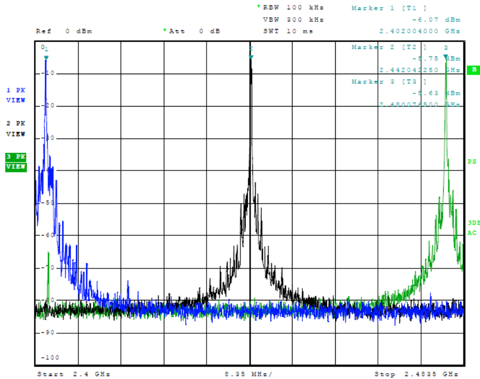
Figure 1 Plot of Transmitter Emissions (Output in Operational Band Protocol 1)
