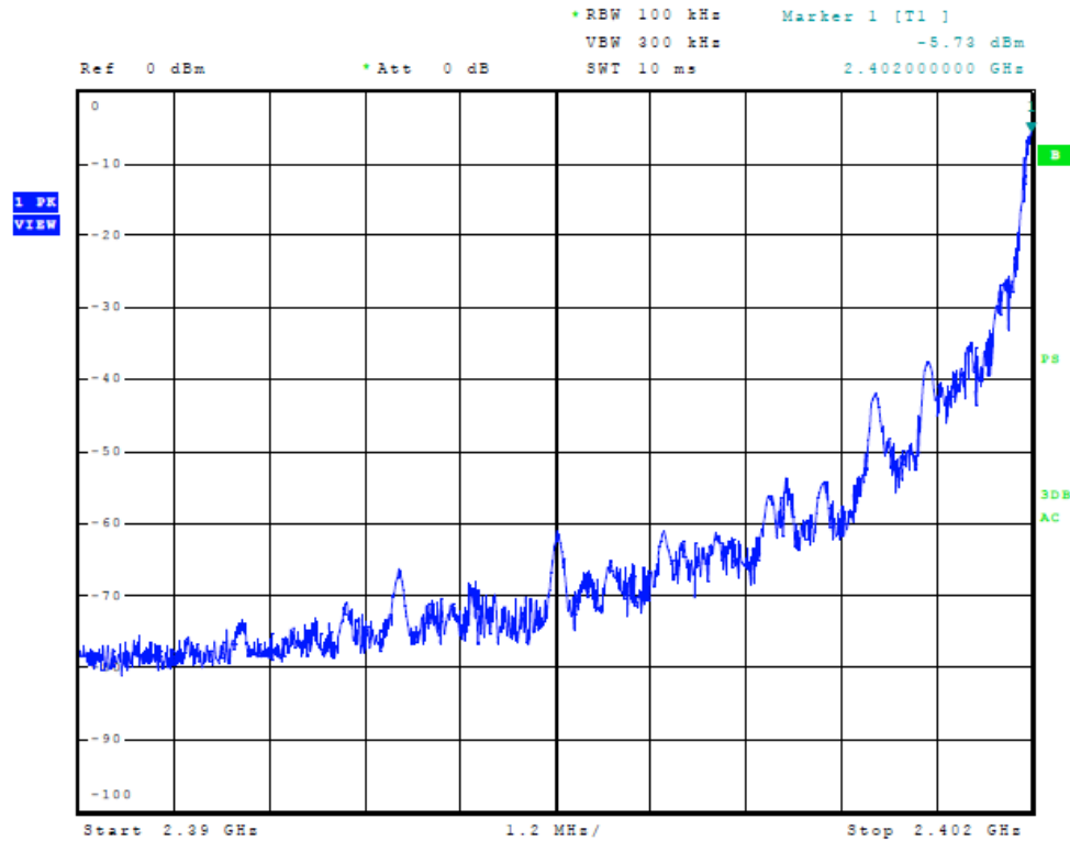
Figure 7 Plot of Transmitter Emissions (Low Band Edge Protocol 2)
