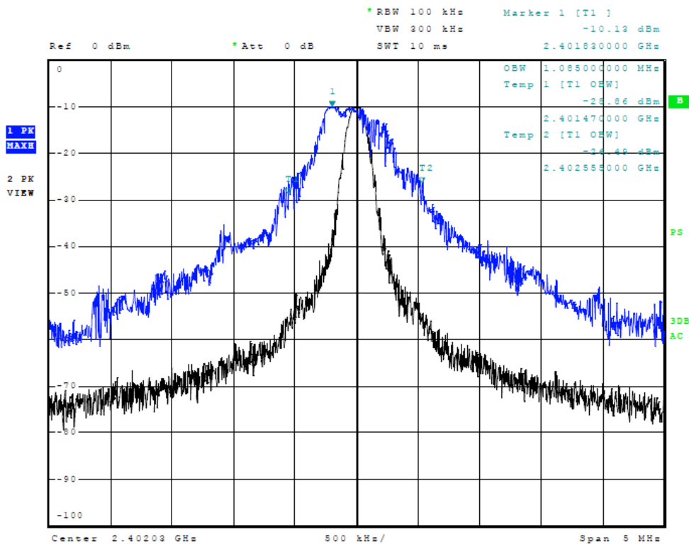
Figure 6 Plot of Transmitter Emissions (Occupied Bandwidth Protocol 2)
