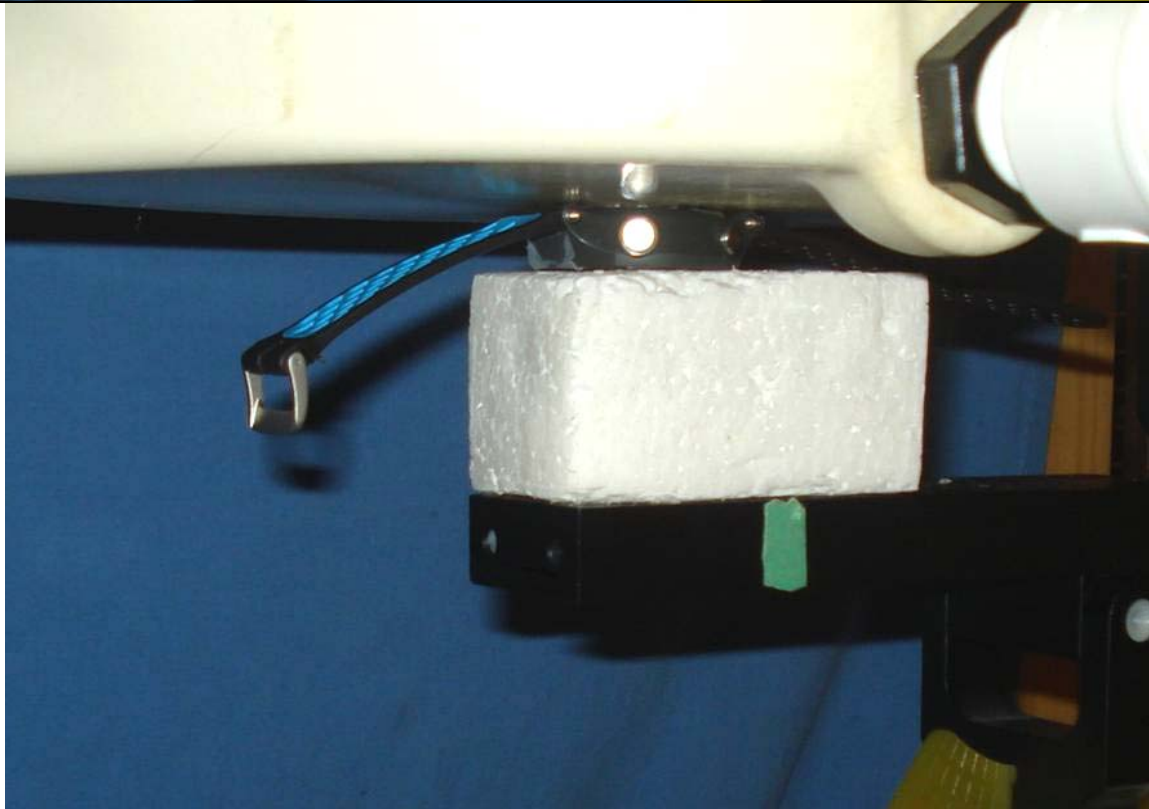
Test Setup
