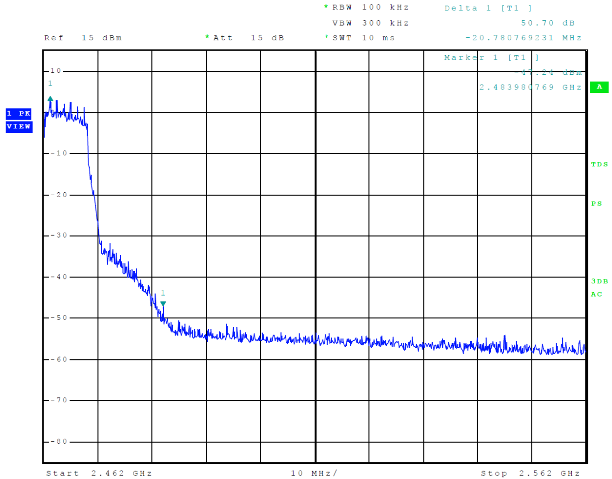
Figure 8 Plot of Transmitter Emissions High Band Edge Mode 2, 802.11g
