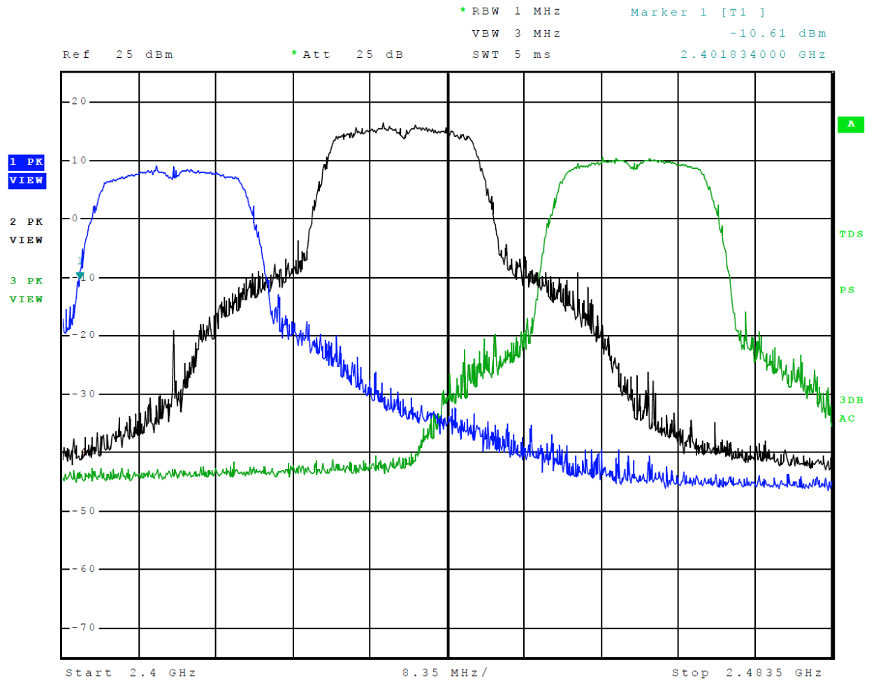
Figure 2 Plot of Transmitter Operation in 2412-2462 MHz Mode 2, 802.11g
