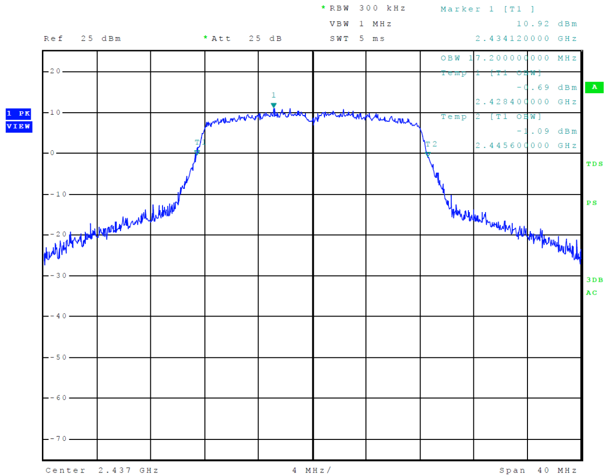
Figure 13 Plot of 99% Occupied Bandwidth Mode 2, 802.11g
