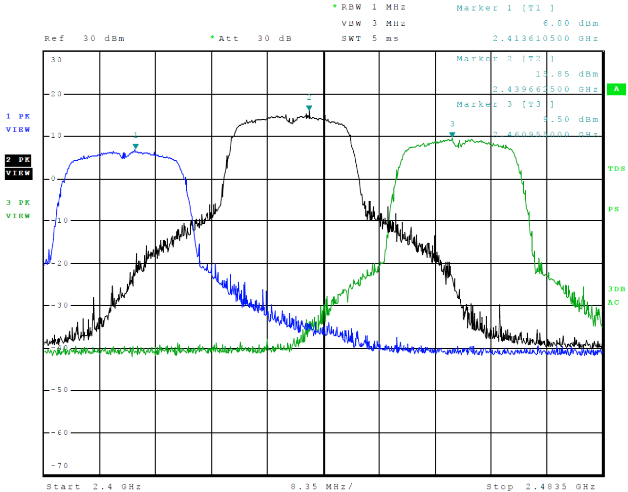
Figure 3 Plot of Transmitter Operation in 2412-2462 MHz Mode 3, 802.11n
