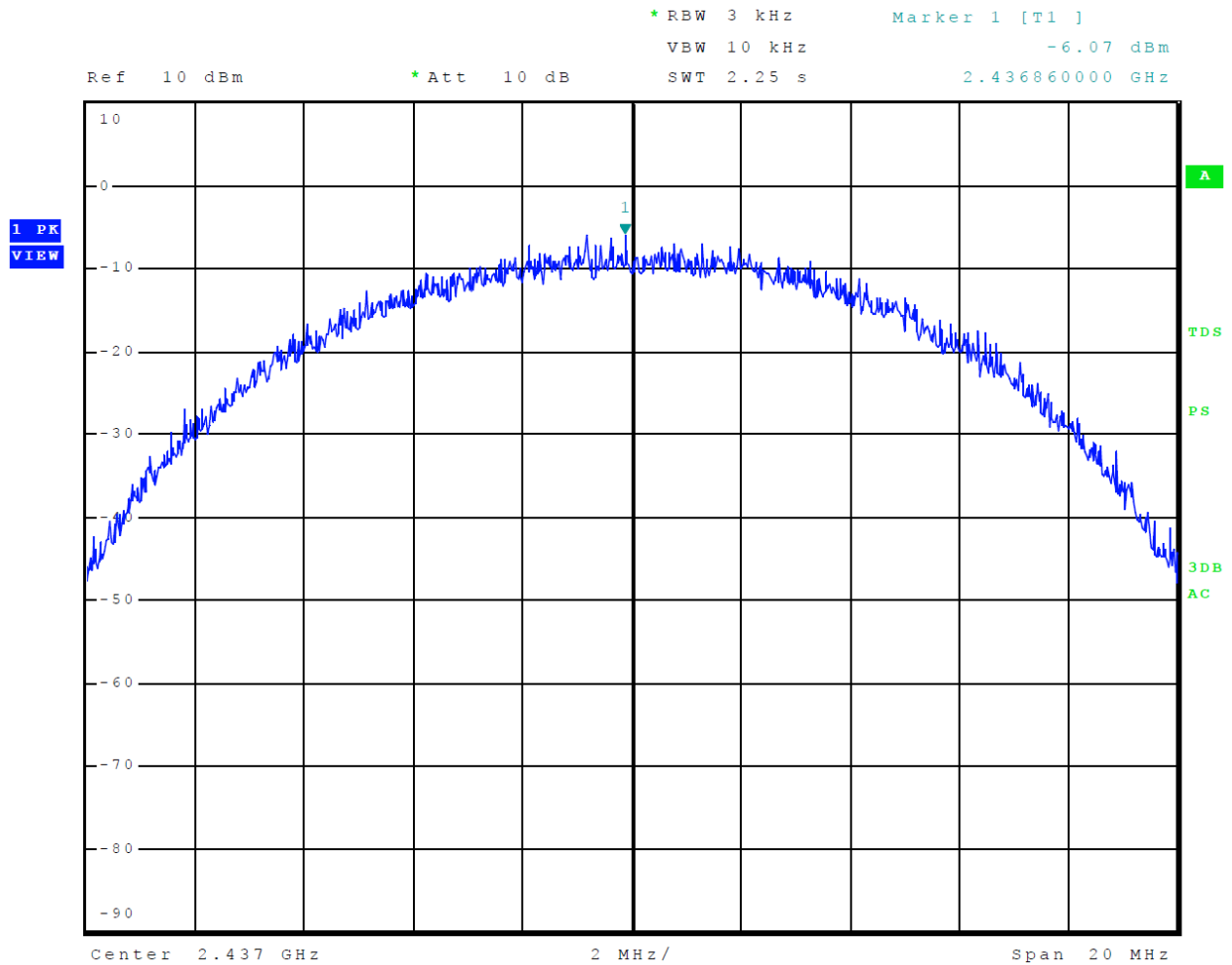
Figure 16 Plot of Transmitter Power Spectral Density Mode 1, 802.11b
