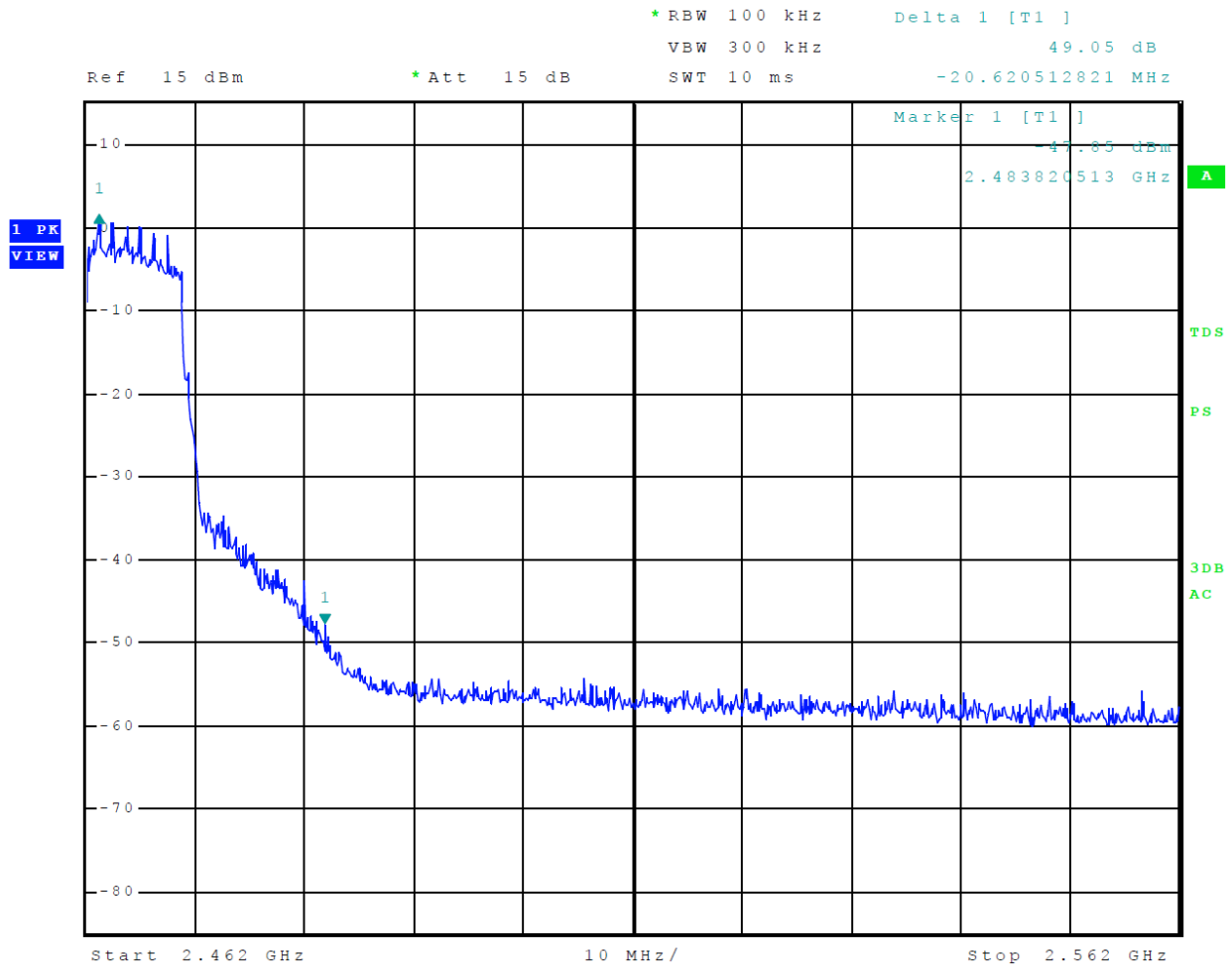
Figure 9 Plot of Transmitter Emissions High Band Edge Mode 3, 802.11n
