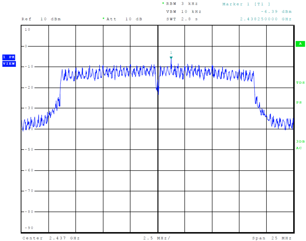
Figure 18 Plot of Transmitter Power Spectral Density Mode 3, 802.11n
