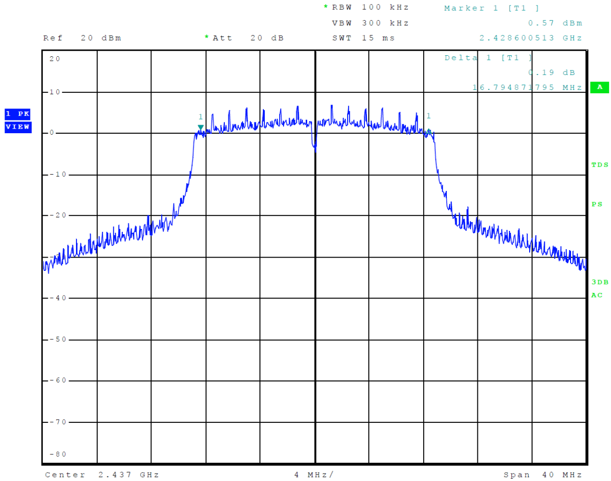
Figure 14 Plot of 6-dB Occupied Bandwidth Mode 3, 802.11n
