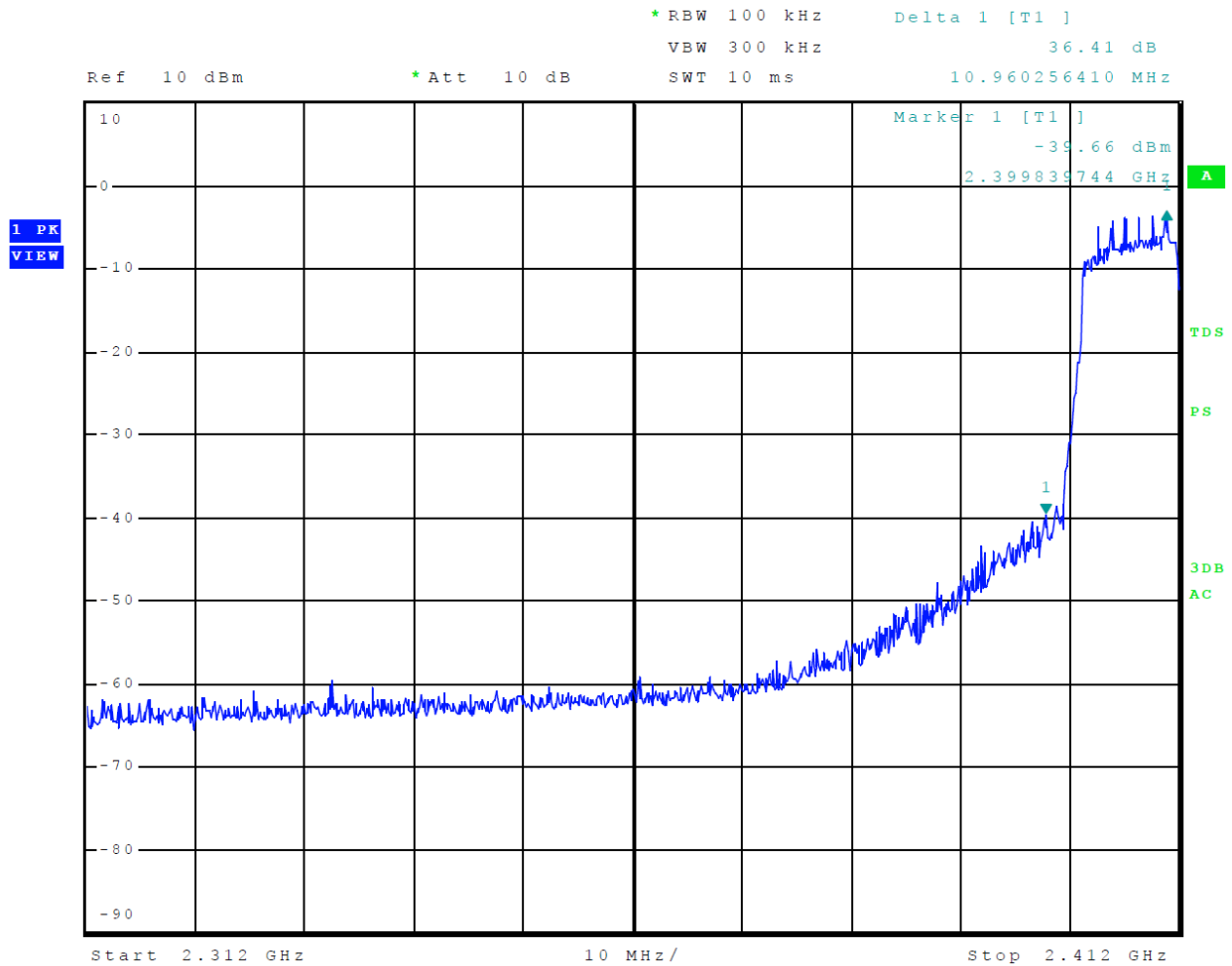
Figure 6 Plot of Transmitter Emissions Low Band Edge Mode 3, 802.11n
