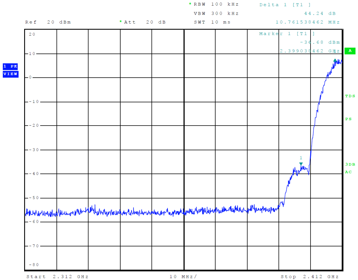
Figure 4 Plot of Transmitter Emissions Low Band Edge Mode 1, 802.11b
