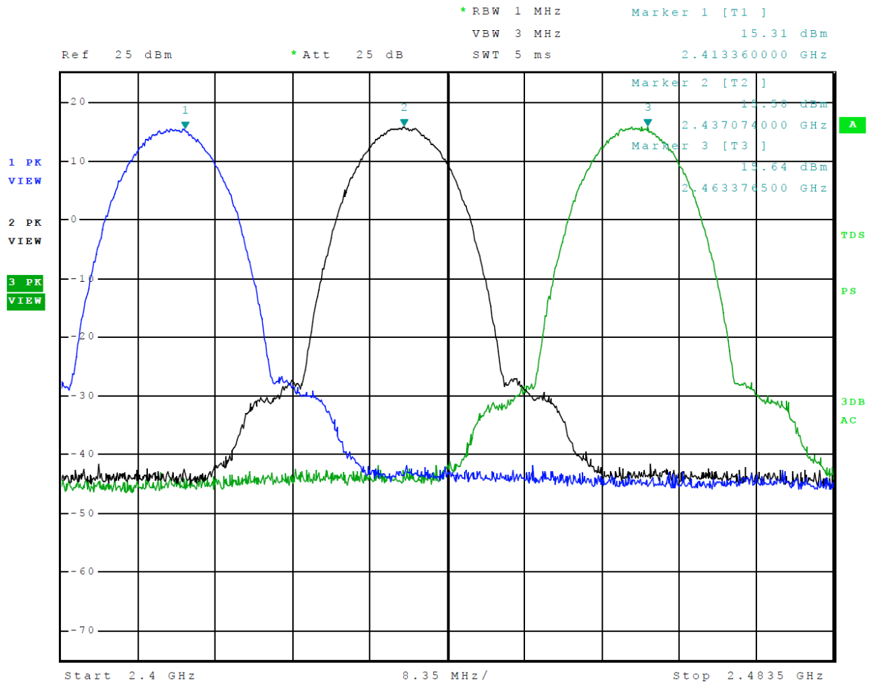
Figure 1 Plot of Transmitter Operation in 2412-2462 MHz Mode 1, 802.11b
