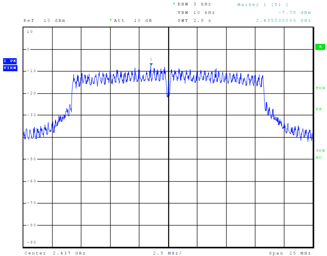
Figure 17 Plot of Transmitter Power Spectral Density Mode 2, 802.11g
