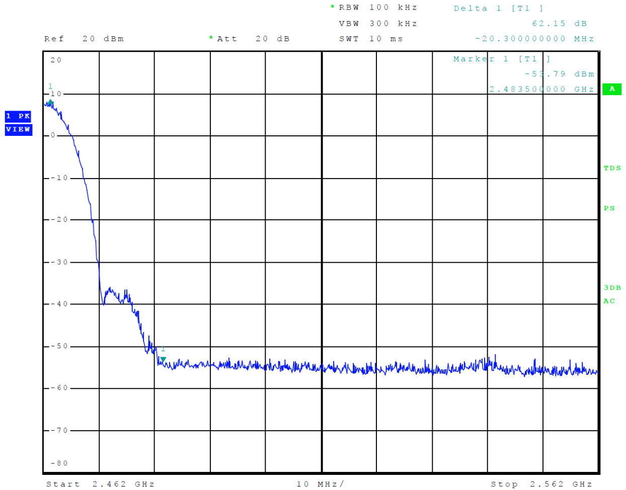
Figure 7 Plot of Transmitter Emissions High Band Edge Mode 1, 802.11b
