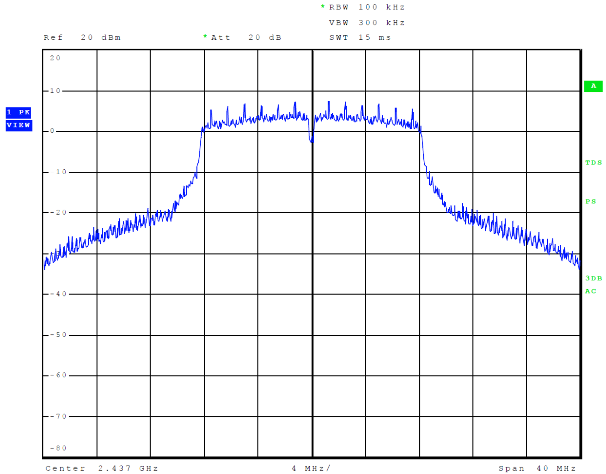
Figure 12 Plot of 6-dB Occupied Bandwidth Mode 2, 802.11g
