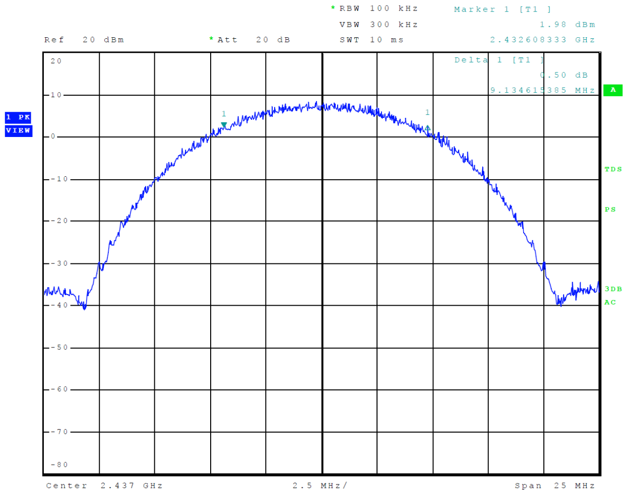
Figure 10 Plot of 6-dB Occupied Bandwidth Mode 1, 802.11b
