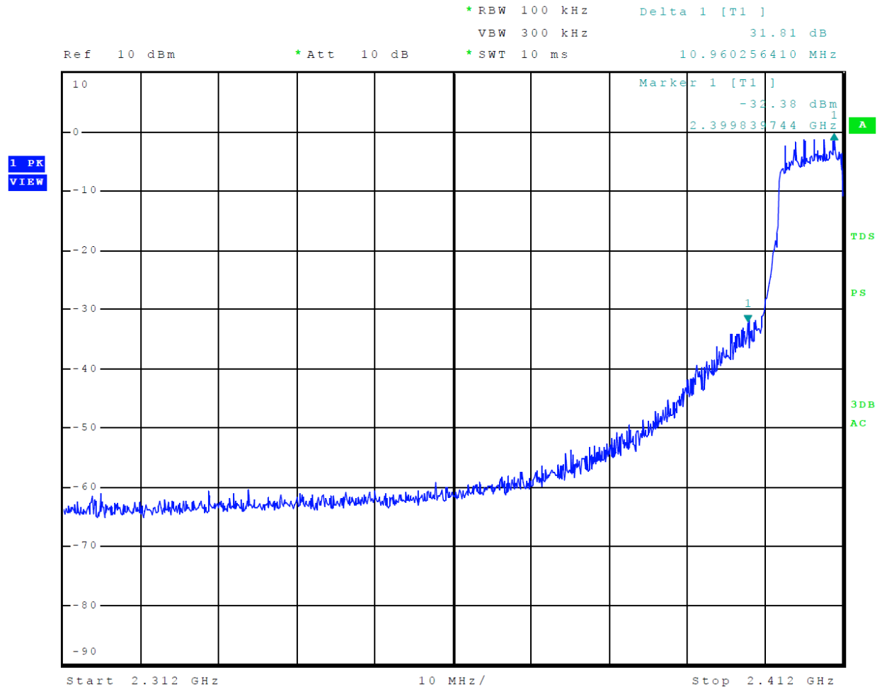
Figure 5 Plot of Transmitter Emissions Low Band Edge Mode 2, 802.11g
