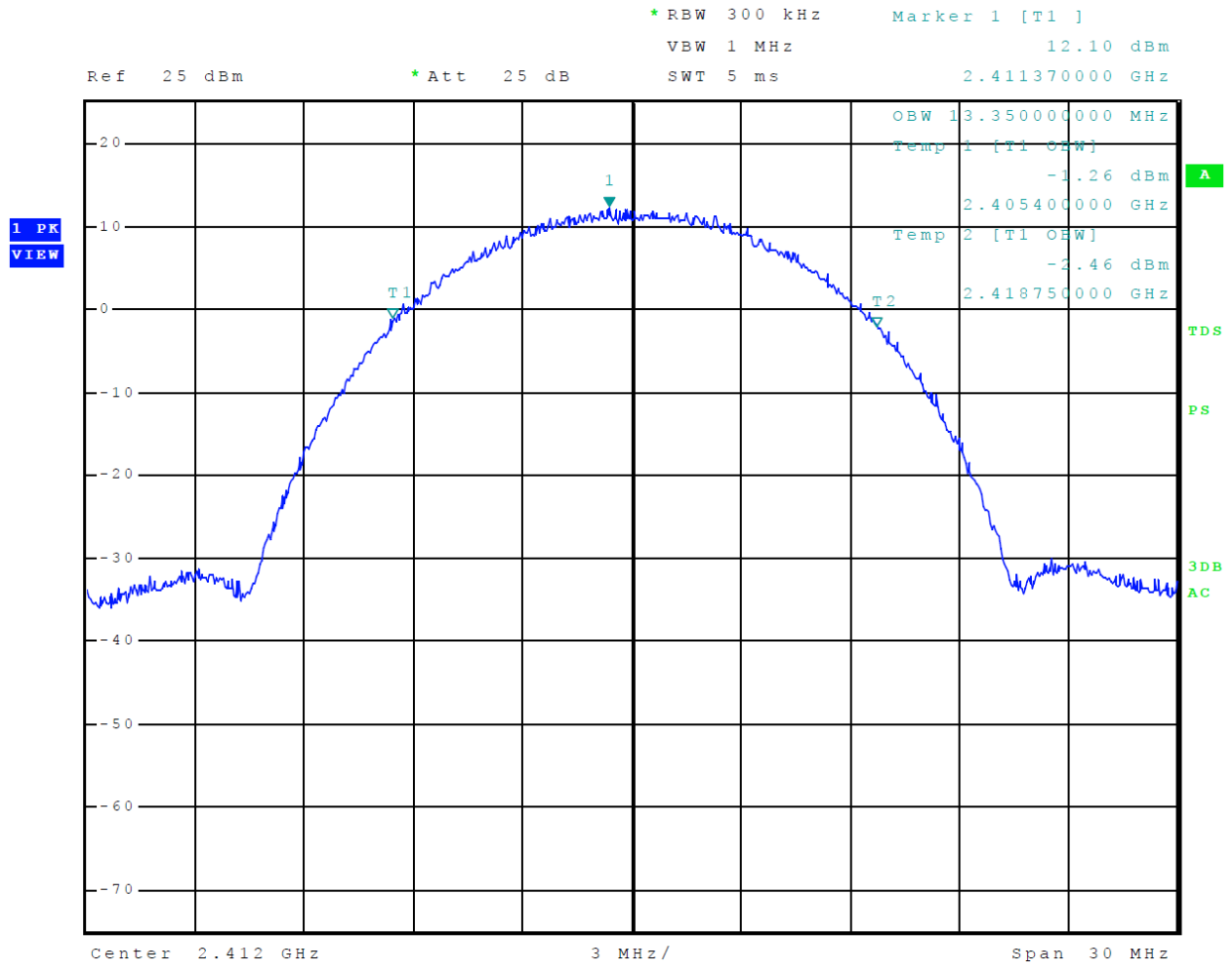
Figure 11 Plot of 99% Occupied Bandwidth Mode 1, 802.11b
