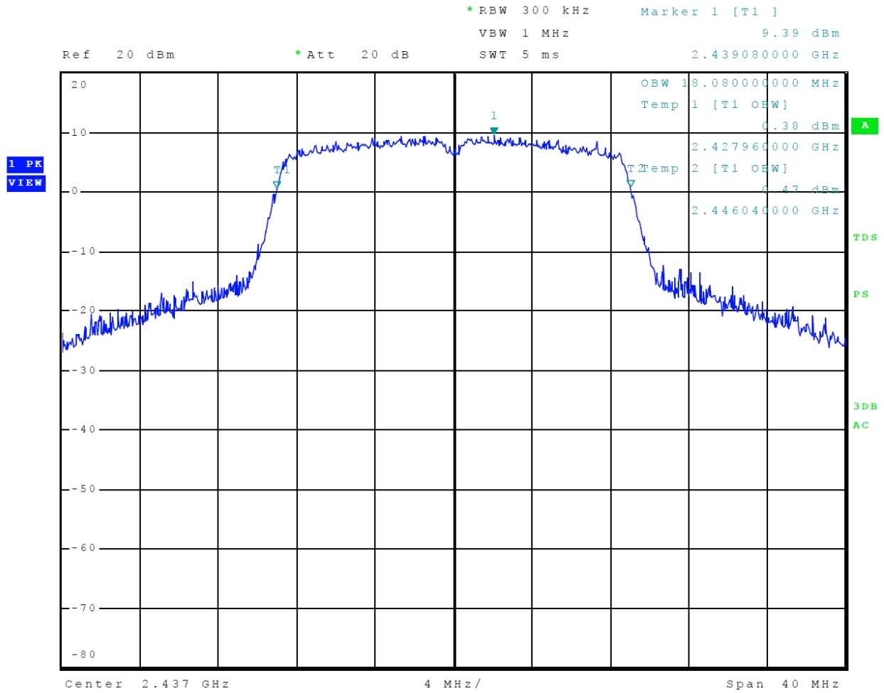
Figure 15 Plot of 99% Occupied Bandwidth Mode 3, 802.11n
