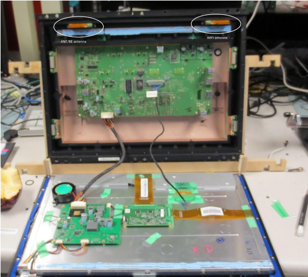
WIFI and ANT/BLE antenna location
