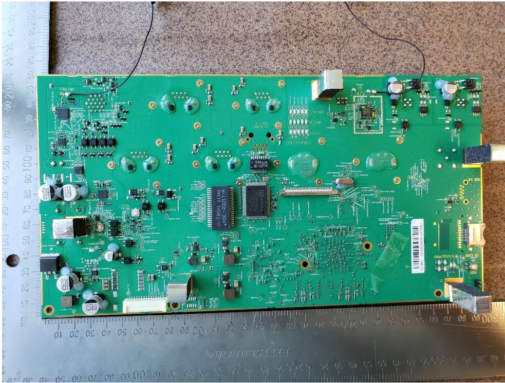
Main PCBA – contains RF transceivers
