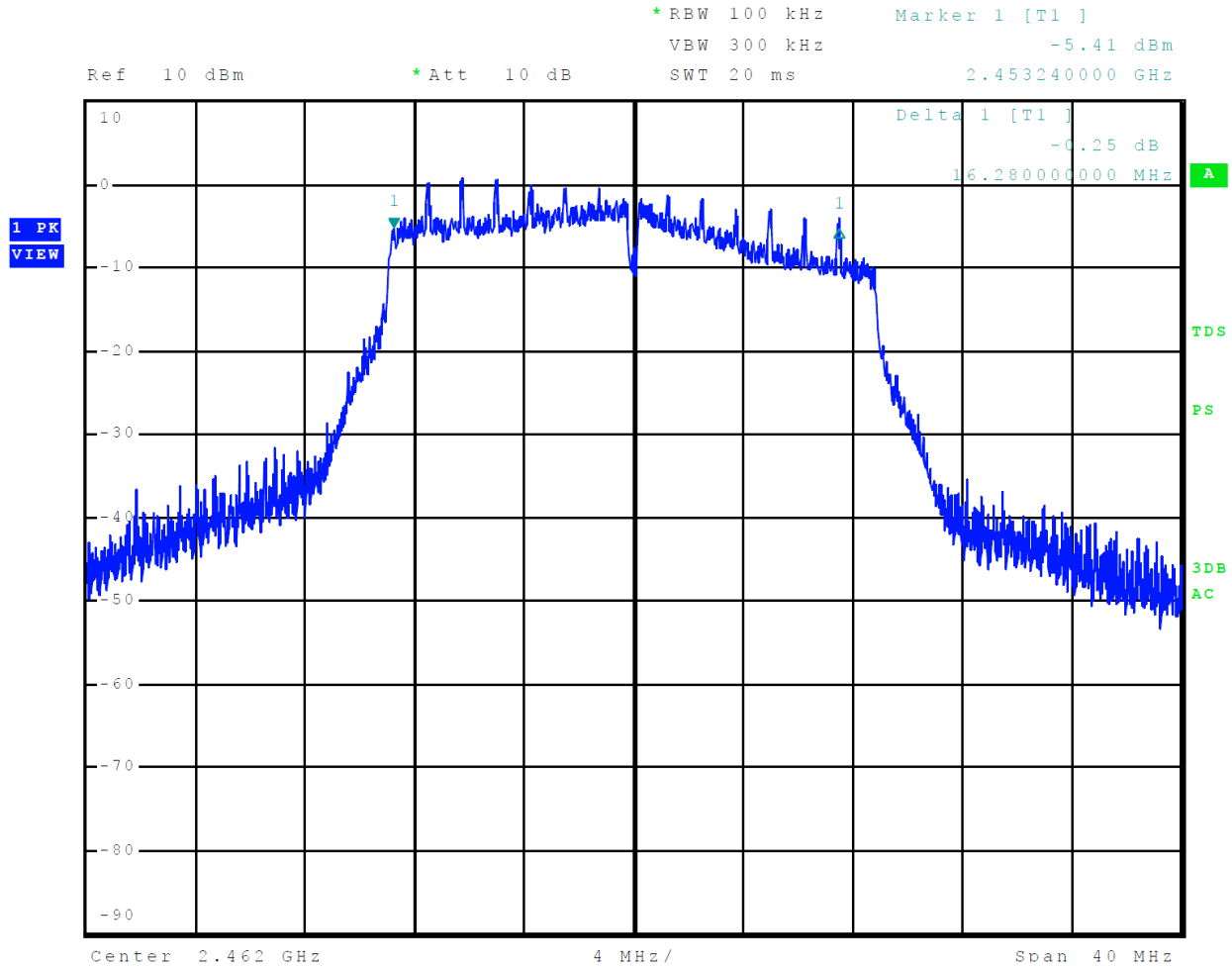
Figure 14 Plot of 6-dB Occupied Bandwidth Mode 5 802.11n
