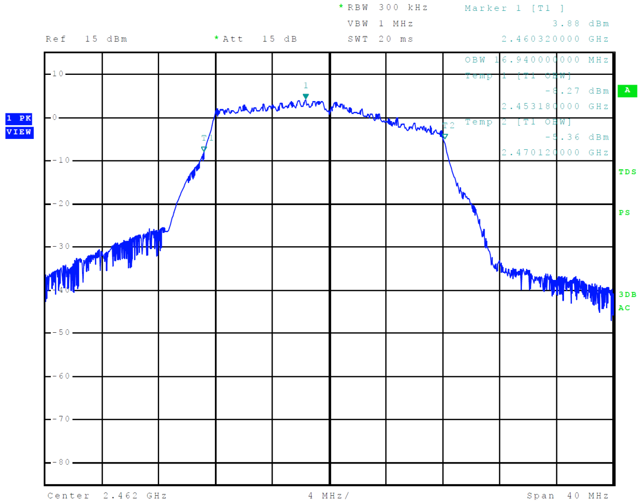
Figure 13 Plot of 99% Occupied Bandwidth Mode 4 802.11g
