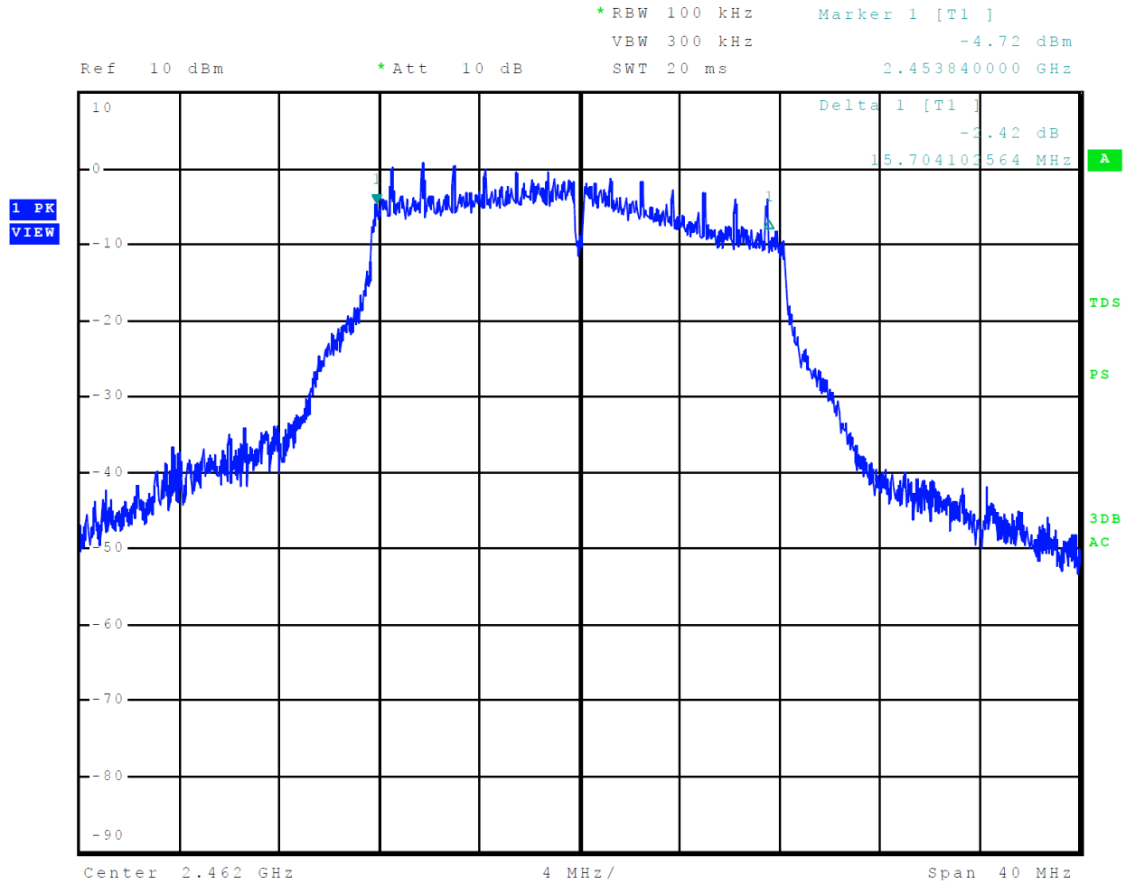
Figure 12 Plot of 6-dB Occupied Bandwidth Mode 4 802.11g
