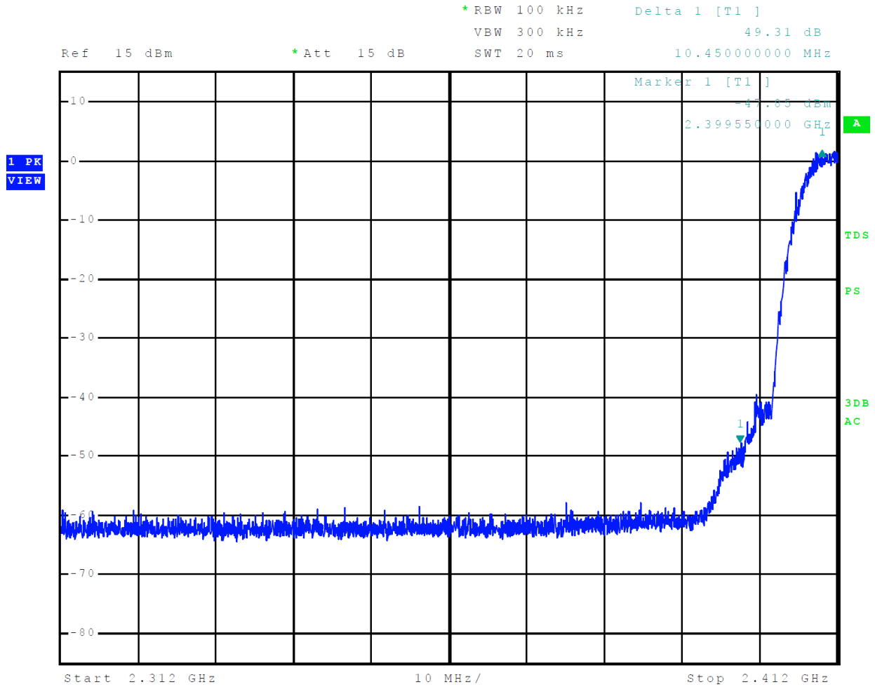
Figure 4 Plot of Transmitter Emissions Low Band Edge Mode 3 802.11b
