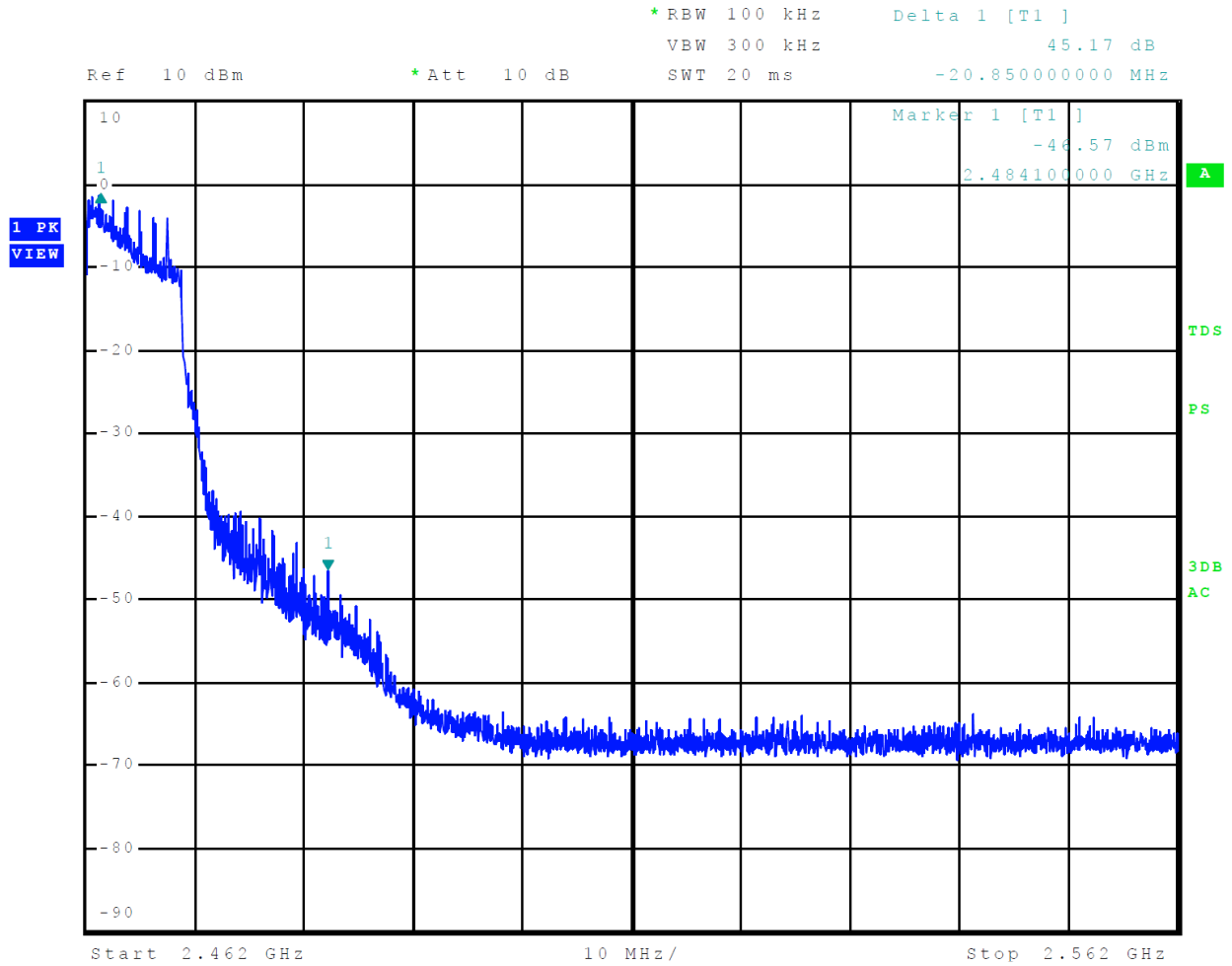
Figure 9 Plot of Transmitter Emissions High Band Edge Mode 5 802.11n
