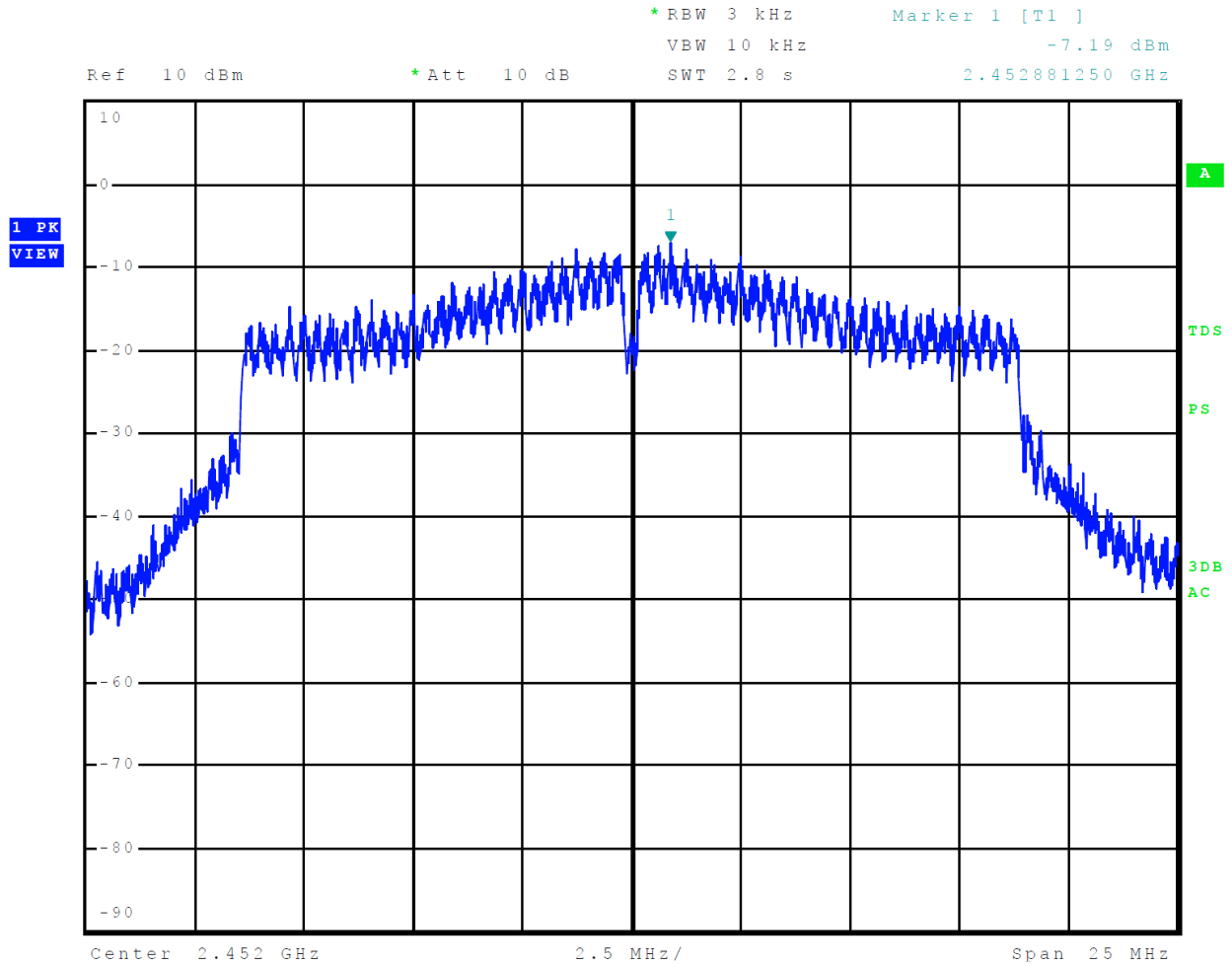
Figure 18 Plot of Transmitter Power Spectral Density Mode 5 802.11n
