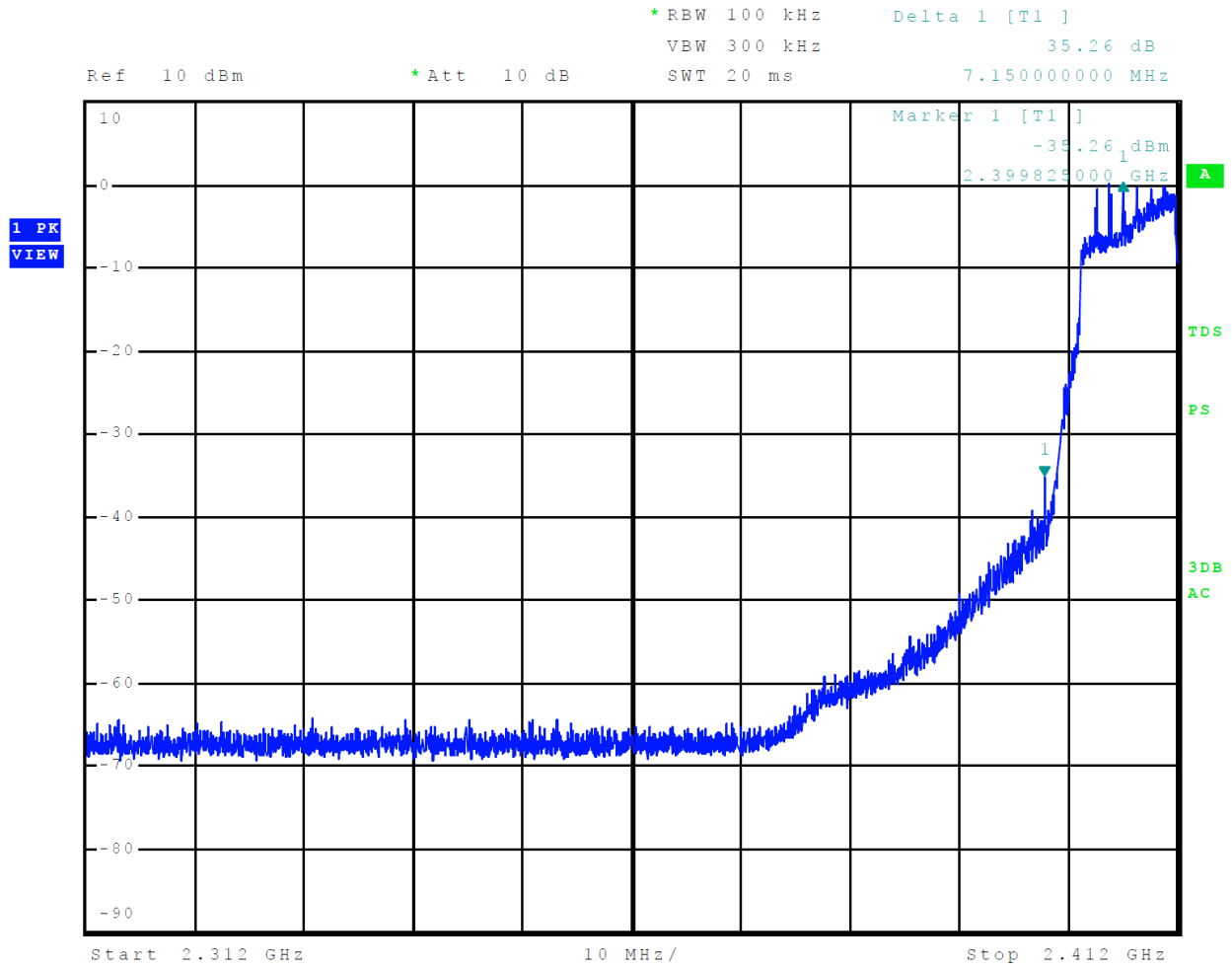
Figure 6 Plot of Transmitter Emissions Low Band Edge Mode 5 802.11n
