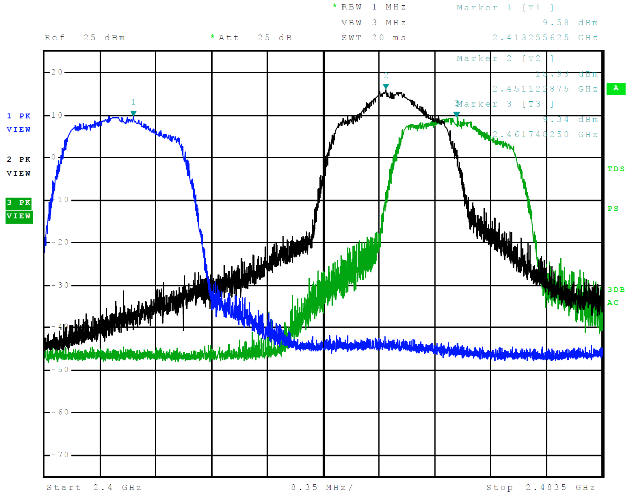
Figure 3 Plot of Transmitter Operation in 2412-2462 MHz Mode 5 802.11n
