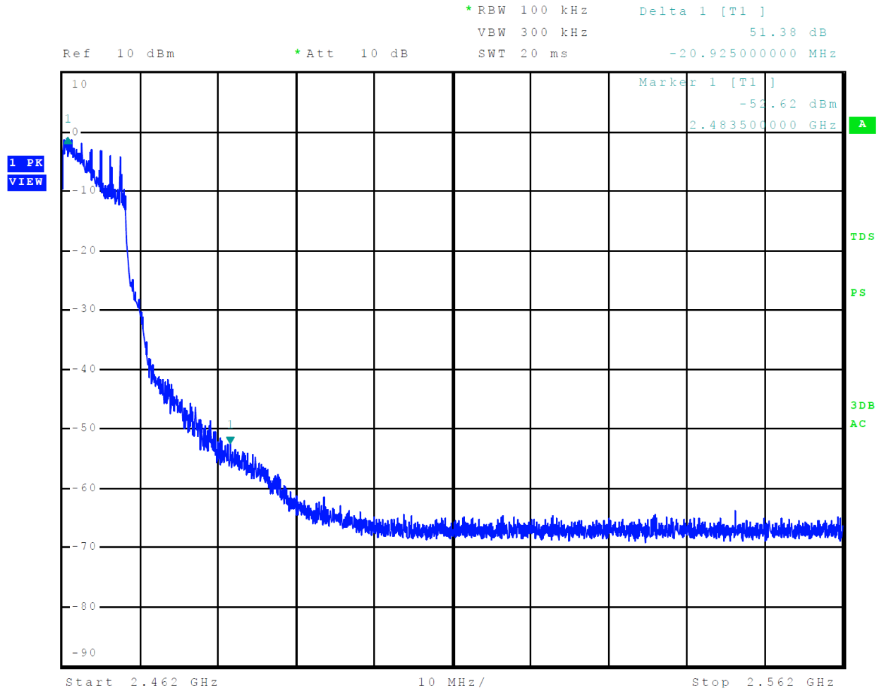
Figure 8 Plot of Transmitter Emissions High Band Edge Mode 4 802.11g
