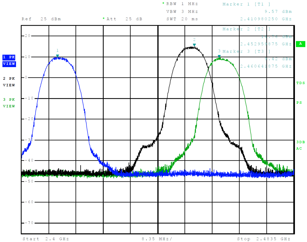
Figure 1 Plot of Transmitter Operation in 2412-2462 MHz Mode 3 802.11b
