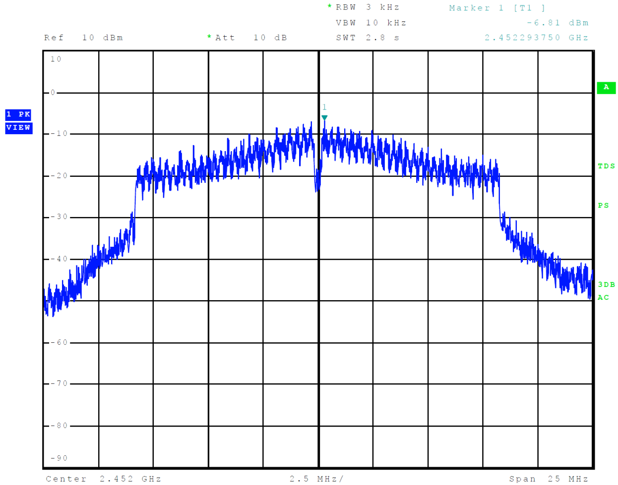
Figure 17 Plot of Transmitter Power Spectral Density Mode 4 802.11g
