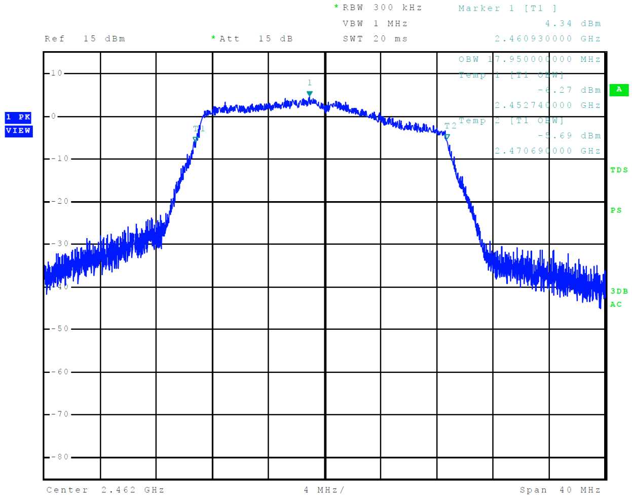
Figure 15 Plot of 99% Occupied Bandwidth Mode 5 802.11n
