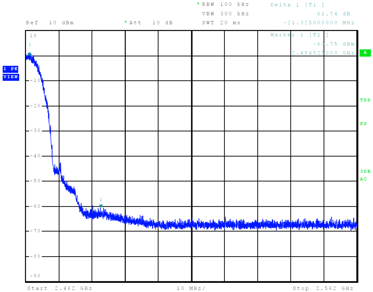
Figure 7 Plot of Transmitter Emissions High Band Edge Mode 3 802.11b
