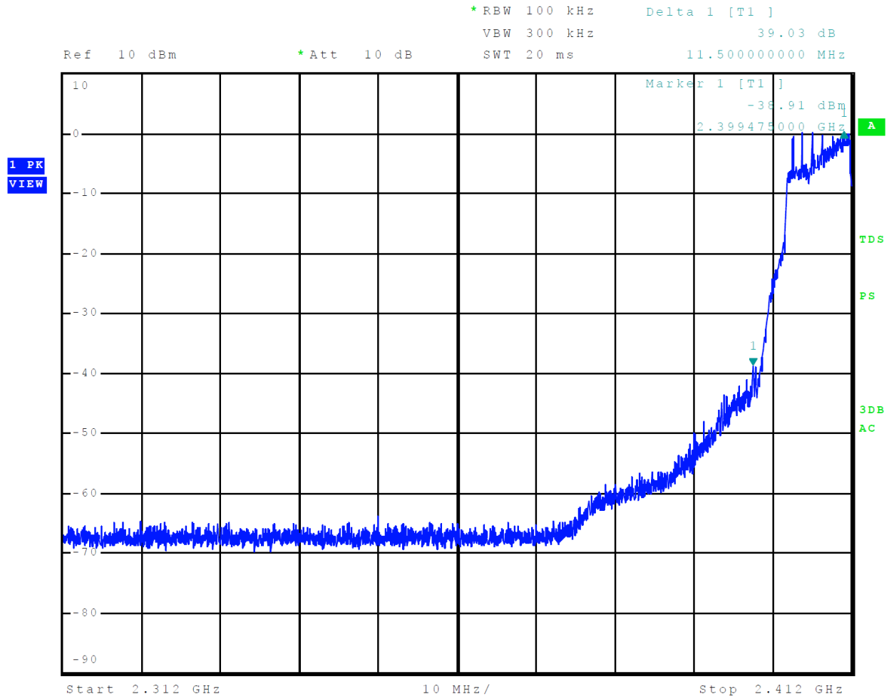
Figure 5 Plot of Transmitter Emissions Low Band Edge Mode 4 802.11g
