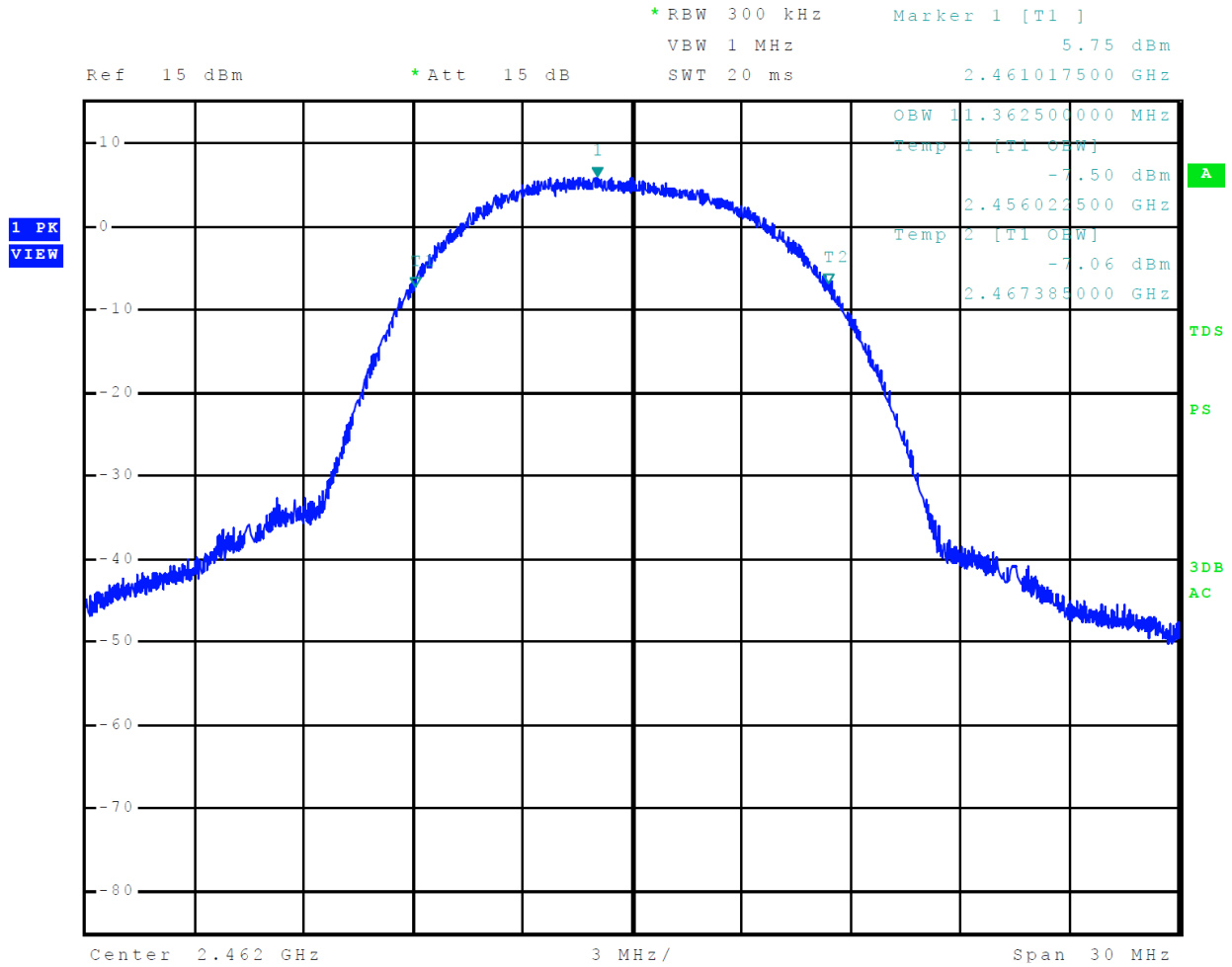
Figure 11 Plot of 99% Occupied Bandwidth Mode 3 802.11b
