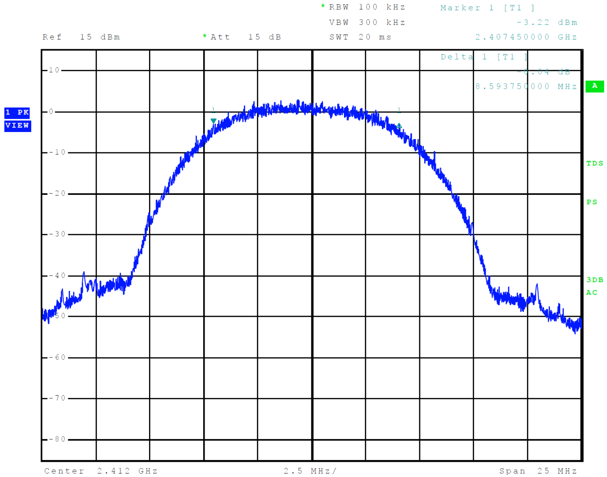
Figure 10 Plot of 6-dB Occupied Bandwidth Mode 3 802.11b
