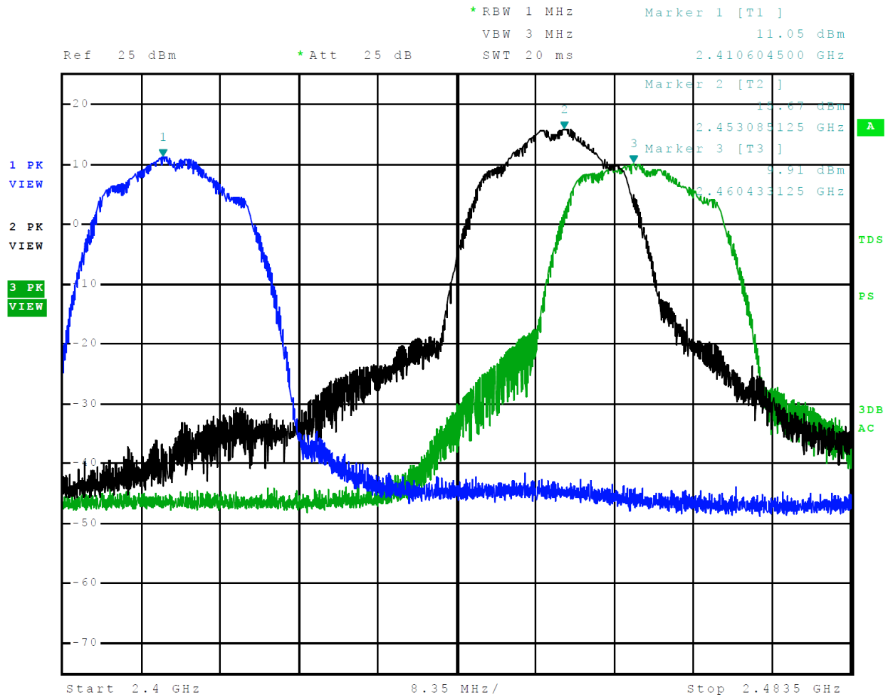
Figure 2 Plot of Transmitter Operation in 2412-2462 MHz Mode 4 802.11g
