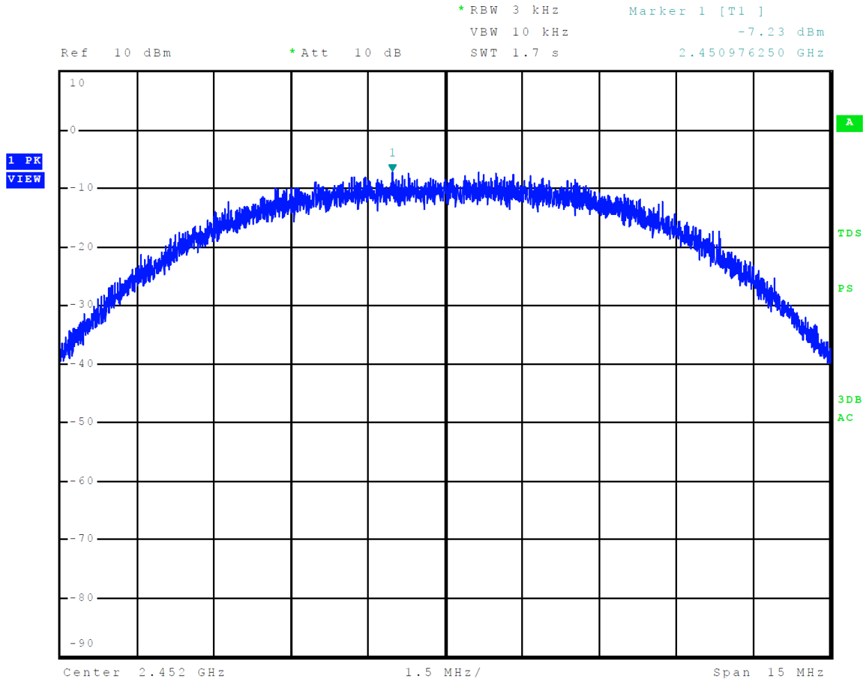
Figure 16 Plot of Transmitter Power Spectral Density Mode 3 802.11b
