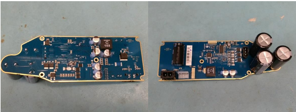
Motor Control Board
