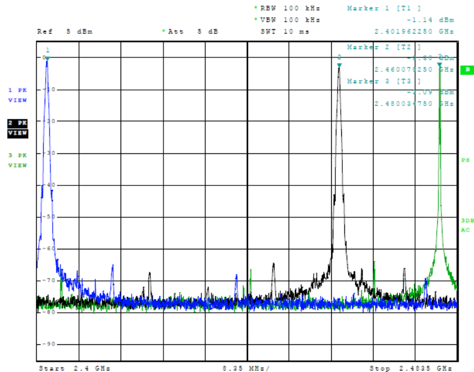
Figure 9 Plot of Transmitter Emissions (In 2402-2480 MHz Band) (Mode 2)
