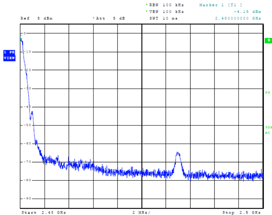
Figure 8 Plot of Low Band Edge (High Band Edge) (Mode 1)
