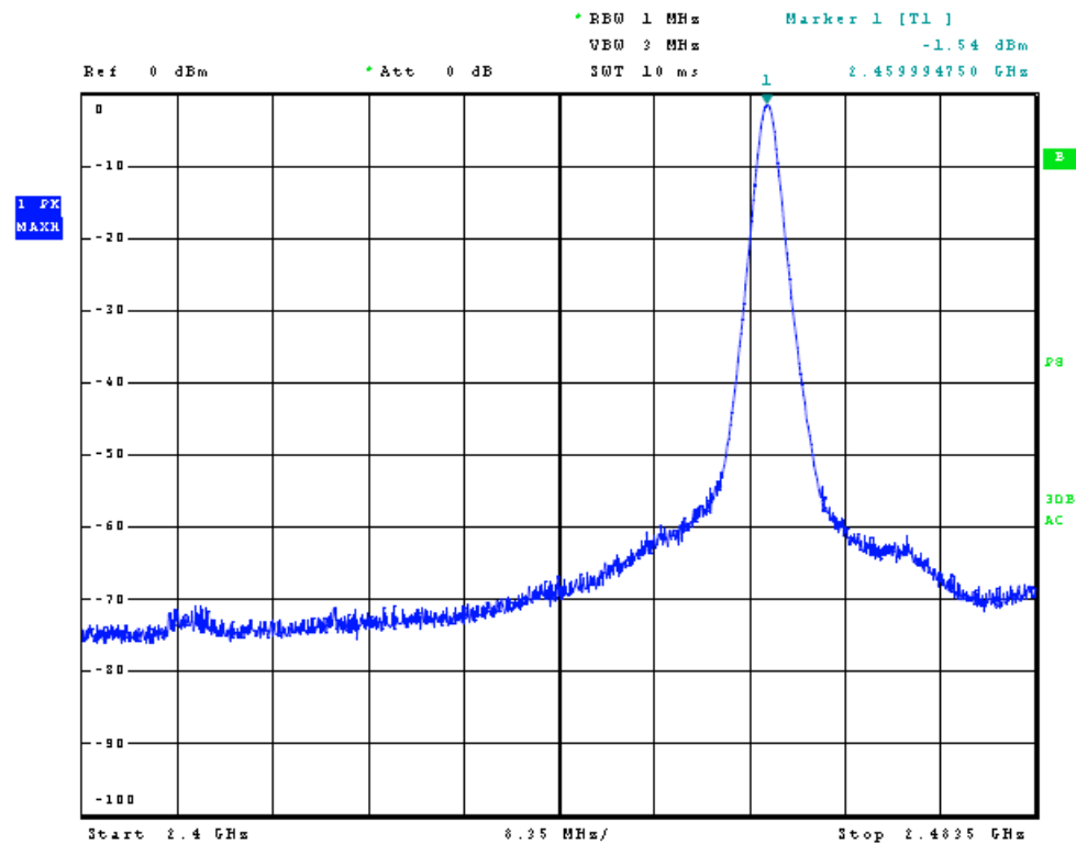
Figure 9 Plot of Transmitter 1 Emissions (2402-2480 MHz, ANT)
