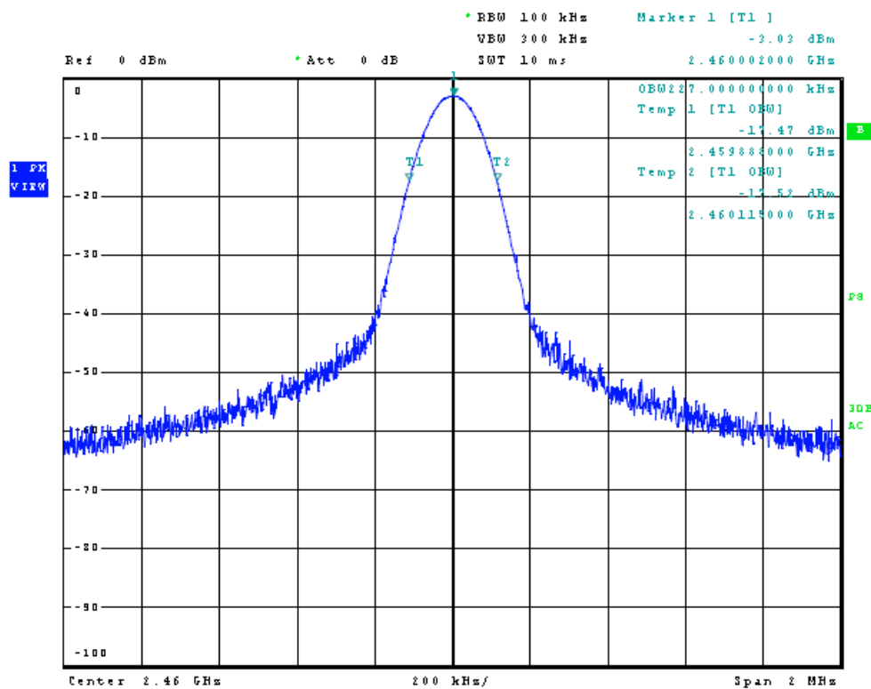
Figure 10 Plot of Transmitter 1 Emissions (99% Occupied Bandwidth, ANT)
