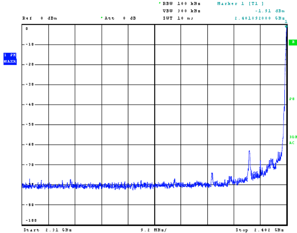
Figure 7 Plot of Transmitter 1 Emissions (Low Band Edge, BT)
