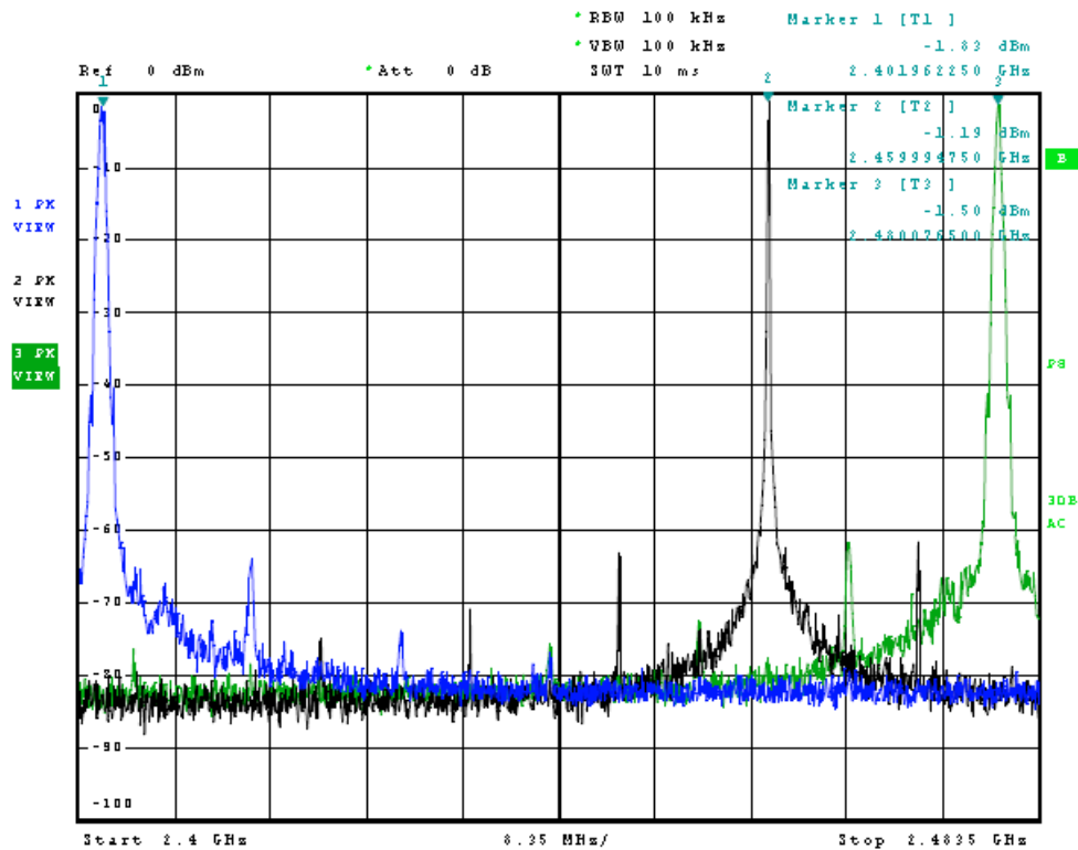
Figure 5 Plot of Transmitter 1 Emissions (2402-2480 MHz, BT)
