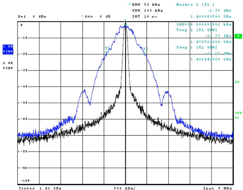
Figure 6 Plot of Transmitter 1 Emissions (99% Occupied Bandwidth, BT)
