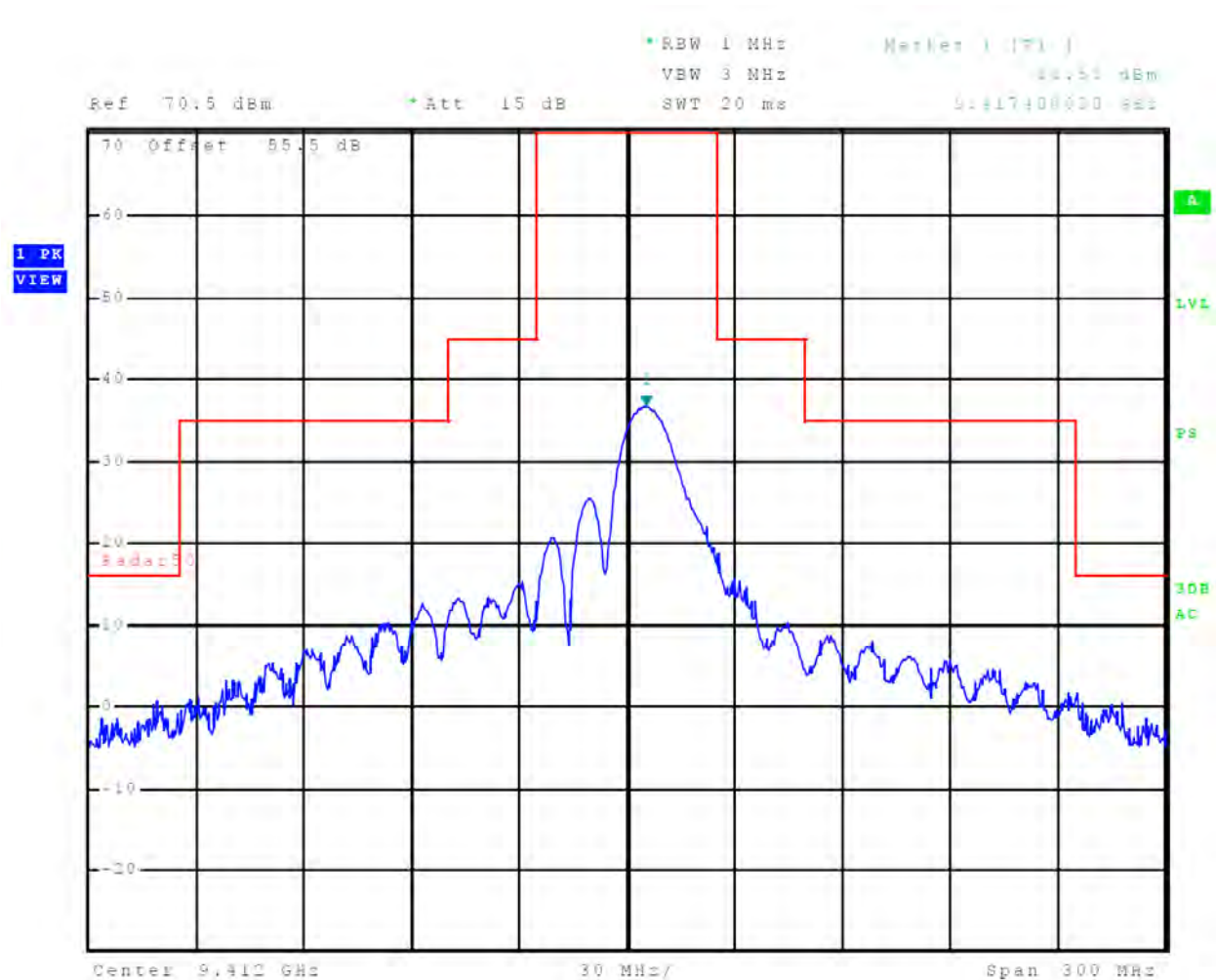
Figure 42 Emissions Mask, 1/16 nm
