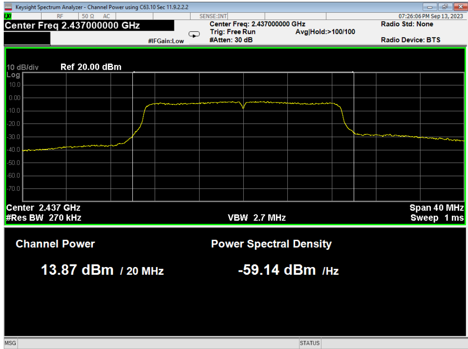
Figure 3 – Conducted Average Power Measurement, 802.11n
