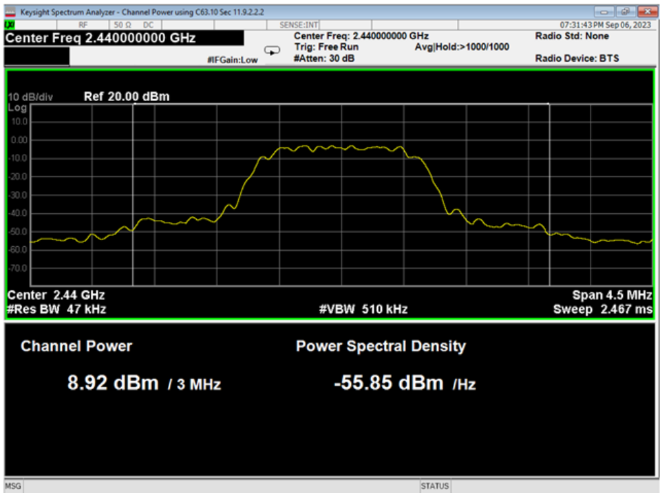
02 Average Power, Mid Channel, 2EDR
