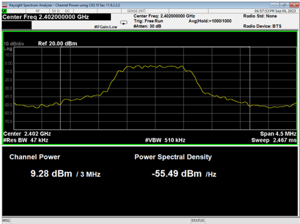
01 Average Power, Low Channel, 2EDR
