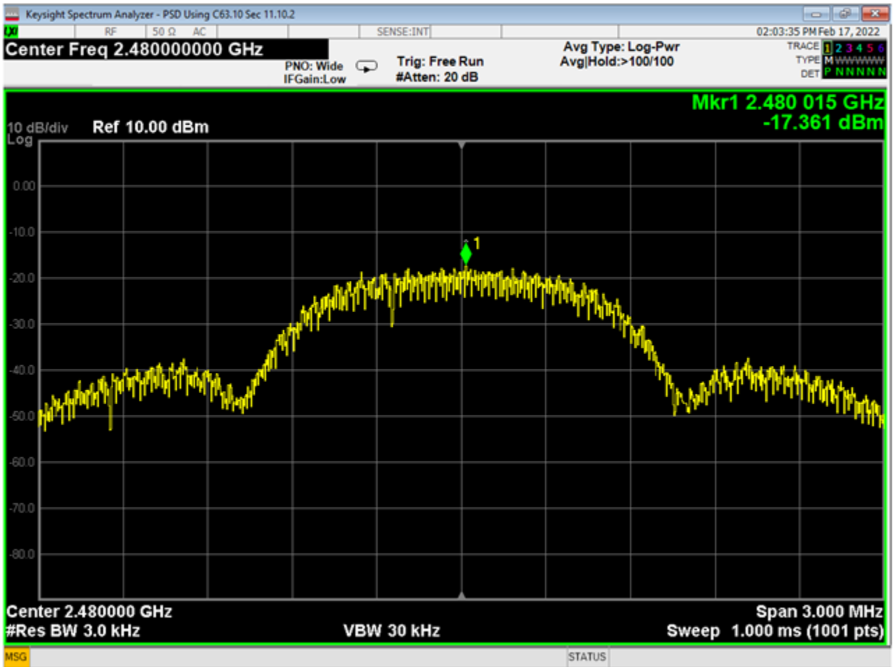
09 PSD, High Channel ANT GFSK
