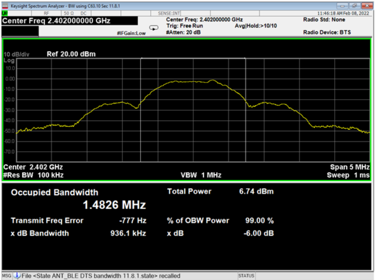
04 Bandwidth, Low Channel ANT GFSK
