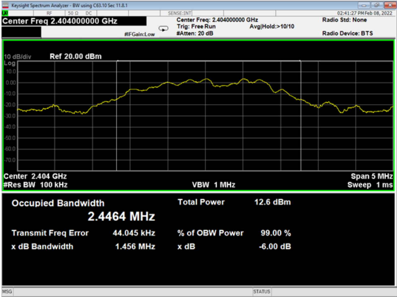
04 Bandwidth, Low Channel, GMSK 2MB
