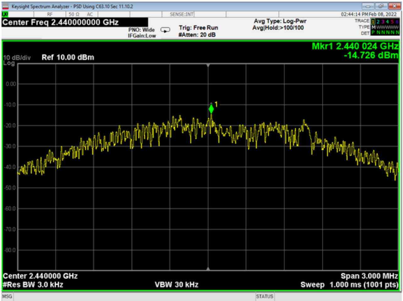
08 PSD, Mid Channel, GMSK 2MB
