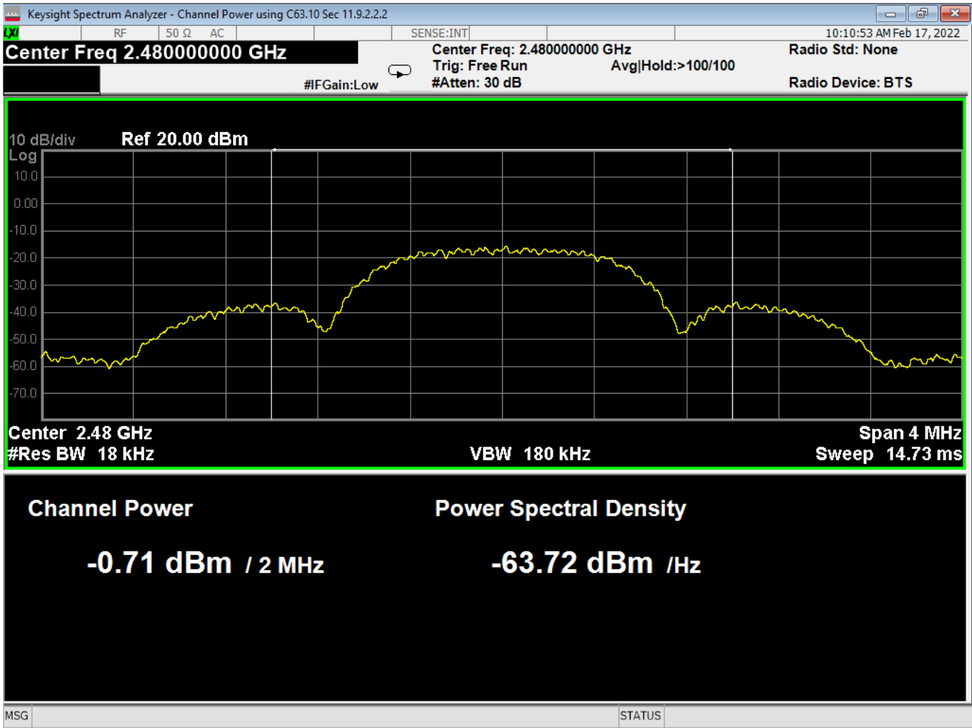
03 Average Output Power, High Channel ANT GFSK
