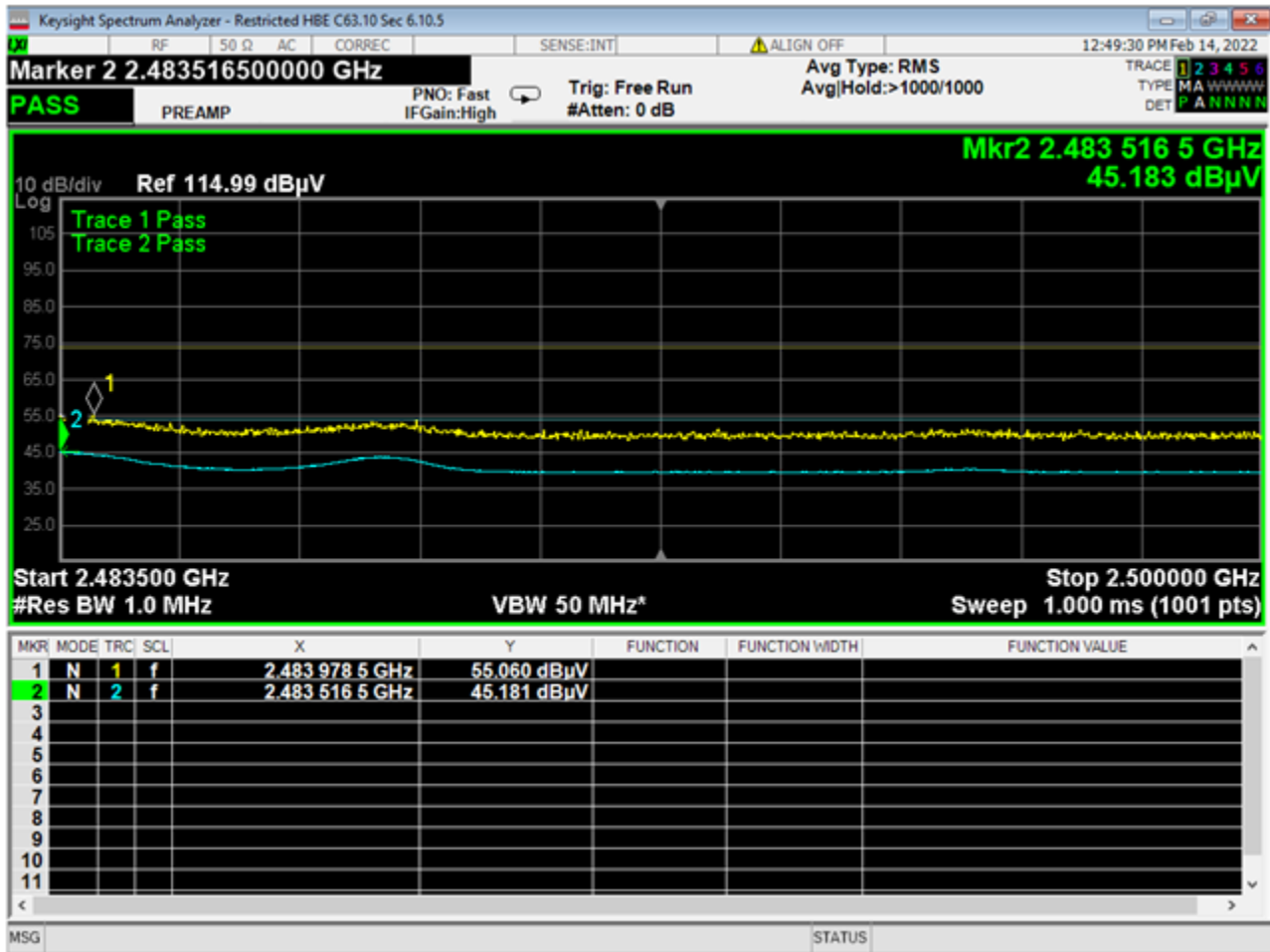
13 HBE, Restricted GMSK 1MB
