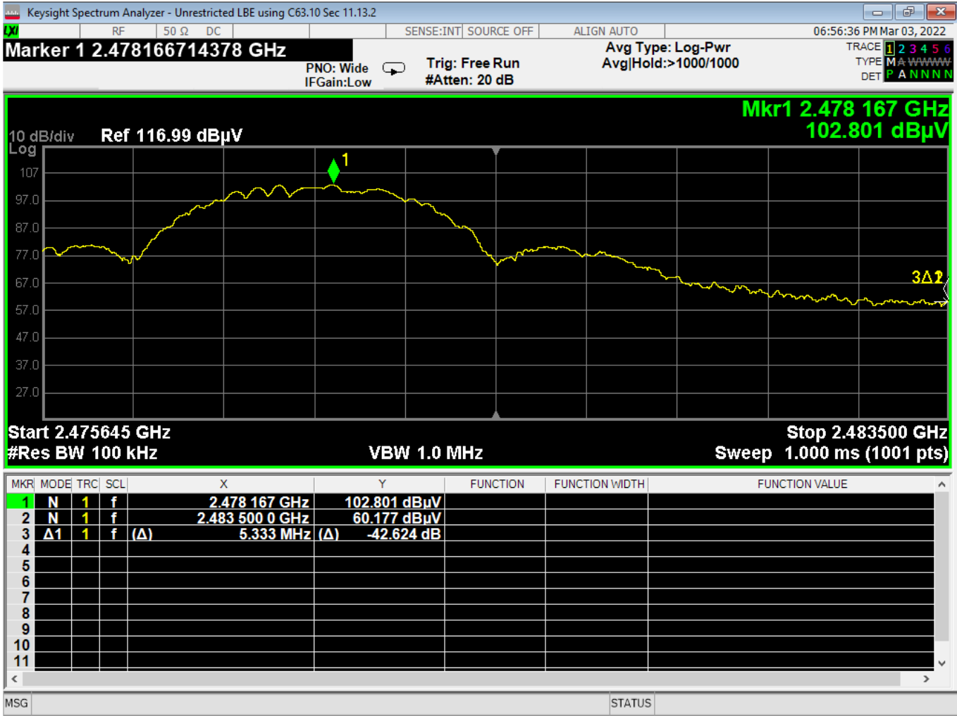
11 Higher Bandedge, Unrestricted, GMSK 2MB
