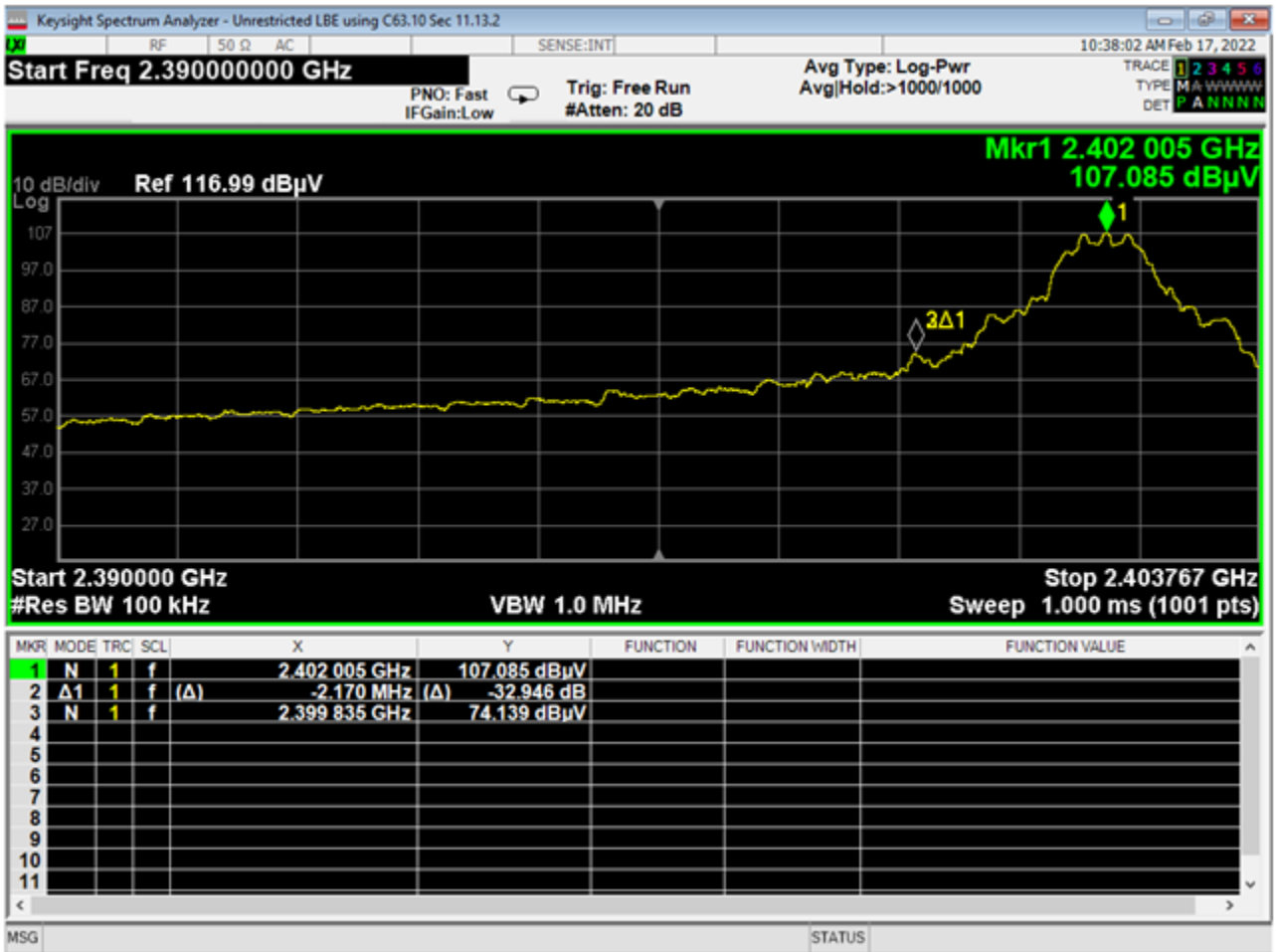
10 LBE, unrestricted GMSK 1MB
