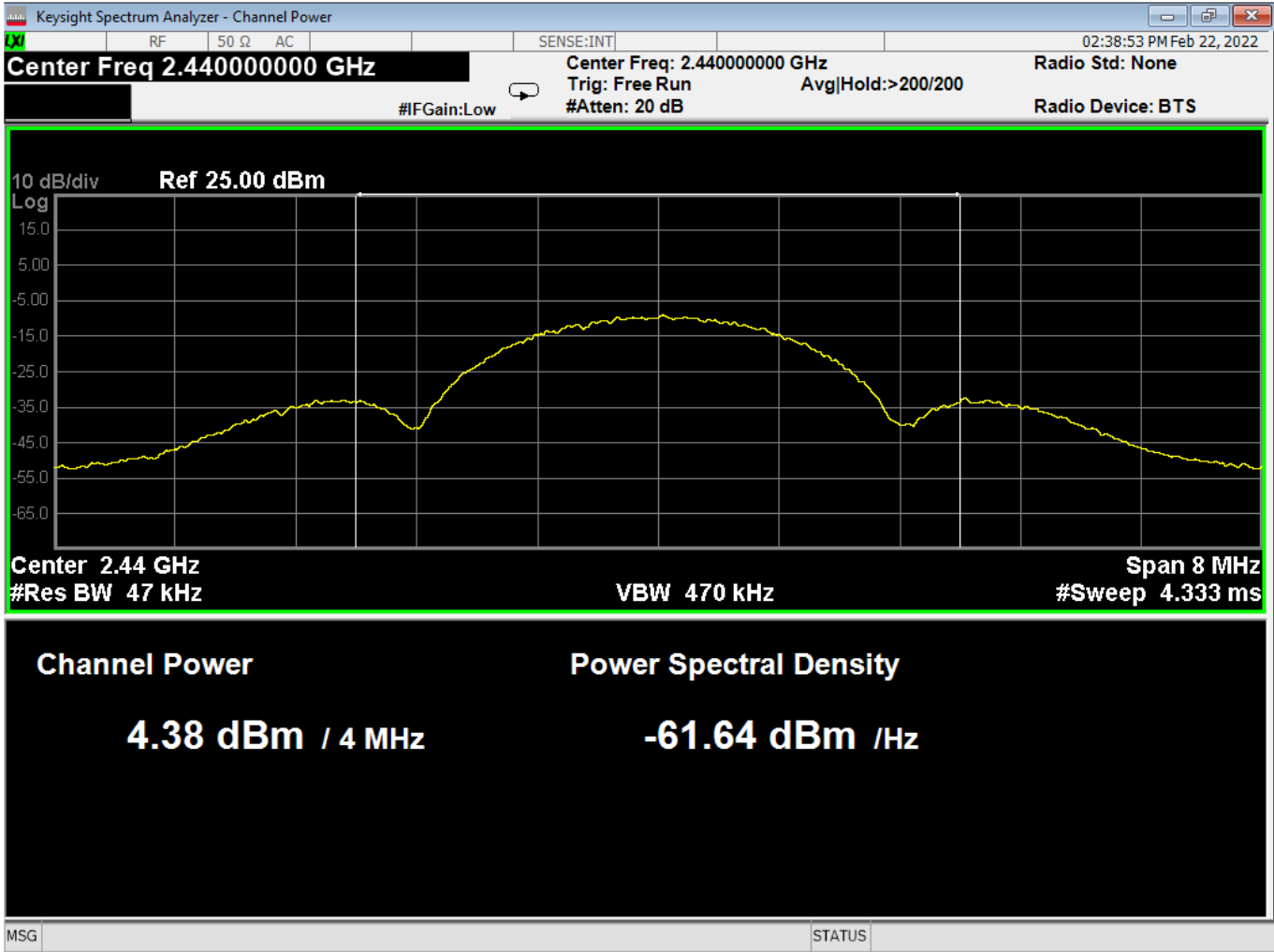
02 Average Power, Mid Channel, GMSK 2MB
