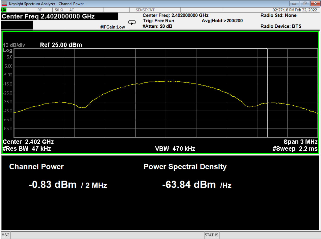
01 Average Output Power, Low Channel GMSK 1MB
