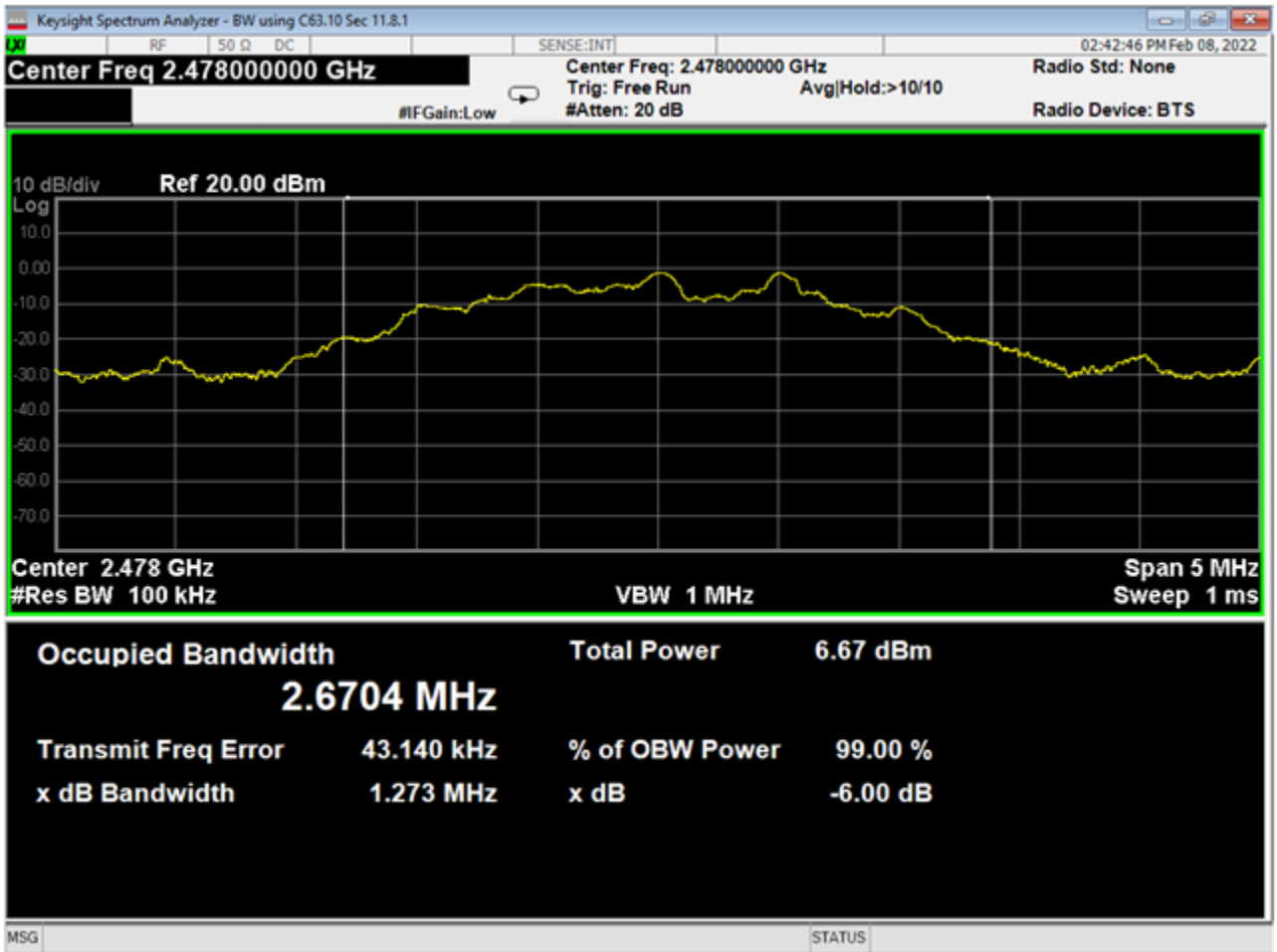
06 Bandwidth, High Channel, GMSK 2MB
