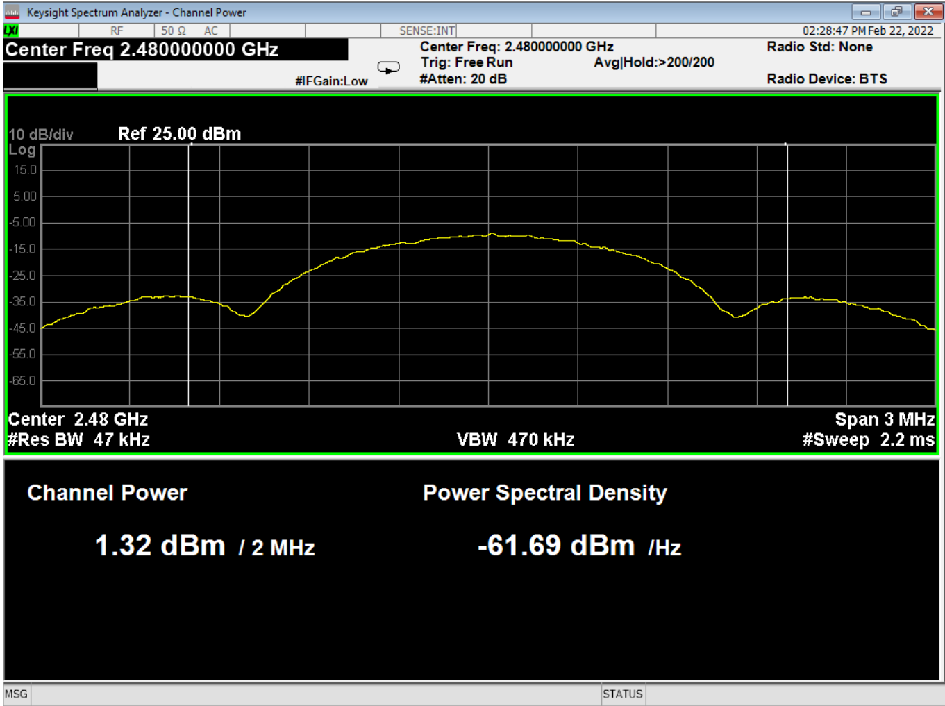
03 Average Output Power, High Channel GMSK 1MB
