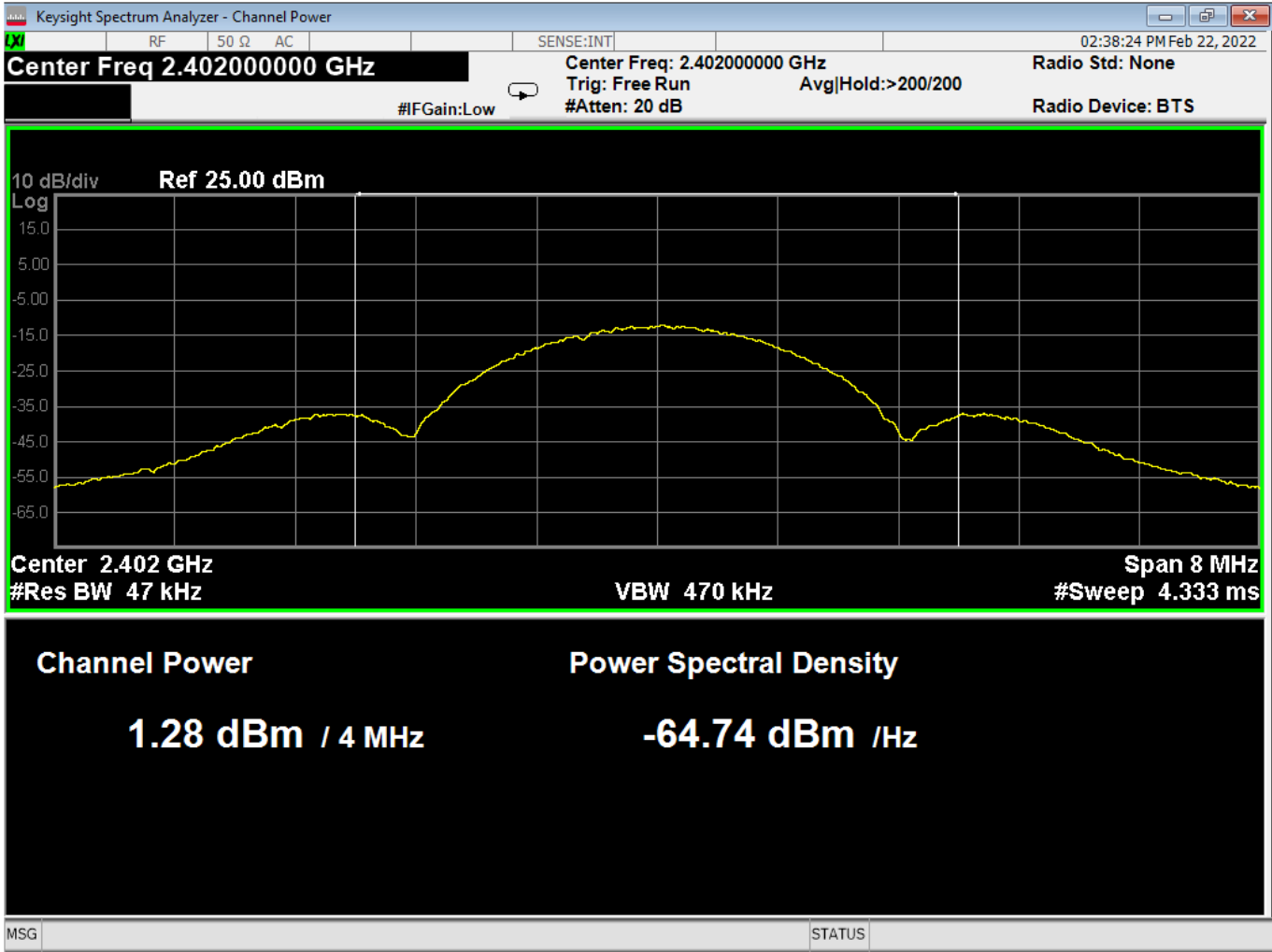
01 Average Power, Low Channel, GMSK 2MB
