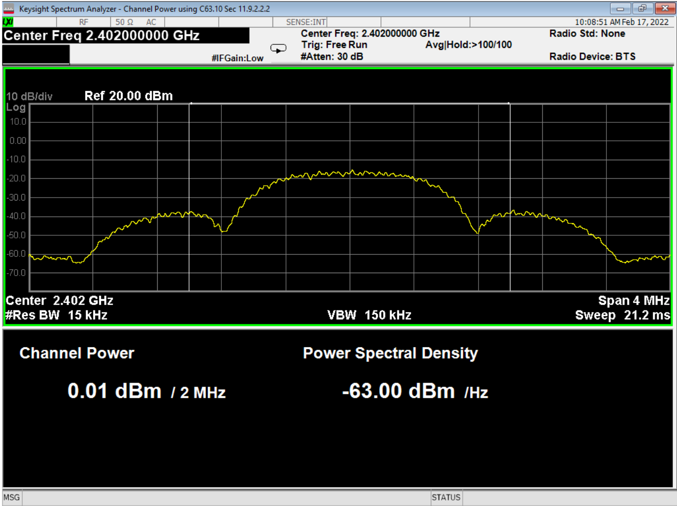
01 Average Output Power, Low Channel ANT GFSK
