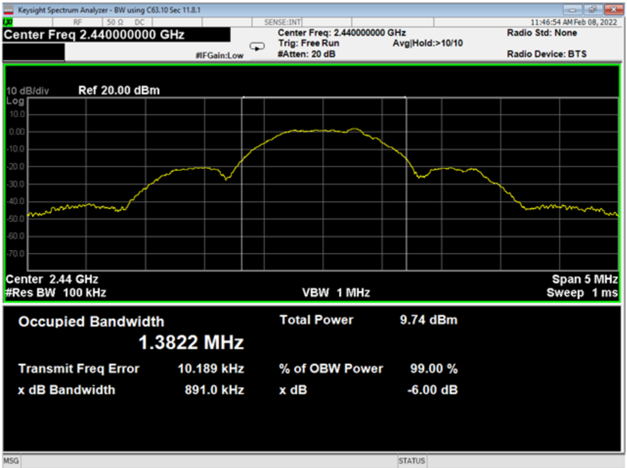
05 Bandwidth, Mid Channel ANT GFSK
