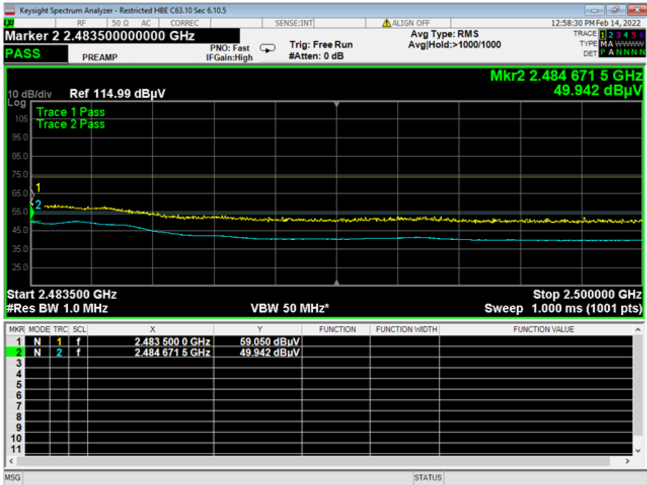
13 Higher Bandedge, Restricted, GMSK 2MB
