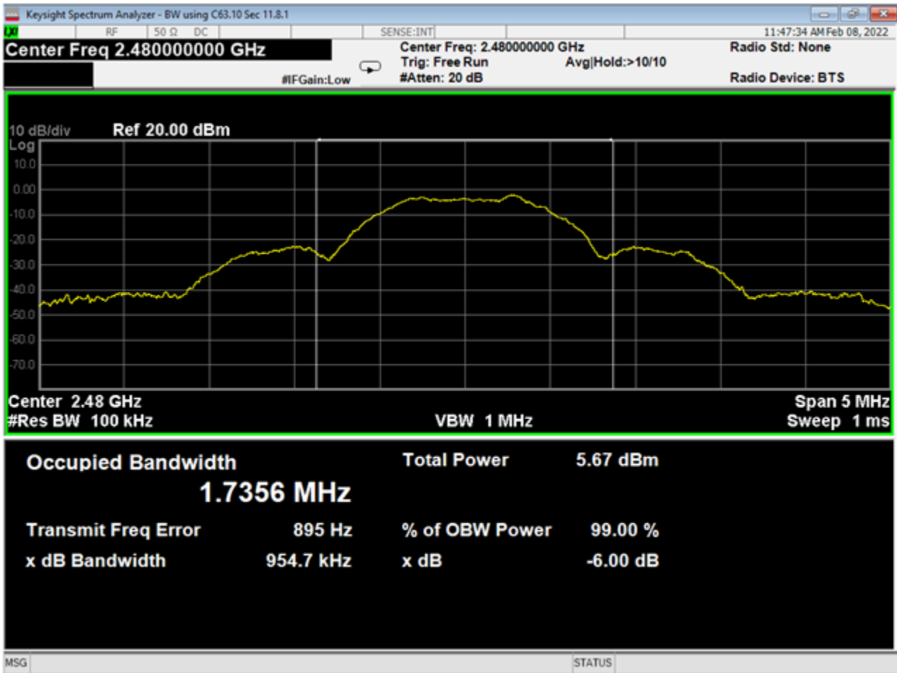
06 Bandwidth, High Channel ANT GFSK
