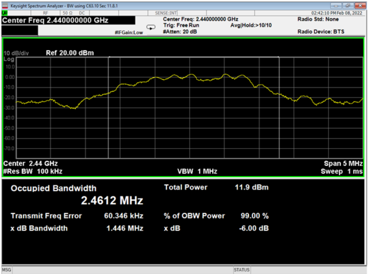
05 Bandwidth, Mid Channel, GMSK 2MB
