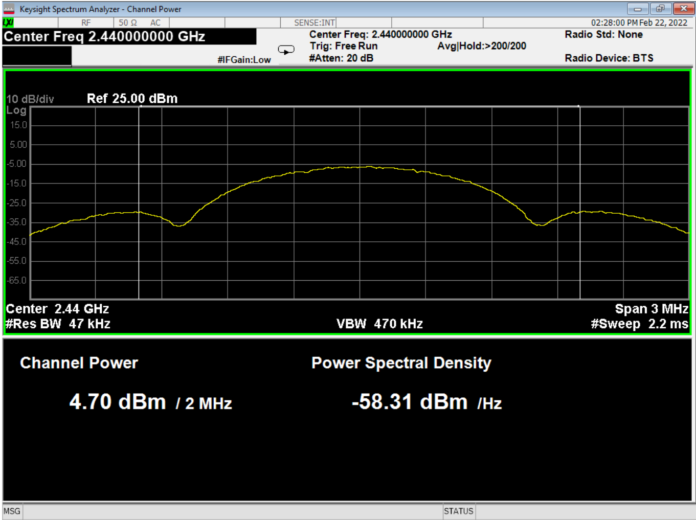
02 Average Output Power, Mid Channel GMSK 1MB
