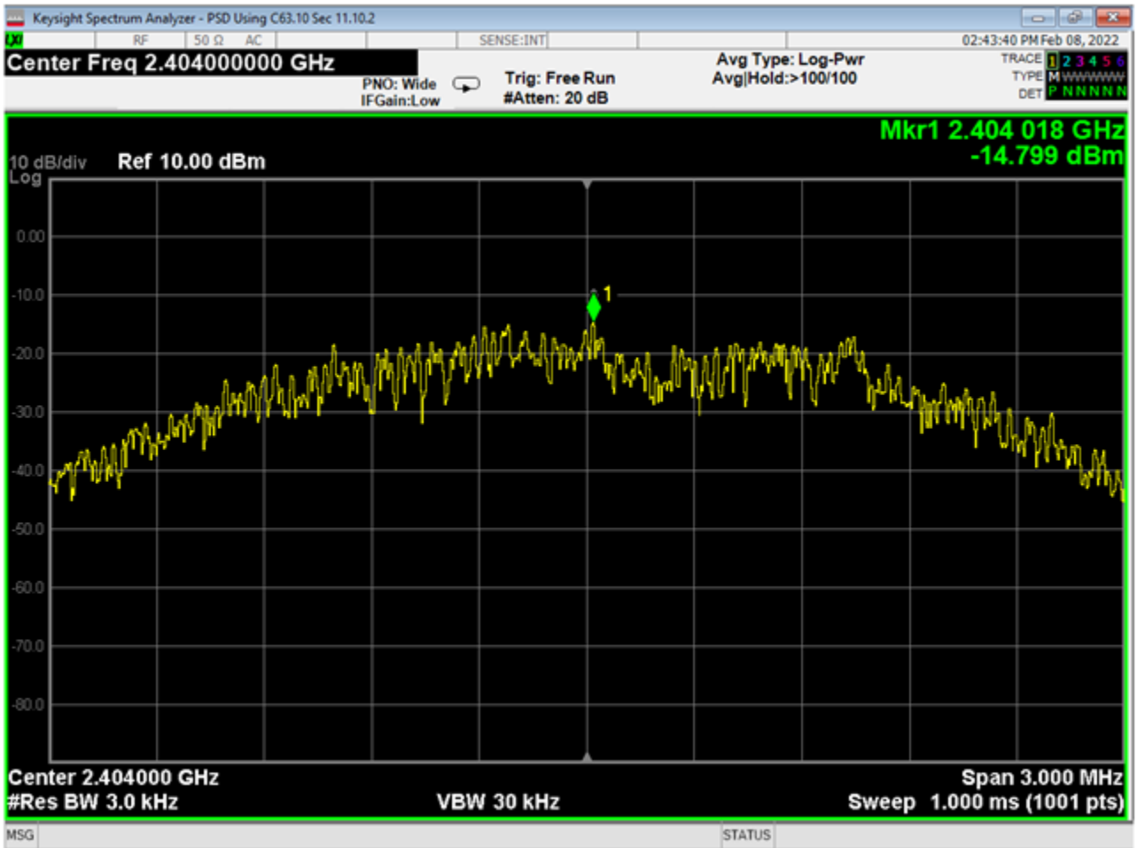
07 PSD, Low Channel, GMSK 2MB
