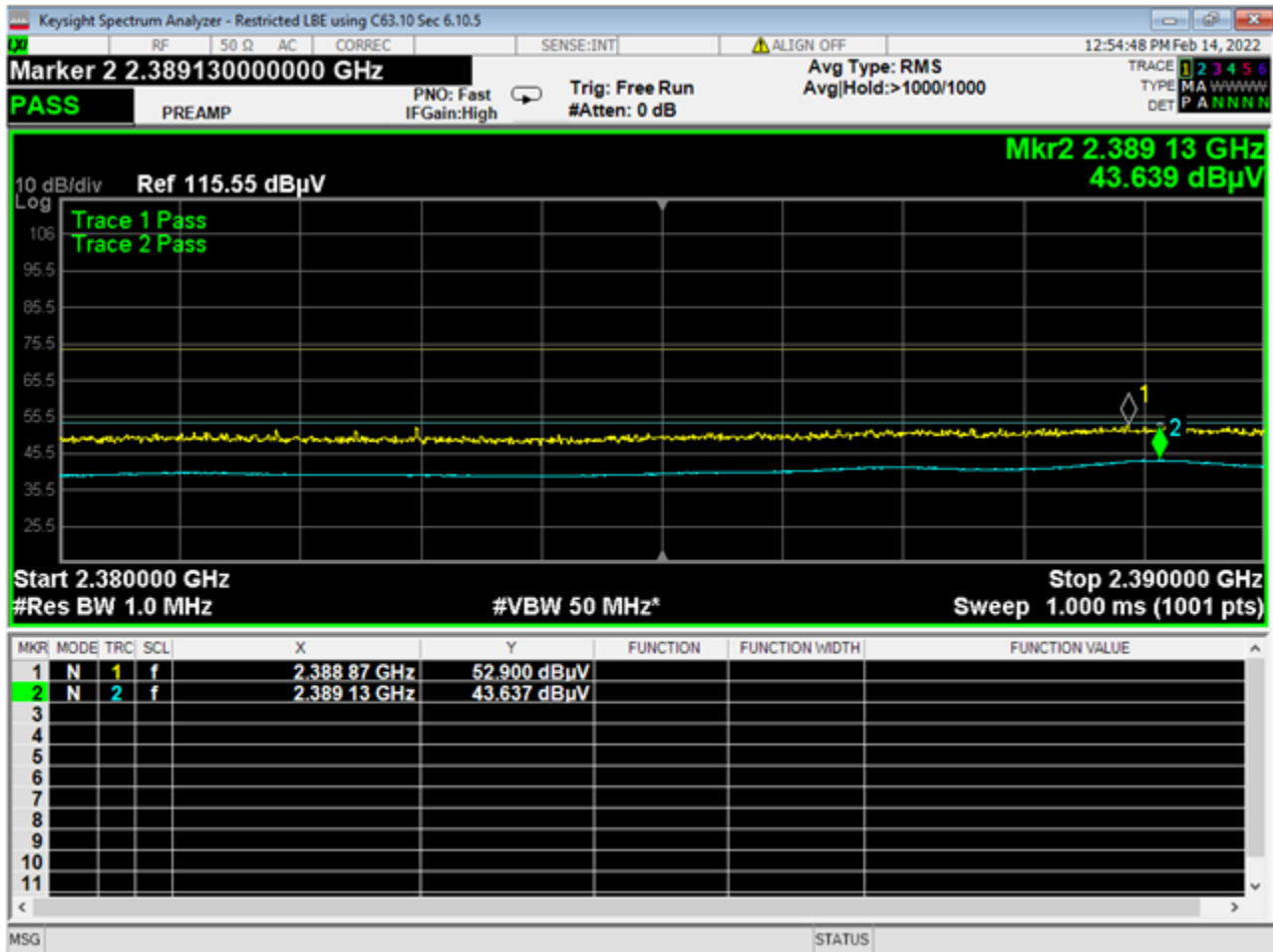
12 Lower Bandedge, Restricted, GMSK 2MB
