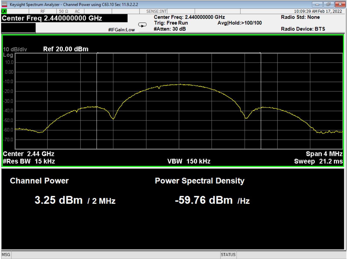
02 Average Output Power, Mid Channel ANT GFSK
