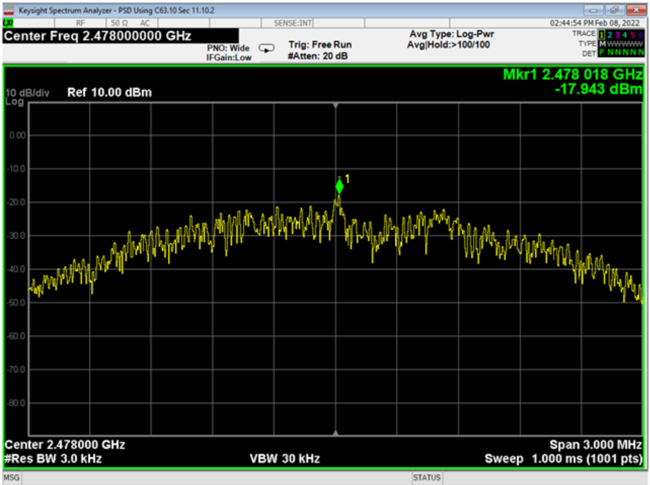
09 PSD, High Channel, GMSK 2MB
