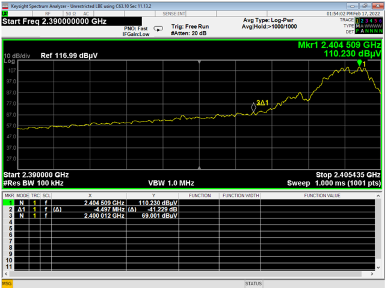
10 Lower Bandedge, Unrestricted, GMSK 2MB
