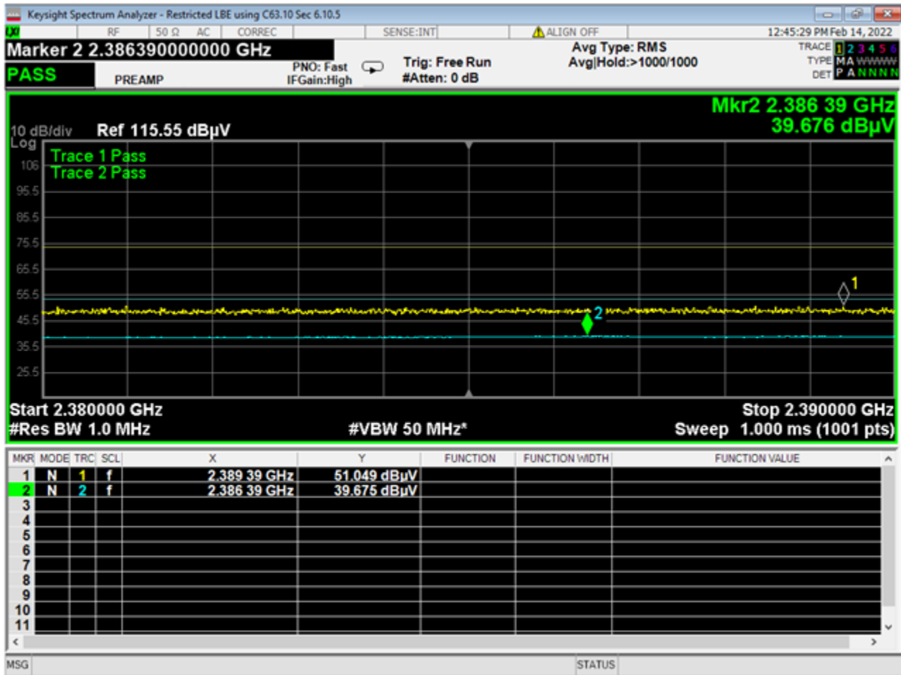
12 LBE, Restricted GMSK 1MB
