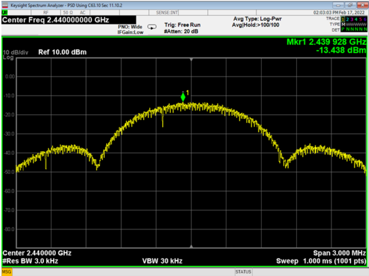
08 PSD, Mid Channel ANT GFSK
