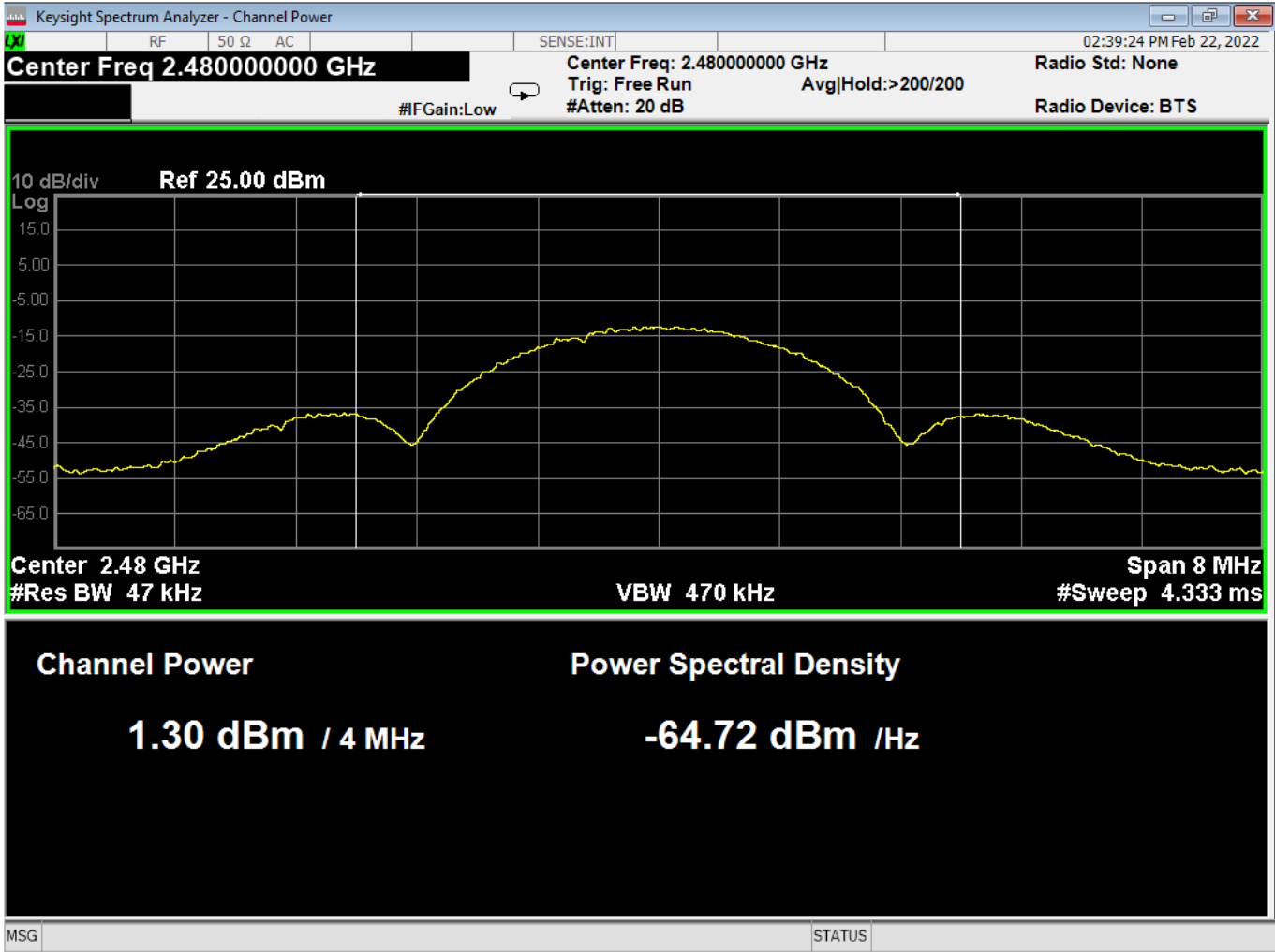
03 Average Power, High Channel, GMSK 2MB
