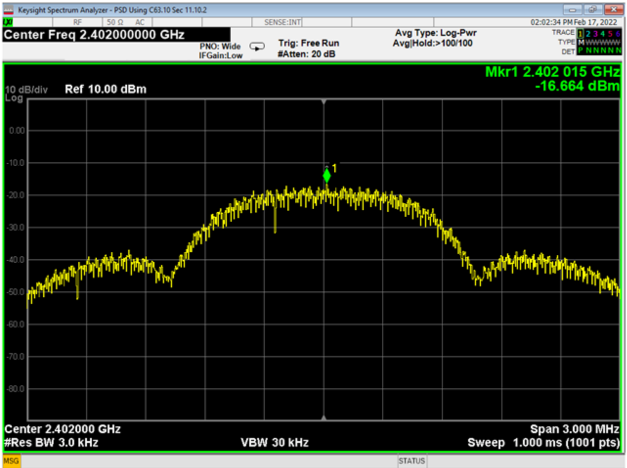
07 PSD, Low Channel ANT GFSK
