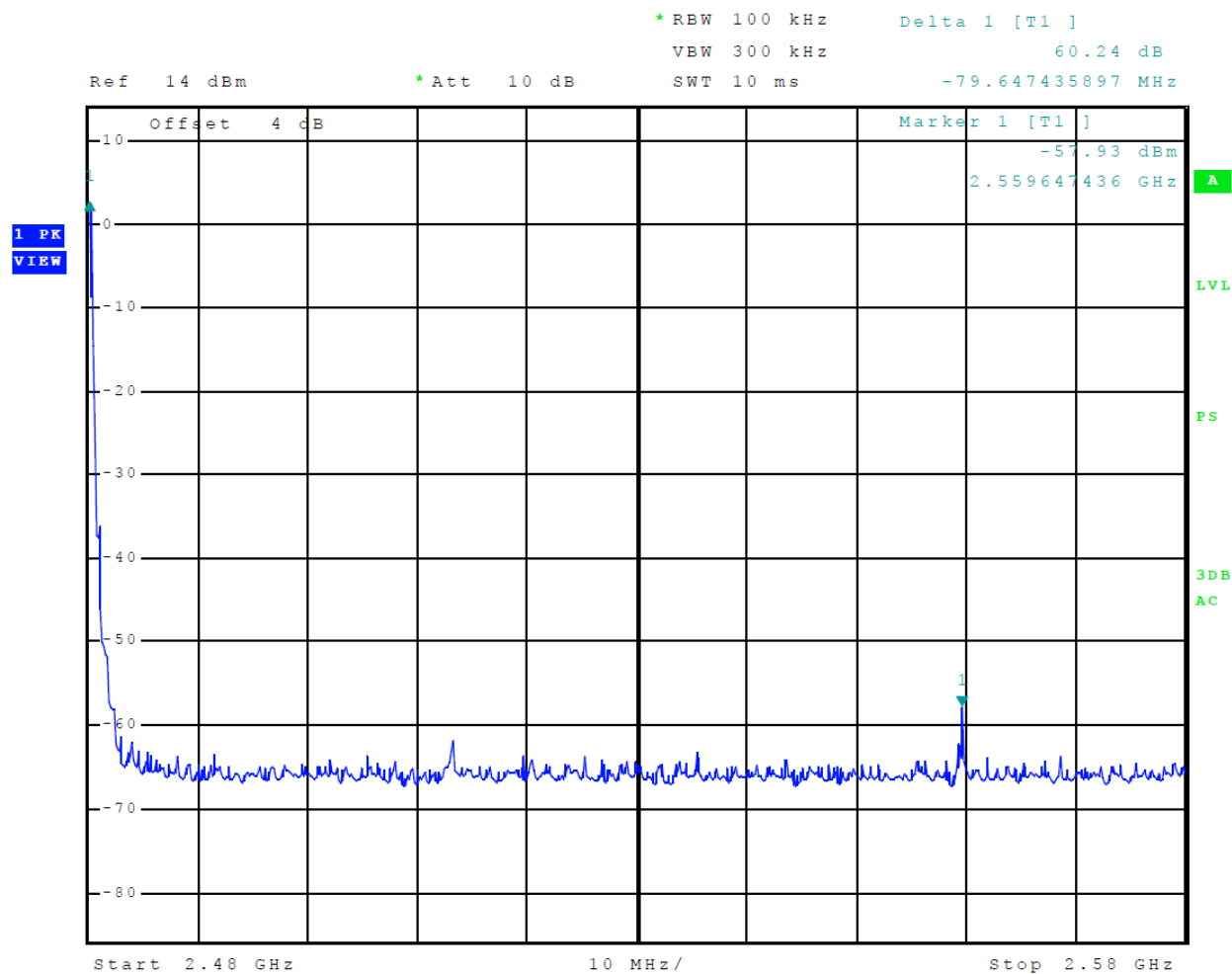
Figure 9 Plot of Transmitter Emissions High Band Edge Mode 1 BT BR
