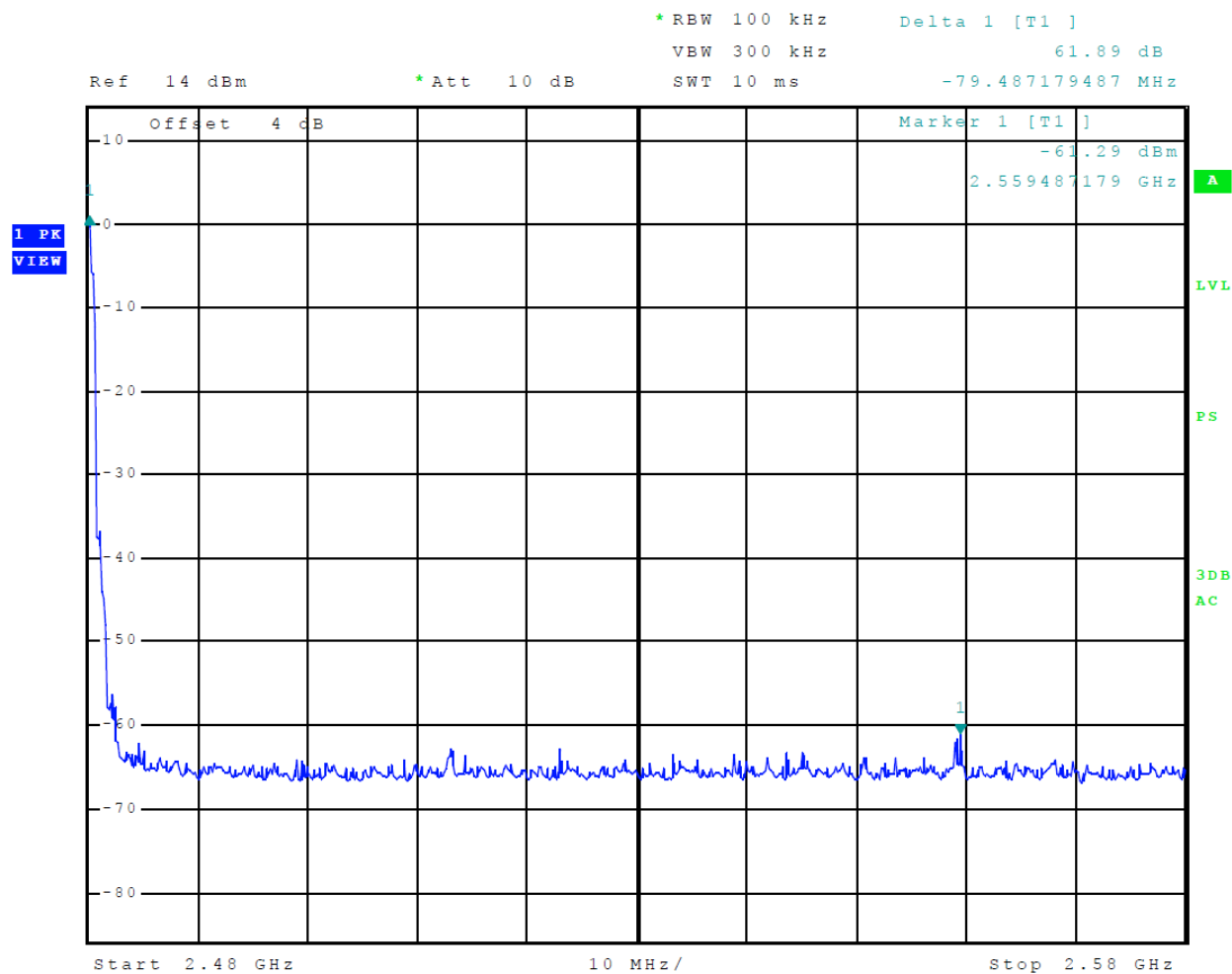
Figure 10 Plot of Transmitter Emissions High Band Edge Mode 2 BT 2EDR
