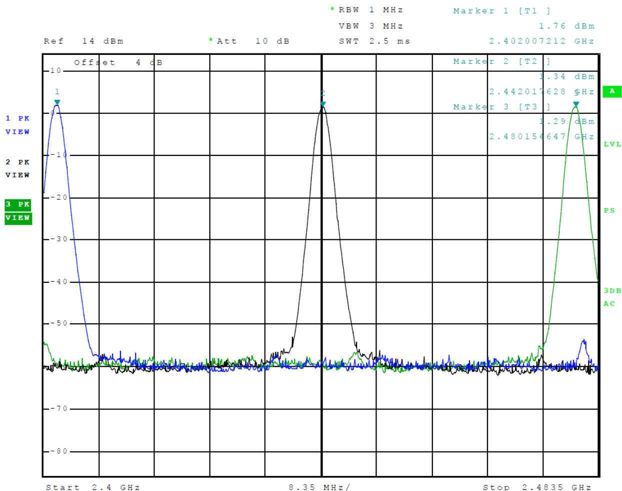
Figure 4 Plot of Transmitter Emissions Operation in 2402-2480 MHz Mode 2 BT 2EDR
