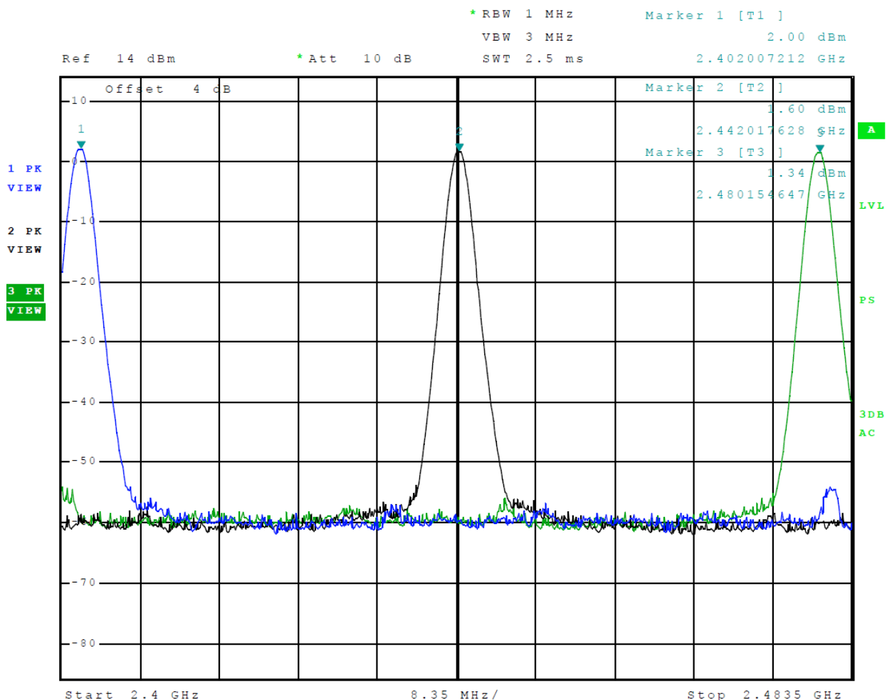
Figure 5 Plot of Transmitter Emissions Operation in 2402-2480 MHz Mode 3 BT 3EDR
