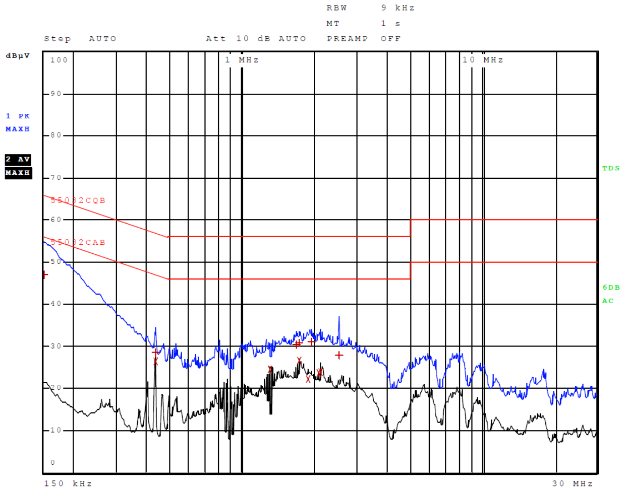
Figure 2 AC Line Conducted emissions of EUT line 2 (EUT – Computer)
