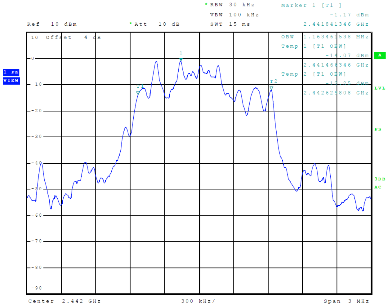
Figure 13 Plot of Transmitter Emissions 99% Occupied Bandwidth Mode 1 BT 2EDR
