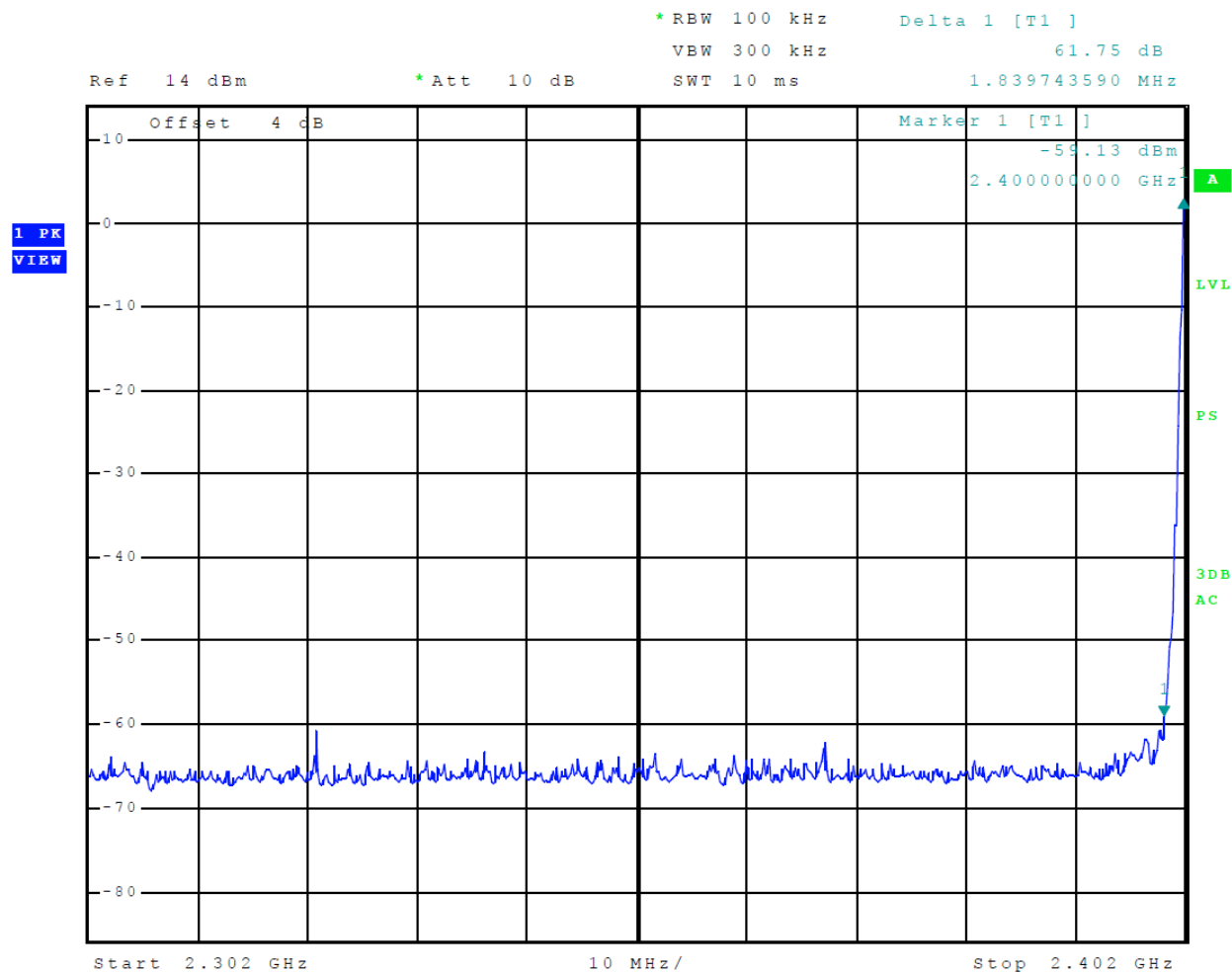
Figure 6 Plot of Transmitter Emissions Low Band Edge Mode 1 BT BR
