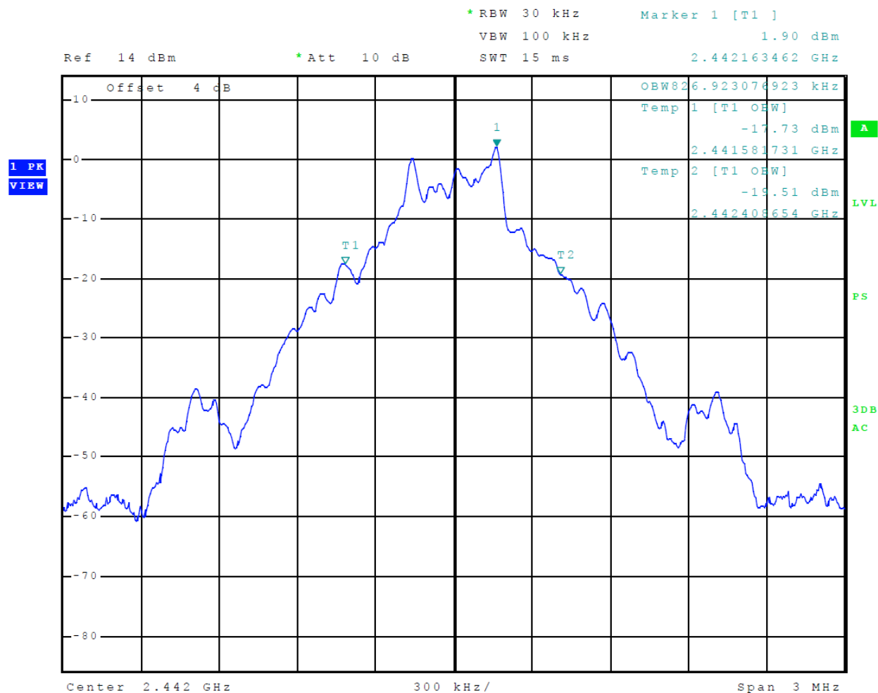
Figure 12 Plot of Transmitter Emissions 99% Occupied Bandwidth Mode 1 BT BR
