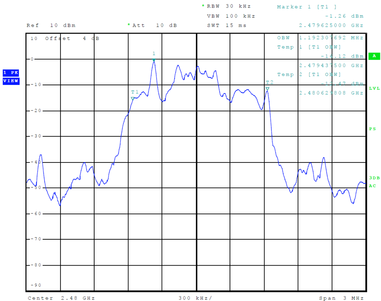
Figure 14 Plot of Transmitter Emissions 99% Occupied Bandwidth Mode 1 BT 3EDR
