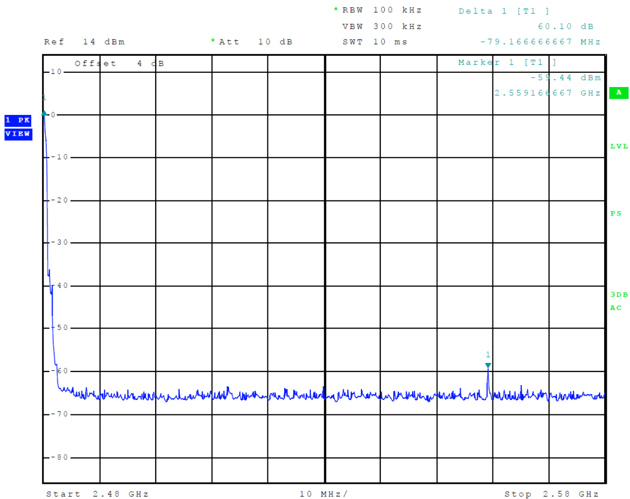
Figure 11 Plot of Transmitter Emissions High Band Edge Mode 3 BR 2EDR
