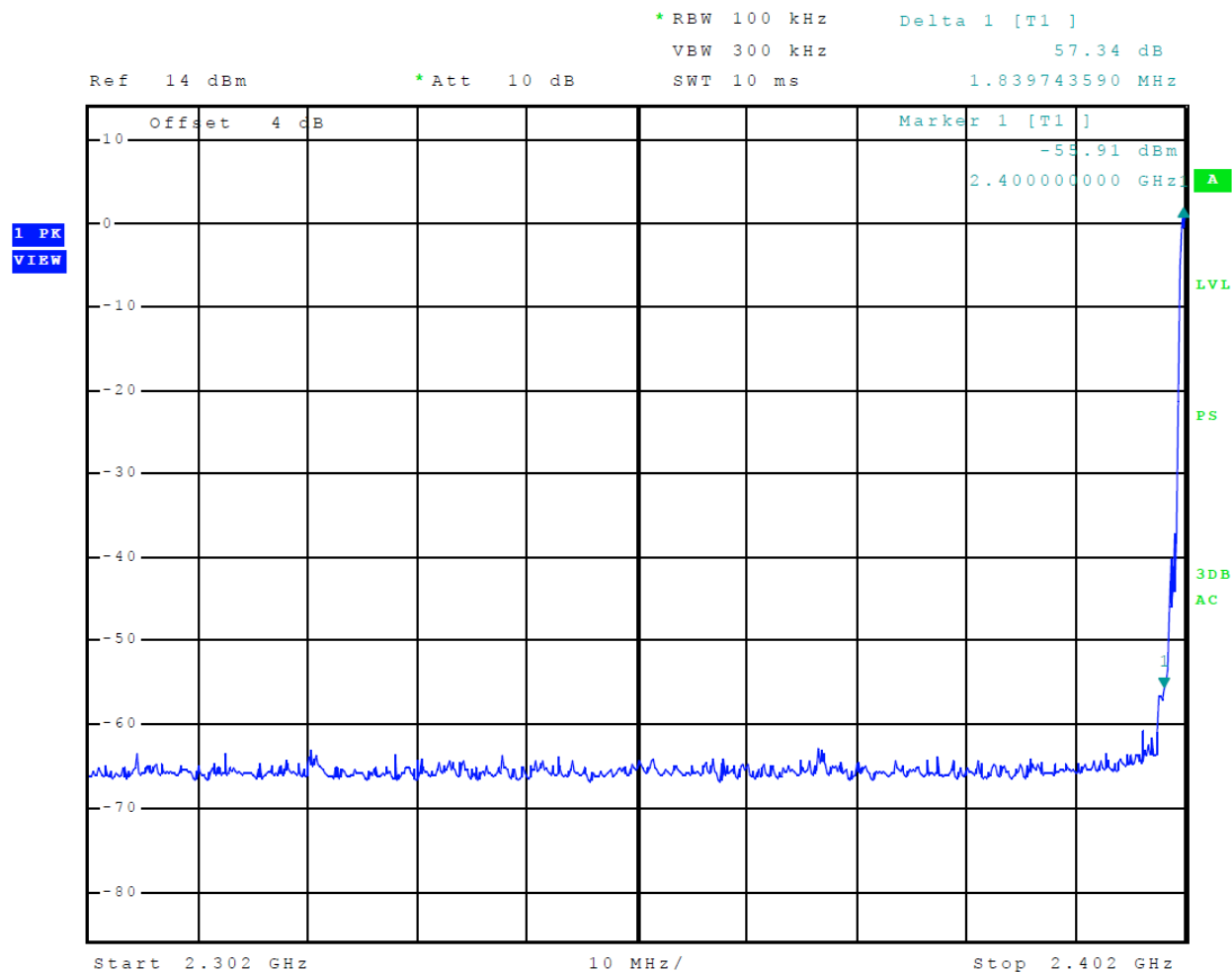
Figure 7 Plot of Transmitter Emissions Low Band Edge Mode 2 BT 2EDR
