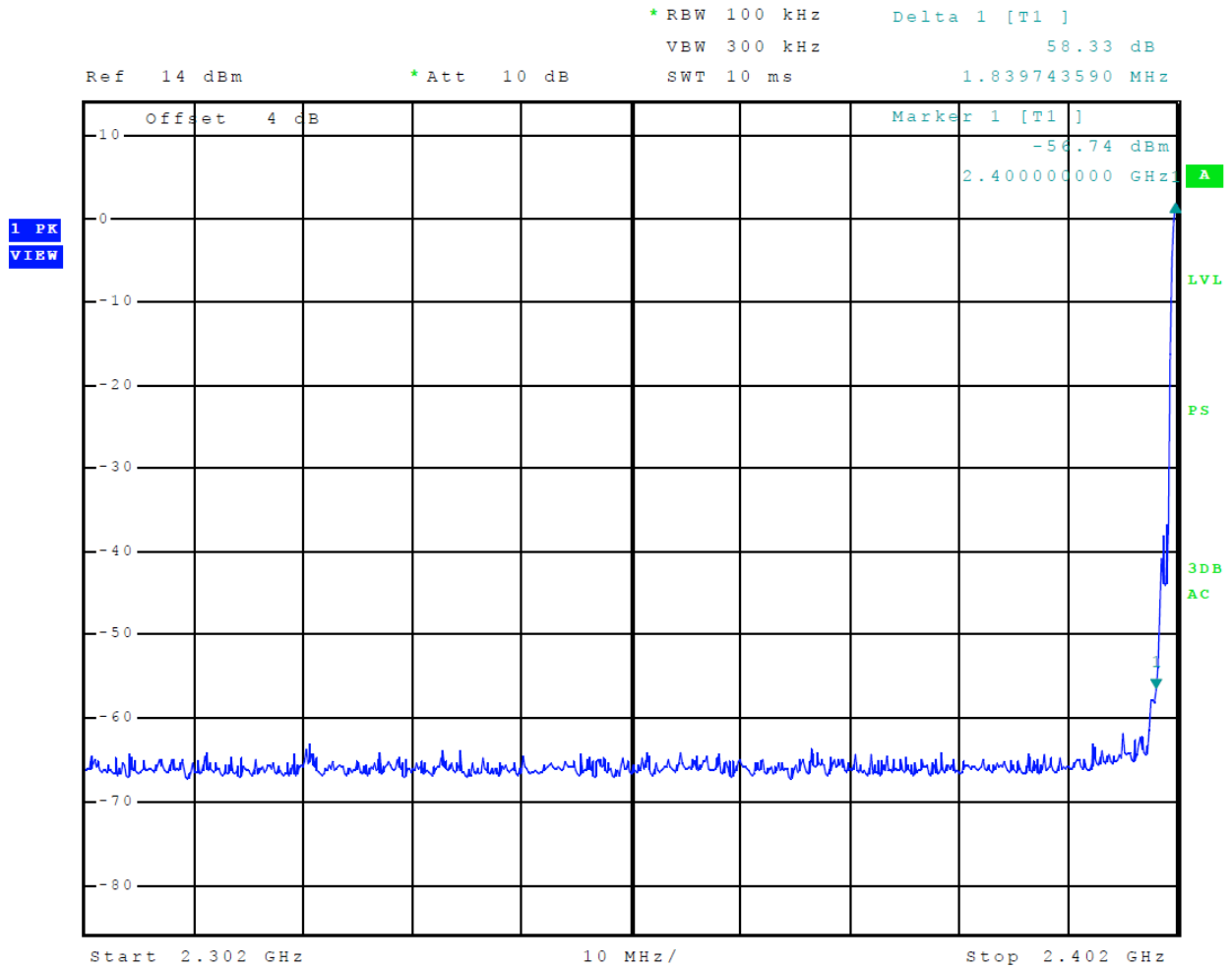
Figure 8 Plot of Transmitter Emissions Low Band Edge Mode 3 BT 3EDR
