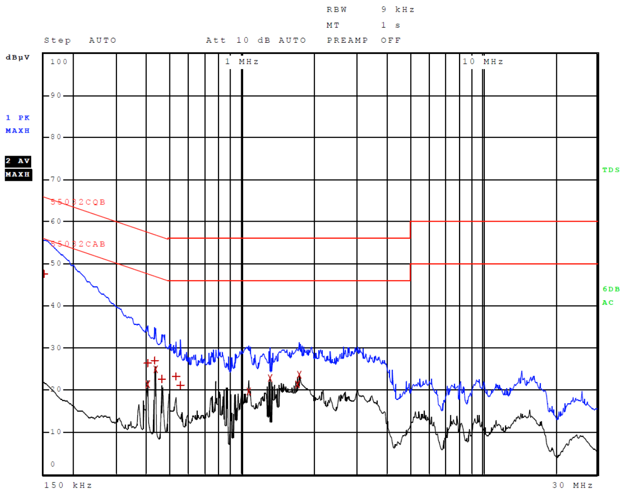
Figure 1 AC Line Conducted emissions of EUT line 1 (EUT – Computer)
