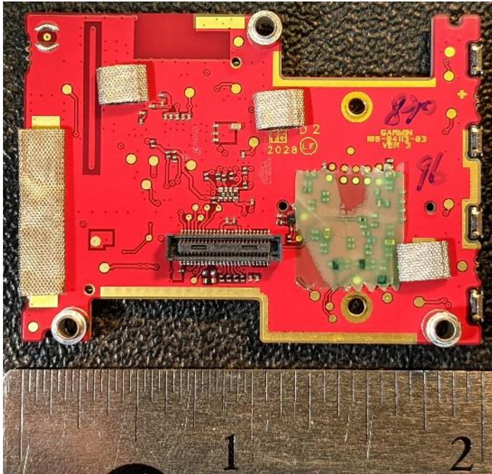
Sensor Board bottom side
