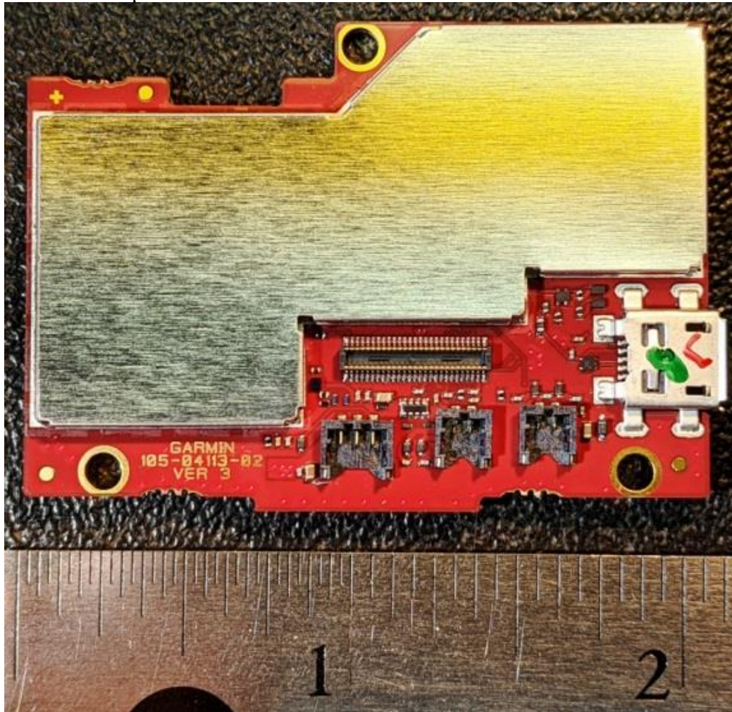
Main board top side shield
