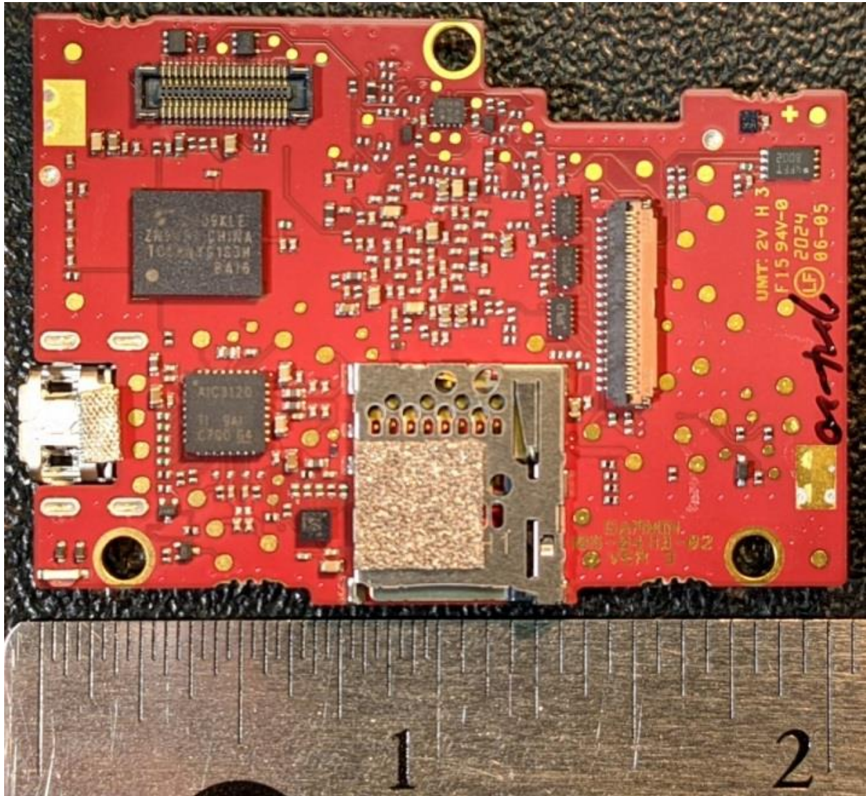
Main board bottom side
