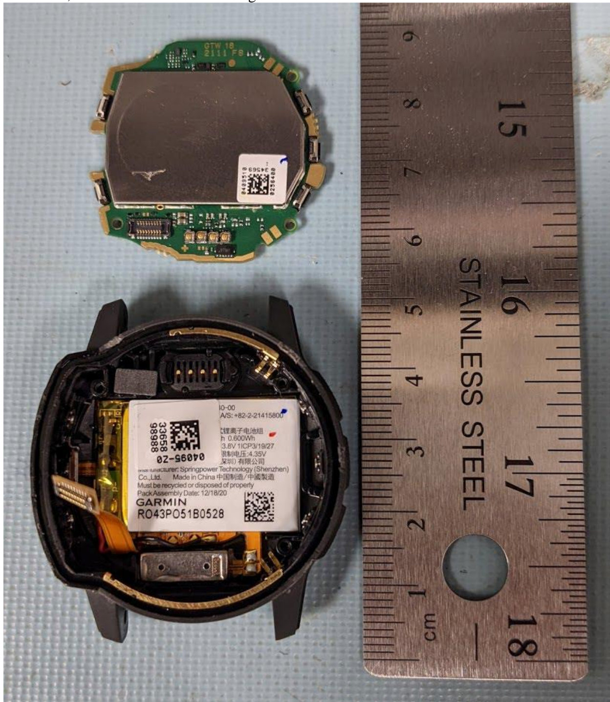
Rear Case, PCB removed with shielding
