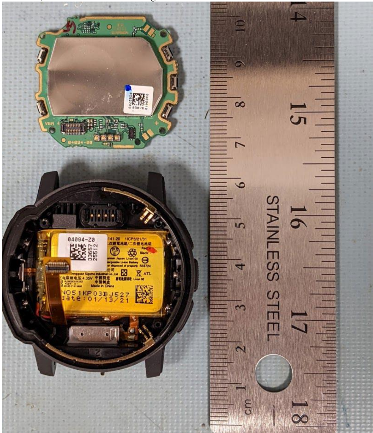
Rear Case, PCB removed with shielding
