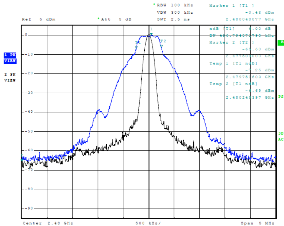
Figure Five Occupied Bandwidth (high channel)
