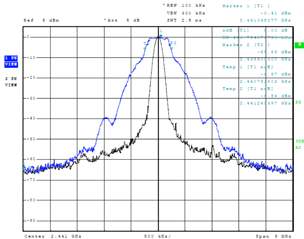
Figure Four Occupied Bandwidth (middle channel)
