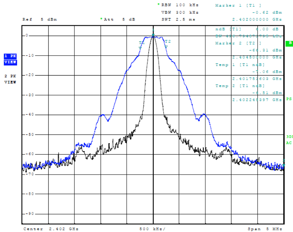
Figure Three Occupied Bandwidth (low channel)
