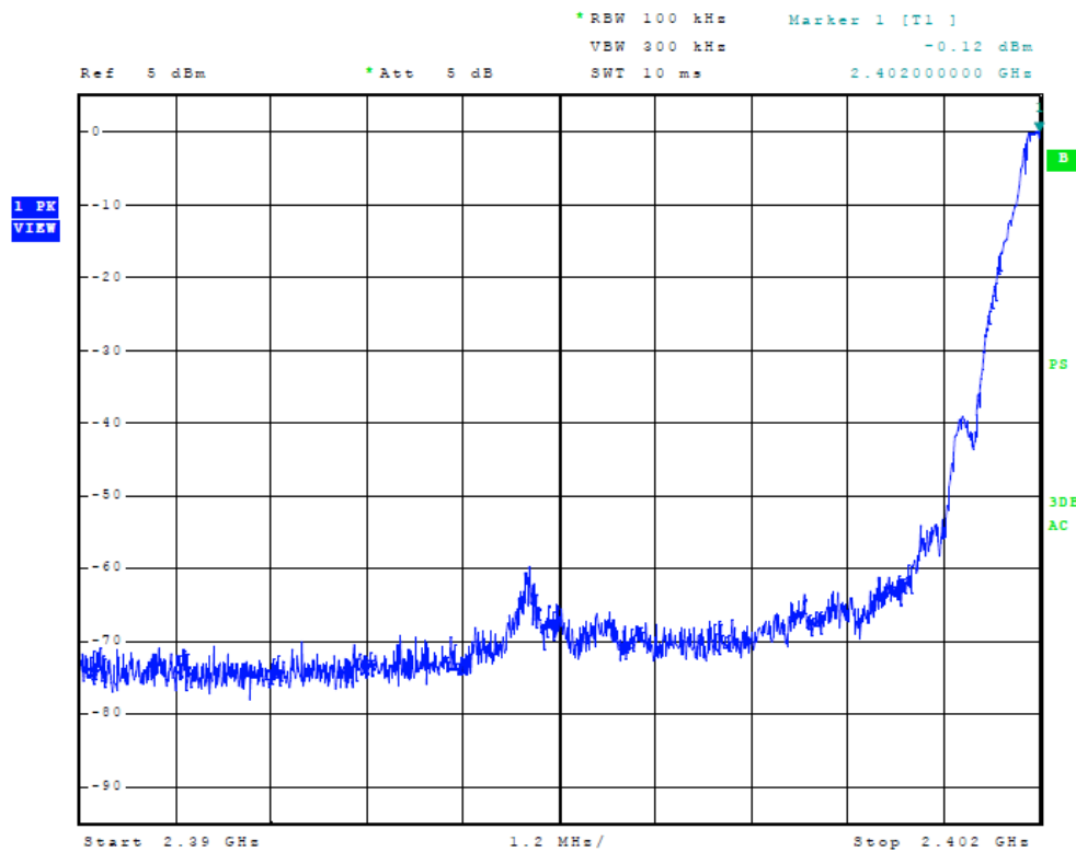
Figure 7 Plot of Lower Band Edge
