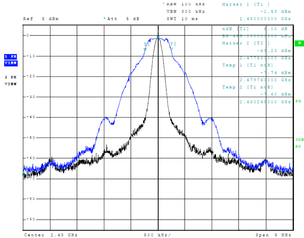
Figure 5 Plot of Occupied Bandwidth
