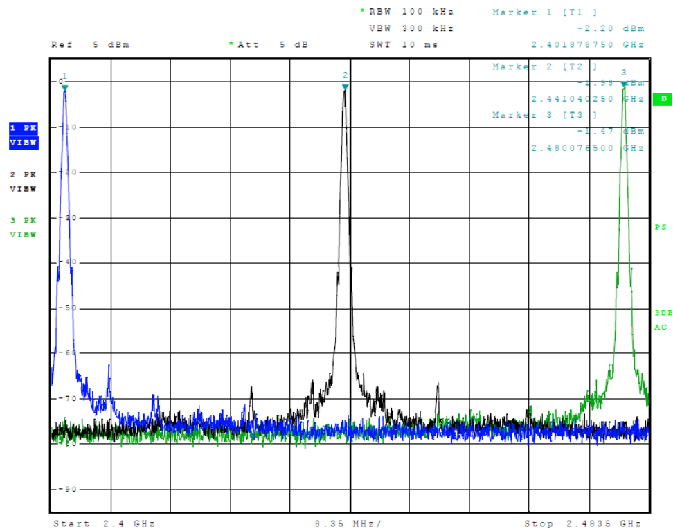
Figure 6 Plot of Operation across frequency band
