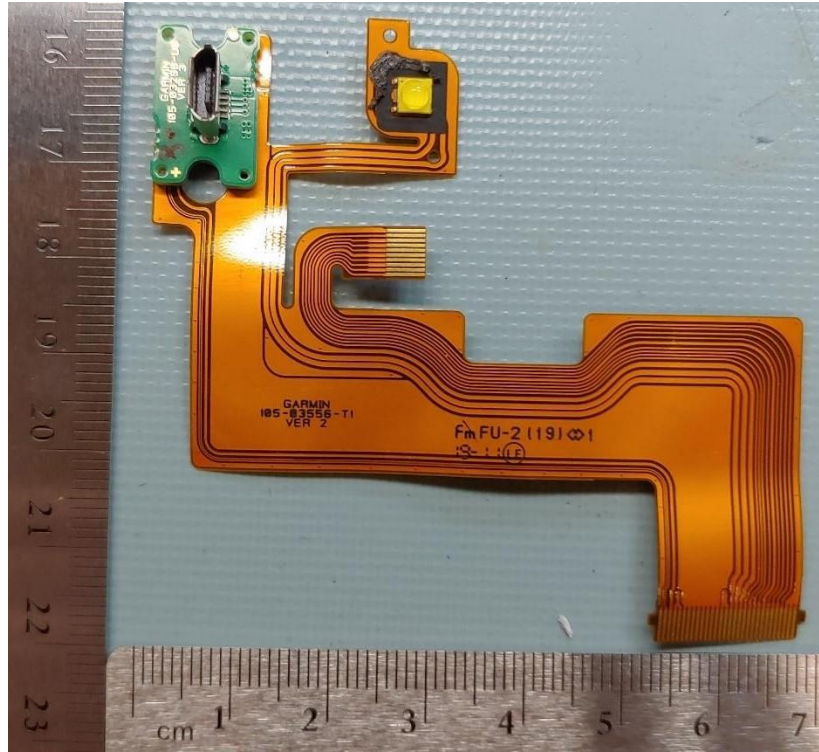
USB back
