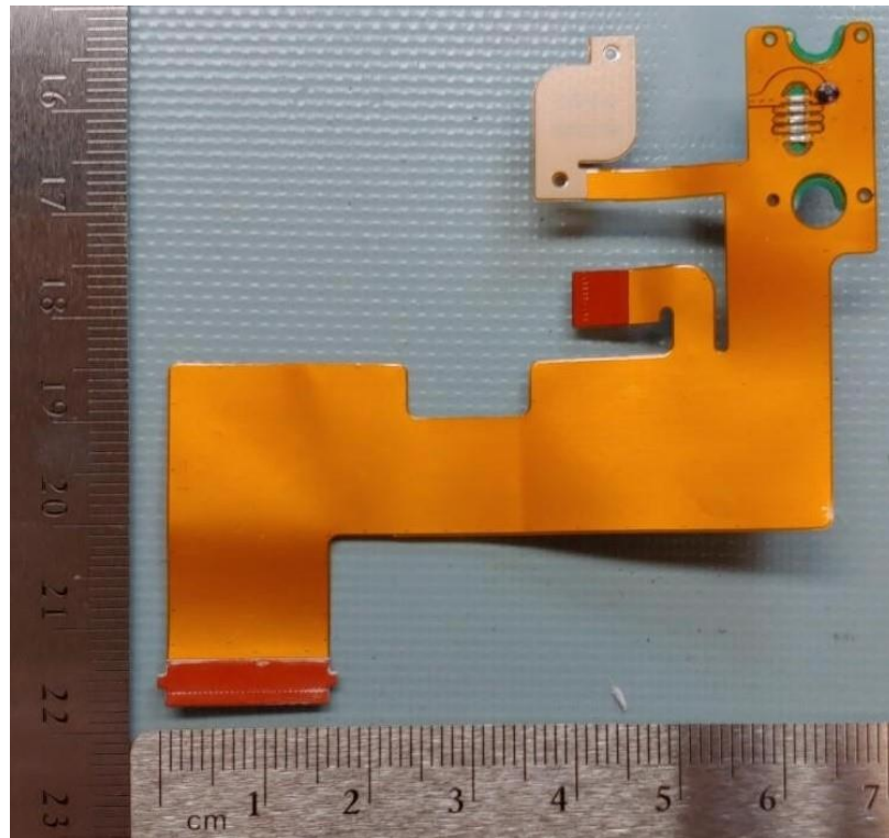
USB front
