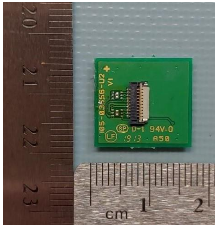
Micro SD card board – front
