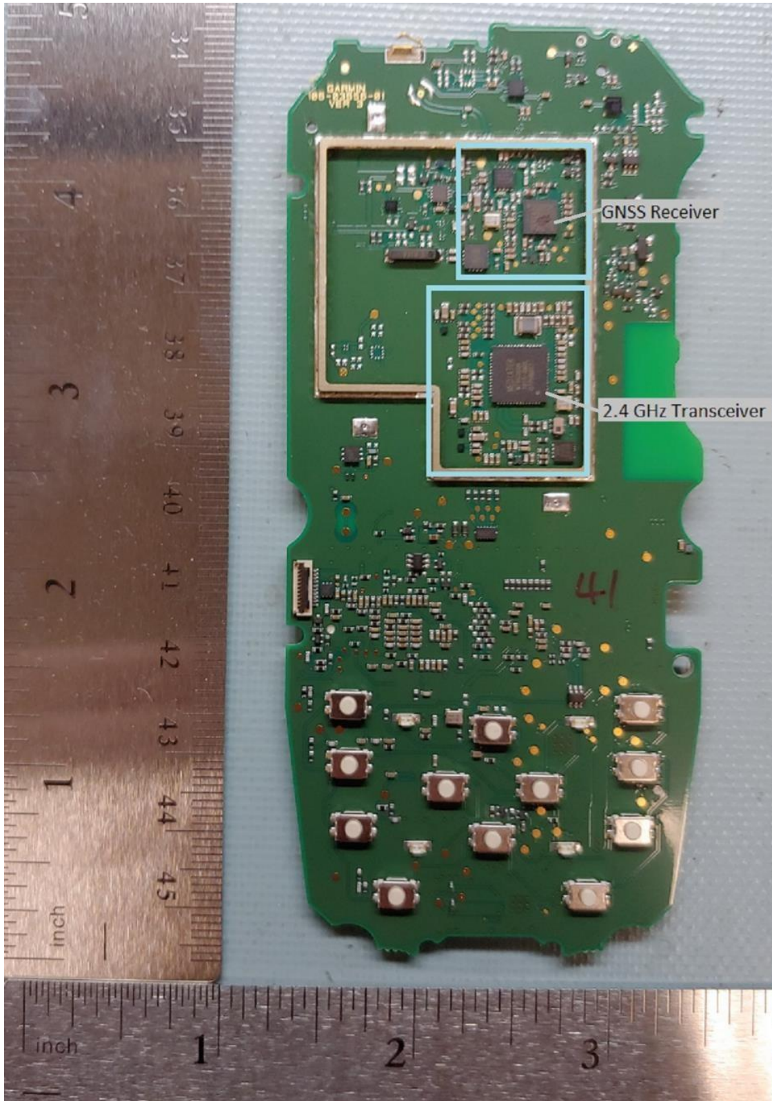
Main board front
