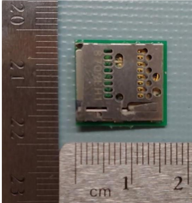
Micro SD card board – back
