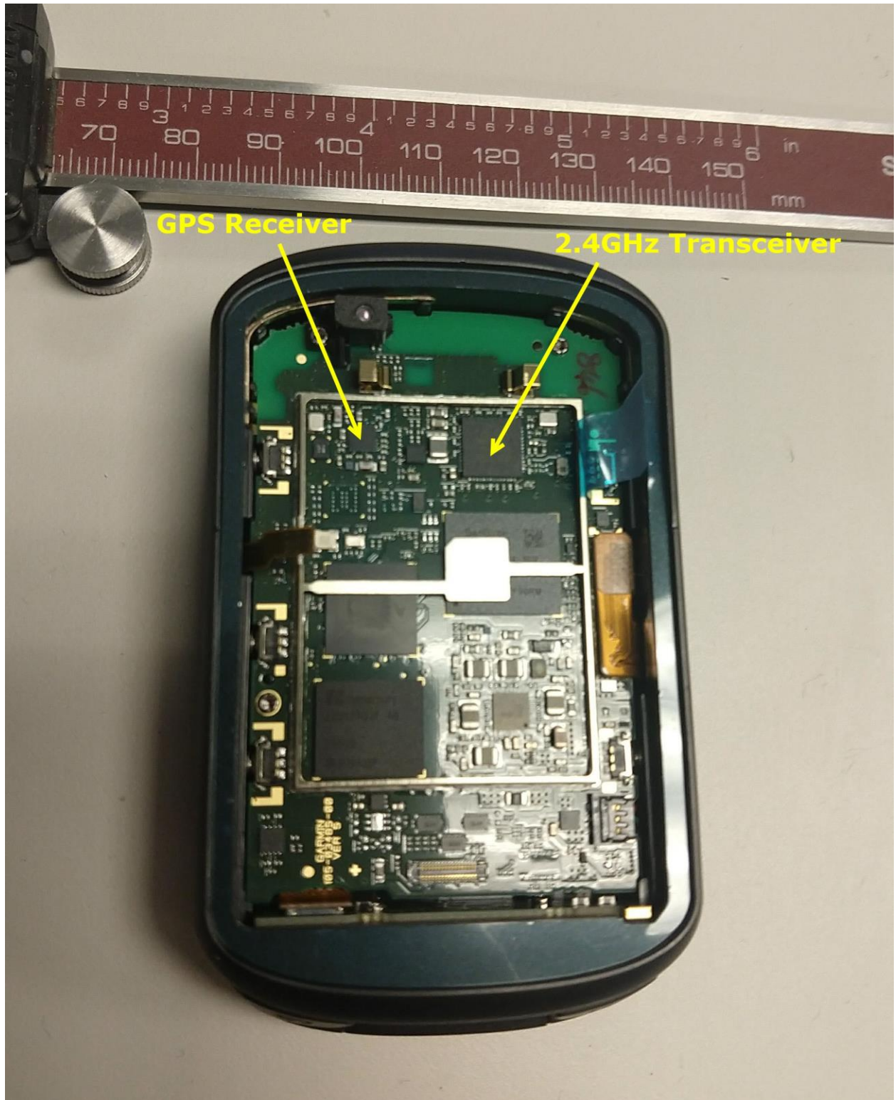
Top side of PCB with cover of shielded enclosure removed to show transceivers.
