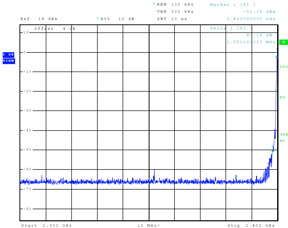
Figure 9 Plot of Transmitter Emissions (Low Band Edge, ANT)
