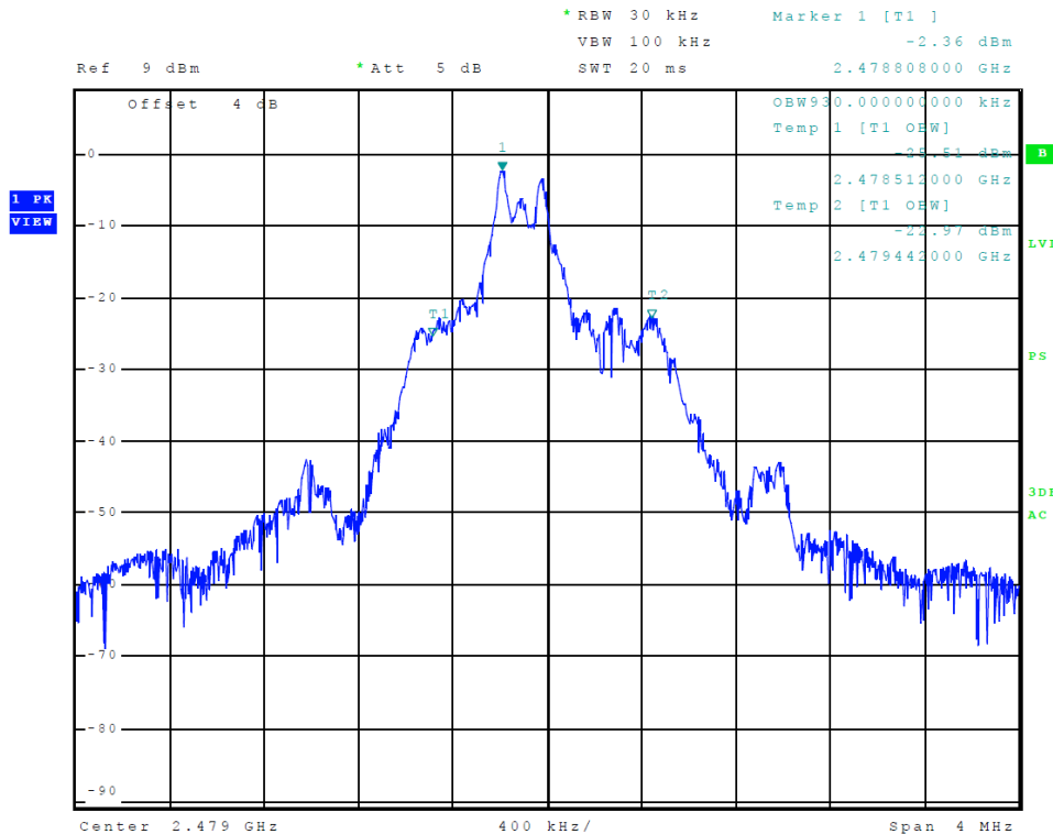
Figure 8 Plot of Transmitter Emissions (99% Occupied Bandwidth, ANT)
