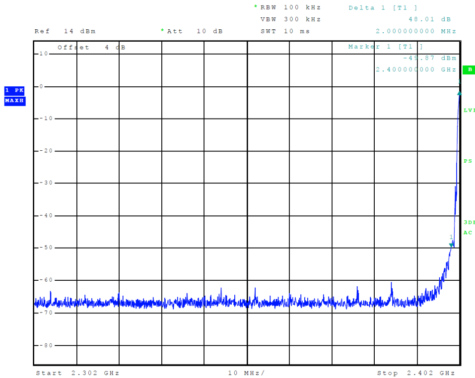
Figure 13 Plot of Transmitter Emissions (Low Band Edge, BLE PRB29)
