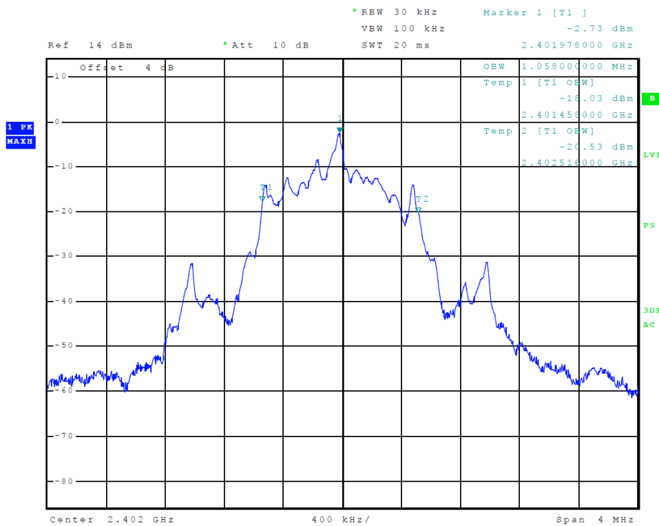
Figure 12 Plot of Transmitter Emissions (99% Occupied Bandwidth, BLE PRB29)
