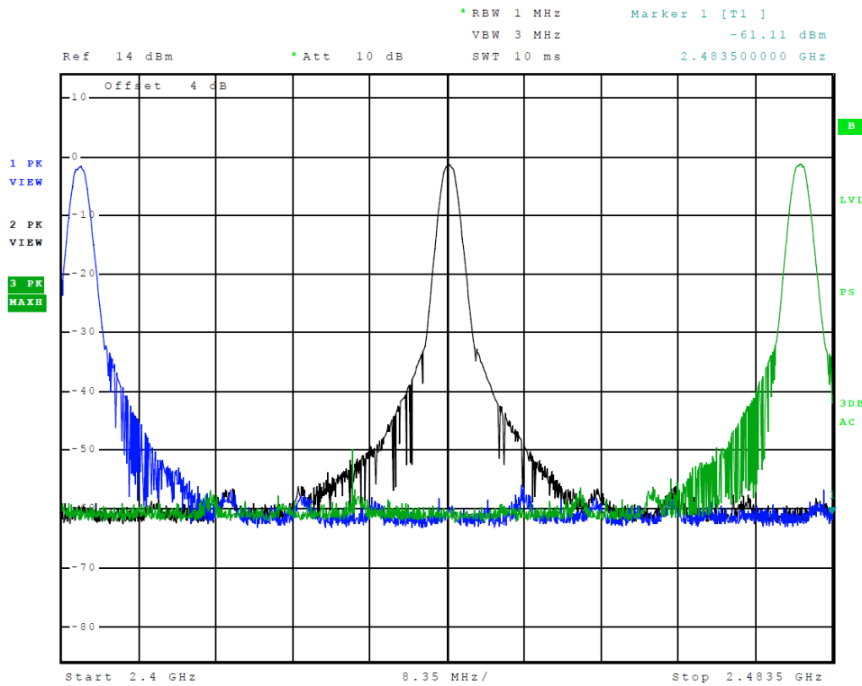
Figure 11 Plot of Transmitter Emissions (Operation in 2402-2480 MHz, BLE PRB29)
