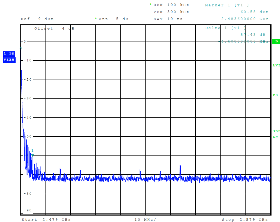
Figure 10 Plot of Transmitter Emissions (High Band Edge, ANT)
