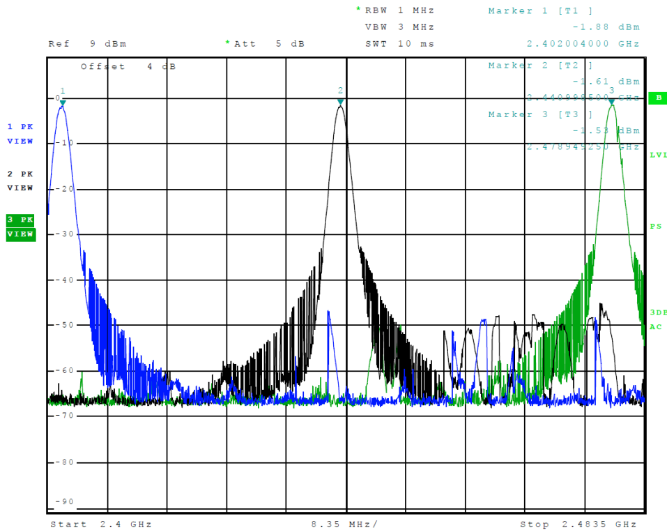
Figure 7 Plot of Transmitter Emissions (Operation in 2402-2479 MHz, ANT)
