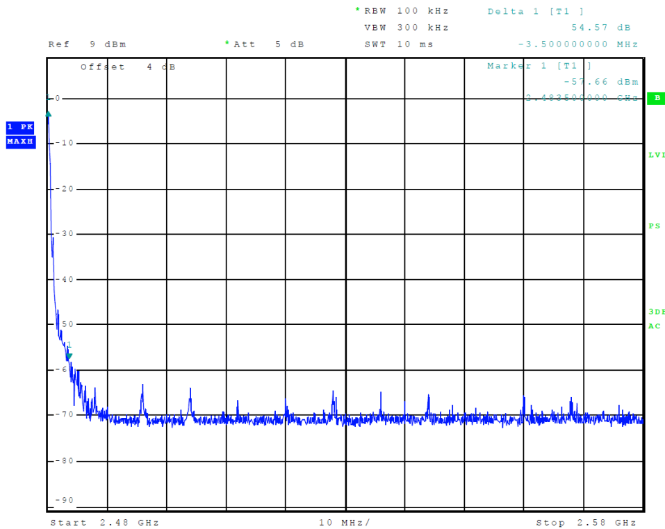
Figure 14 Plot of Transmitter Emissions (High Band Edge, BLE PRB29)
