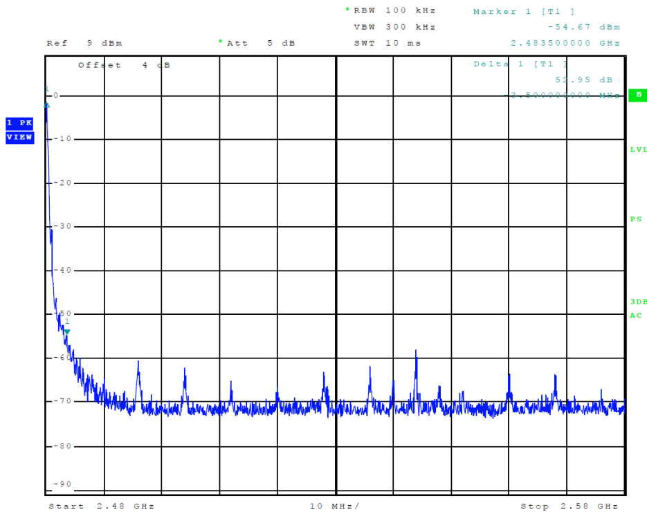
Figure 20 Plot of Transmitter Emissions (High Band Edge, BT 0x55)
