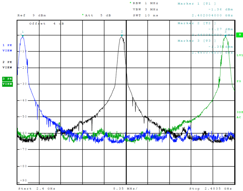
Figure 17 Plot of Transmitter Emissions (Operation in 2402-2480 MHz, BT 0x55)
