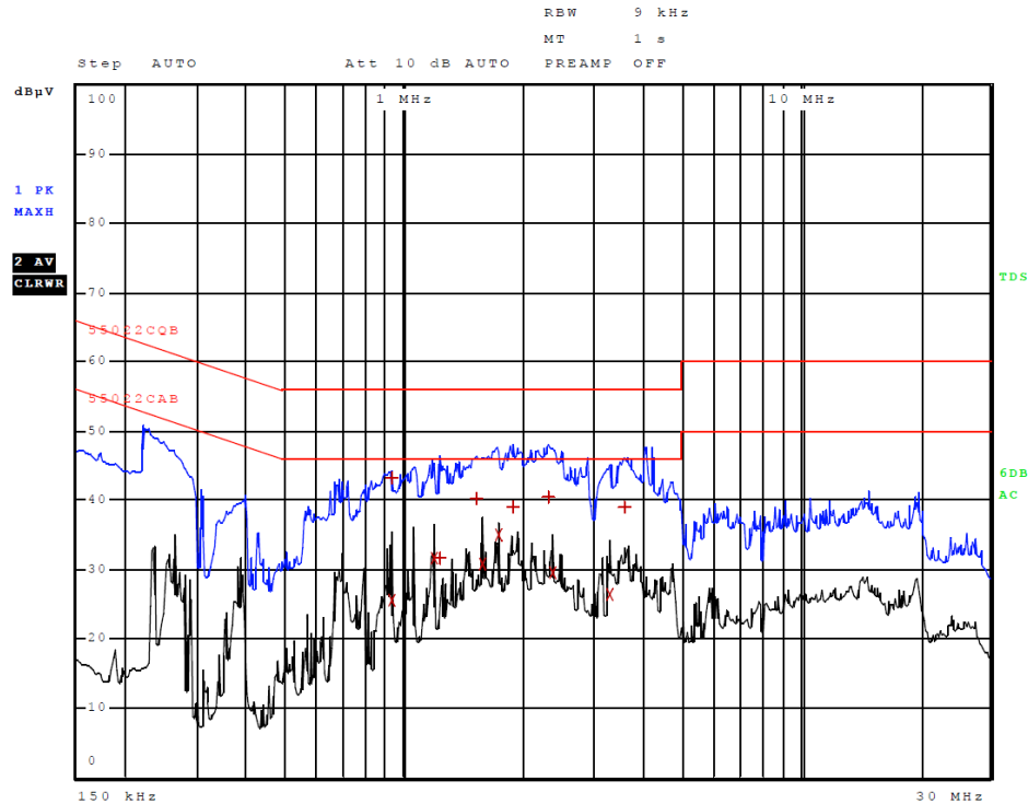
Figure 1 AC Line Conducted emissions of EUT line 1 (#2, EUT – CPU)
