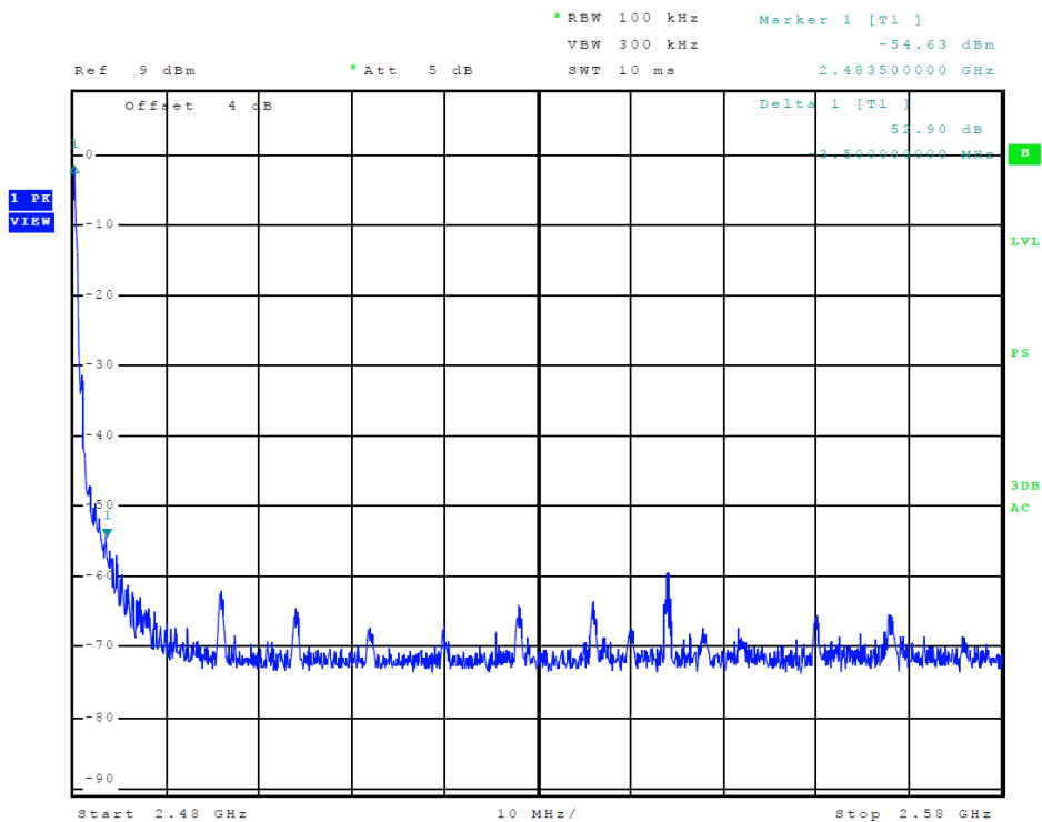
Figure 16 Plot of Transmitter Emissions (High Band Edge, BT 0x0F)
