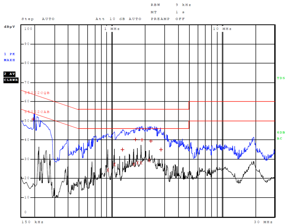
Figure 2 AC Line Conducted emissions of EUT line 2 (#2, EUT – CPU)
