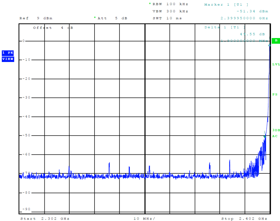
Figure 7 Plot of Transmitter Emissions (Low Band Edge, ANT)
