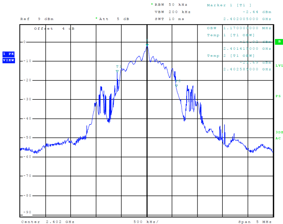
Figure 18 Plot of Transmitter Emissions (99% Occupied Bandwidth, BT 0x55)
