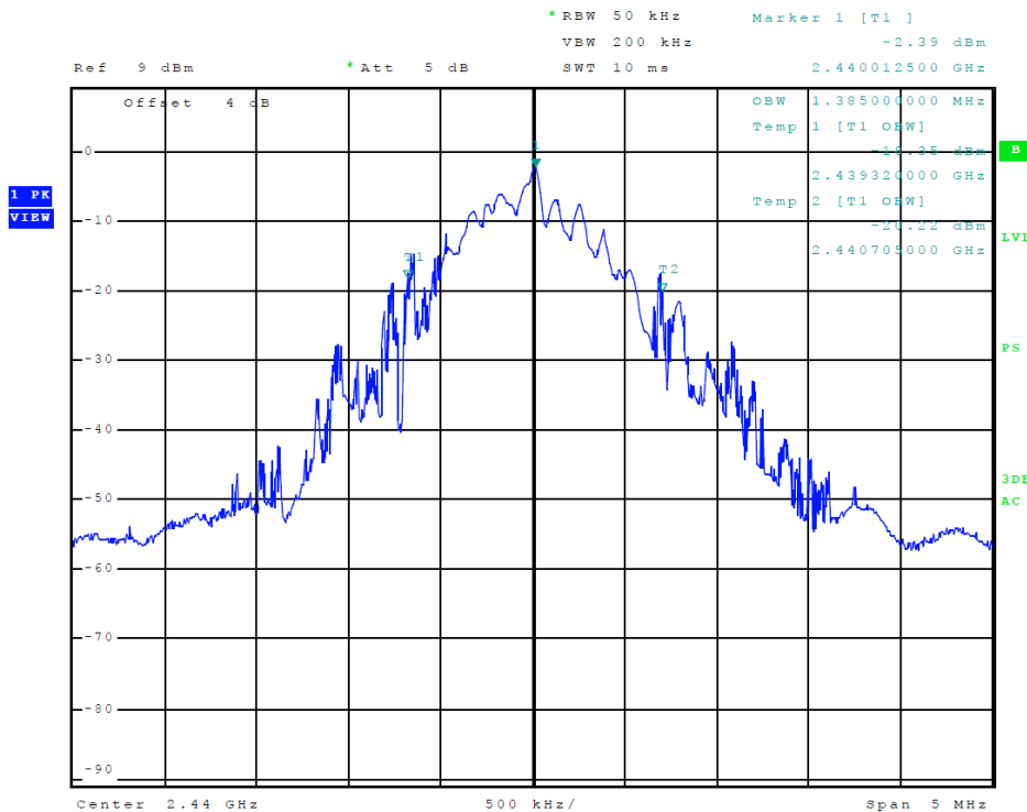
Figure 14 Plot of Transmitter Emissions (99% Occupied Bandwidth, BT 0x0F)
