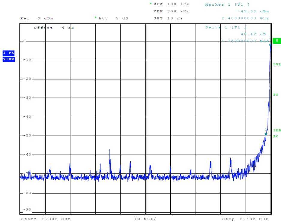
Figure 11 Plot of Transmitter Emissions (Low Band Edge, BT PRB29)
