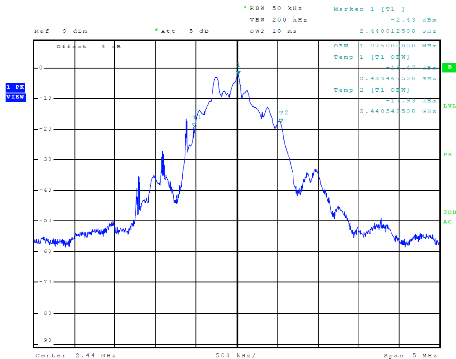
Figure 10 Plot of Transmitter Emissions (99% Occupied Bandwidth, BT PRB29)
