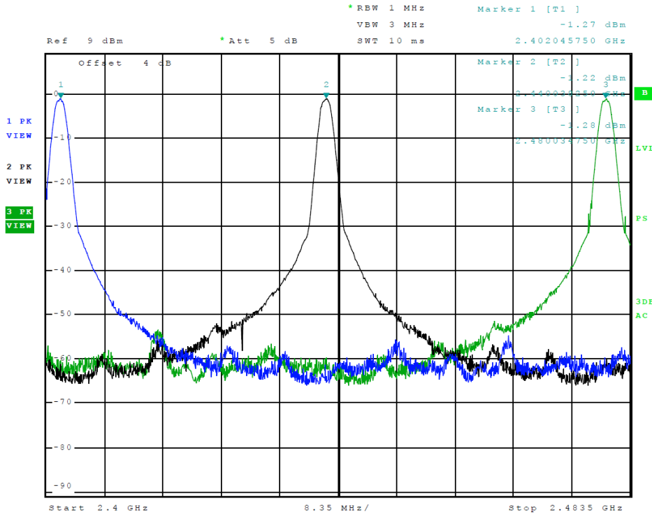
Figure 13 Plot of Transmitter Emissions (Operation in 2402-2480 MHz, BT 0x0F)
