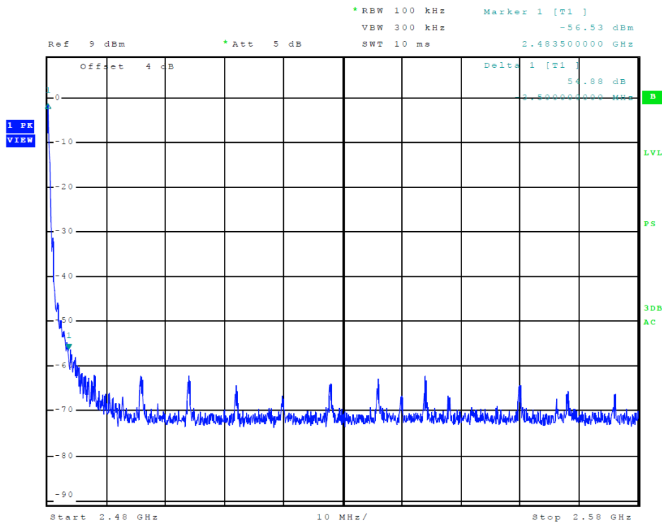
Figure 12 Plot of Transmitter Emissions (High Band Edge, BT PRB29)
