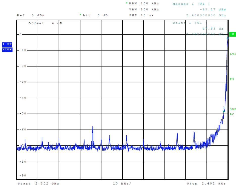
Figure 19 Plot of Transmitter Emissions (Low Band Edge, BT 0x55)
