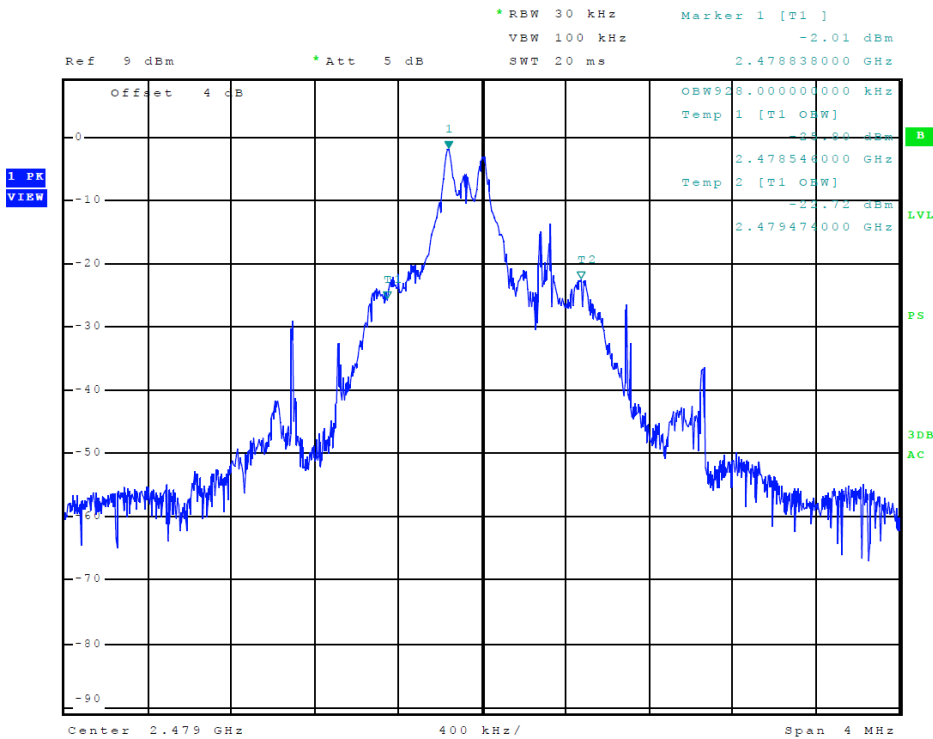
Figure 6 Plot of Transmitter Emissions (99% Occupied Bandwidth, ANT)
