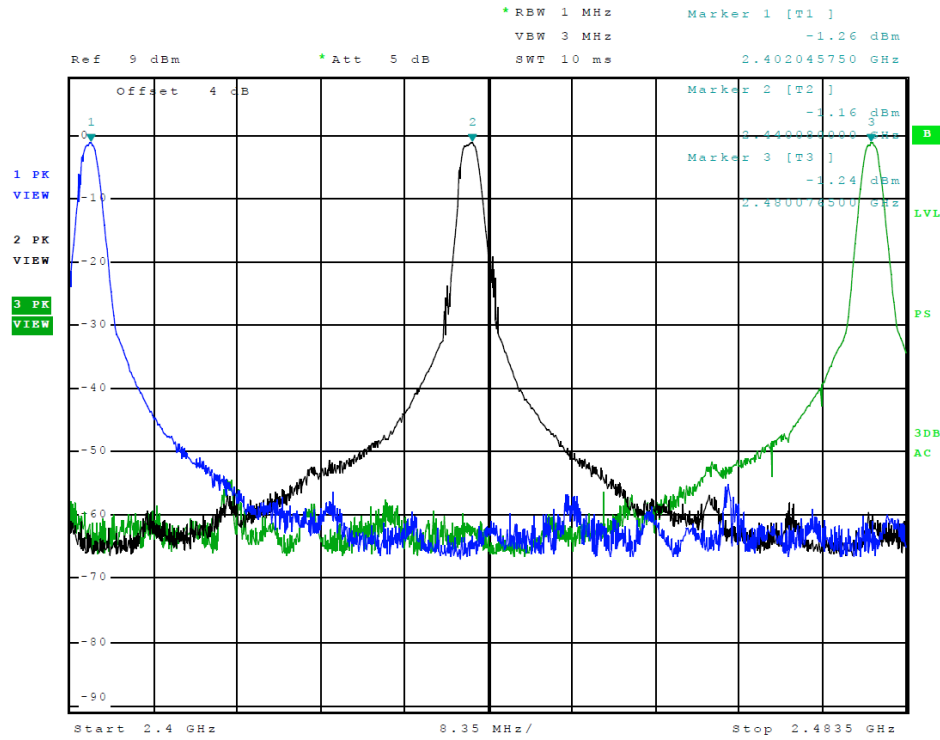
Figure 9 Plot of Transmitter Emissions (Operation in 2402-2480 MHz, BT PRB29)
