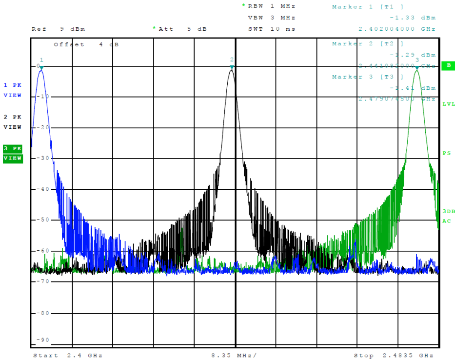
Figure 5 Plot of Transmitter Emissions (Operation in 2402-2480 MHz, ANT)
