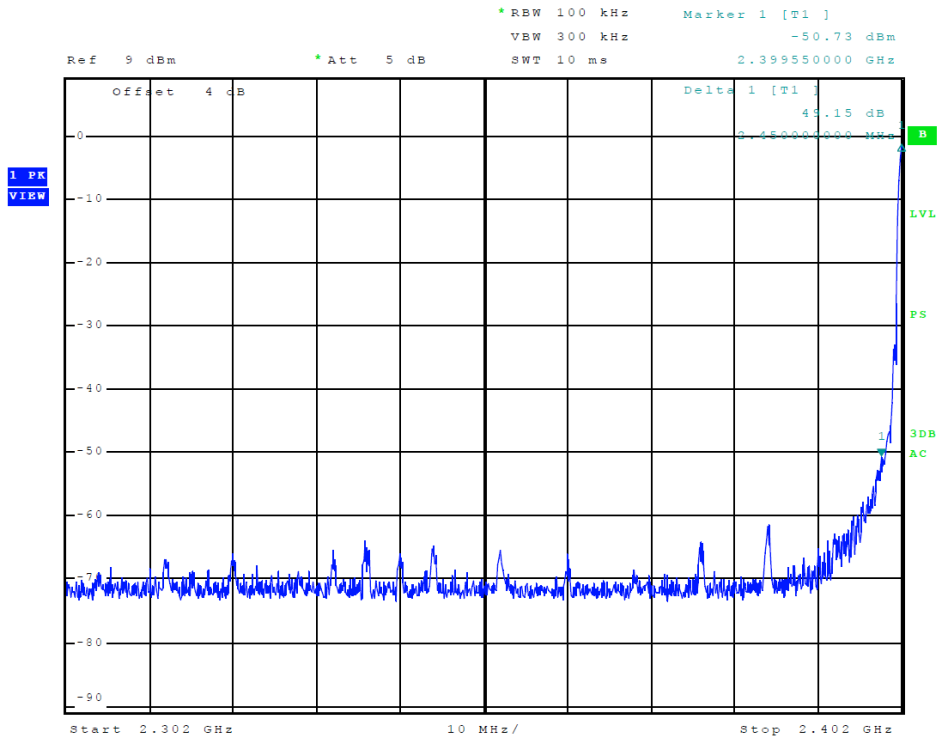
Figure 15 Plot of Transmitter Emissions (Low Band Edge, BT 0x0F)
