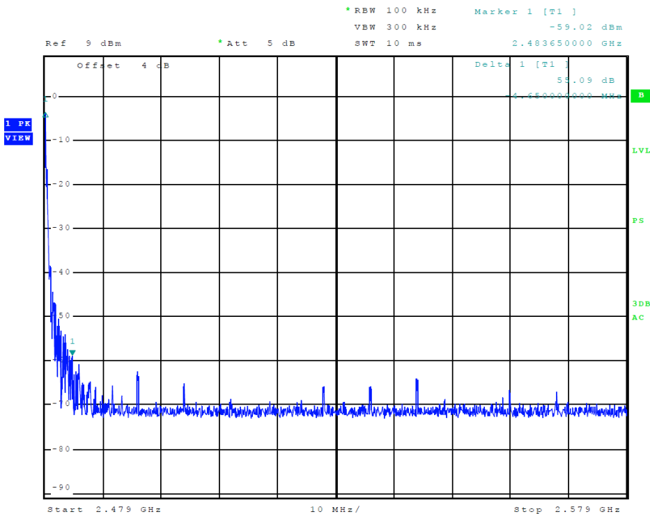
Figure 8 Plot of Transmitter Emissions (High Band Edge, ANT)
