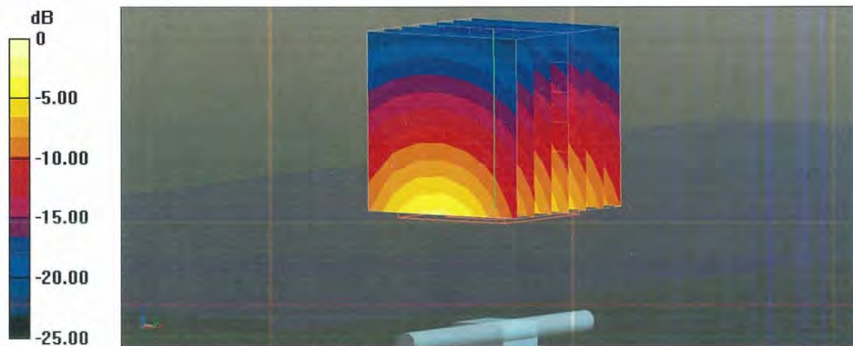
0 dB = 20.8 W/kg = 13.18 dBW/kg
