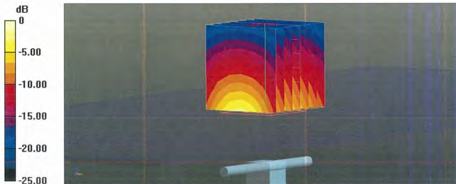
0 dB = 20.0 W/kg = 13.01 dBW/kg
