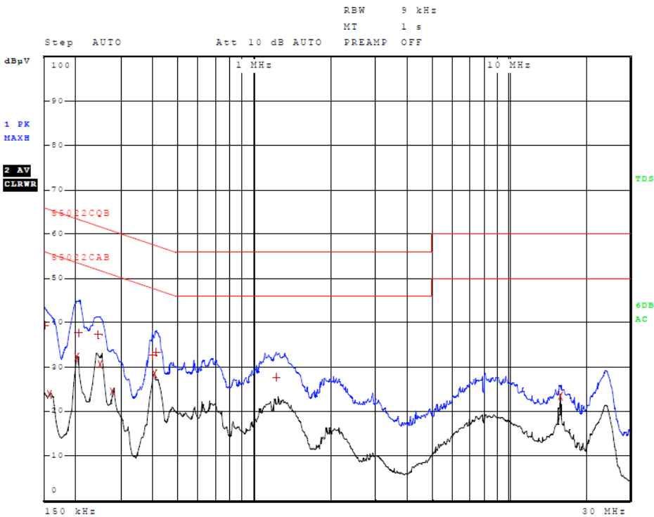
Figure 4 AC Line Conducted emissions of EUT line 2 (#3, EUT AC Adapter)
