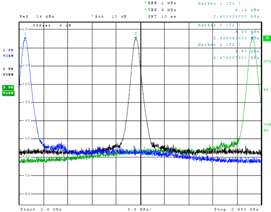
Figure 5 Plot of Transmitter Emissions (ANT, Mode 1 Operation in 2402-2480 MHz)
