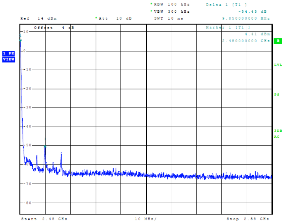
Figure 8 Plot of Transmitter Emissions (ANT, Mode 1 High Band Edge)
