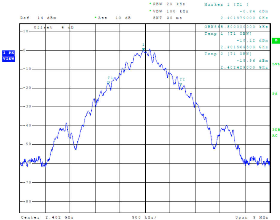
Figure 6 Plot of Transmitter Emissions (ANT, Mode 1 99% Occupied Bandwidth)
