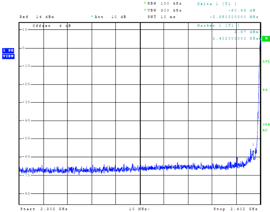
Figure 7 Plot of Transmitter Emissions (ANT, Mode 1 Low Band Edge)
