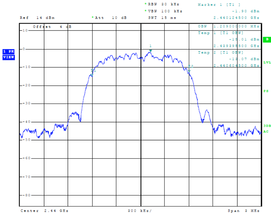
Figure 10 Plot of Transmitter Emissions (BT, Mode 2 99% Occupied Bandwidth)
