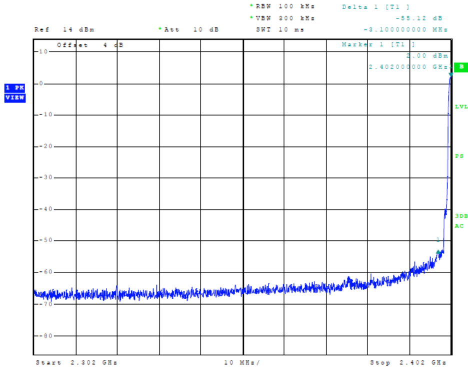
Figure 11 Plot of Transmitter Emissions (BT, Mode 2 Low Band Edge)
