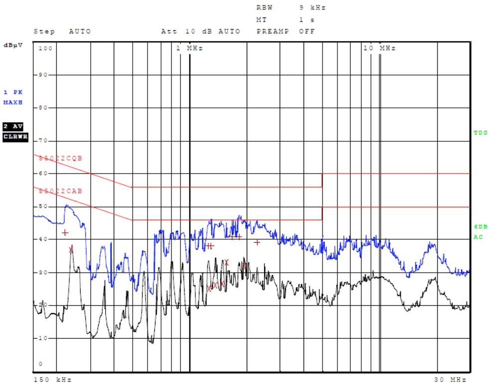
Figure 2 AC Line Conducted emissions of EUT line 2 (#2, EUT USB CPU Adapter)
