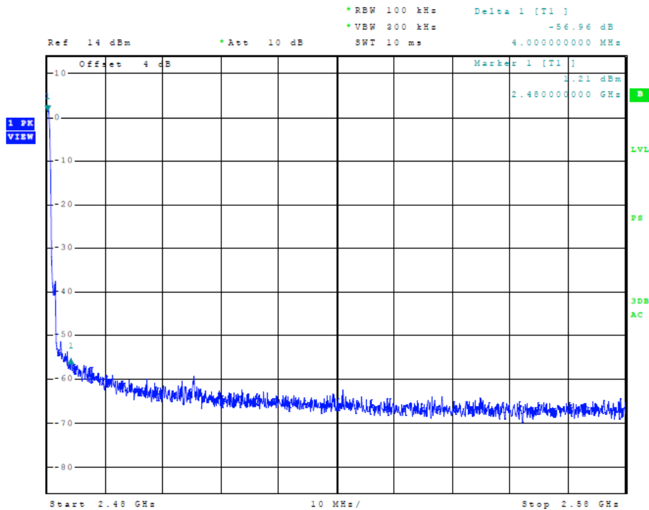
Figure 12 Plot of Transmitter Emissions (BT, Mode 2 High Band Edge)
