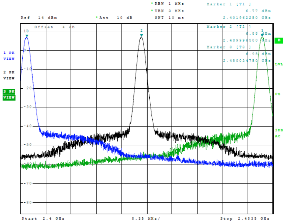
Figure 9 Plot of Transmitter Emissions (BT, Mode 2 Operation in 2402-2480 MHz)
