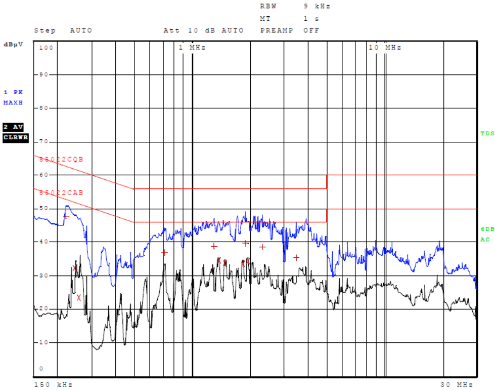
Figure 1 AC Line Conducted emissions of EUT line 1 (#2, EUT USB CPU Adapter)
