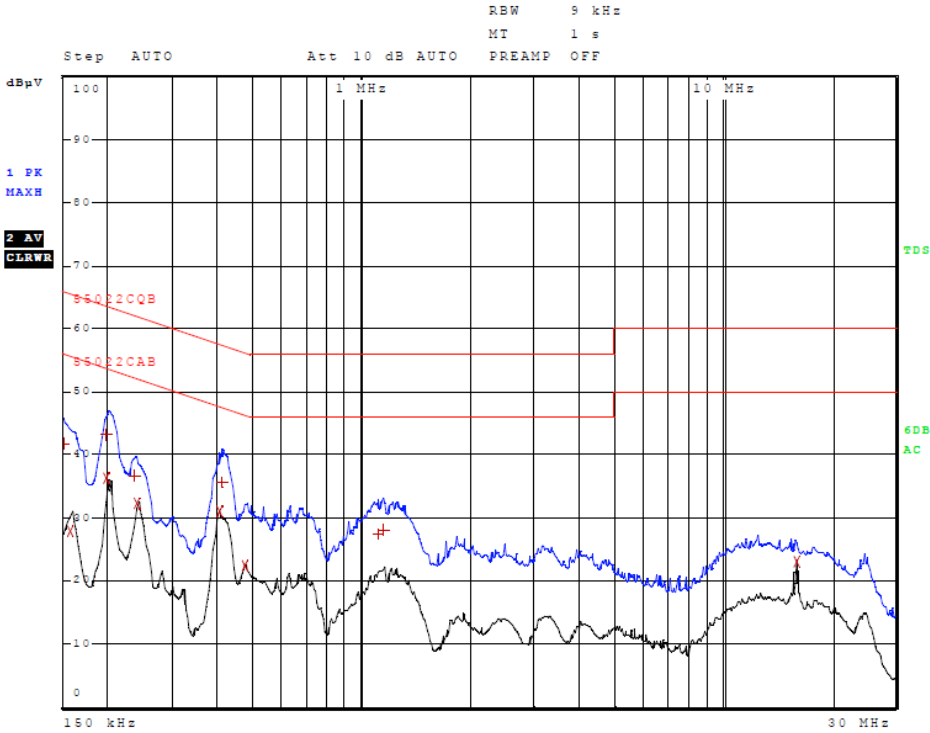
Figure 3 AC Line Conducted emissions of EUT line 1 (#3, EUT AC Adapter)
