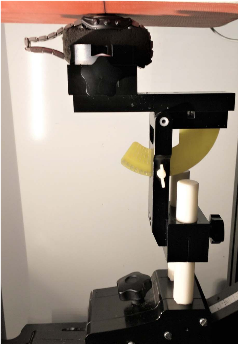
Figure E16.11 – Setup, DUT Back Side
