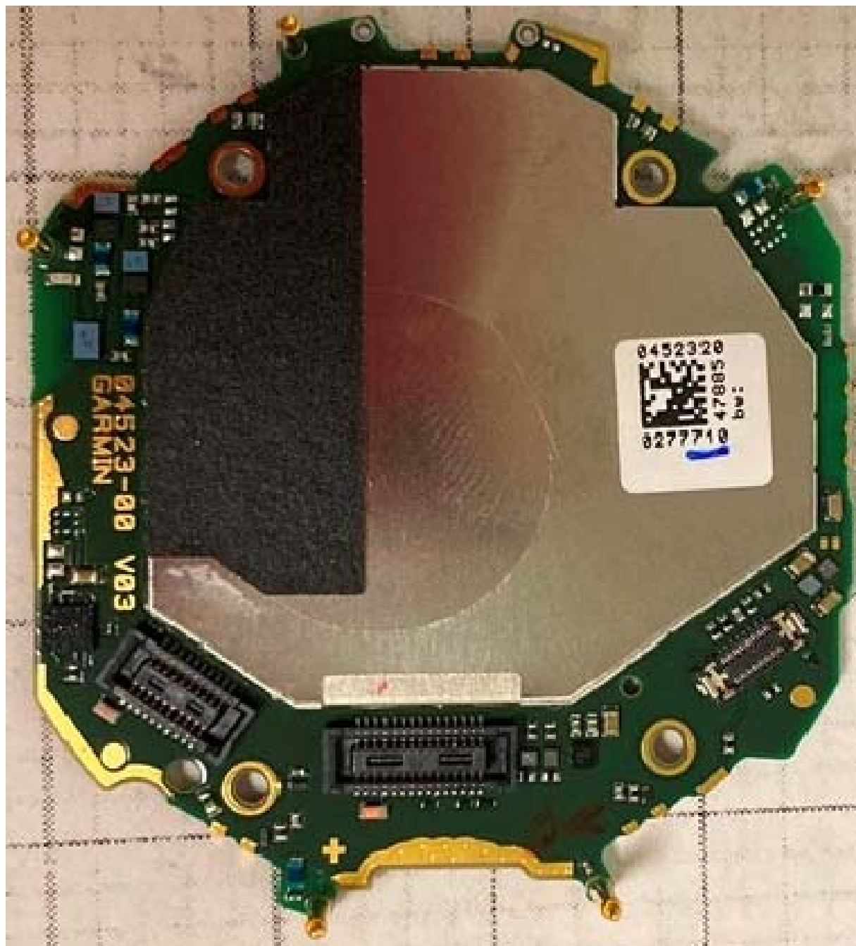
Figure E15.4 – Internal, PCB Top Side
