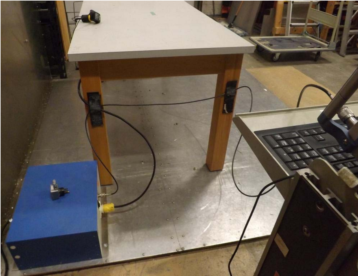
Figure E16.9 – Setup, Line Conducted Measurements
