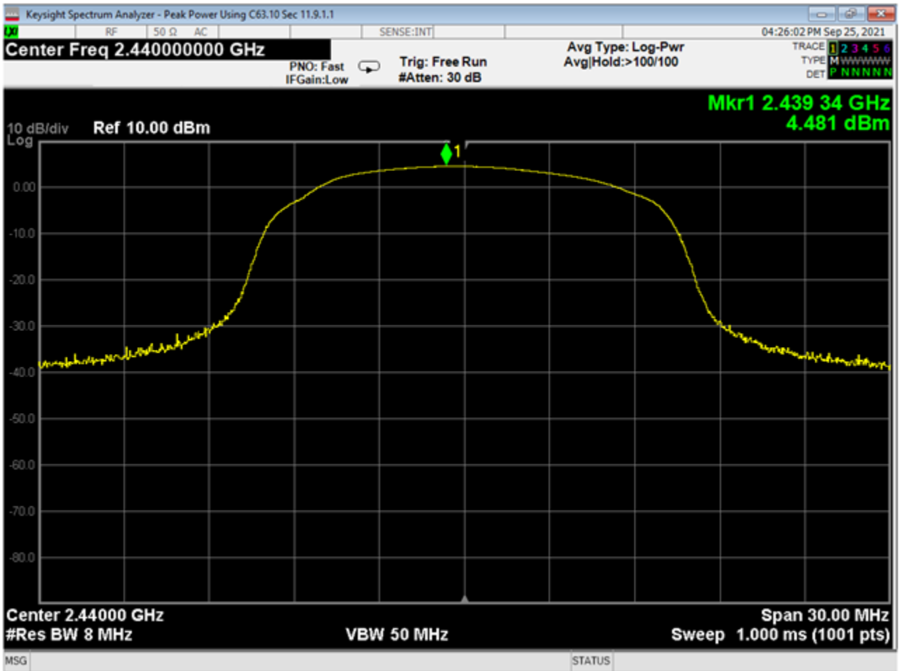
15 Peak Power, Mid Channel, GMSK 1MB
