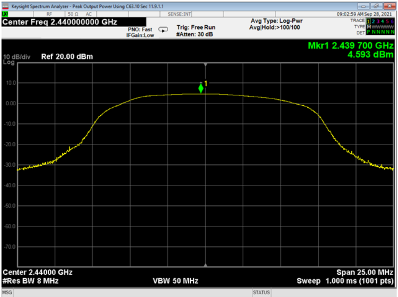
28 Peak Power, Mid Channel, GMSK 2MB
