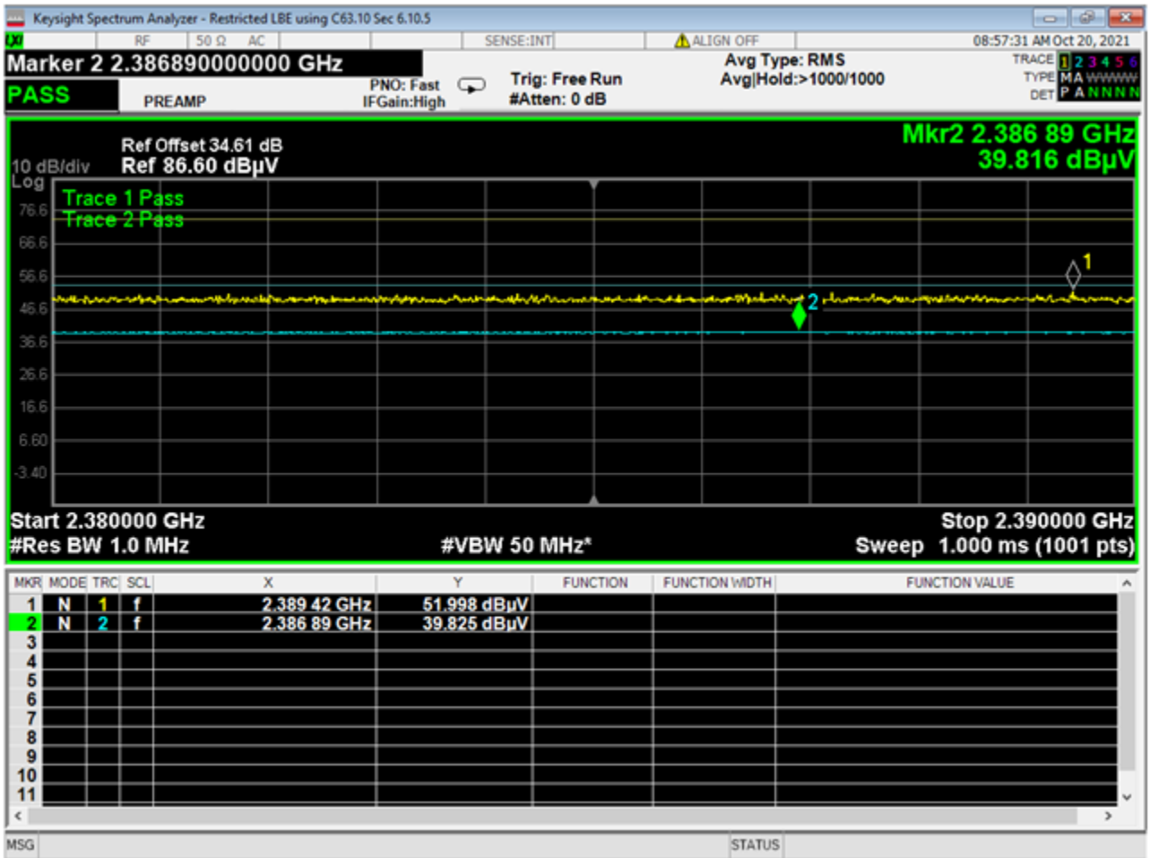
25 LBE, Restricted GMSK 1MB
