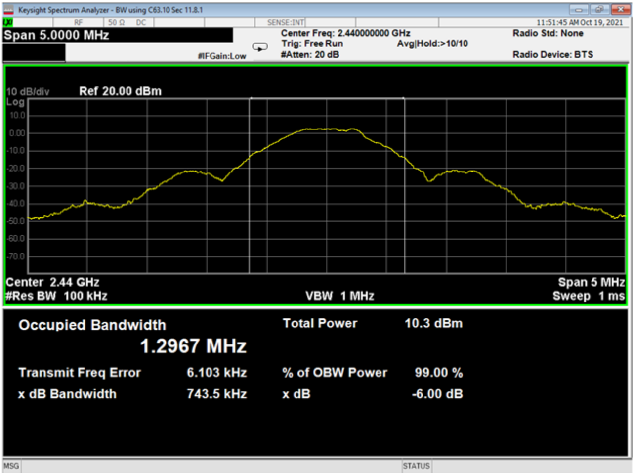
05 OBW-6dB, Mid Channel, GFSK
