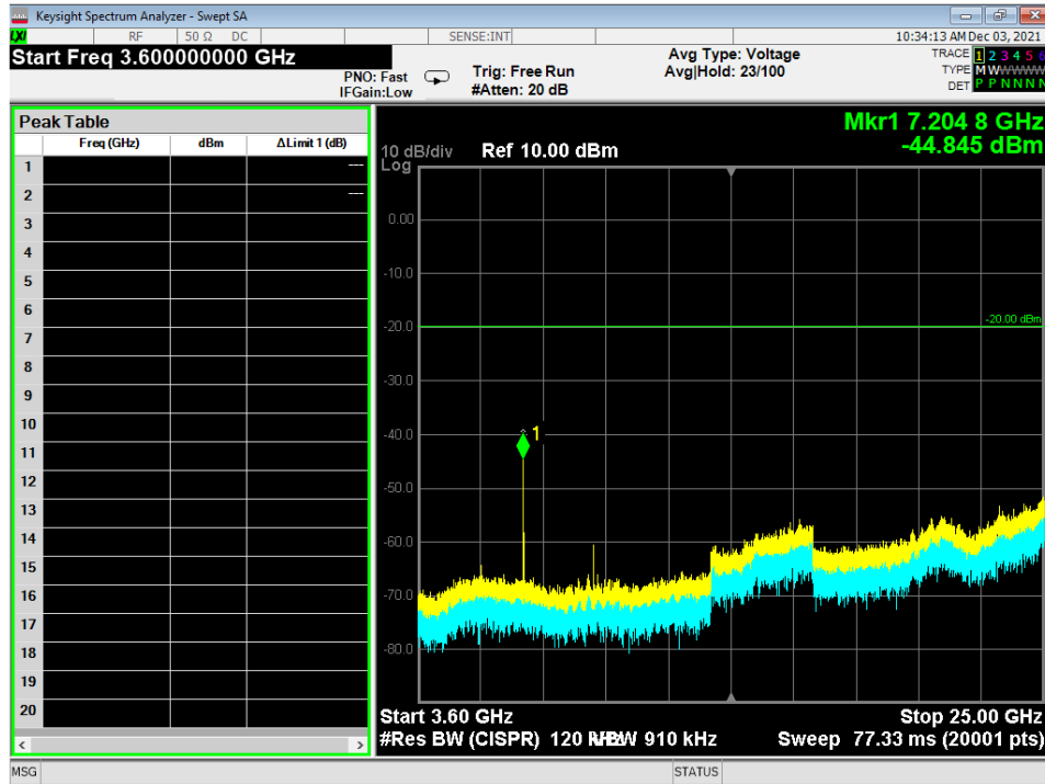
Figure 10 - Radiated Emissions Plot, GFSK, 3.6G – 25G, Low
