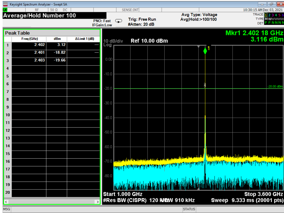
Figure 12 - Radiated Emissions Plot, GMSK 1MB, 1G – 3.6G, Low
