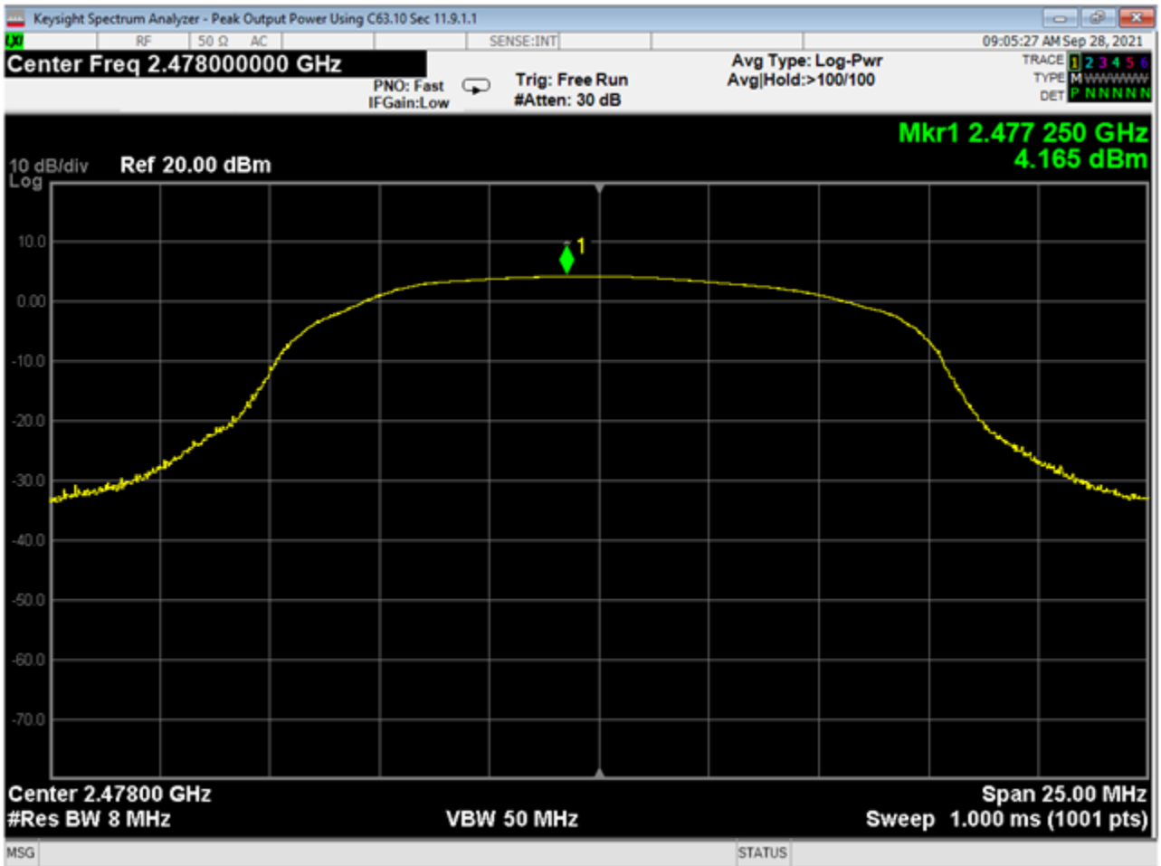
29 Peak Power, High Channel, GMSK 2MB
