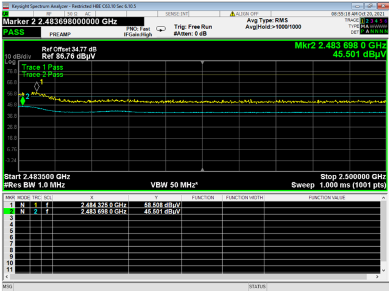
26 HBE, Restricted GMSK 1MB
