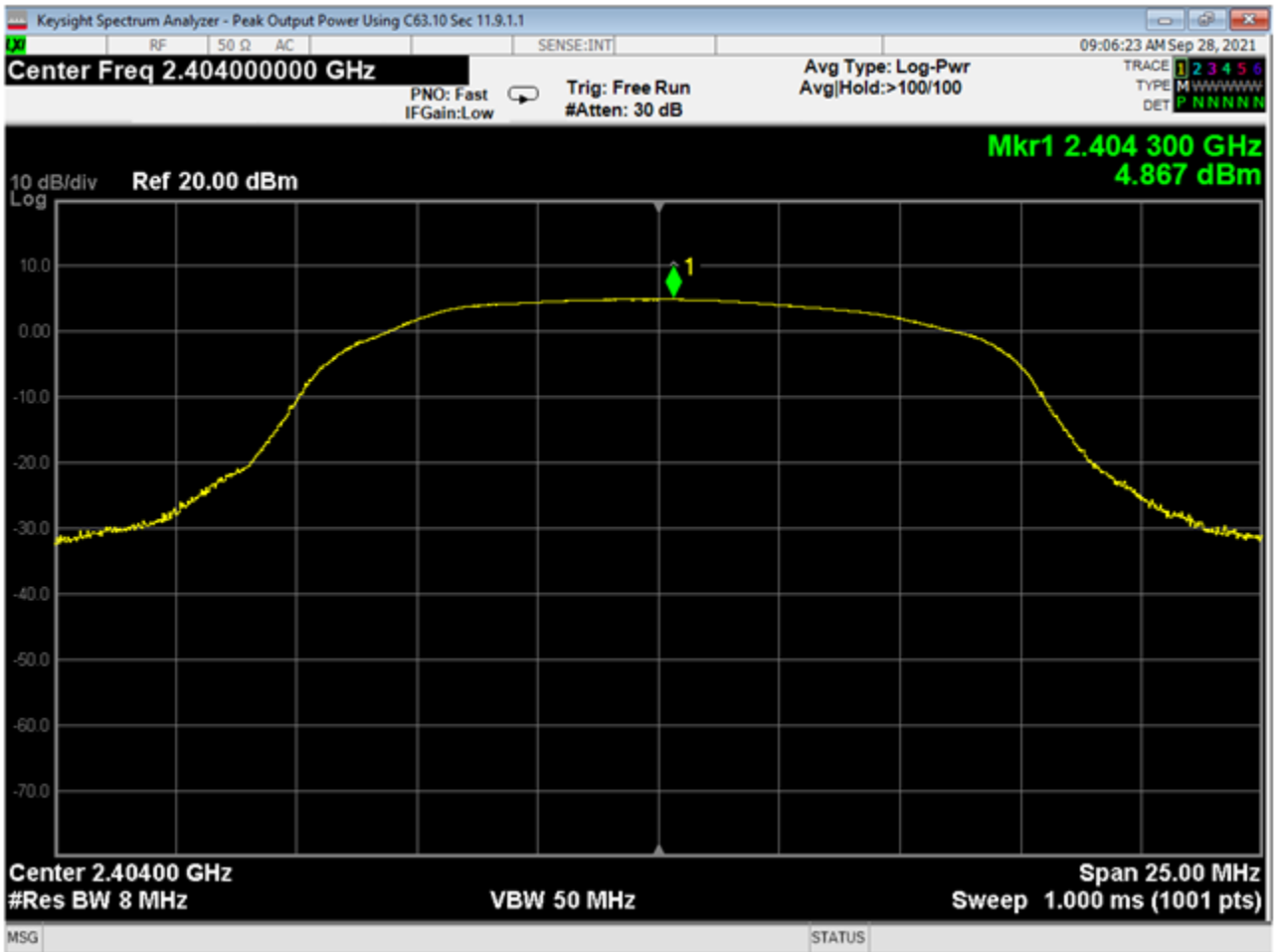
27 Peak Power, Low Channel, GMSK 2MB
