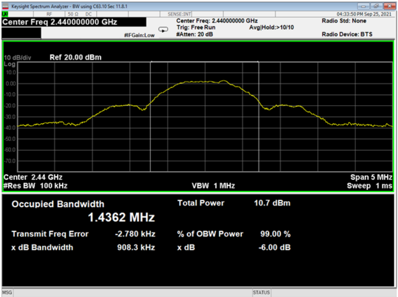
18 Bandwidth, Mid Channel, GMSK 1MB
