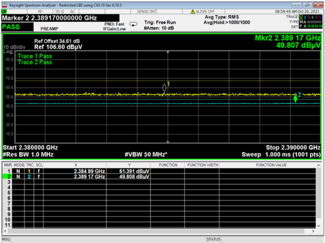
38 Lower Bandedge, Restricted, GMSK 2MB
