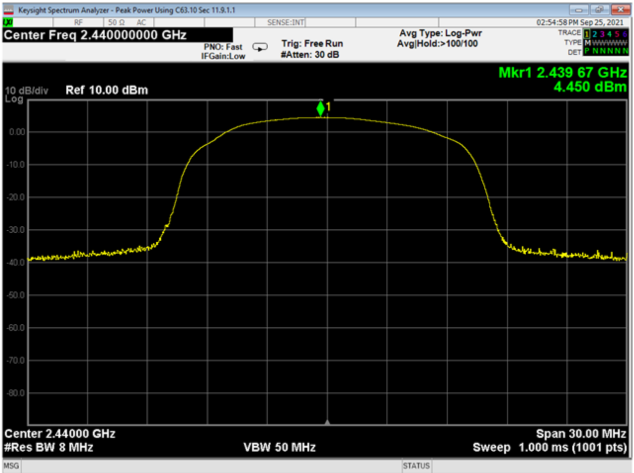
02 Peak Power, Mid Channel, GFSK
