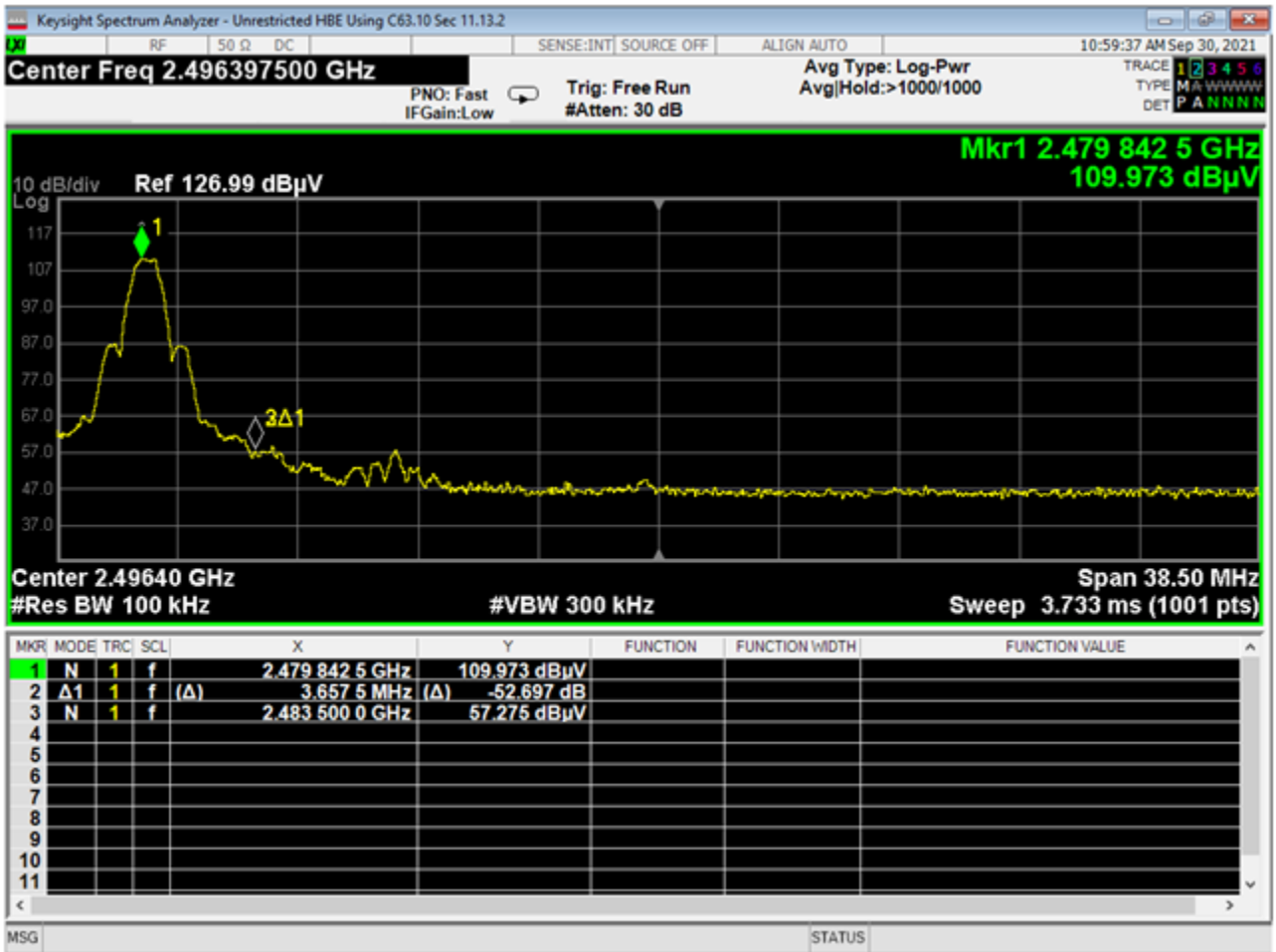
24 HBE, unrestricted GMSK 1MB
