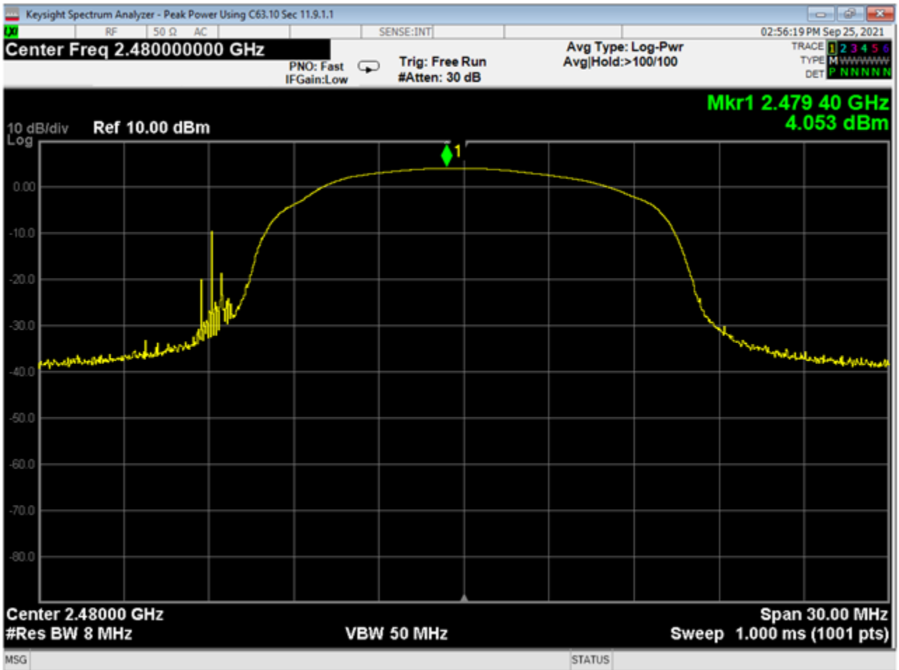
03 Peak Power, High Channel, GFSK
