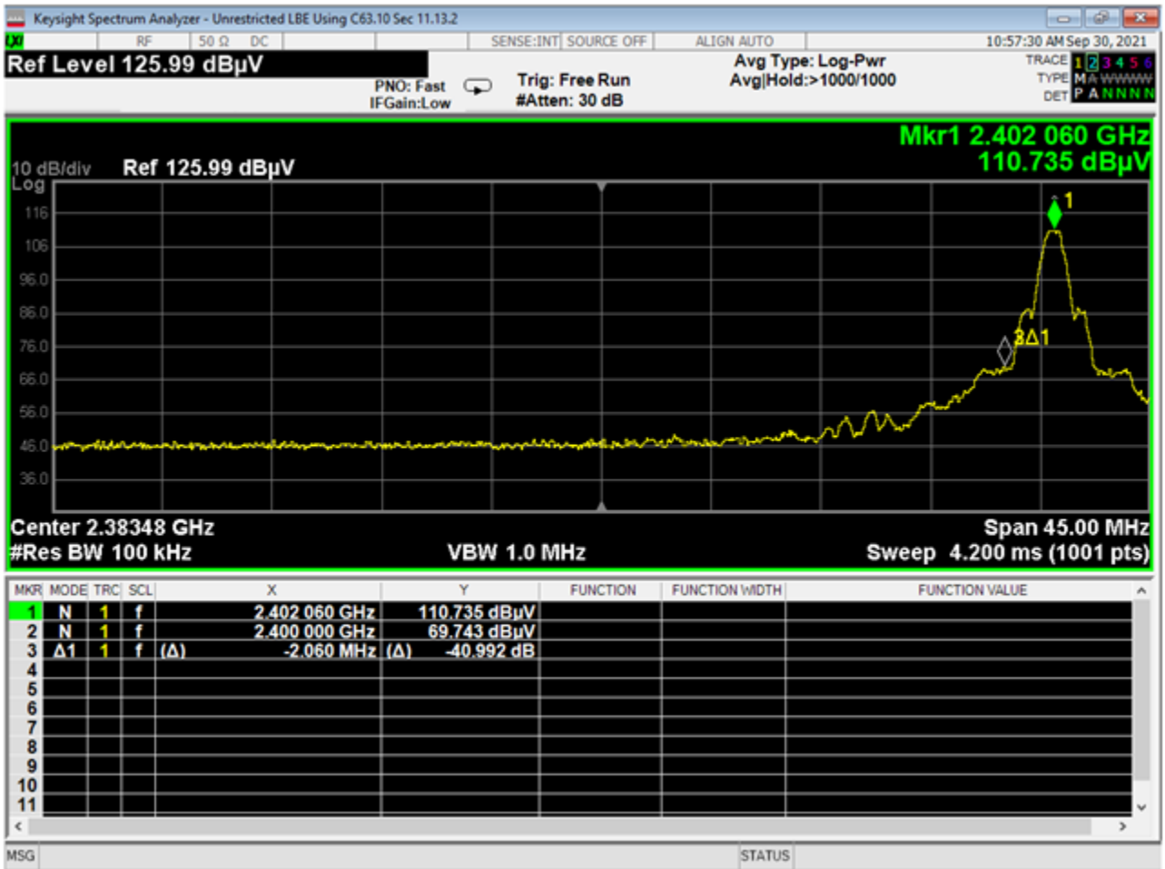
23 LBE, unrestricted GMSK 1MB
