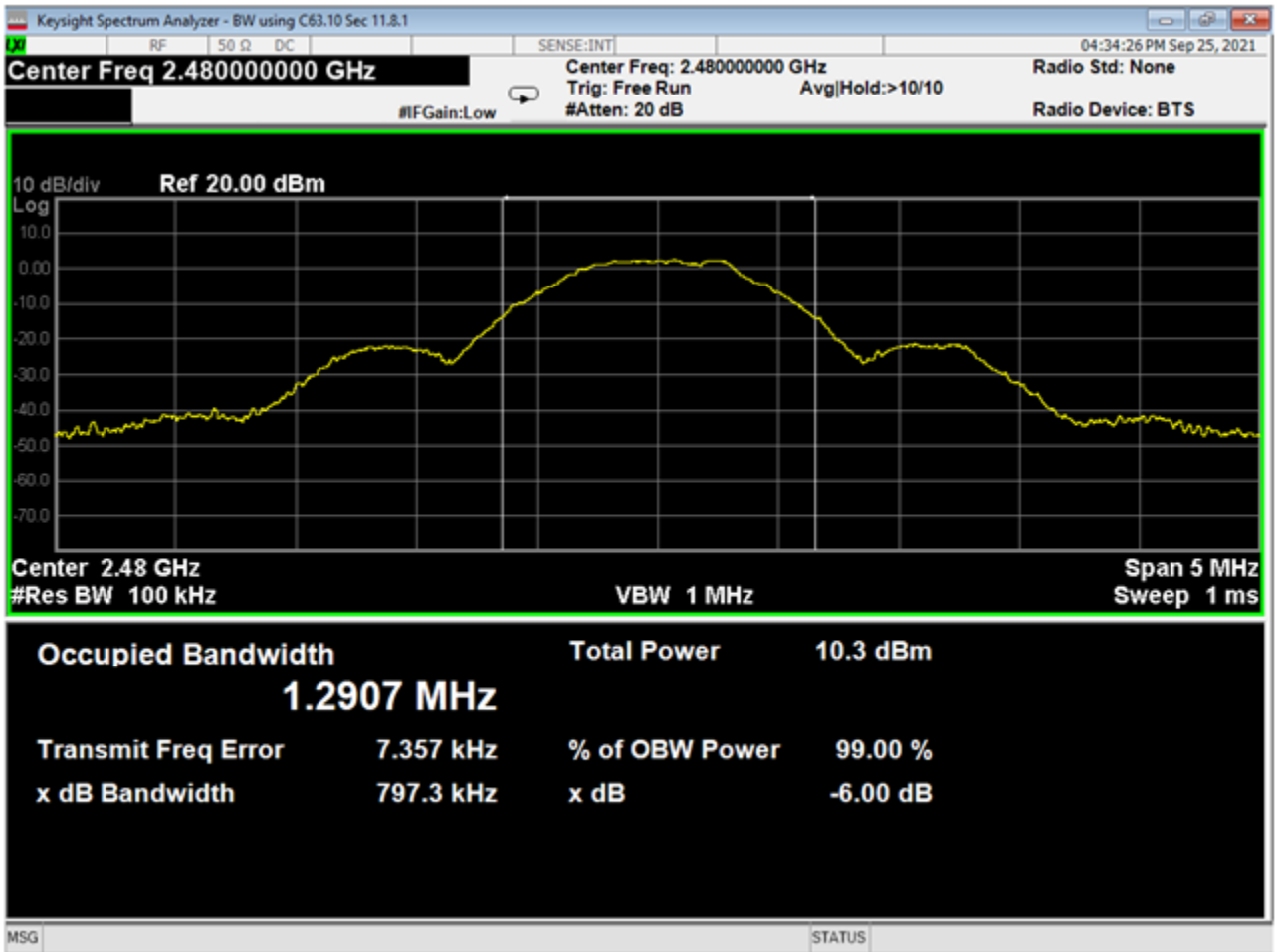
19 Bandwidth, High Channel, GMSK 1MB
