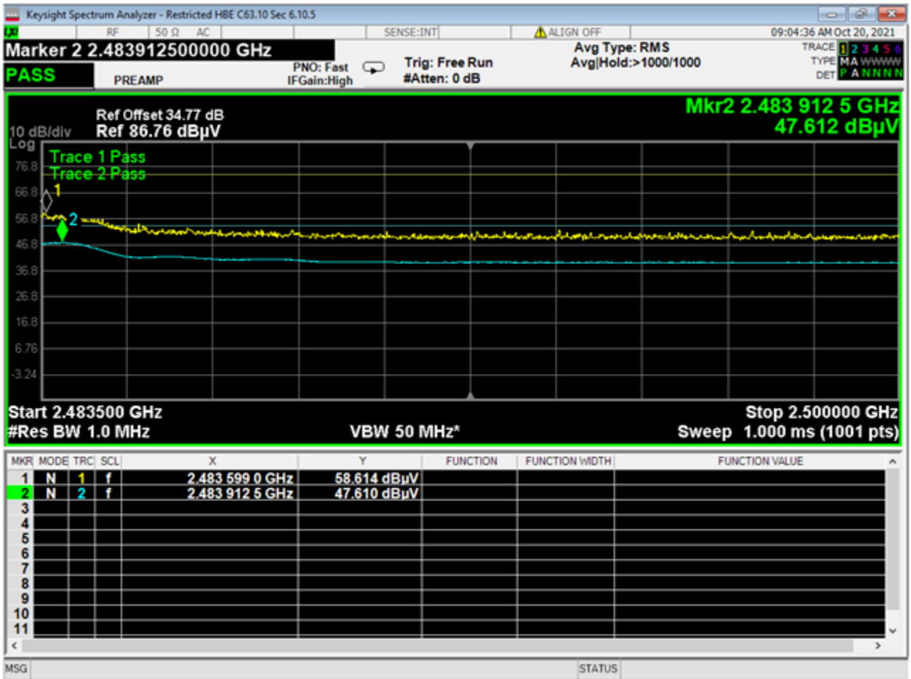
13 Higher Bandedge, Restricted, GFSK
