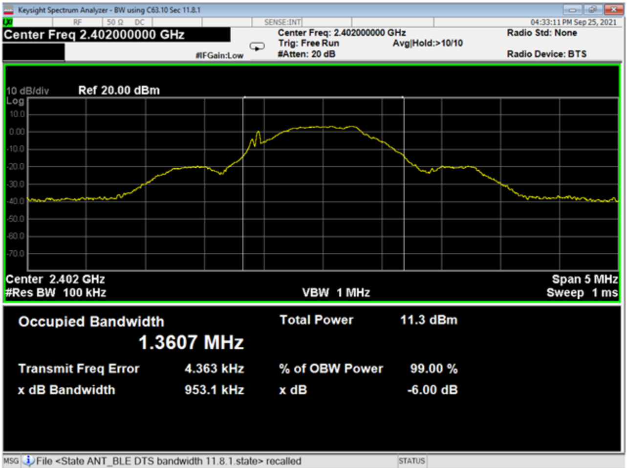
17 Bandwidth, Low Channel, GMSK 1MB
