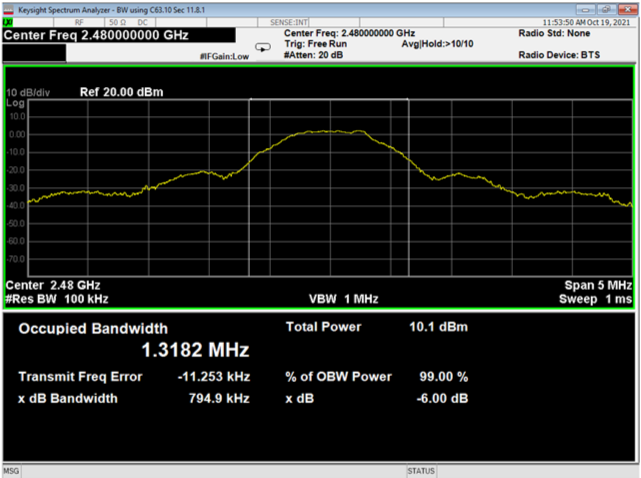
06 OBW-6dB, High Channel, GFSK
