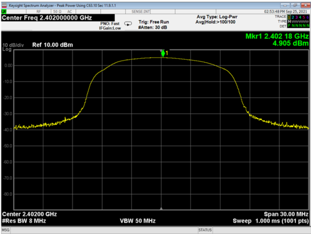
01 Peak Power, Low Channel, GFSK
