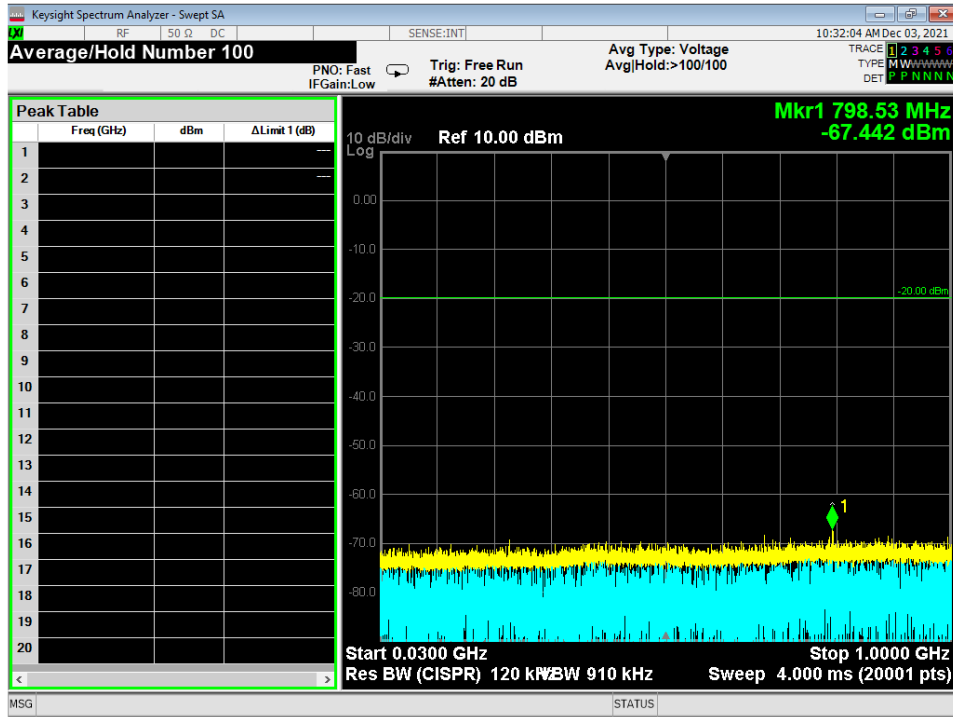
Figure 14 - Radiated Emissions Plot, GMSK 2MB, 30M – 1G, Low
