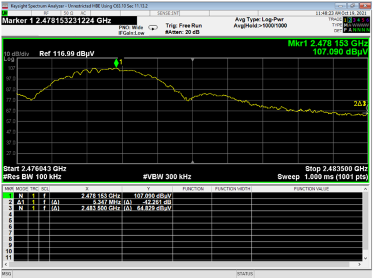
37 Higher Bandedge, Unrestricted, GMSK 2MB
