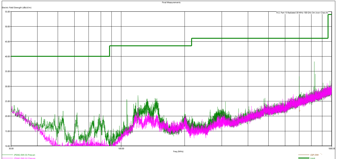
Figure 6 - Radiated Emissions Plot, GSK 1MB
