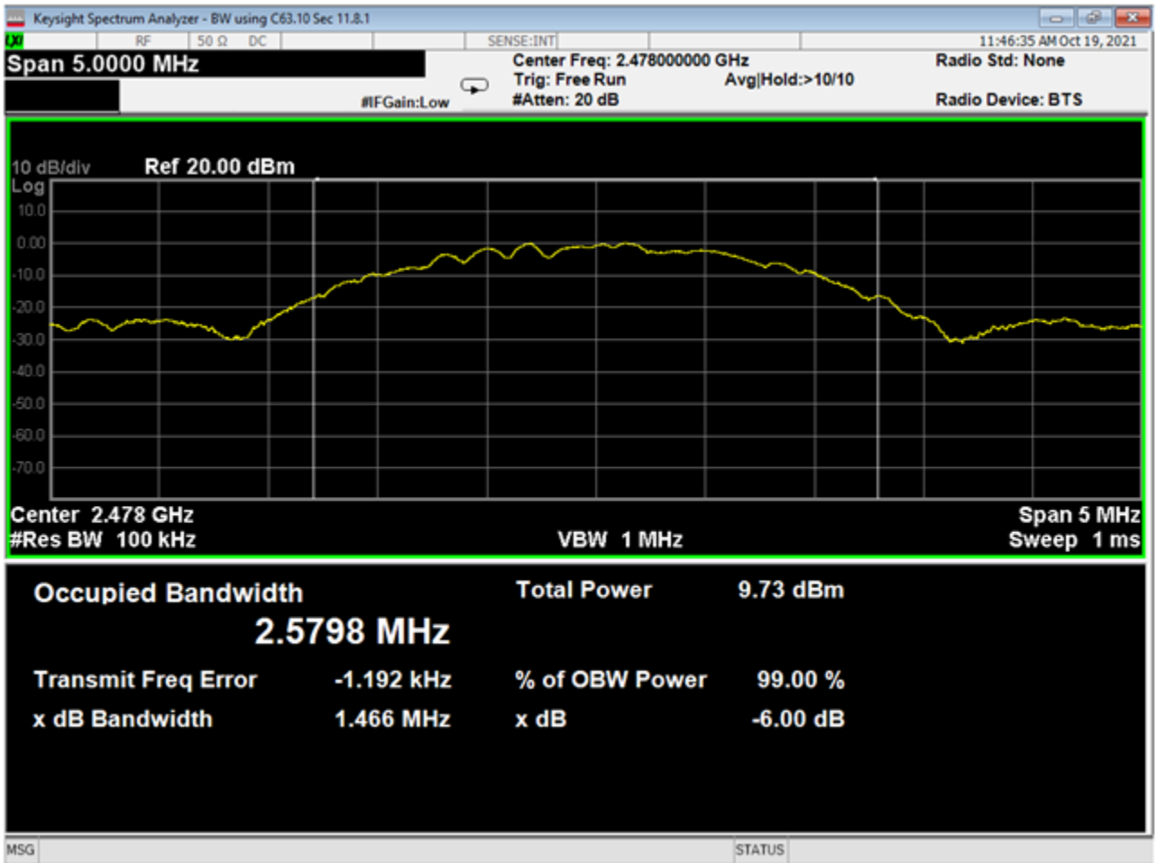
32 OBW-6dB, High Channel, GMSK 2MB
