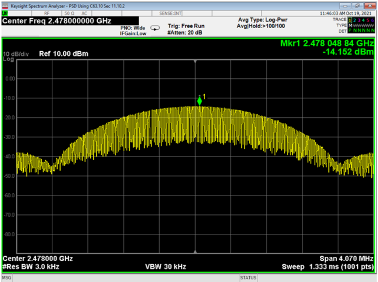
35 PSD, High Channel, GMSK 2MB
