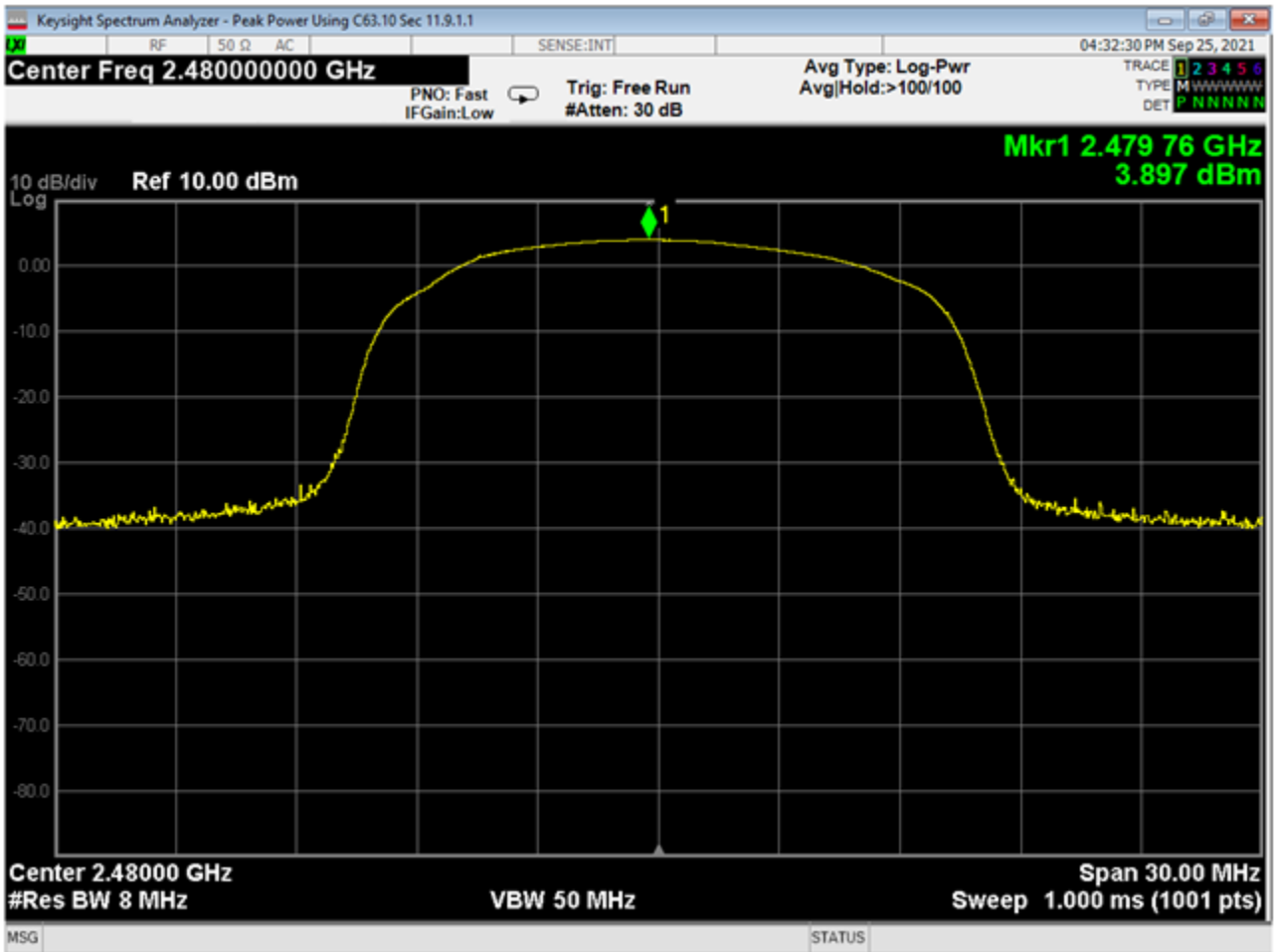
16 Peak Power, High Channel, GMSK 1MB
