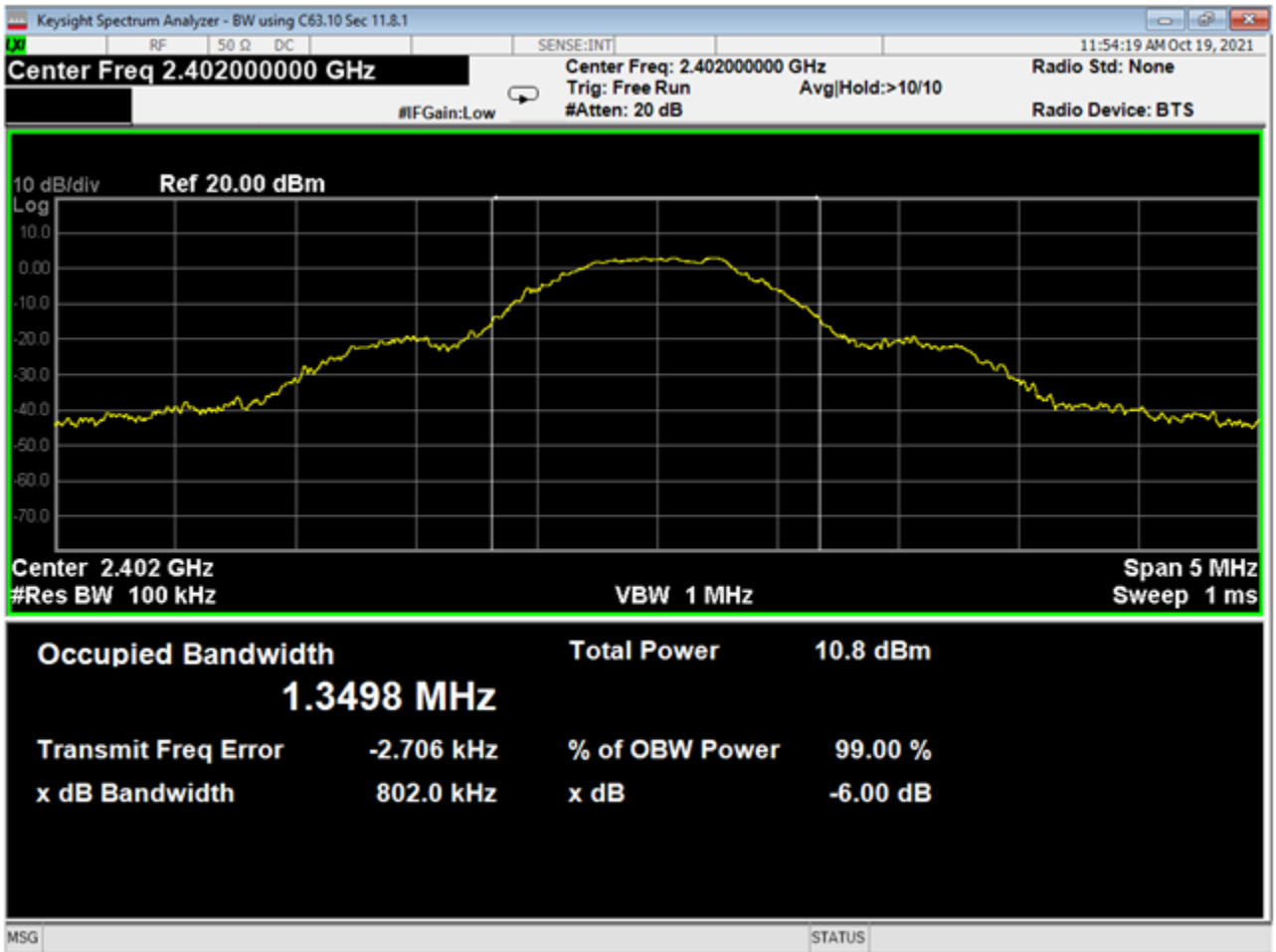
04 OBW-6dB, Low Channel, GFSK
