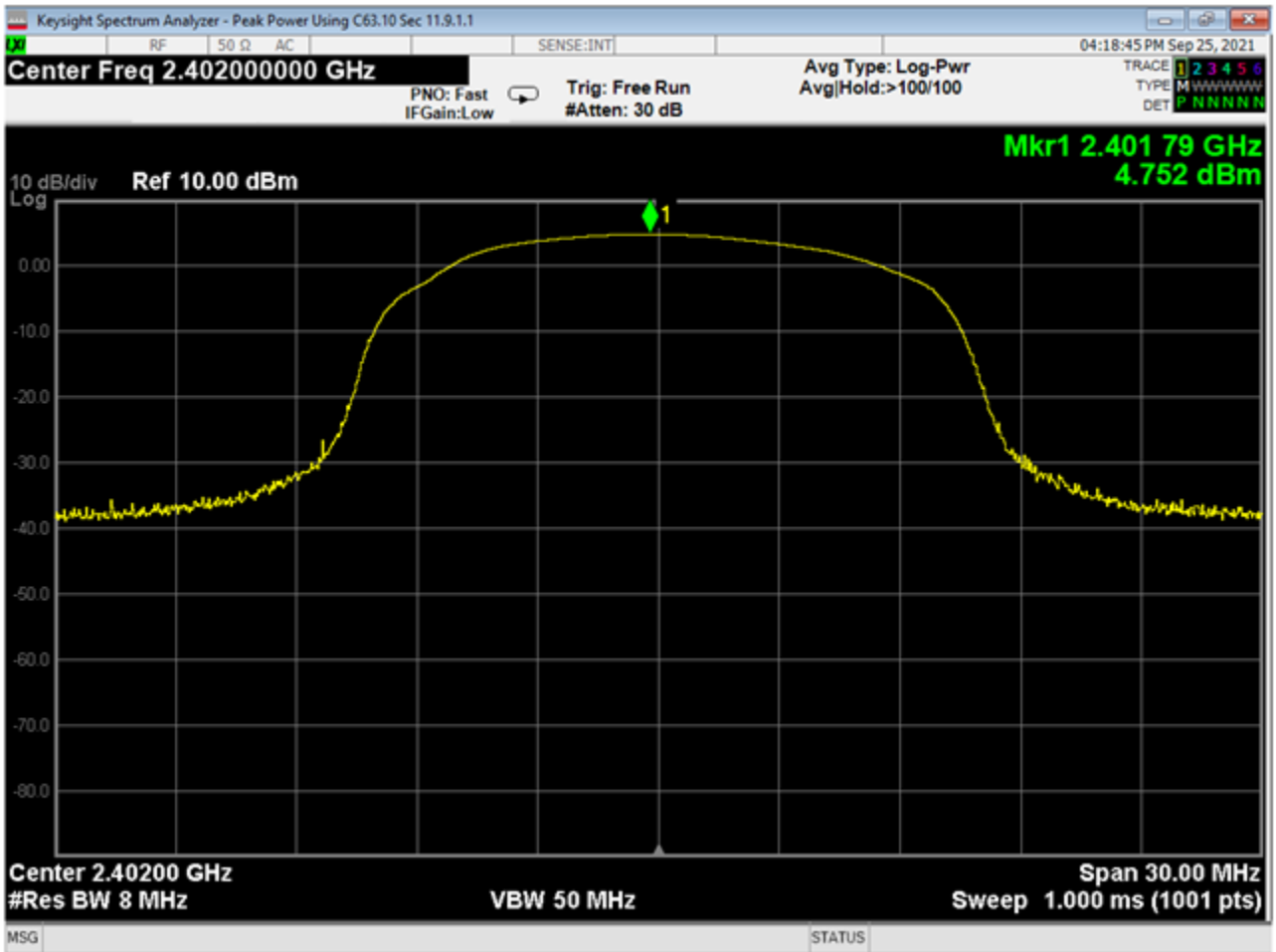
14 Peak Power, Low Channel, GMSK 1MB
