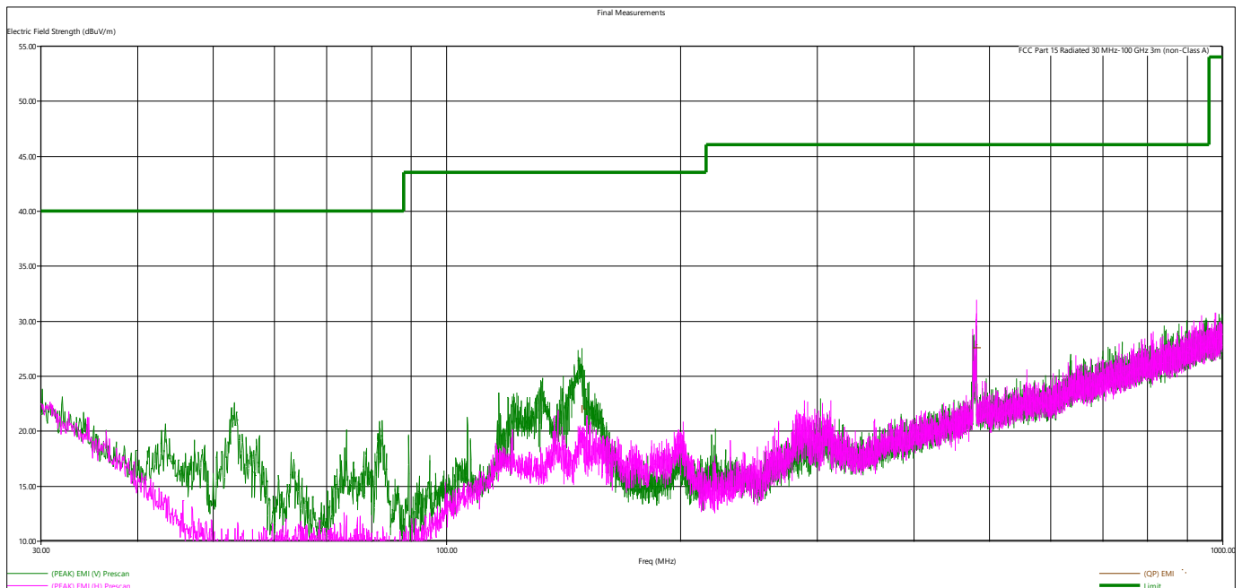
Figure 7 - Radiated Emissions Plot, GSK 2MB
