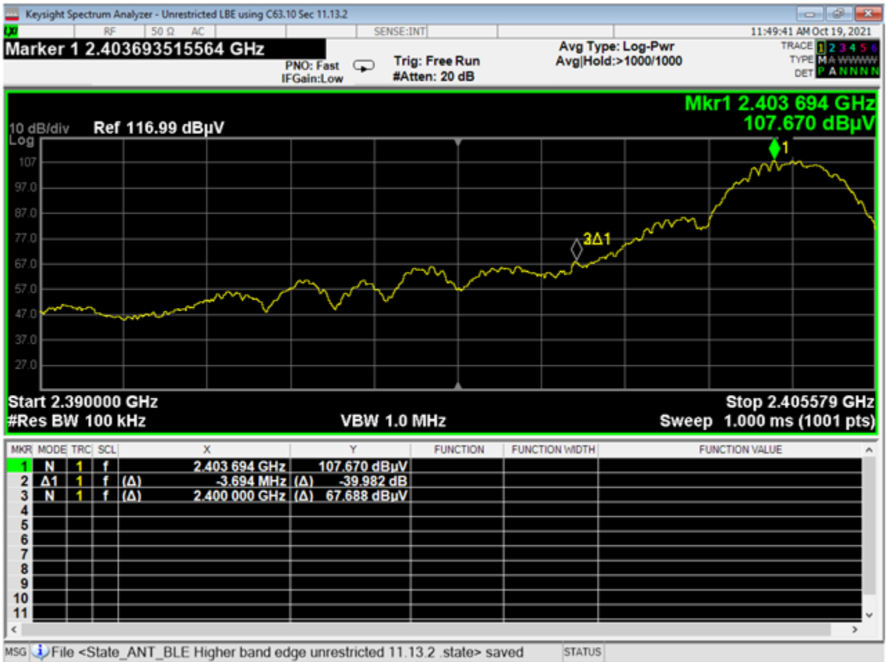
36 Lower Bandedge, Unrestricted, GMSK 2MB
