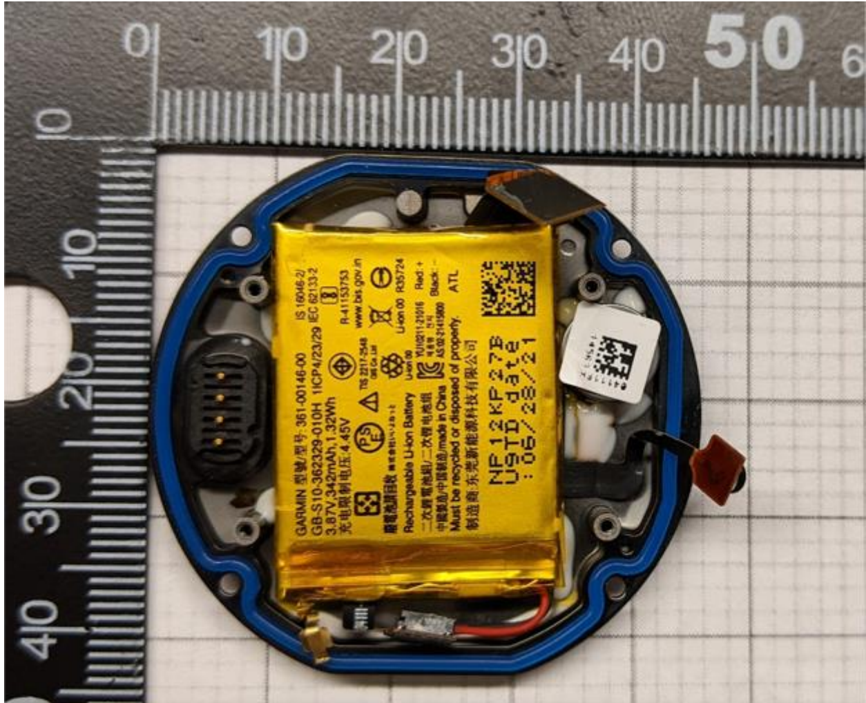
Inside of rear case
