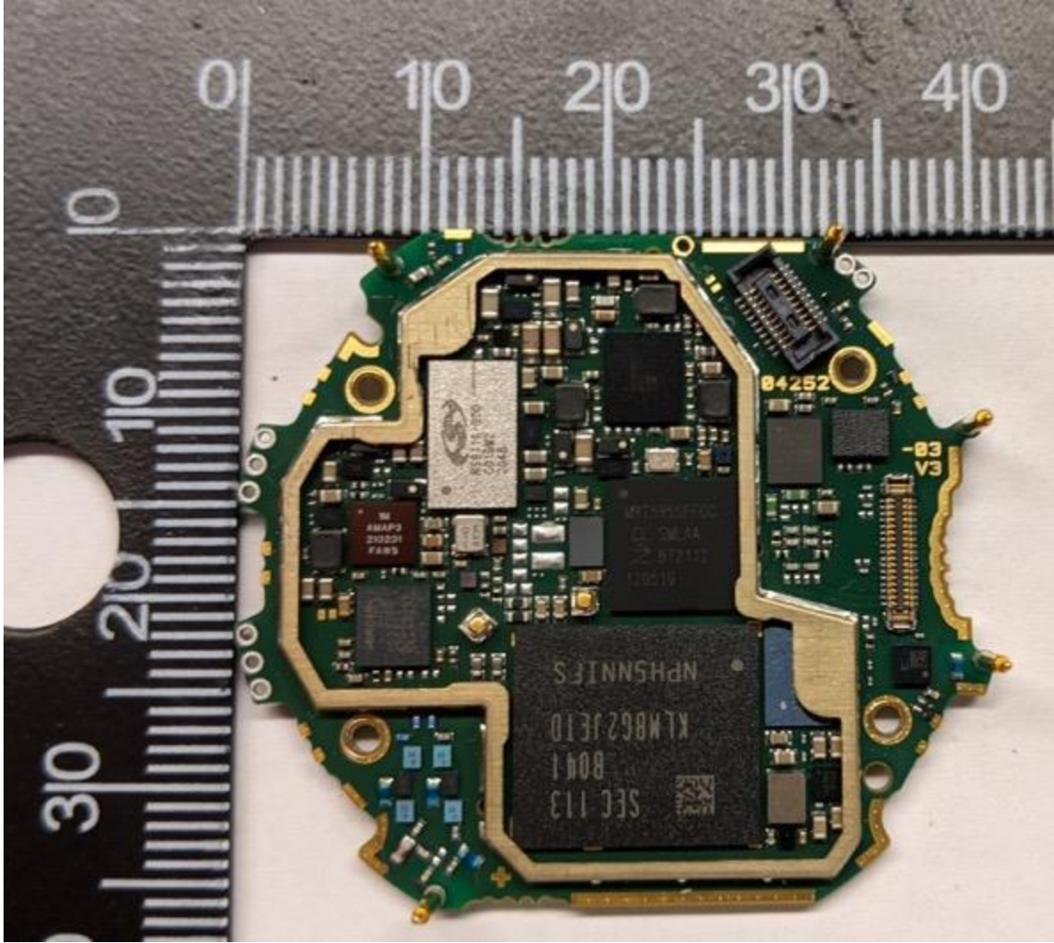
Front face of main PCB
