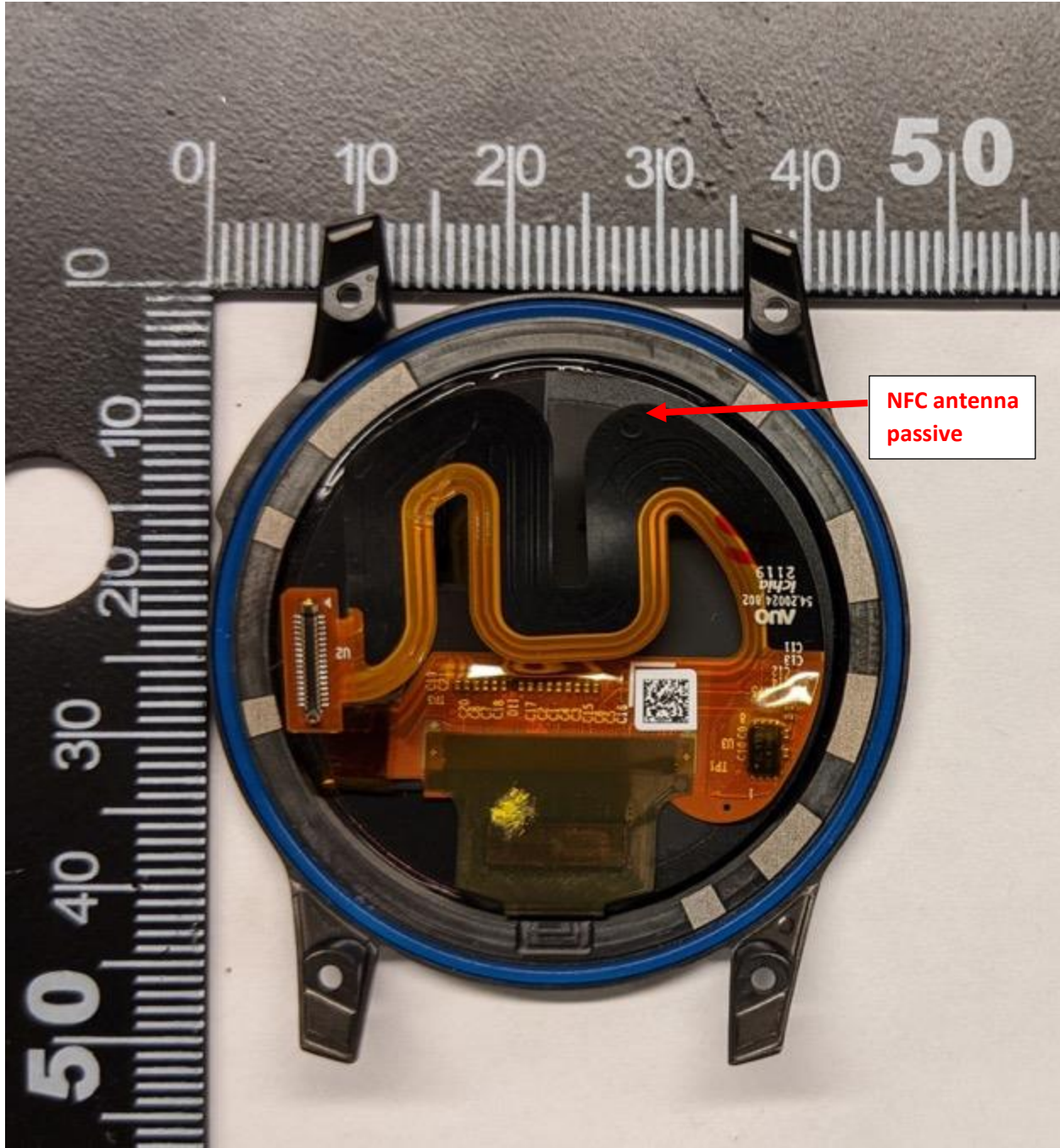
Inside of display
