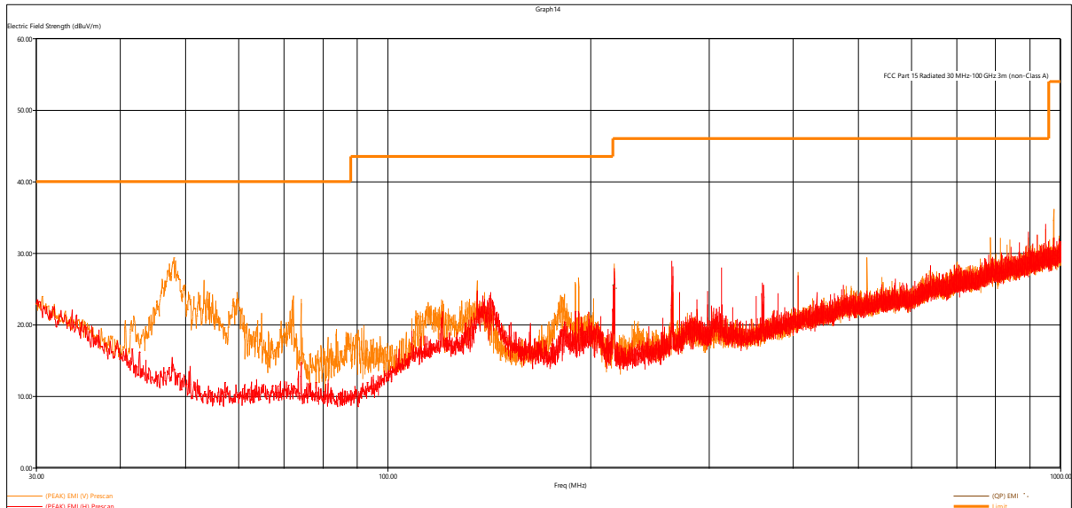
Figure 2 – NFC Radiated Emissions Plot, 30MHz – 1GHz All emissions found to be at least 6dB below limit line
