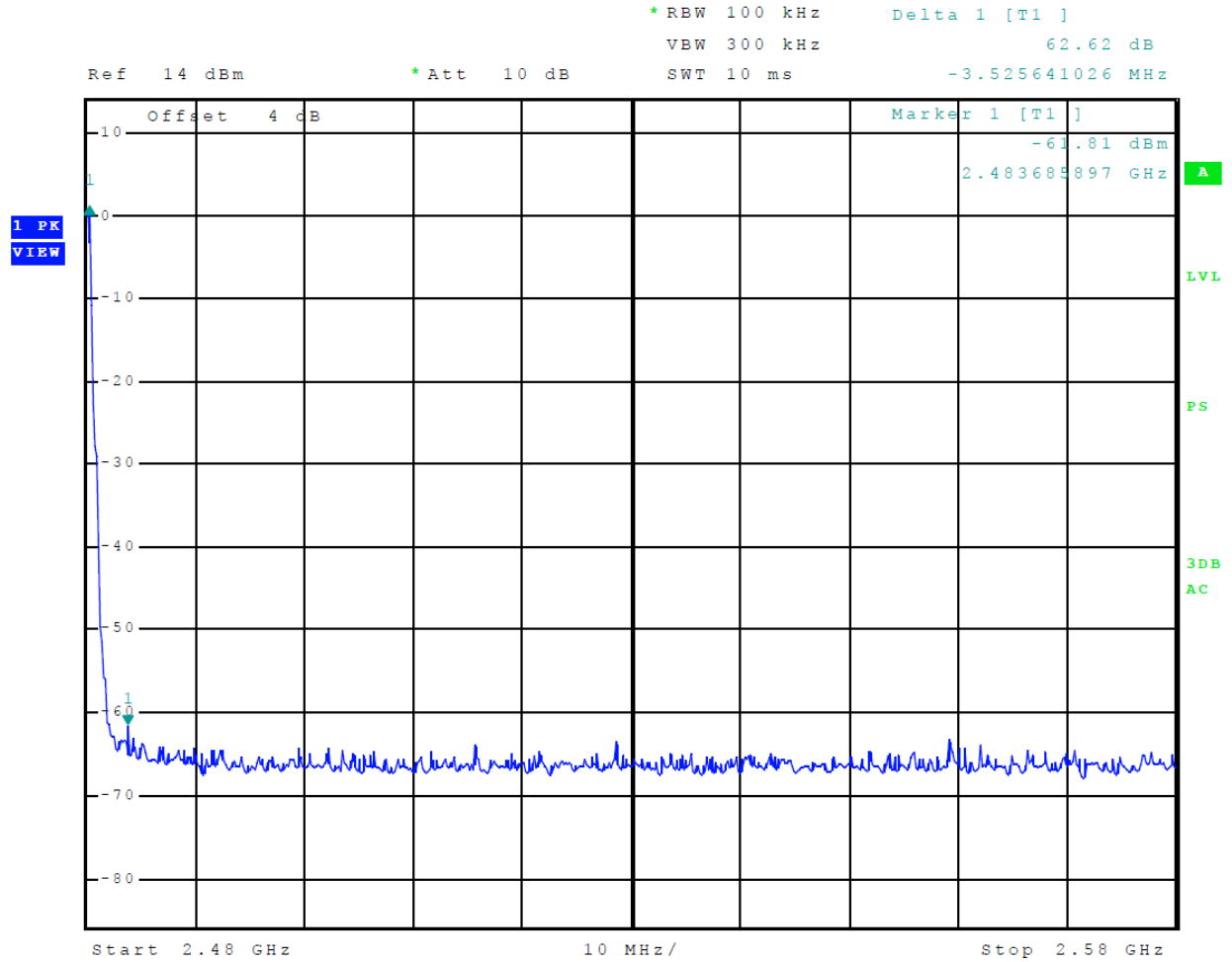
Figure 11 Plot of Transmitter Emissions High Band Edge Mode 4 BLE
