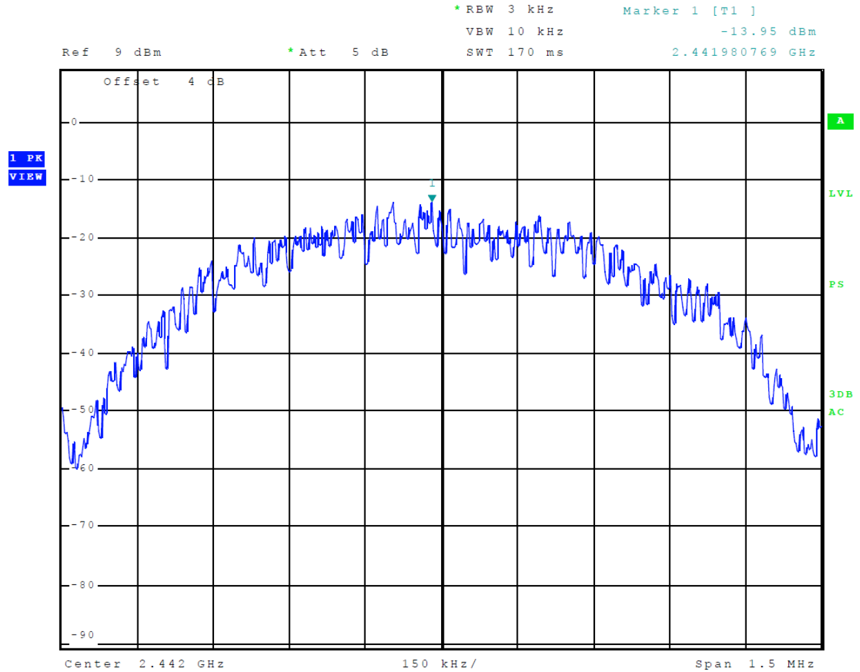
Figure 23 Plot of Transmitter Power Spectral Density Mode 4 BLE
