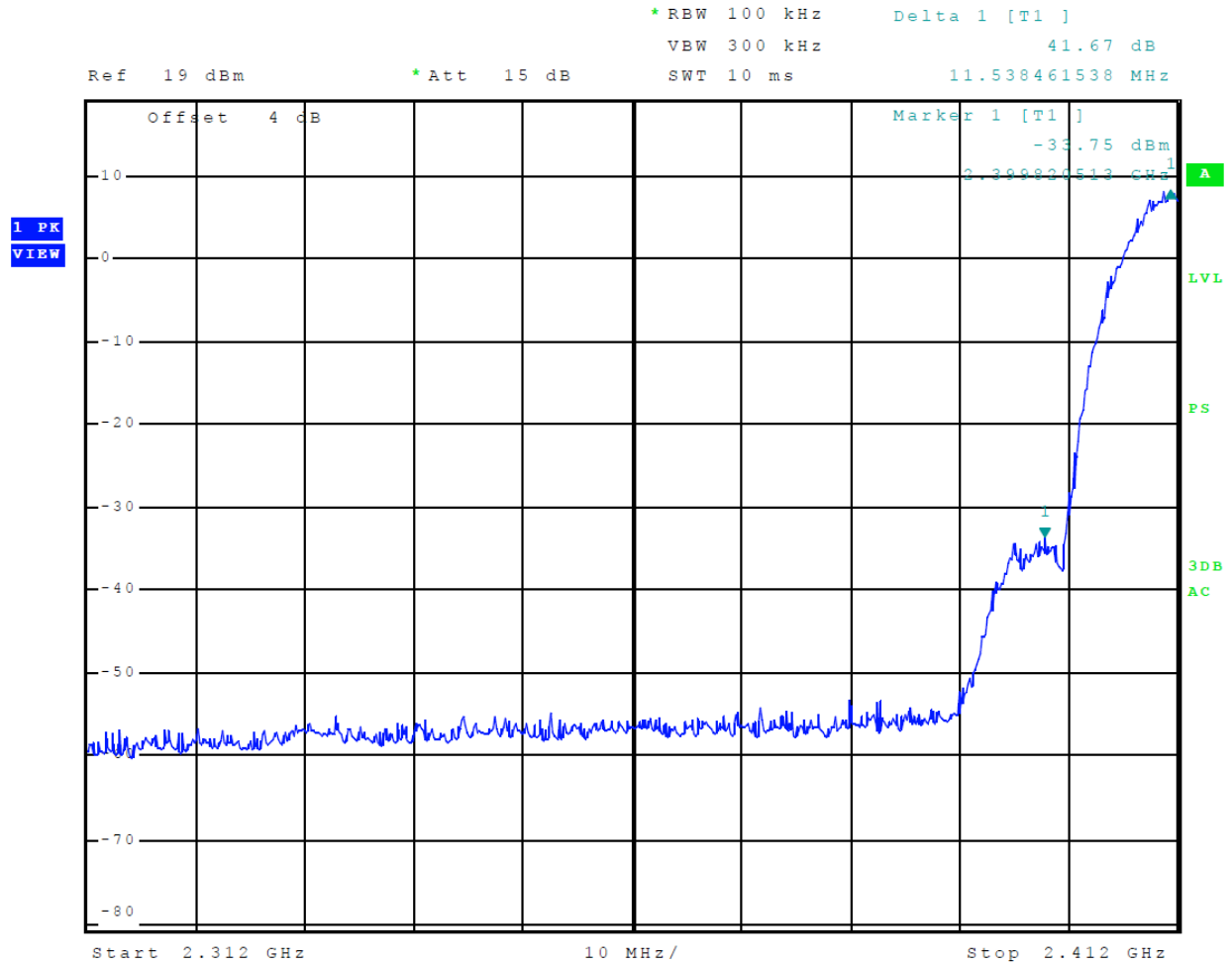
Figure 8 Plot of Transmitter Emissions Low Band Edge Mode 5 802.11b
