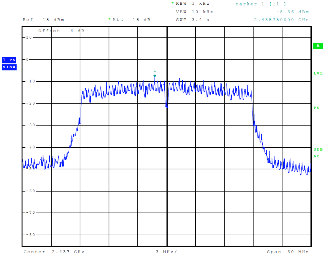
Figure 26 Plot of Transmitter Power Spectral Density Mode 7 802.11n
