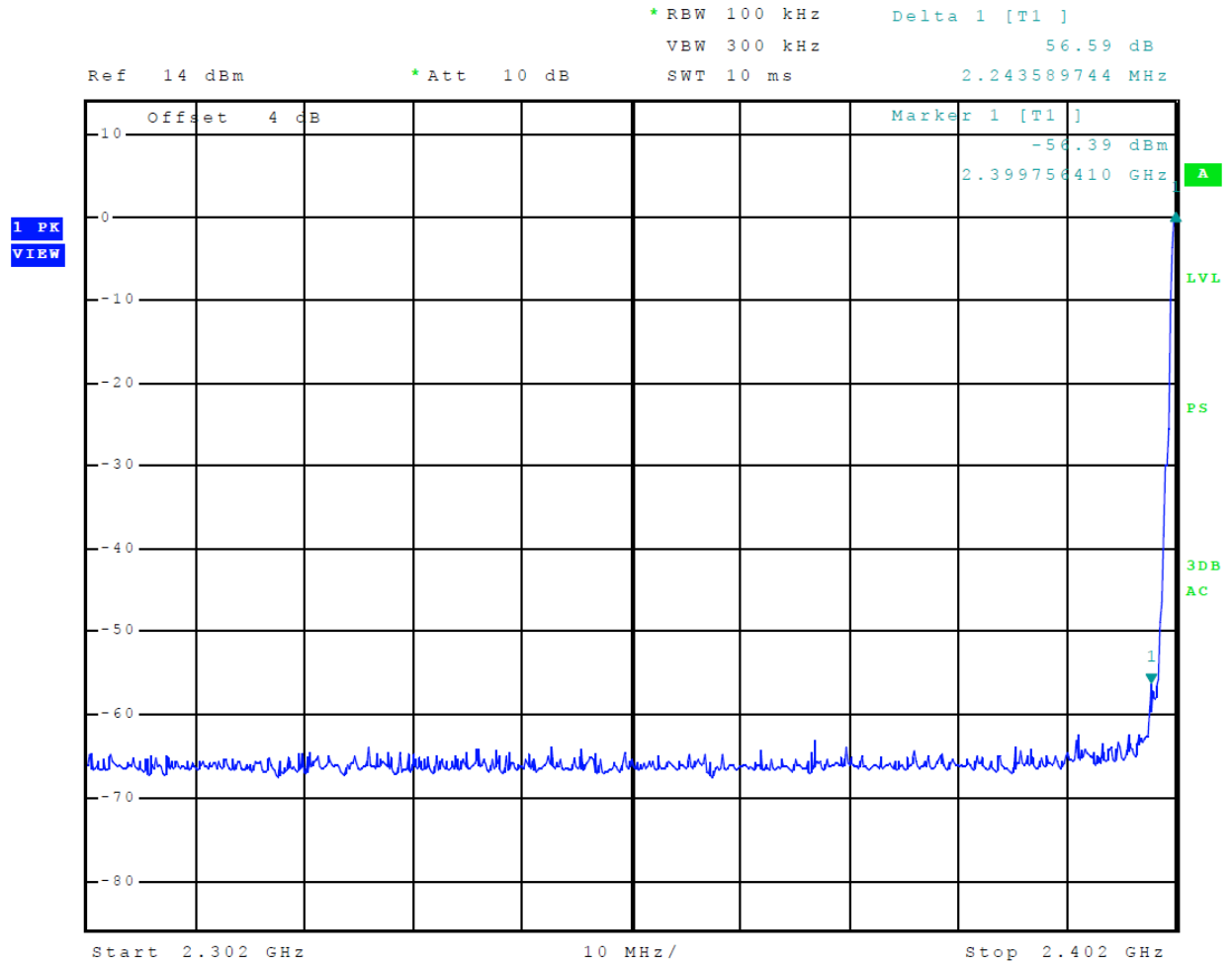
Figure 7 Plot of Transmitter Emissions Low Band Edge Mode 4 BLE
