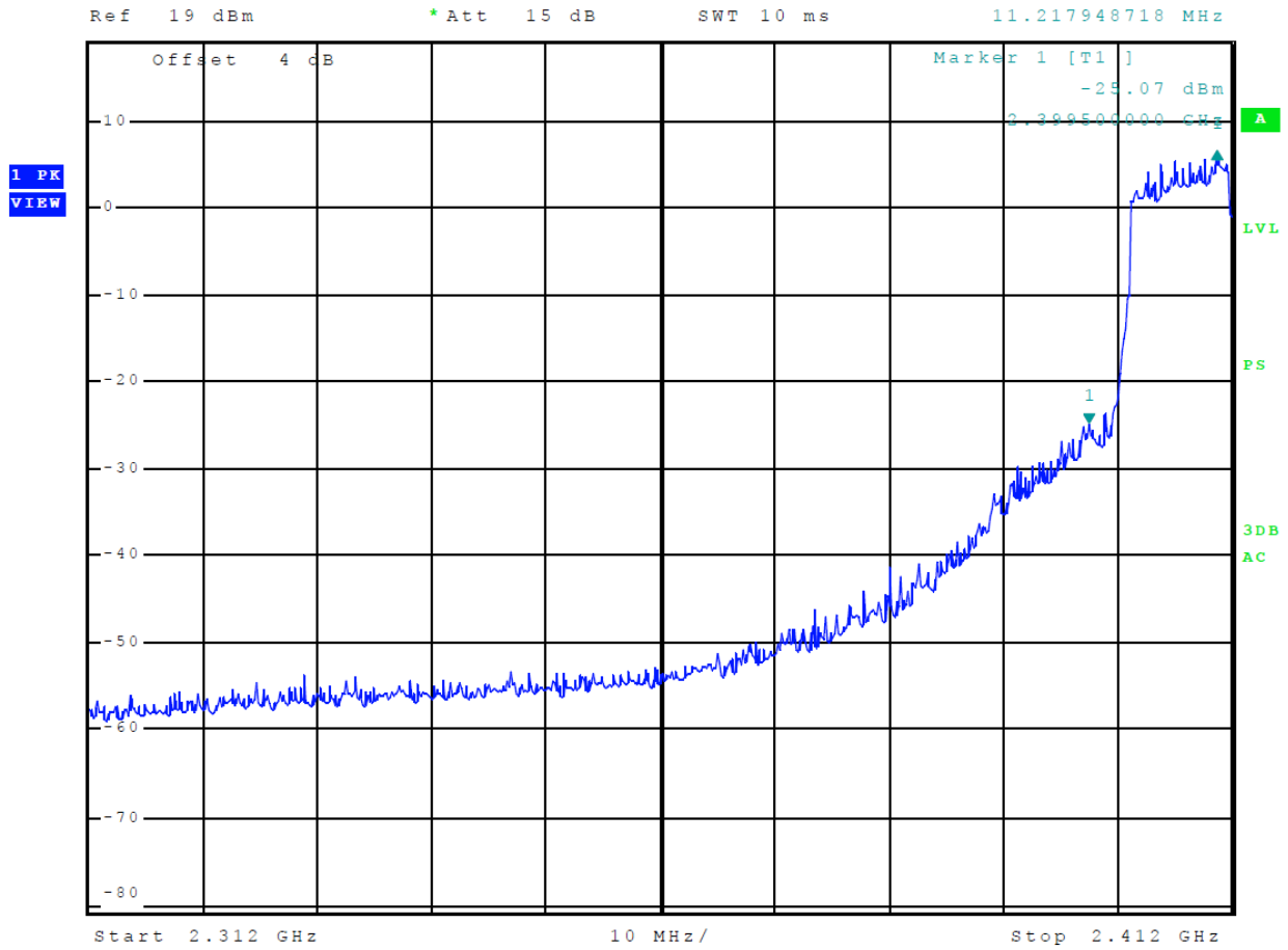
Figure 10 Plot of Transmitter Emissions Low Band Edge Mode 7 802.11n
