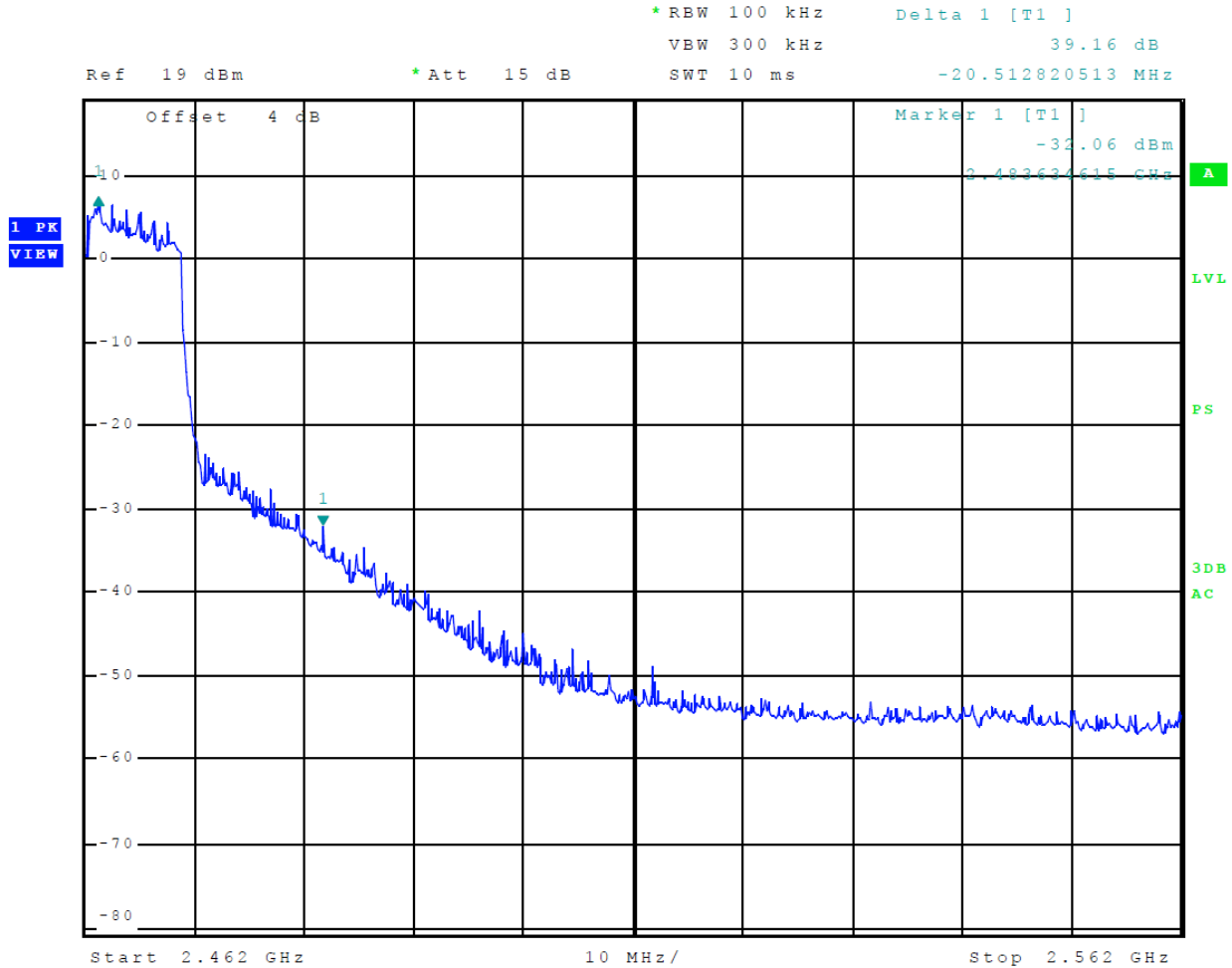
Figure 14 Plot of Transmitter Emissions High Band Edge Mode 7 802.11n
