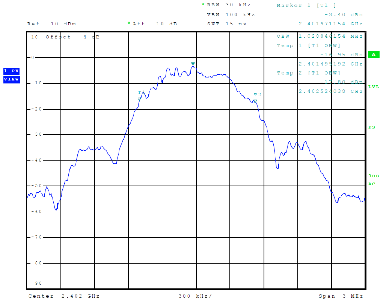
Figure 16 Plot of 99% Occupied Bandwidth Mode 4 BLE
