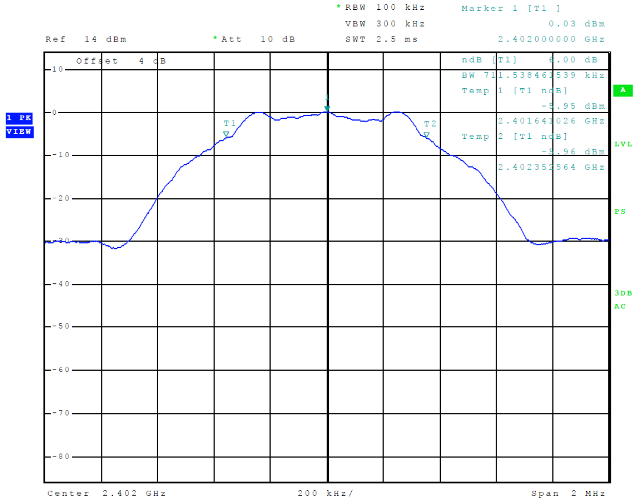
Figure 15 Plot of 6-dB Occupied Bandwidth Mode 4 BLE
