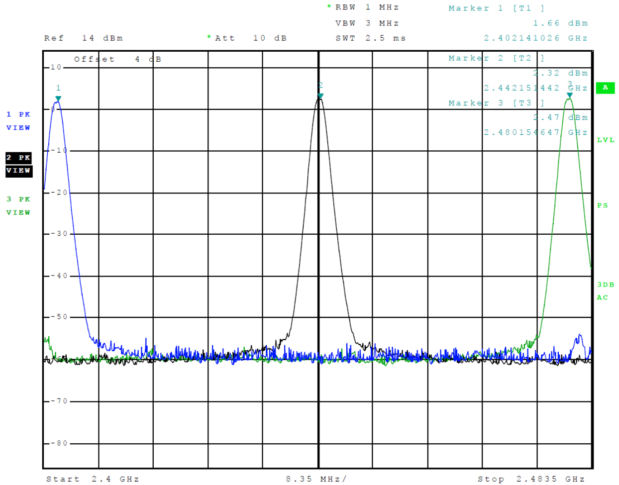
Figure 3 Plot of Transmitter Operation in 2402-2480 MHz Mode 4 BLE
