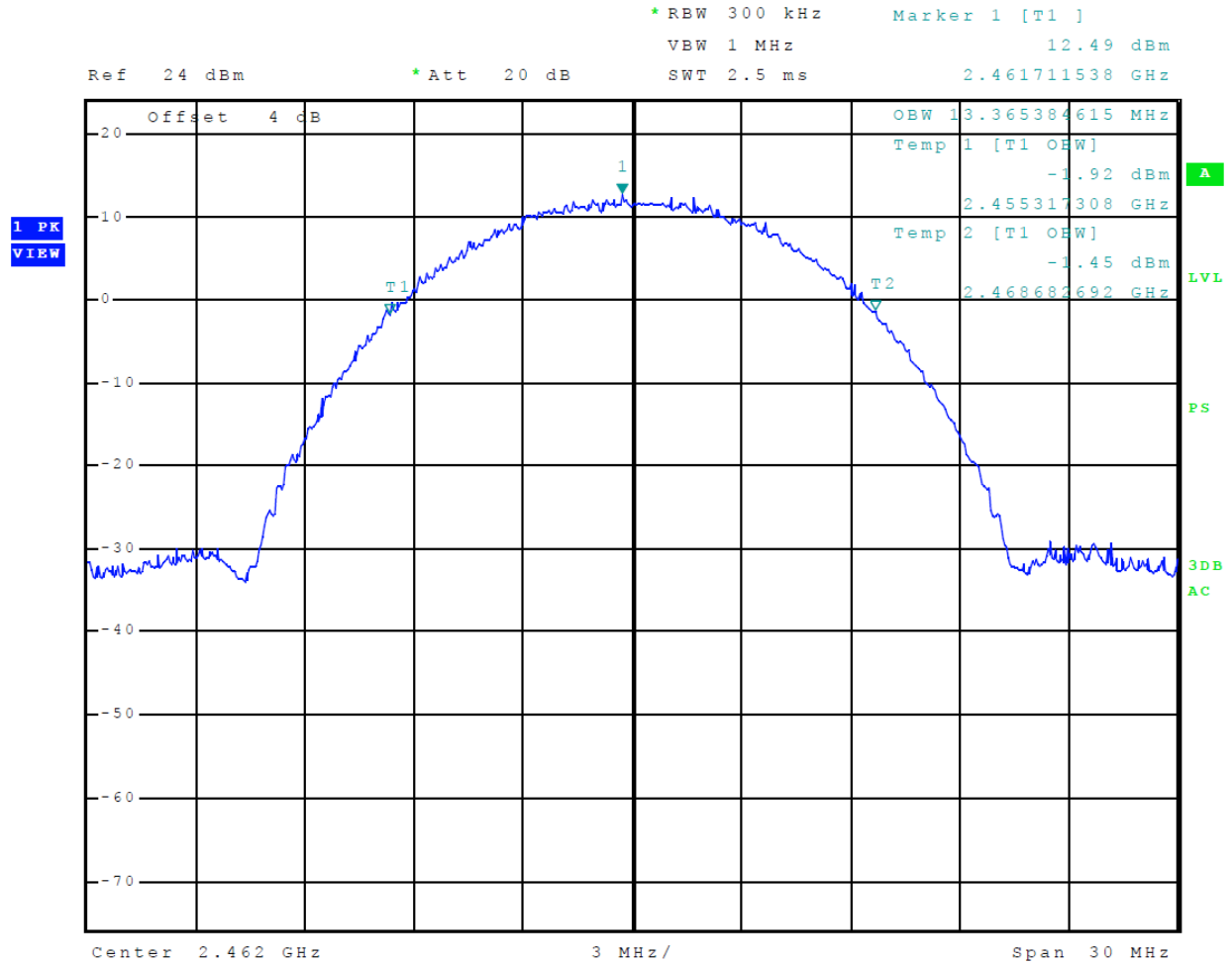
Figure 18 Plot of 99% Occupied Bandwidth Mode 5 802.11b
