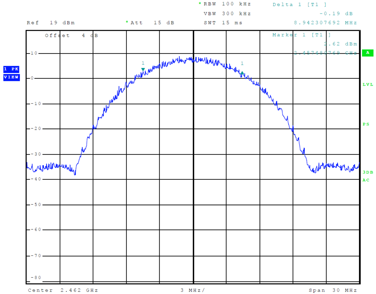
Figure 17 Plot of 6-dB Occupied Bandwidth Mode 5 802.11b
