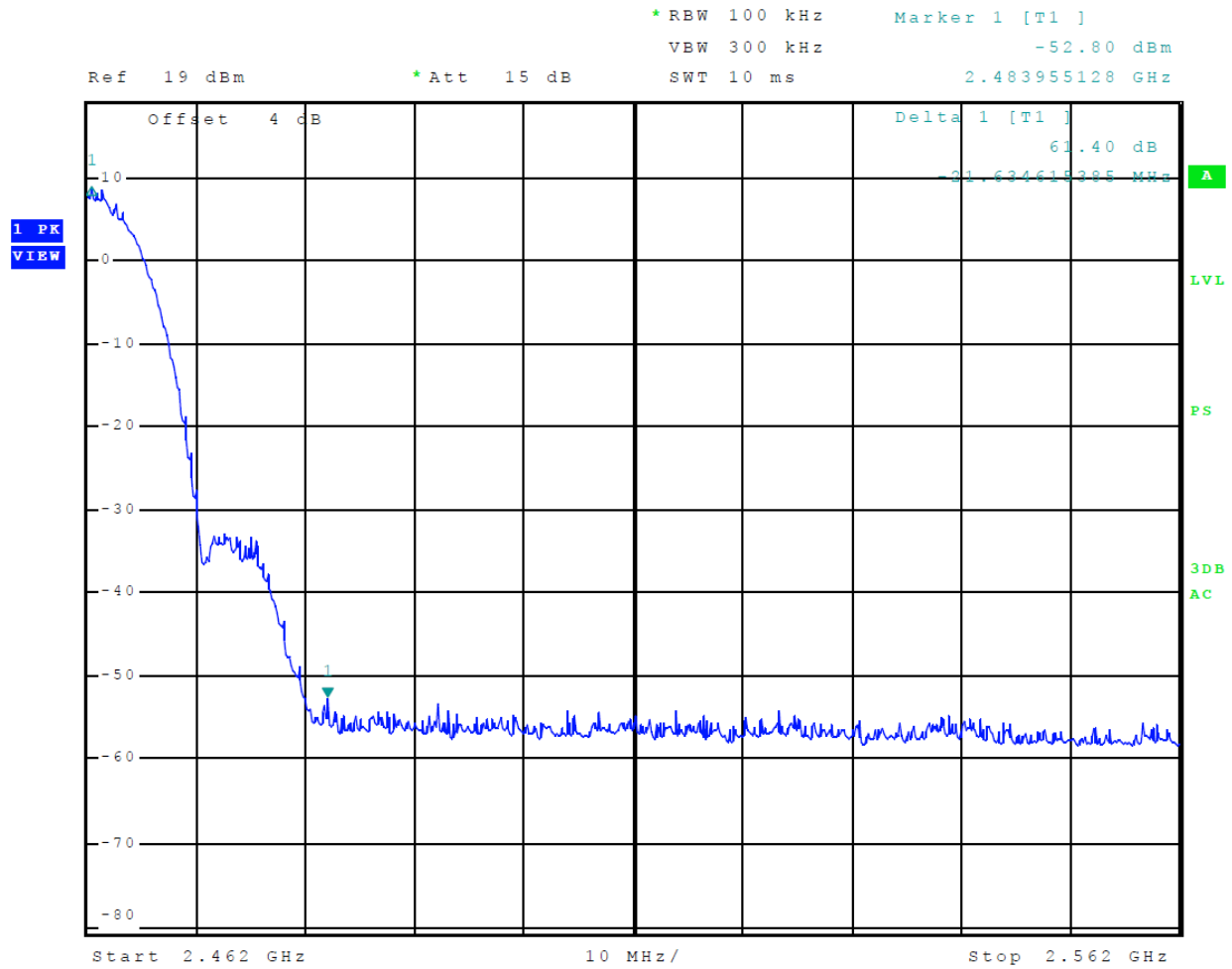
Figure 12 Plot of Transmitter Emissions High Band Edge Mode 5 802.11b
