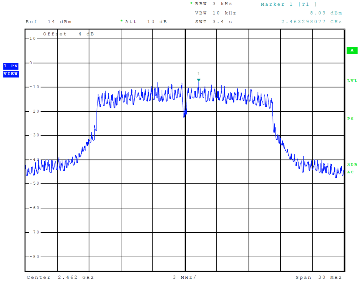
Figure 25 Plot of Transmitter Power Spectral Density Mode 6 802.11g
