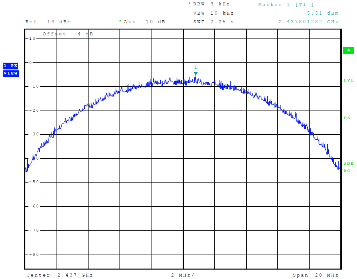
Figure 24 Plot of Transmitter Power Spectral Density Mode 5 802.11b
