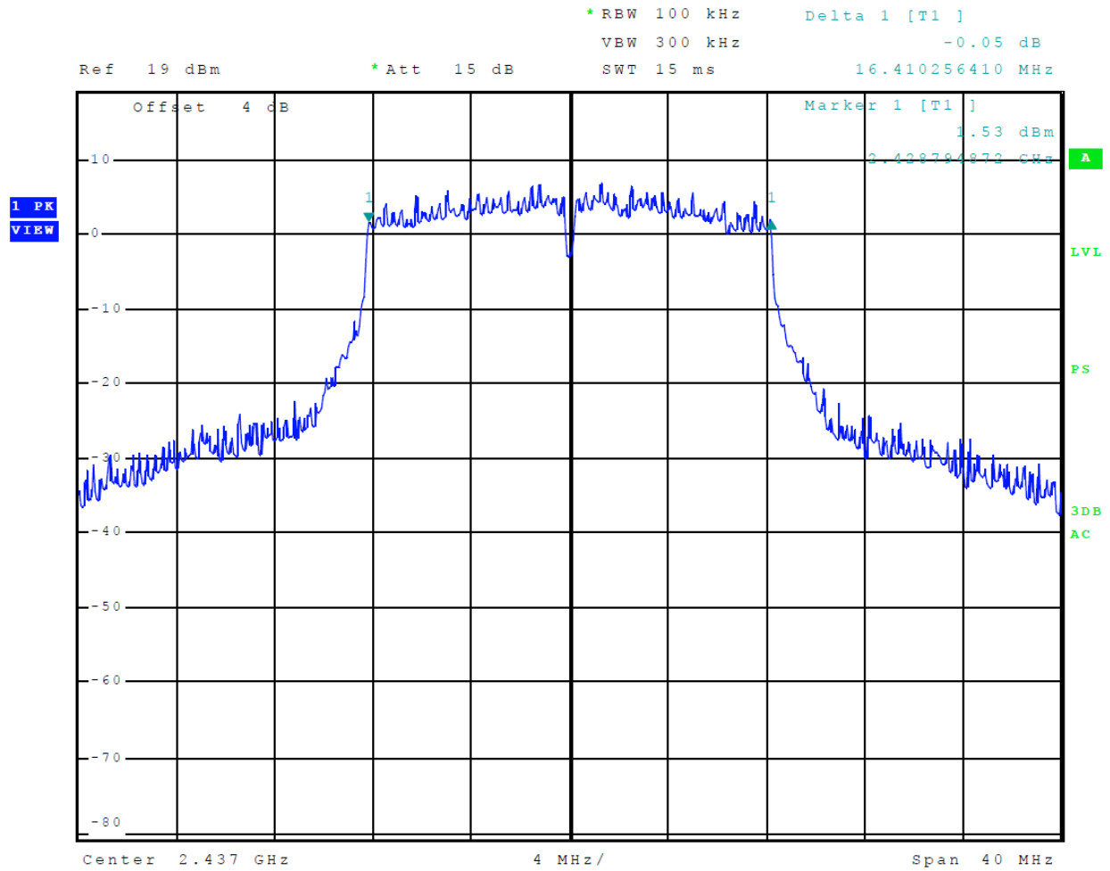
Figure 19 Plot of 6-dB Occupied Bandwidth Mode 6 802.11g
