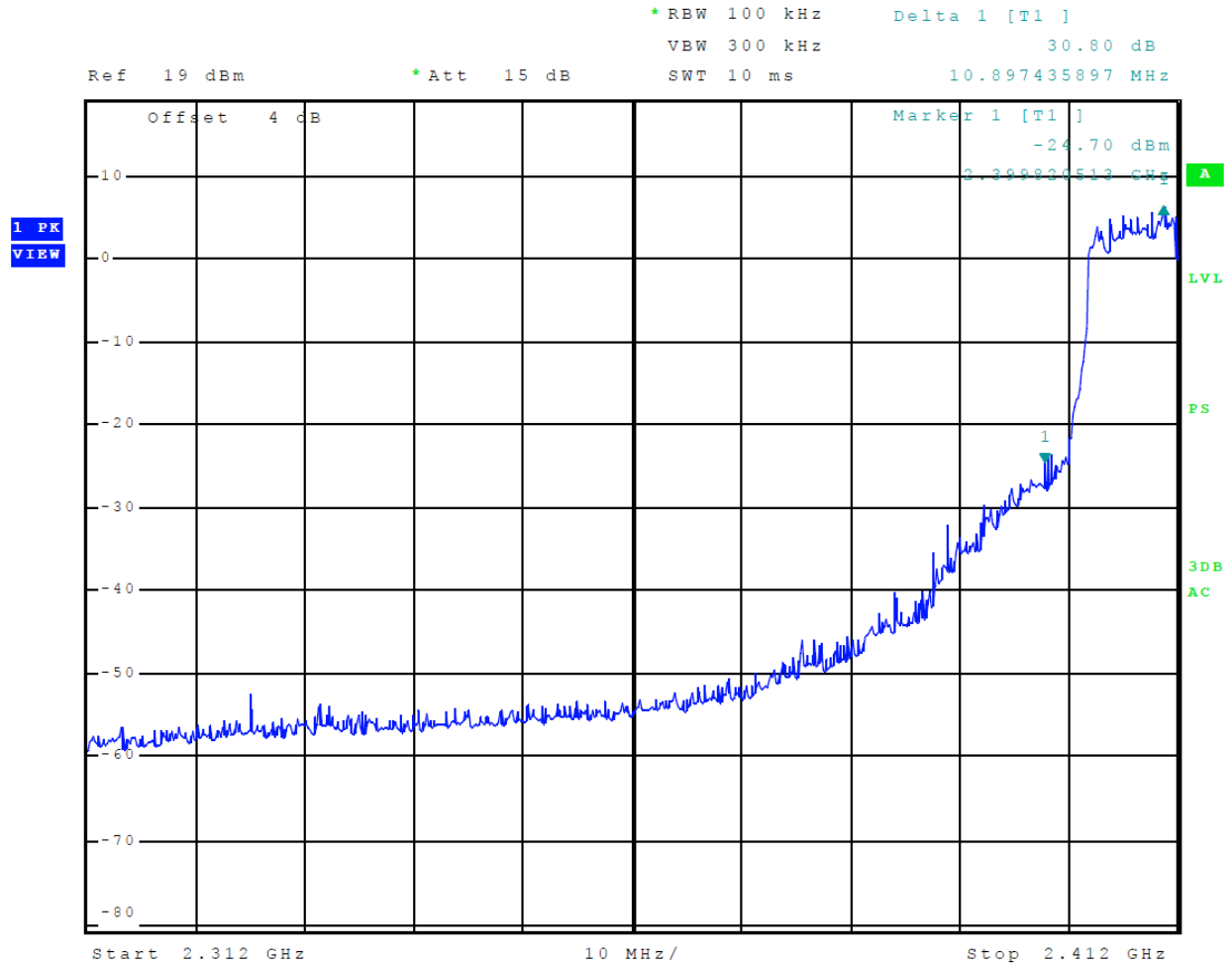
Figure 9 Plot of Transmitter Emissions Low Band Edge Mode 6 802.11g
