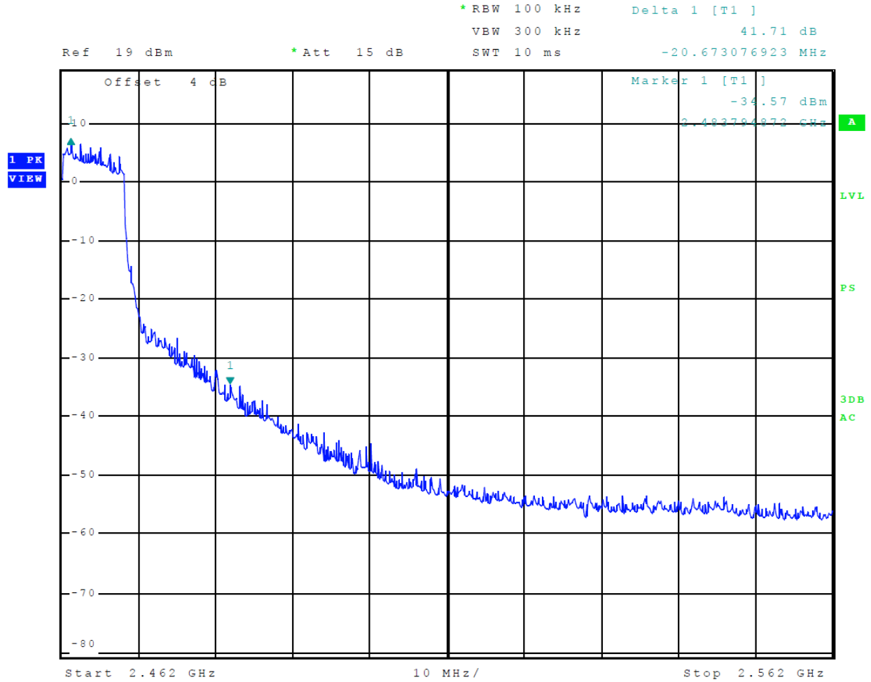
Figure 13 Plot of Transmitter Emissions High Band Edge Mode 6 802.11g
