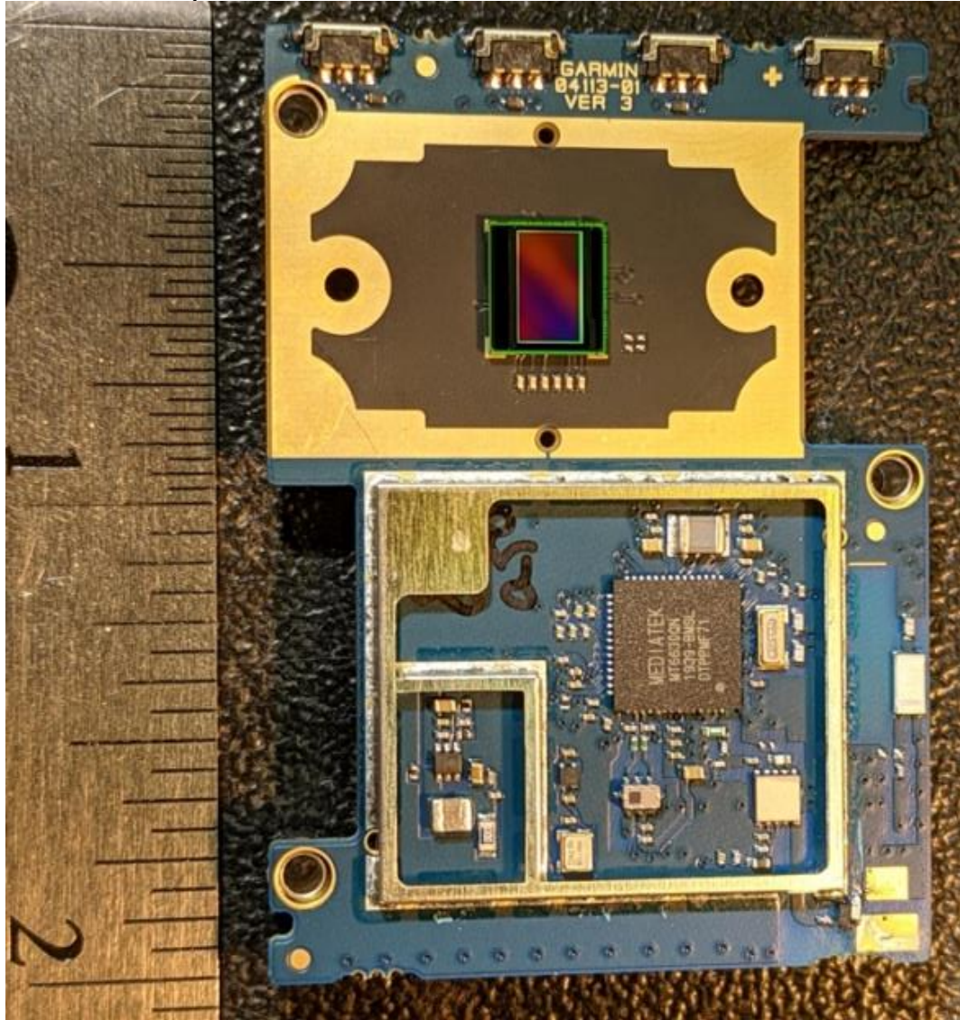
Sensor Board top side shield removed
