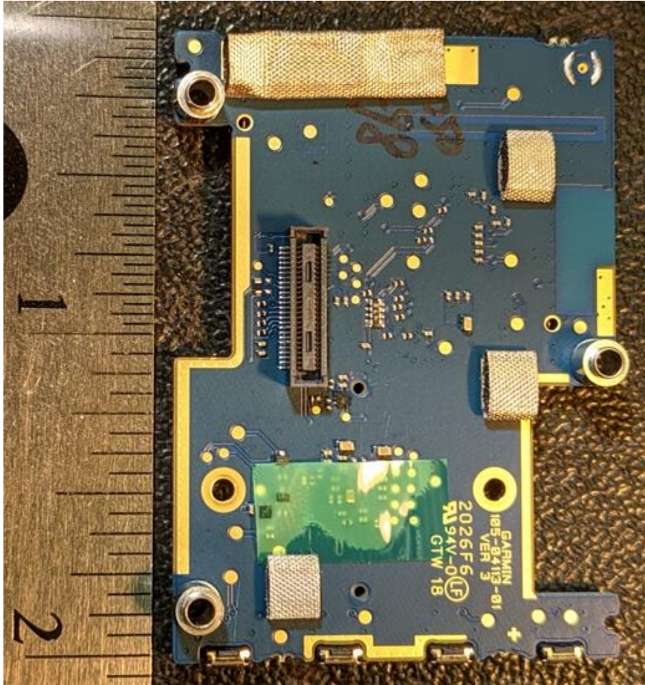
Sensor Board bottom side
