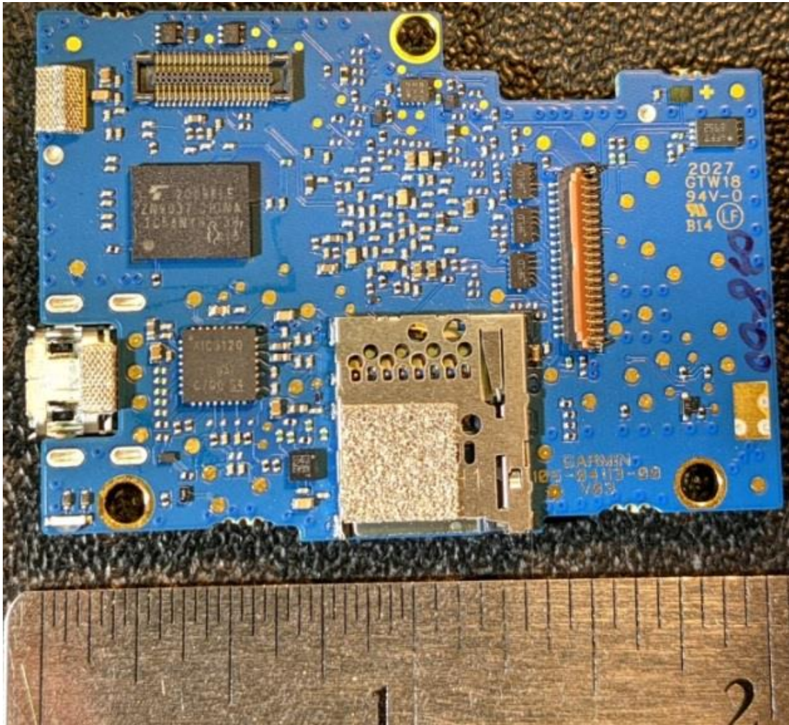
Main Board Bottom side
