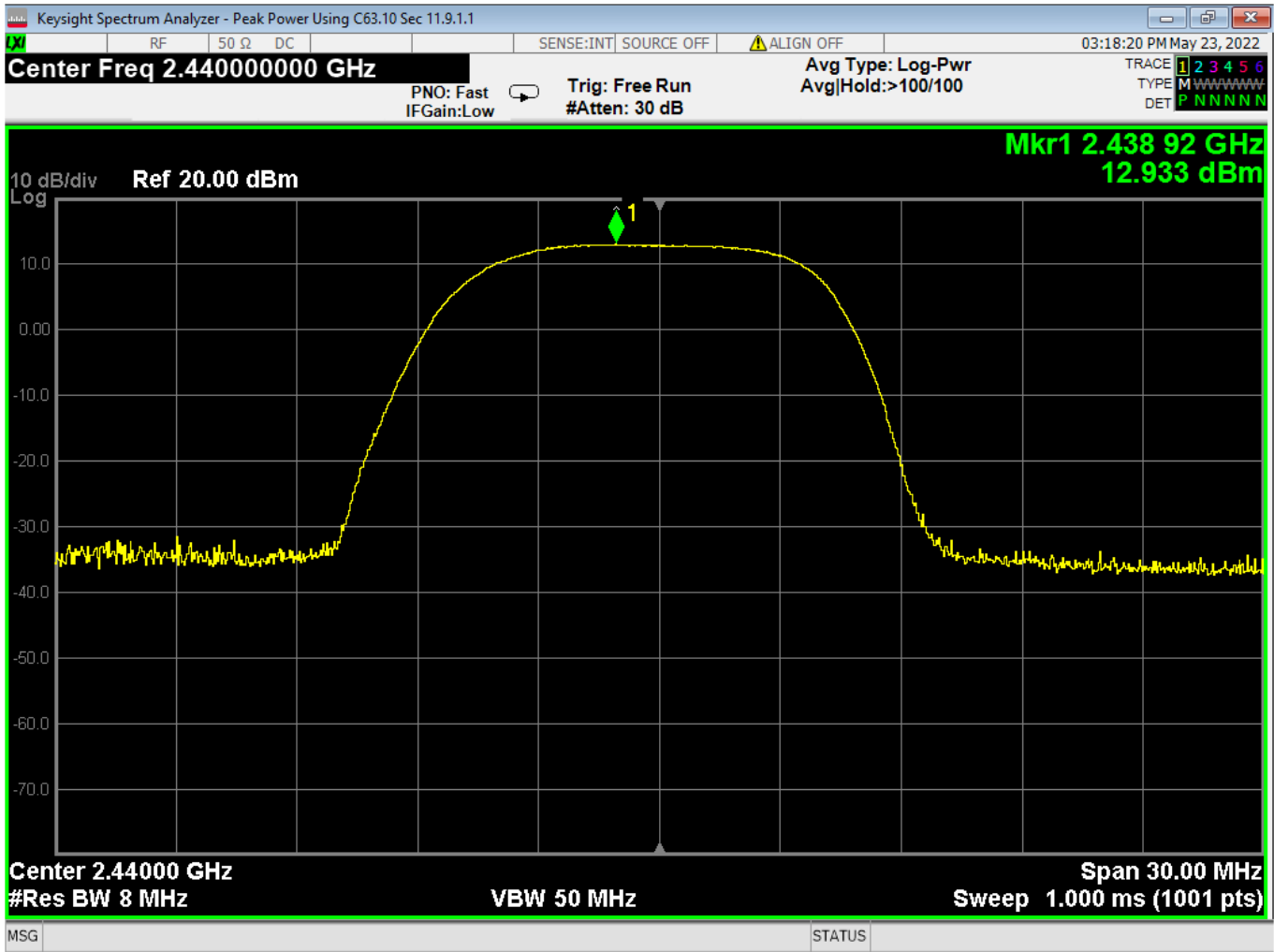
02 Peak Output Power, Mid Channel, 2EDR
