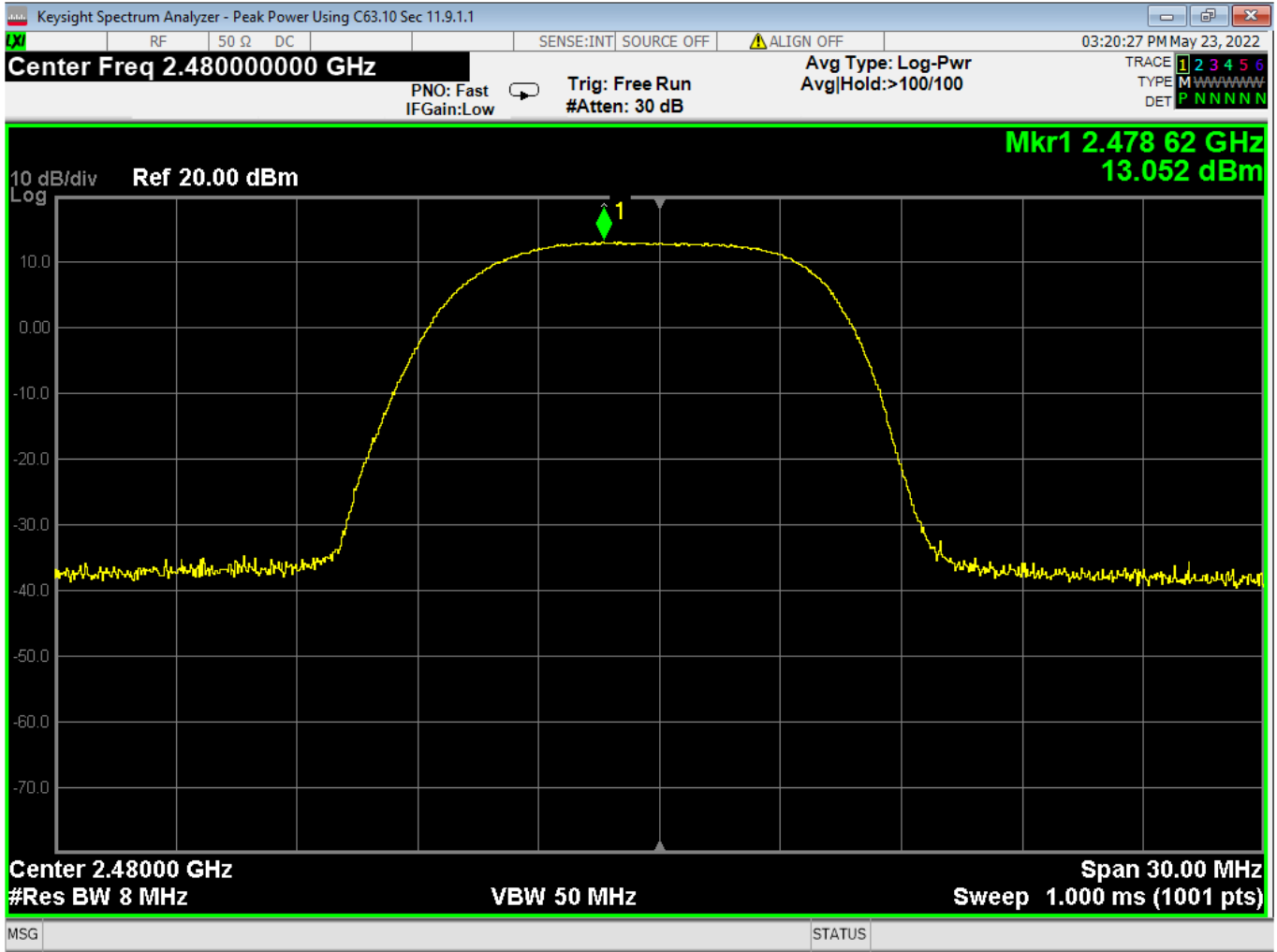
08 Peak Output Power, High Channel, 3EDR
