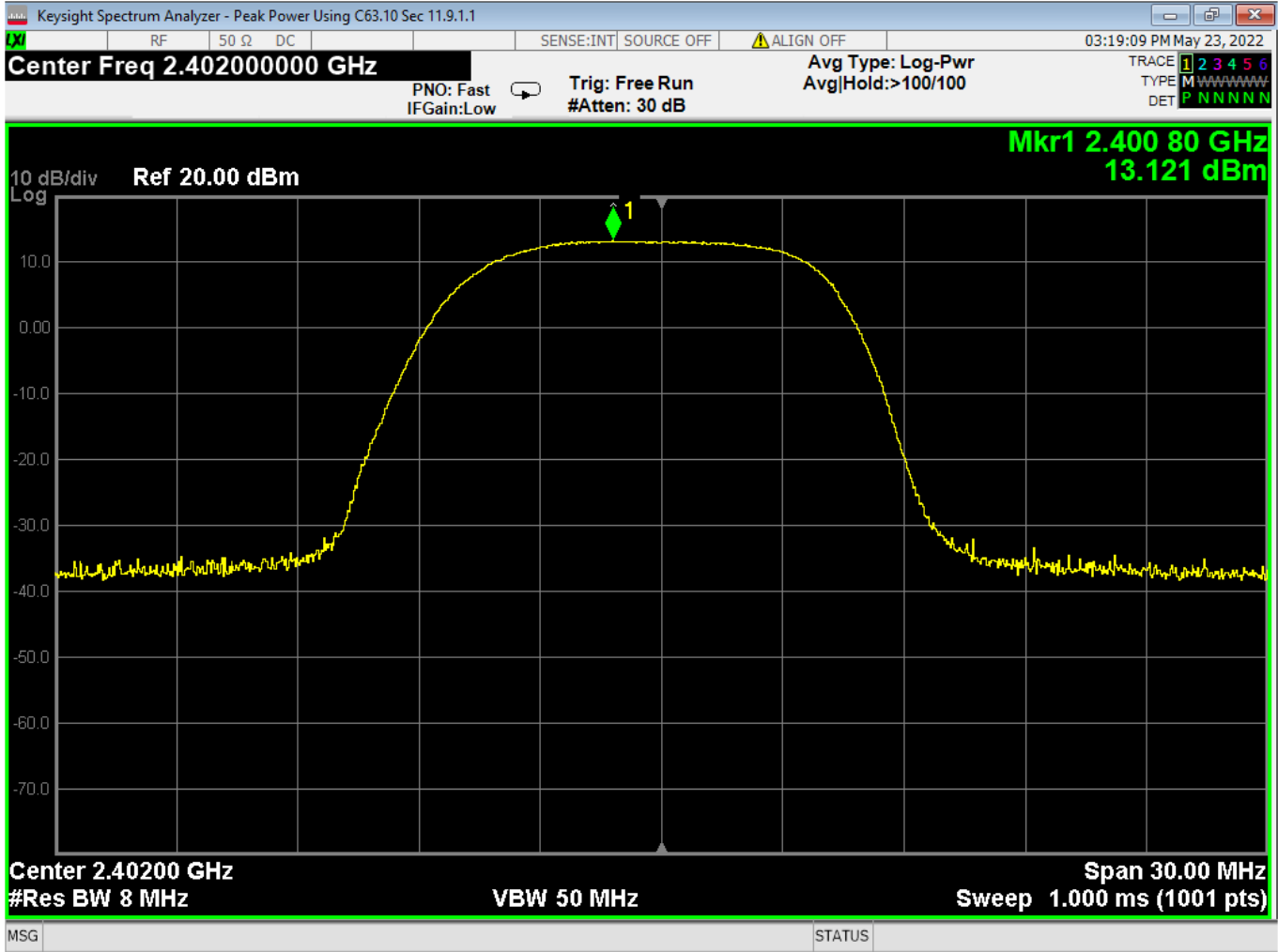
01 Peak Output Power, Low Channel, 2EDR
