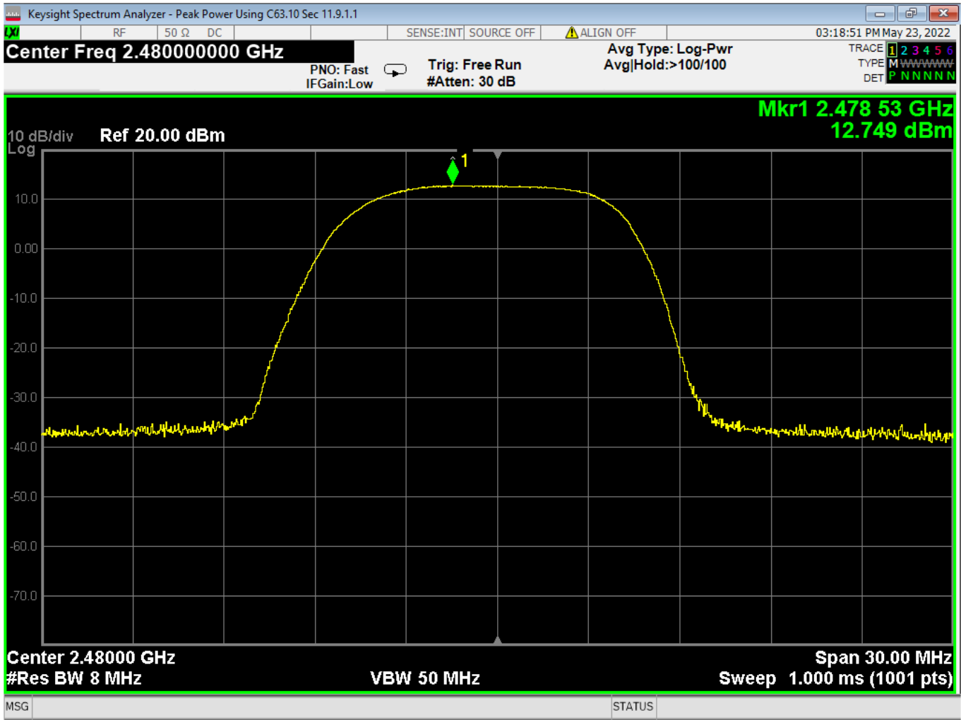
03 Peak Output Power, High Channel, 2EDR
