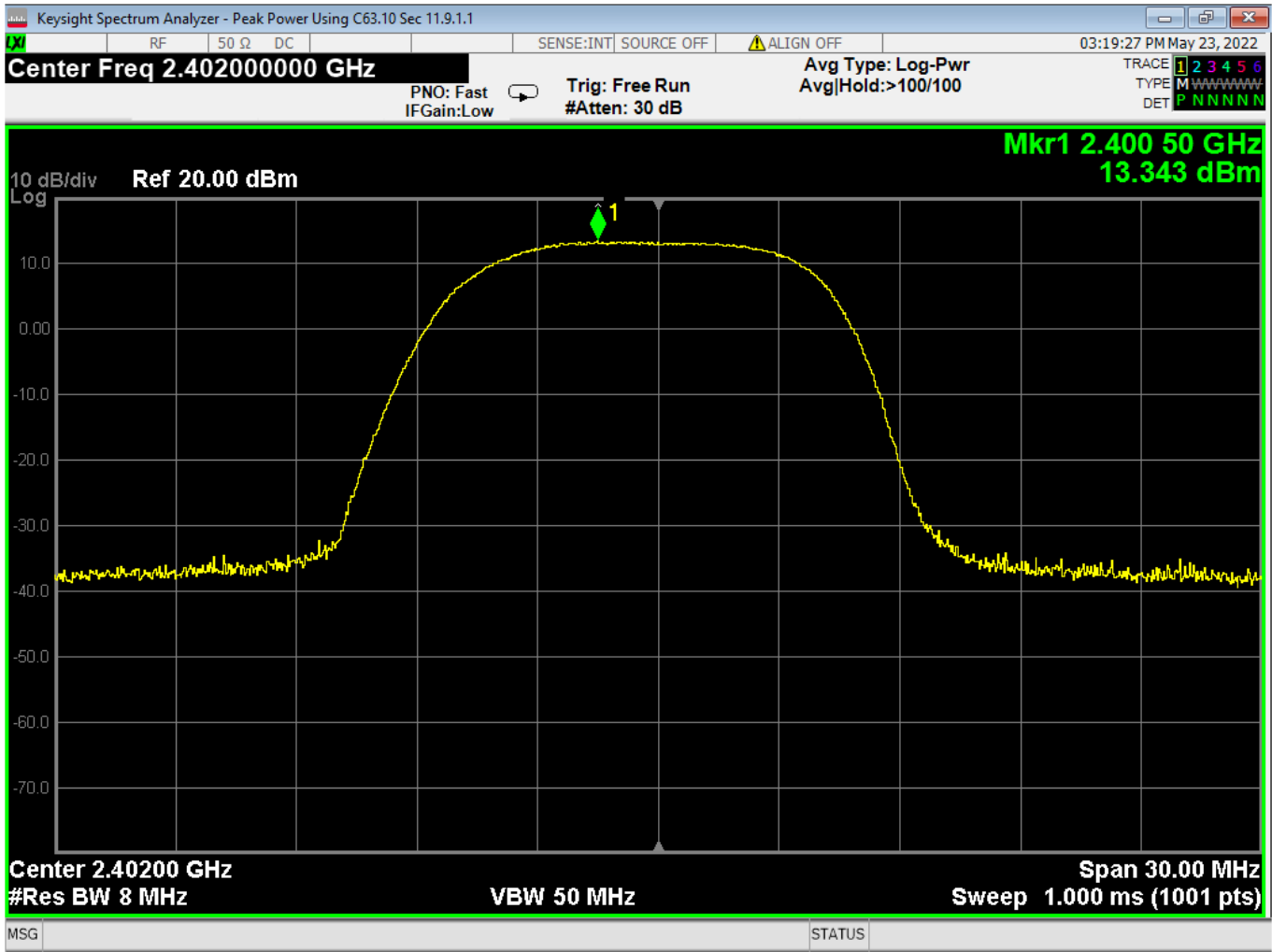
06 Peak Output Power, Low Channel, 3EDR
