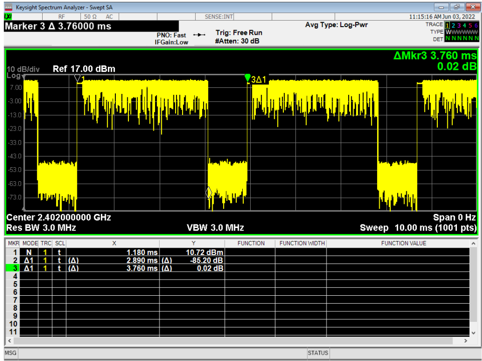
Figure 4 – 3EDR Duty Cycle DCCF (Duty Cycle Correction Factor) = 20 * Log(Duty Cycle / 100) -2.28 = 20 * Log(0.769)
