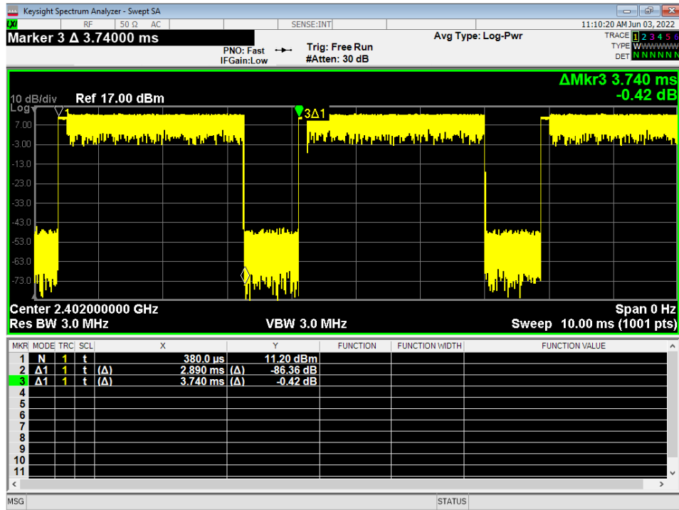
Figure 3 – 2EDR Duty Cycle
