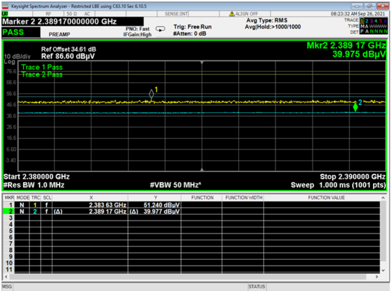
25 Lower Bandedge, Restricted, BLE 1MB
