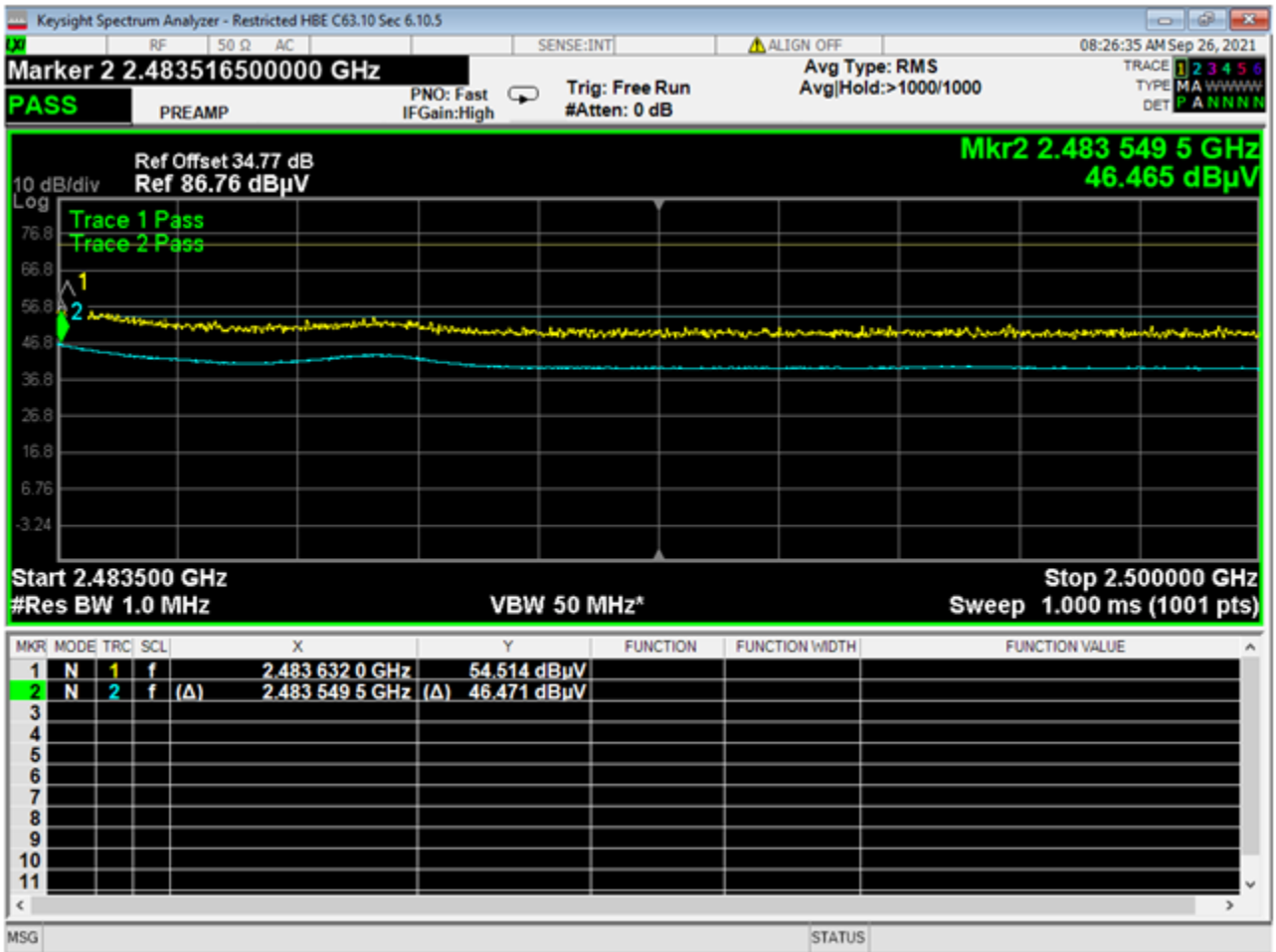
26 Higher Bandedge, Restricted, BLE 1MB
