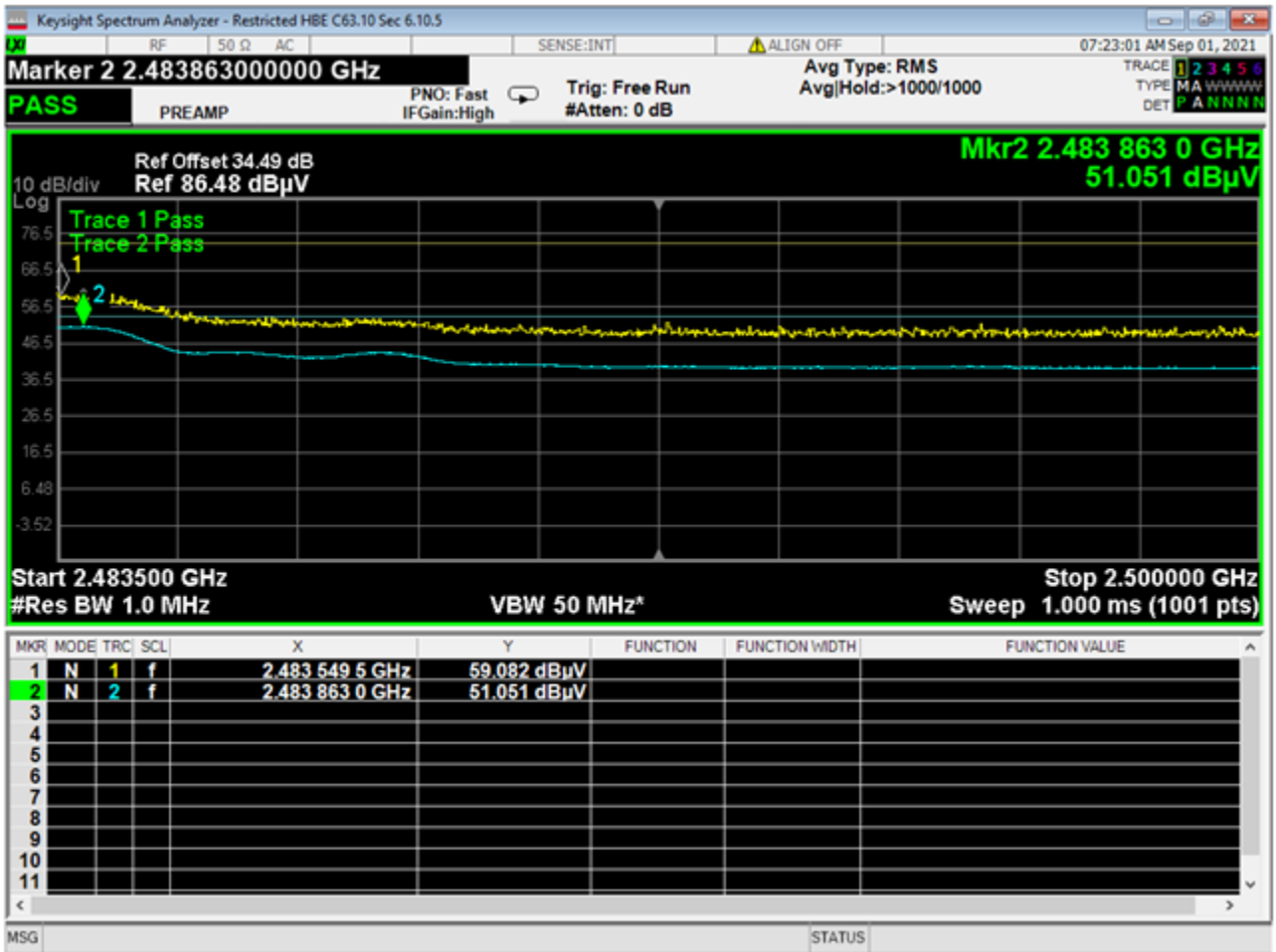
13 Higher Bandedge, Restricted, ANT
