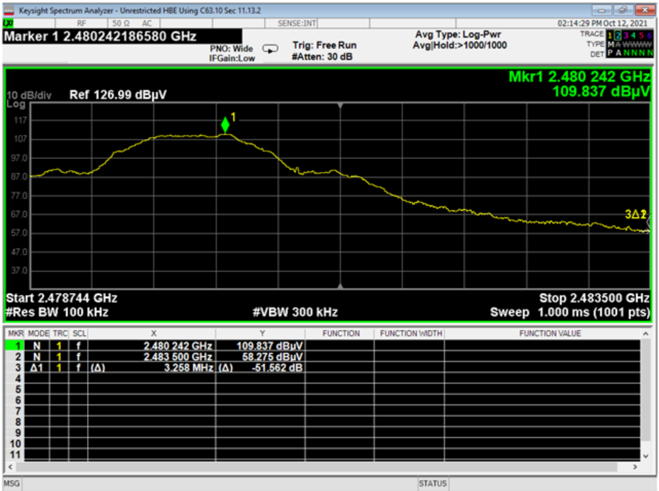
24 Higher Bandedge, Unrestricted, BLE 1MB
