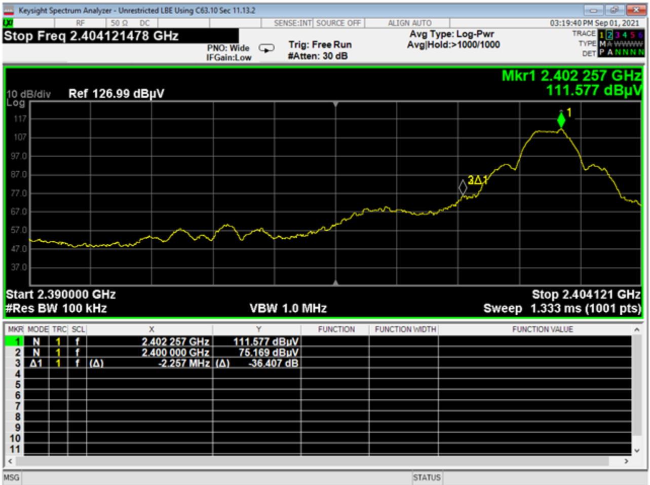
10 Lower Bandedge, Unrestricted, ANT
