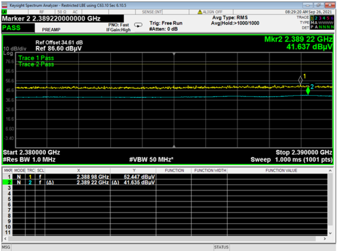
38 Lower Bandedge, Restricted, BLE 2MB
