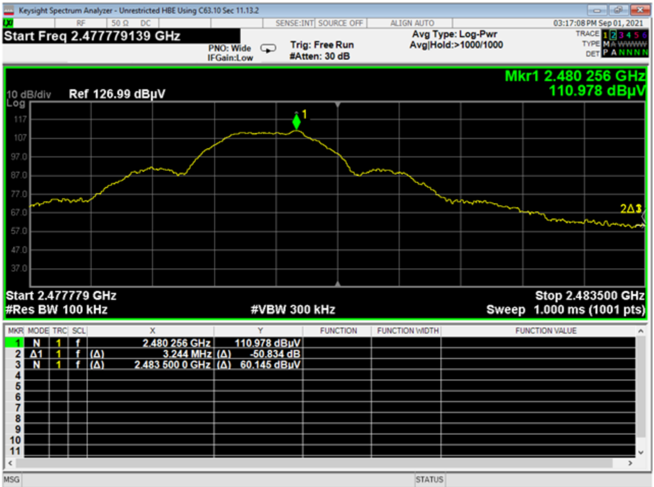
11 Higher Bandedge, Unrestricted, ANT
