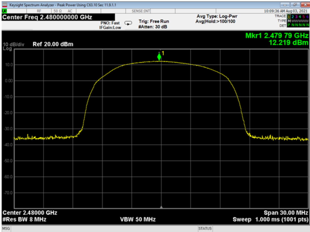
16 Peak Output Power, High, 3EDR
