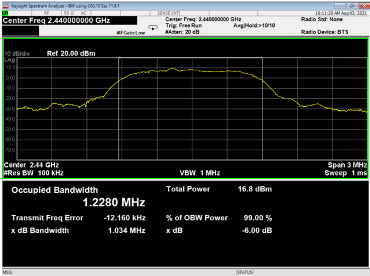
18 Bandwidth, Mid, 3EDR
