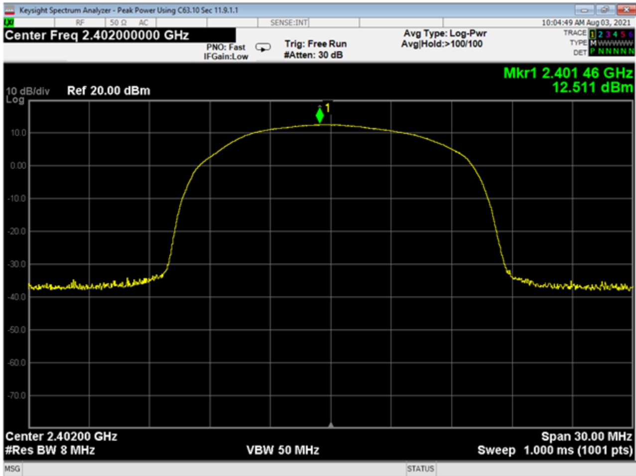
14 Peak Output Power, Low, 3EDR
