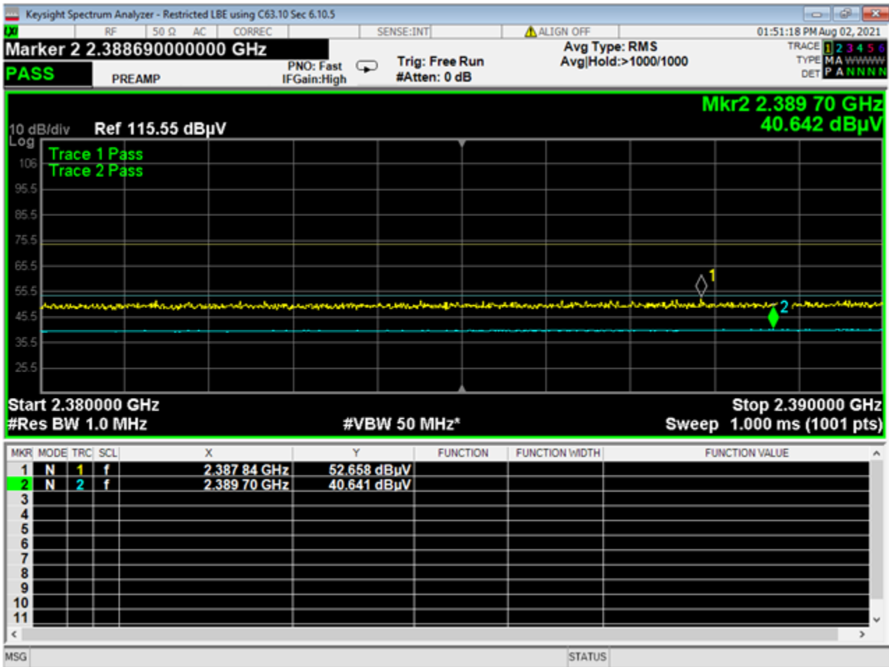
23 Lower Band Edge Restricted
