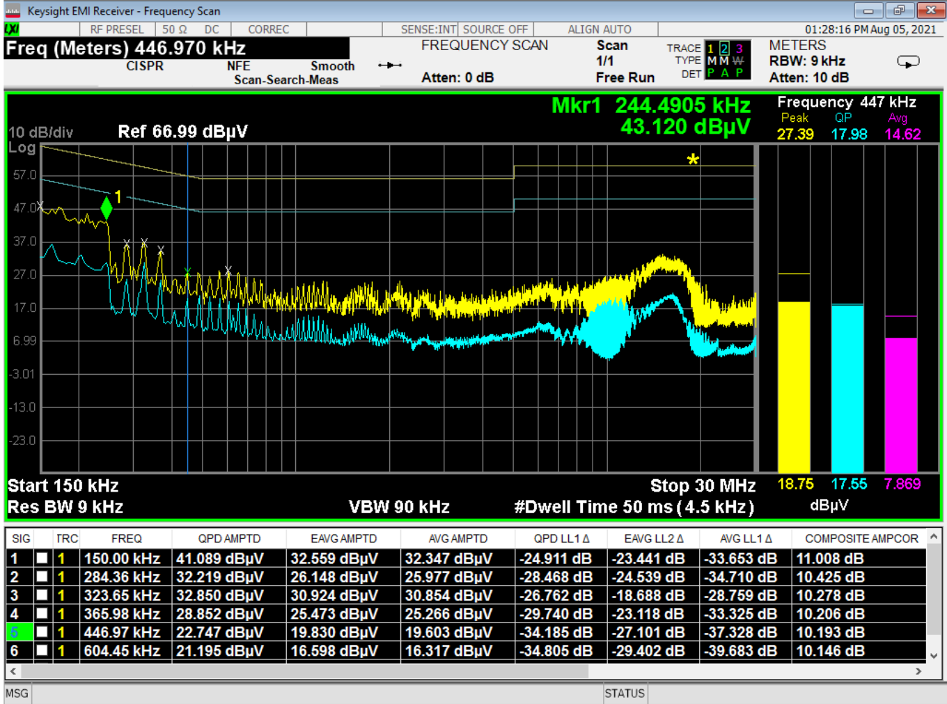
Figure 15 - Conducted Emissions Plot, Line, IDLE
