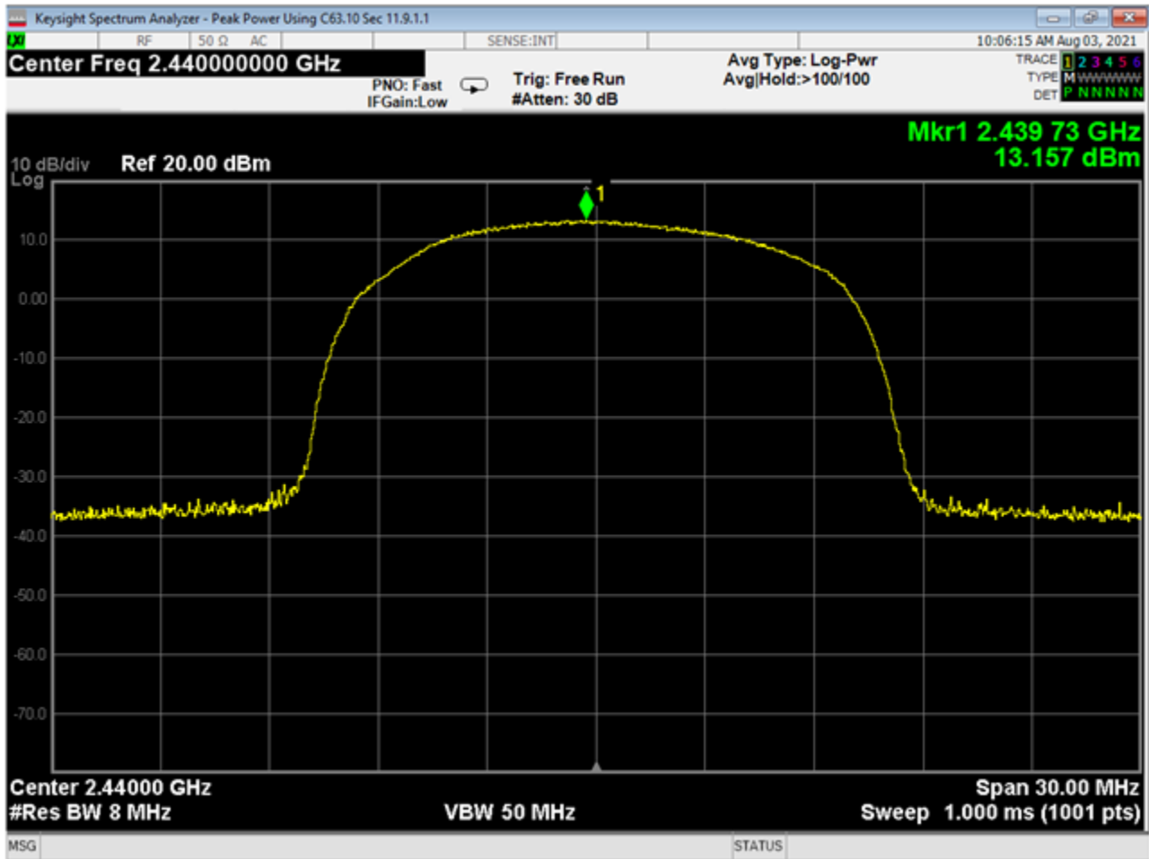
15 Peak Output Power, Mid, 3EDR
