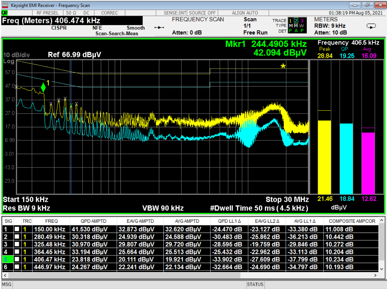
Figure 13 - Conducted Emissions Plot, Line, TX
