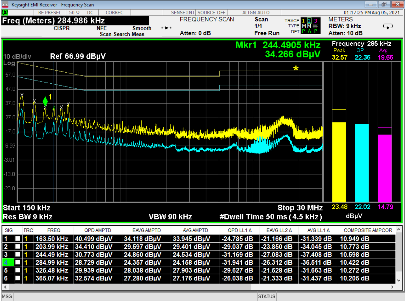
Figure 16 - Conducted Emissions Plot, Neutral, IDLE
