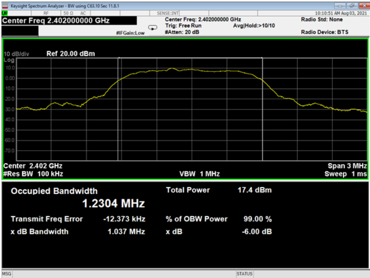
17 Bandwidth, Low, 3EDR
