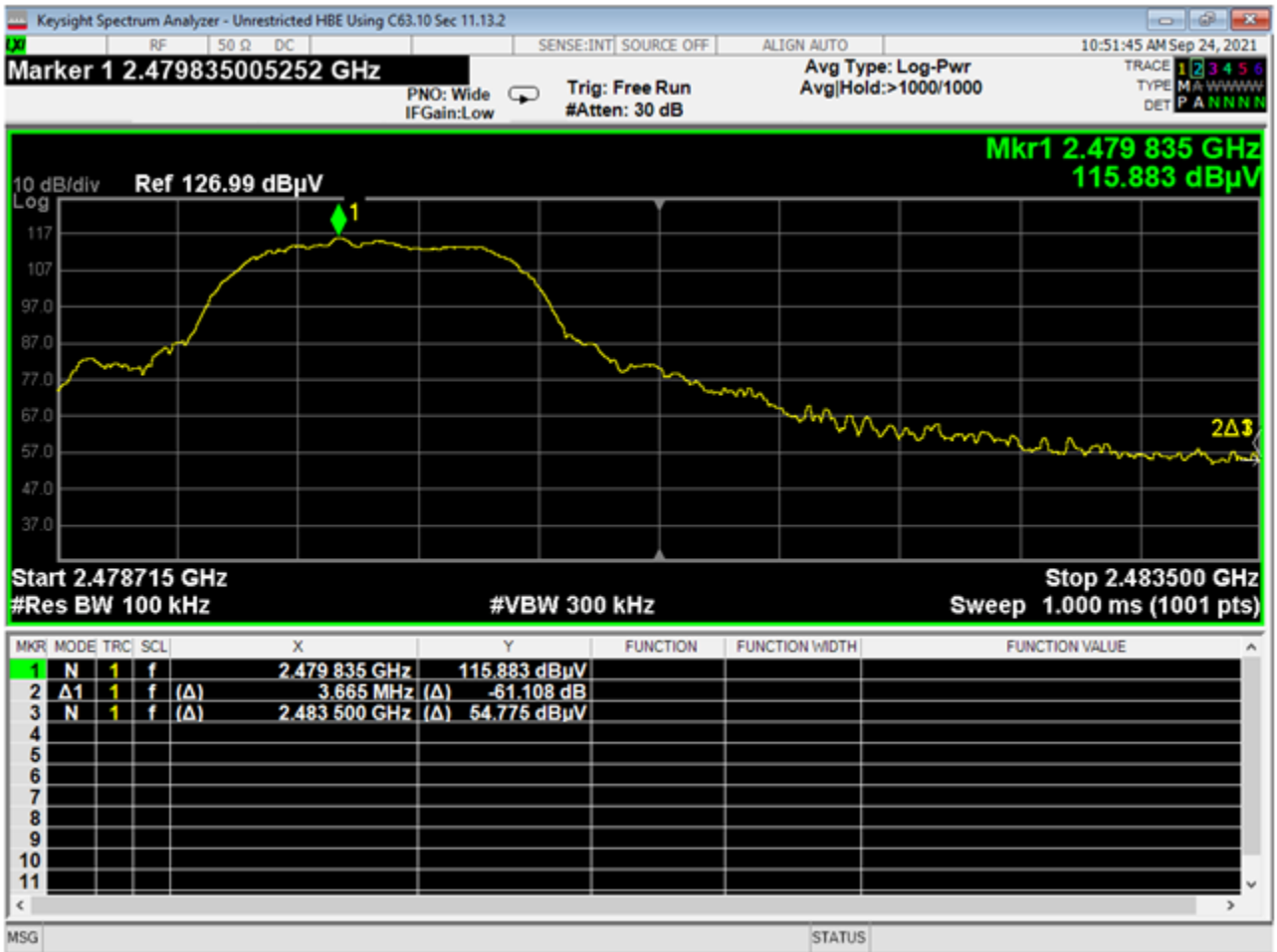
25 Higher Band Edge Unrestricted, 3EDR
