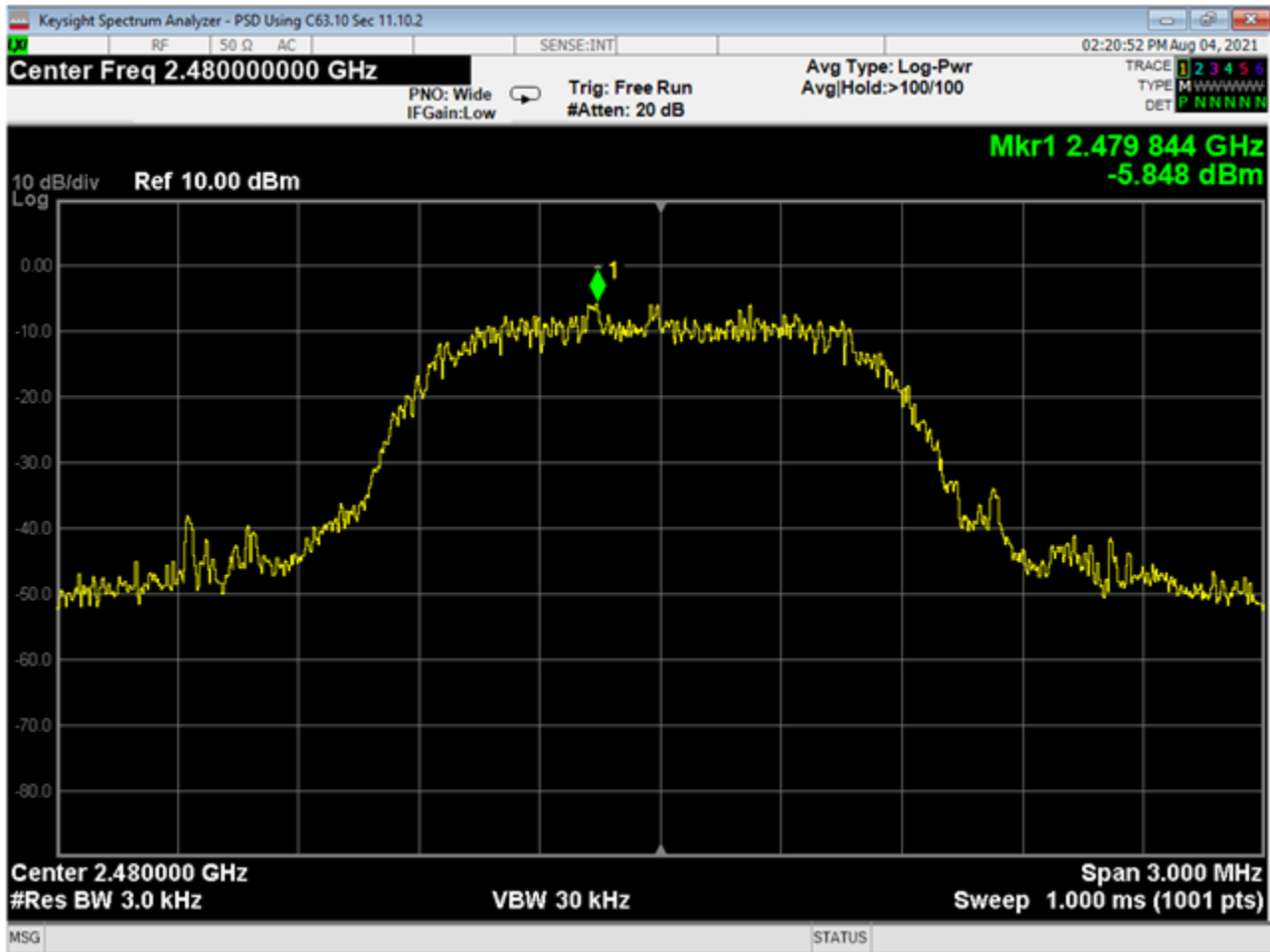
22 PSD, High, 3EDR
