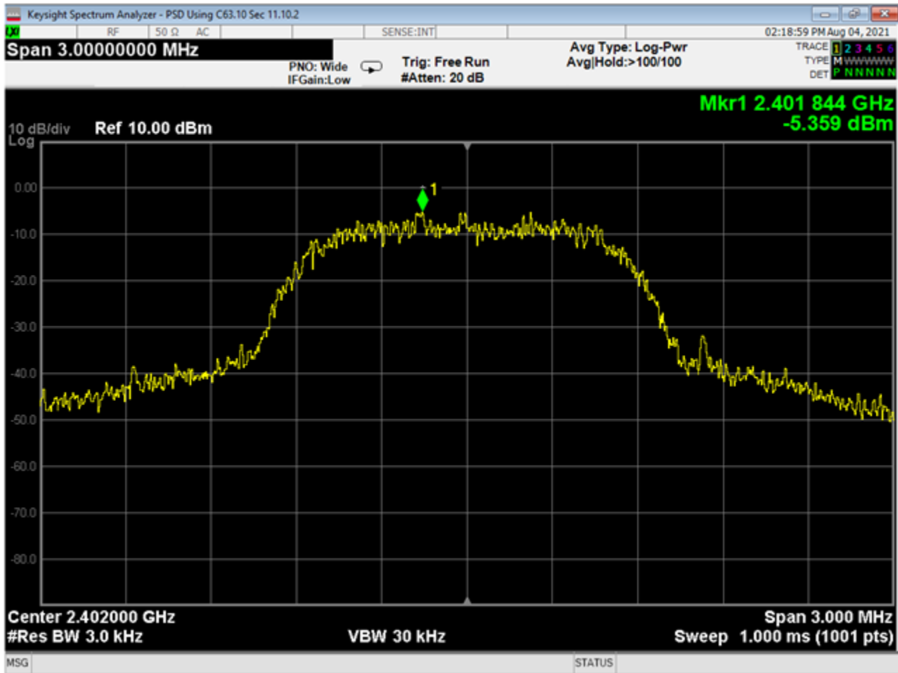
20 PSD, Low, 3EDR
