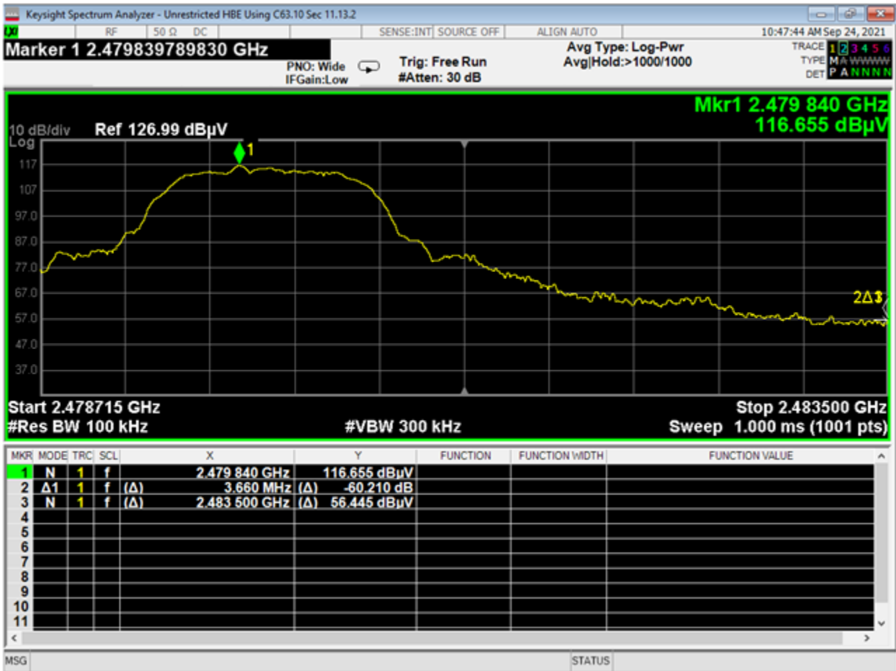
12 Higher Band Edge Unrestricted, 2EDR
