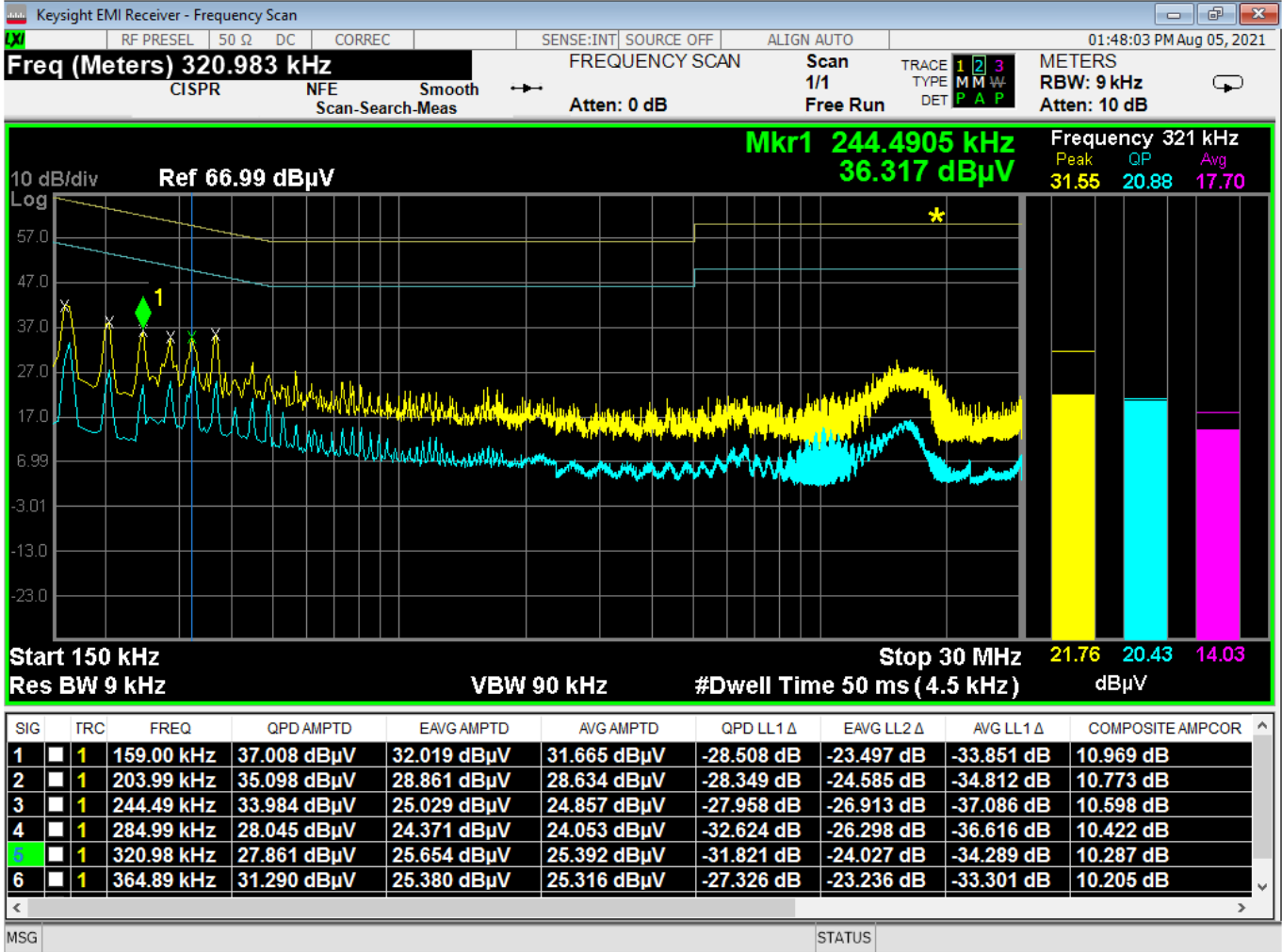
Figure 14 - Conducted Emissions Plot, Neutral, TX
