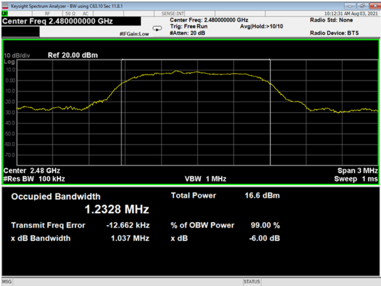
19 Bandwidth, High, 3EDR
