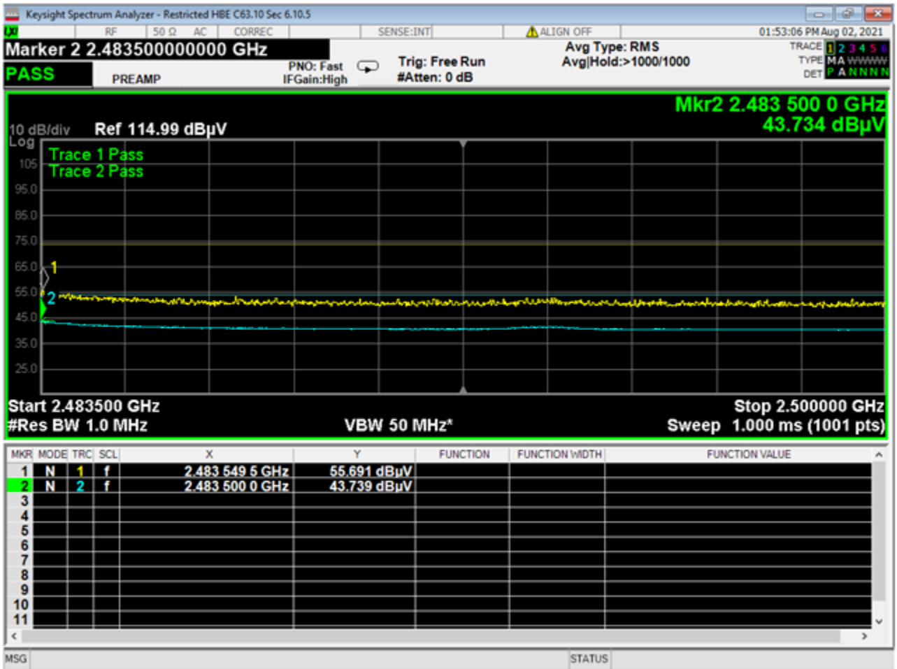
24 Higher Band Edge Restricted
