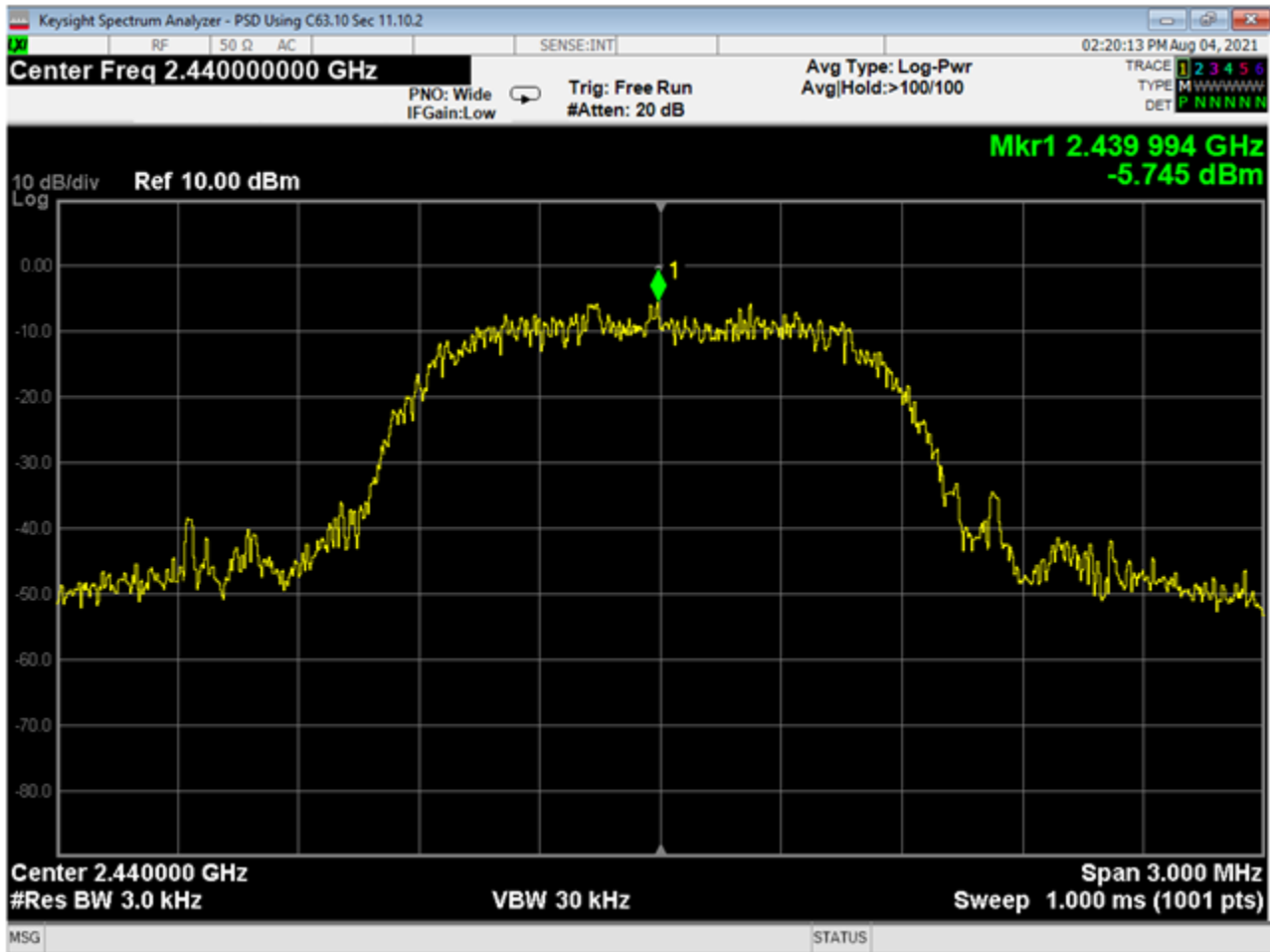
21 PSD, Mid, 3EDR
