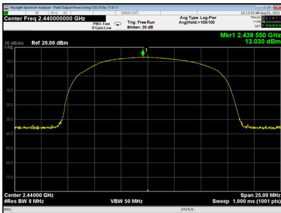
15 Peak Output Power, Mid Channel, 3EDR
