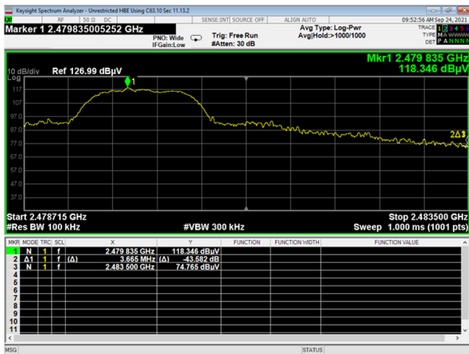
25 Higher Band Edge, Unrestricted, 3EDR
