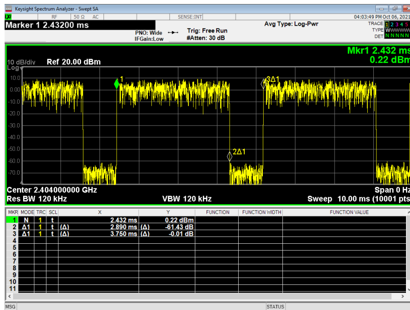
Figure 3 - Duty Cycle, 2EDR, 77.1% Duty Cycle
