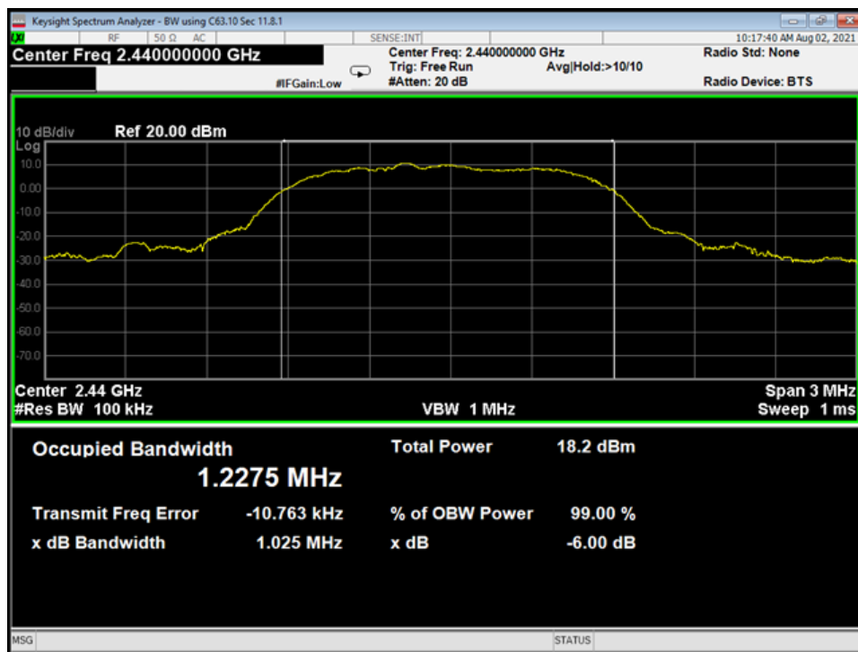
18 Bandwidth, Mid Channel, 3EDR
