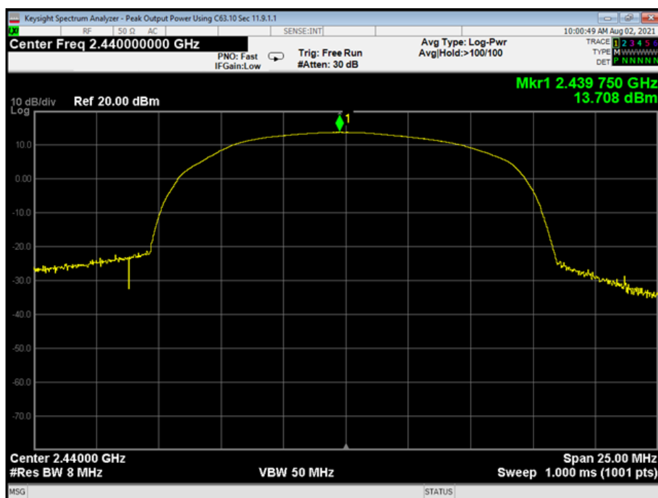
02 Peak Output Power, Mid Channel, 2EDR
