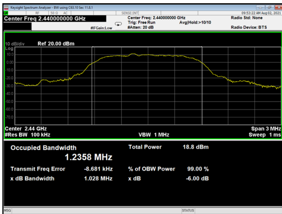
05 Bandwidth, Mid Channel, 2EDR
