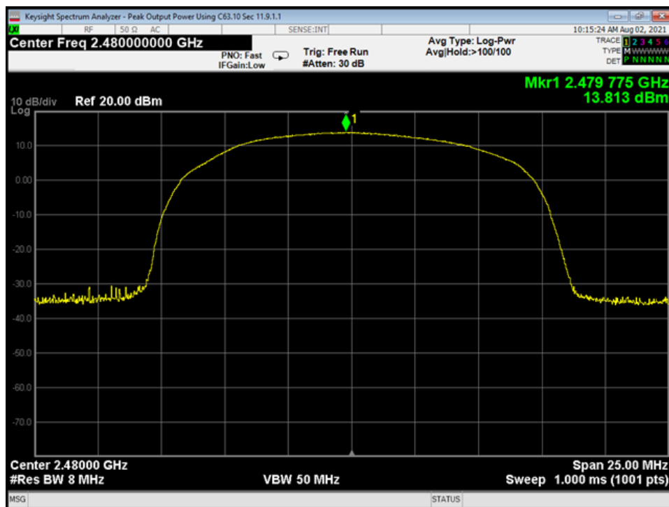
16 Peak Output Power, High Channel, 3EDR
