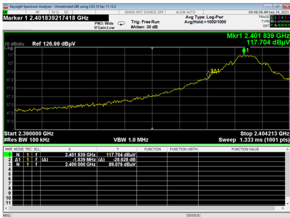
13 Lower Band Edge, Unrestricted, 2EDR
