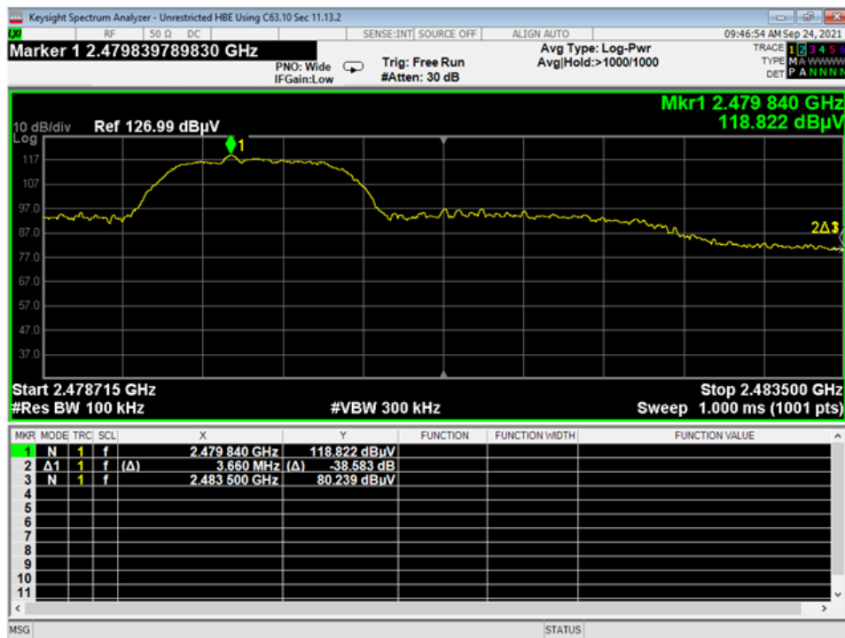
12 Higher Band Edge, Unrestricted, 2EDR
