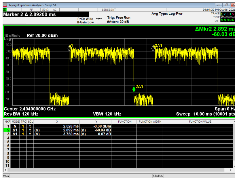
Figure 4 – Duty Cycle, 3EDR, 77.1% Duty Cycle
