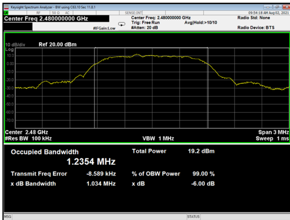
06 Bandwidth, High Channel, 2EDR
