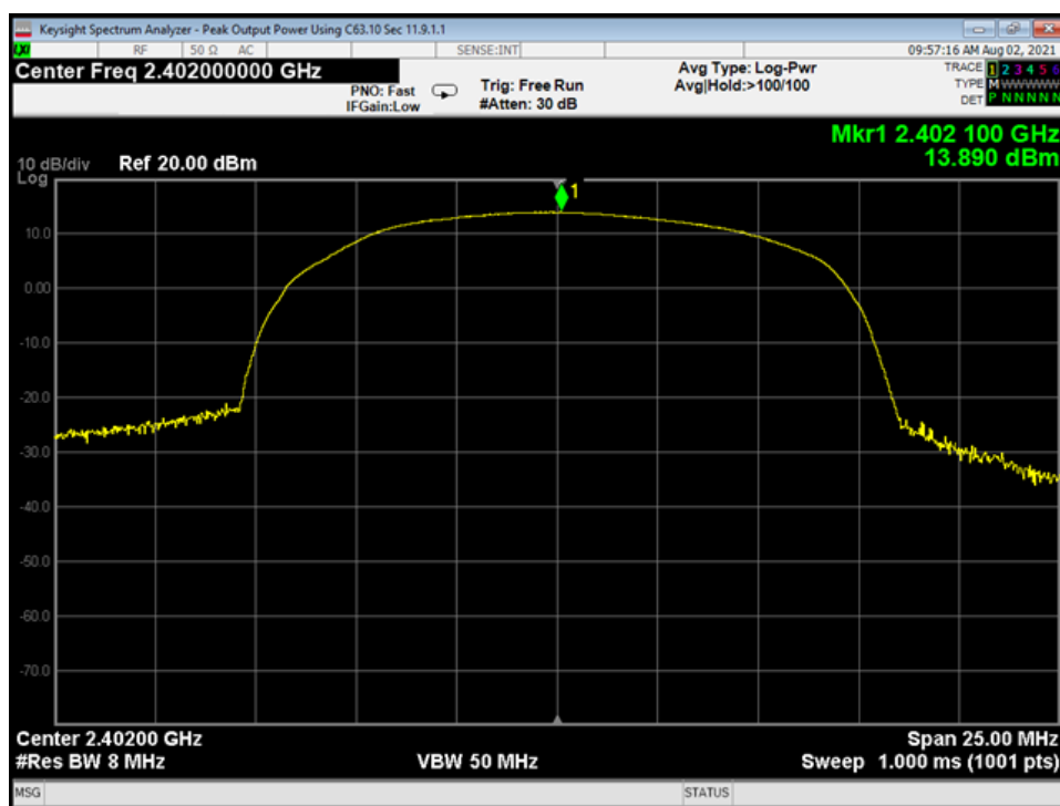
01 Peak Output Power, Low Channel, 2EDR
