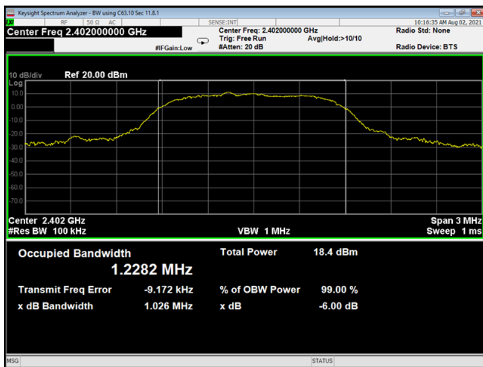
17 Bandwidth, Low Channel, 3EDR
