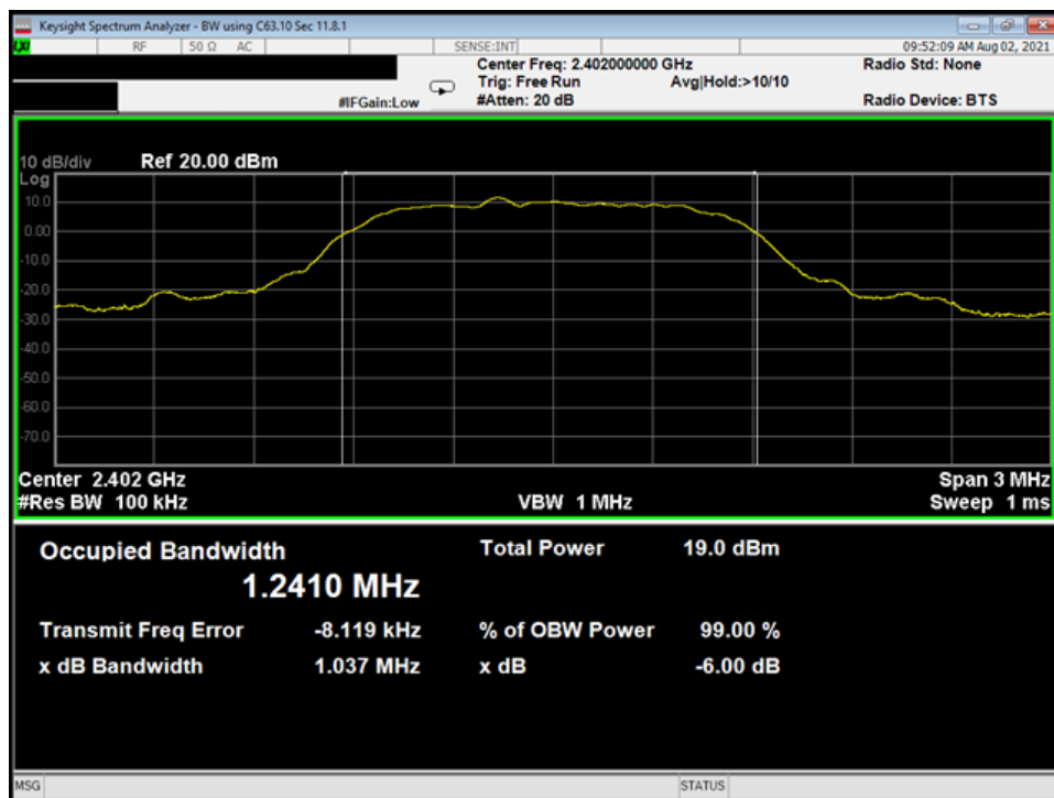
04 Bandwidth, Low Channel, 2EDR
