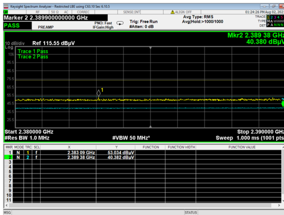
23 Lower Band Edge Restricted, 3EDR
