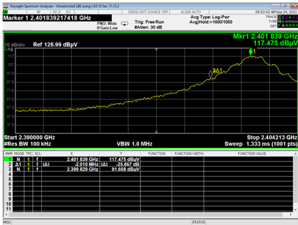
26 Lower Band Edge, Unrestricted, 3EDR
