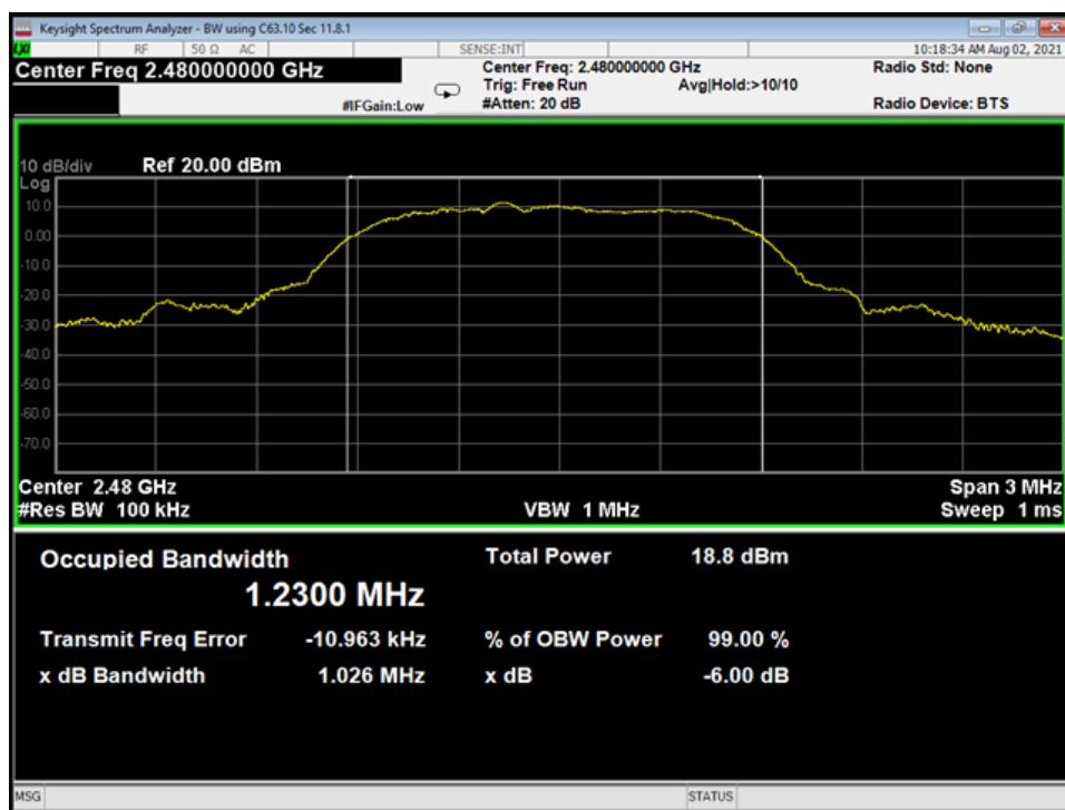
19 Bandwidth, High Channel, 3EDR
