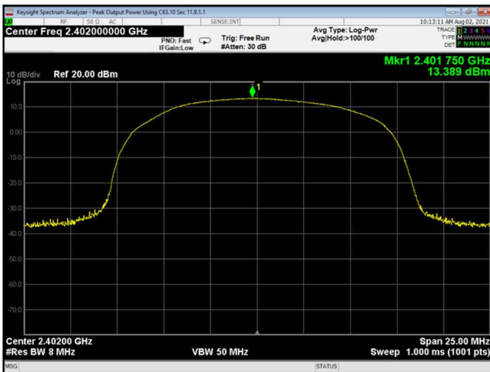
14 Peak Output Power, Low Channel, 3EDR
