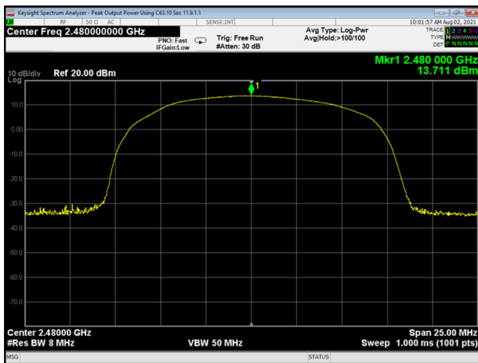
03 Peak Output Power, High Channel, 2EDR
