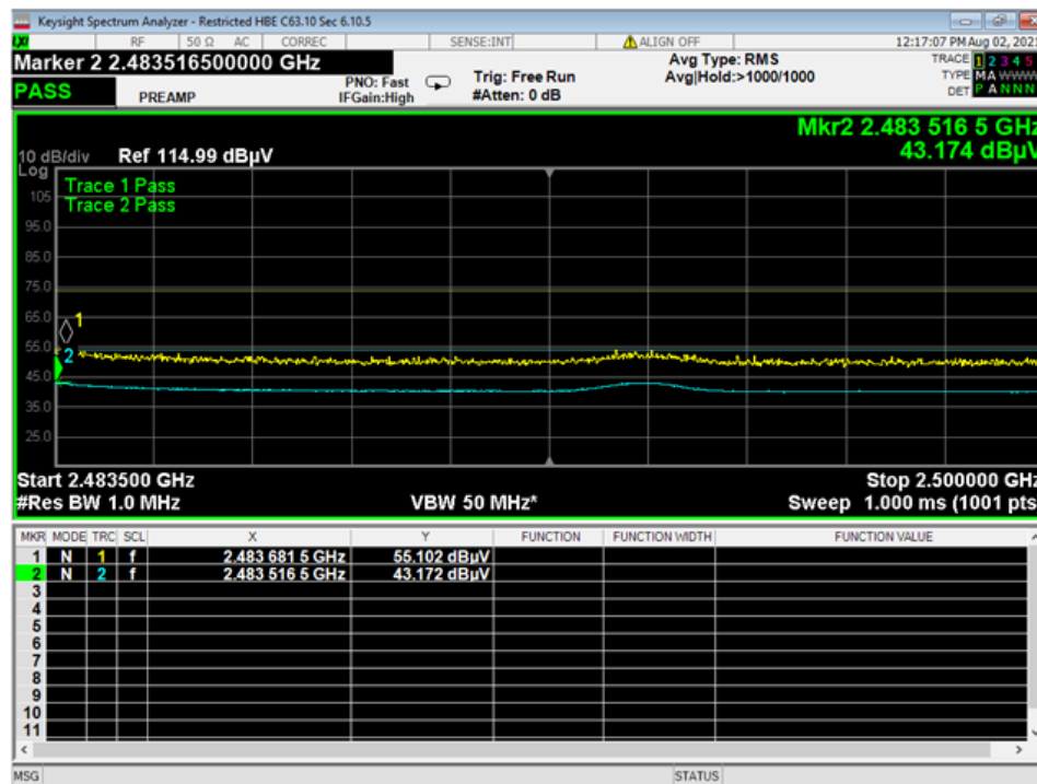
24 Higher Band Edge Restricted, 3EDR
